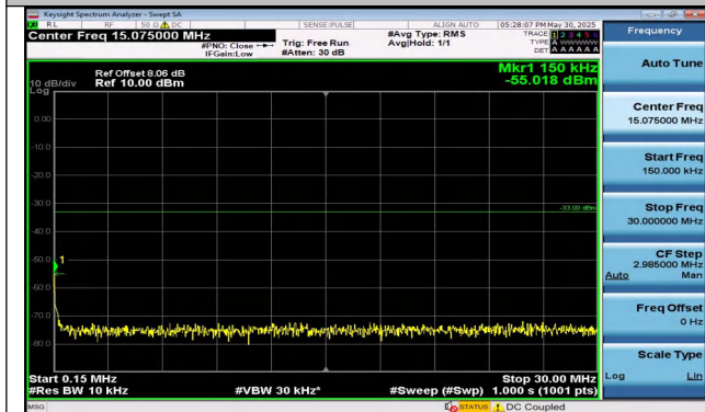
Band25-10MHz-QPSK-26640-1RB#49-0.15~30-PASS
