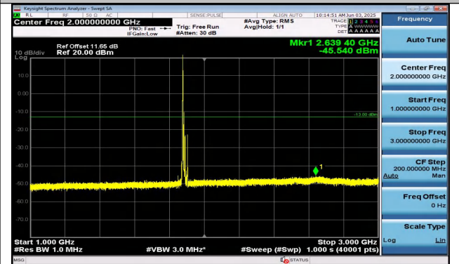
Band25-15MHz-QPSK-26365-1RB#0-1000~3000-PASS
