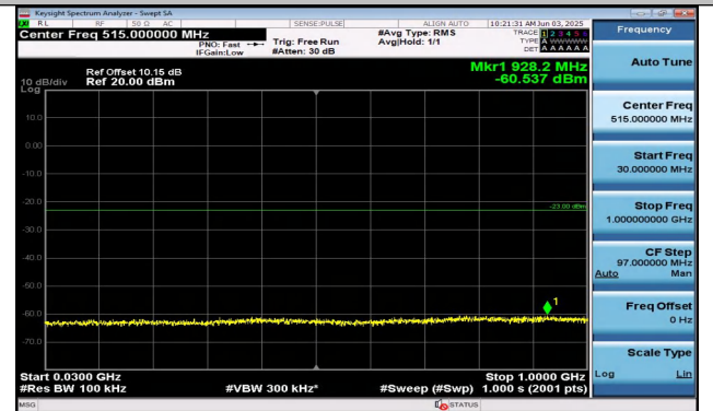
Band25-15MHz-QPSK-26115-75RB#0-30~1000-PASS
