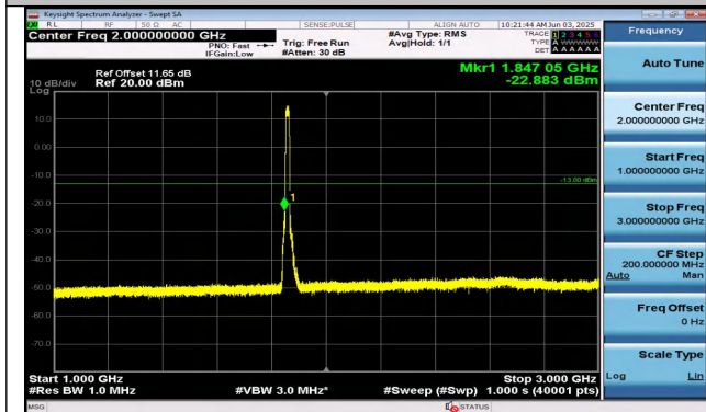
Band25-15MHz-QPSK-26115-75RB#0-1000~3000-PASS
