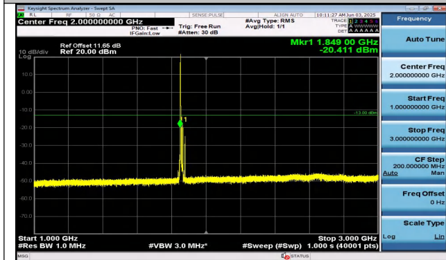
Band25-15MHz-QPSK-26115-1RB#0-1000~3000-PASS
