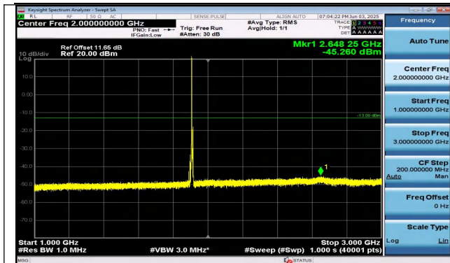
Band25-10MHz-16QAM-26640-1RB#0-1000~3000-PASS
