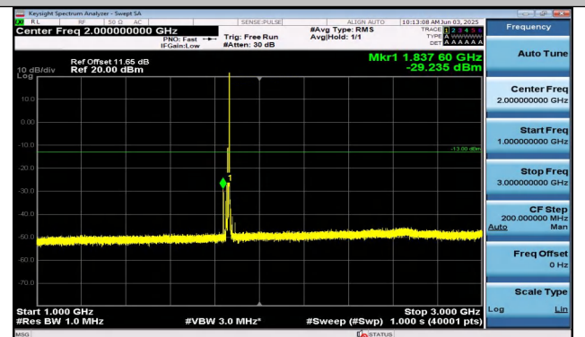
Band25-15MHz-QPSK-26115-1RB#74-1000~3000-PASS
