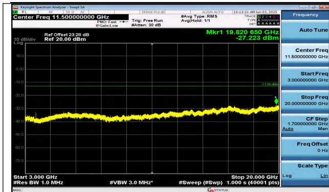
Band25-15MHz-QPSK-26115-1RB#74-3000~20000-PASS
