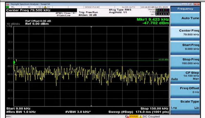
Band25-15MHz-QPSK-26365-1RB#74-0.009~0.15-PASS
