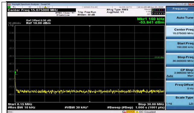
Band25-15MHz-QPSK-26115-1RB#0-0.15~30-PASS
