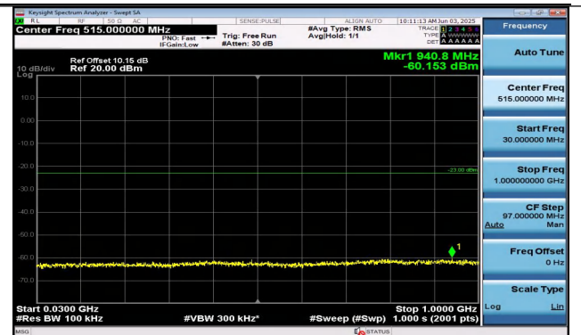
Band25-15MHz-QPSK-26115-1RB#0-30~1000-PASS
