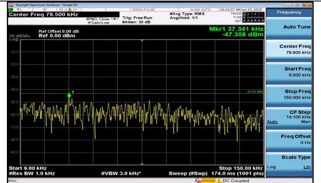
Band25-15MHz-QPSK-26115-1RB#0-0.009~0.15-PASS
