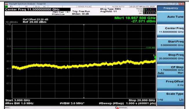
Band25-15MHz-QPSK-26115-75RB#0-3000~20000-PASS
