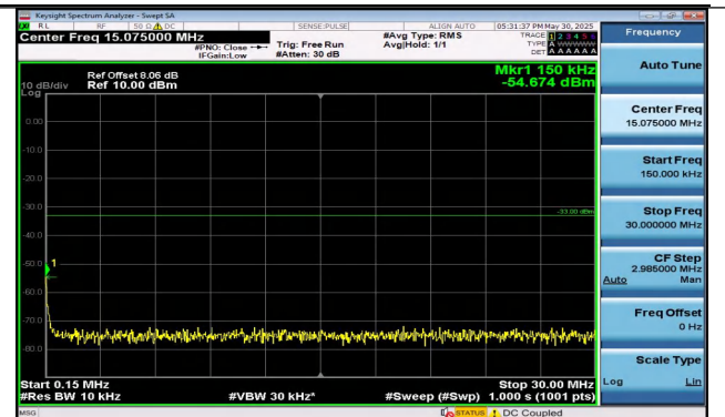
Band25-10MHz-QPSK-26640-50RB#0-0.15~30-PASS
