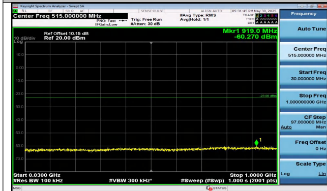
Band25-10MHz-QPSK-26640-50RB#0-30~1000-PASS
