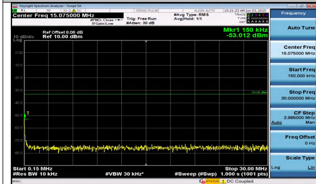
Band25-15MHz-QPSK-26115-75RB#0-0.15~30-PASS
