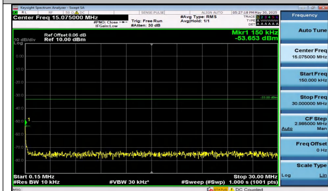
Band25-10MHz-16QAM-26640-1RB#0-0.15~30-PASS
