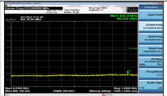
Band25-15MHz-QPSK-26365-1RB#74-30~1000-PASS
