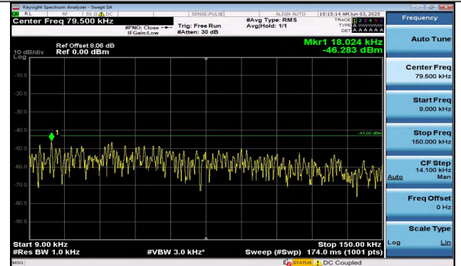
Band25-15MHz-16QAM-26365-1RB#0-0.009~0.15-PASS
