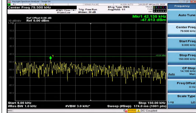
Band25-15MHz-QPSK-26365-75RB#0-0.009~0.15-PASS
