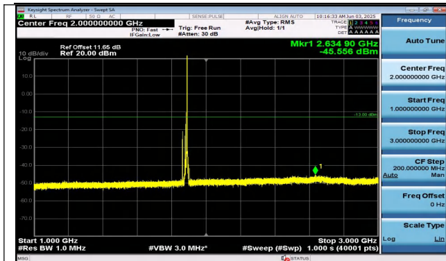
Band25-15MHz-QPSK-26365-1RB#74-1000~3000-PASS
