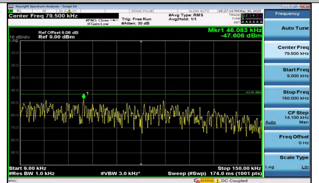
Band25-10MHz-16QAM-26640-1RB#0-0.009~0.15-PASS
