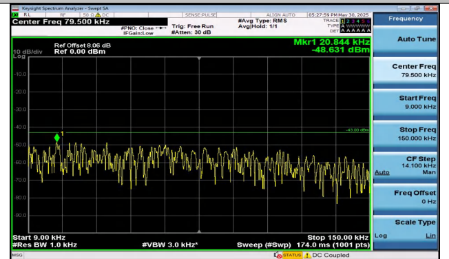
Band25-10MHz-QPSK-26640-1RB#49-0.009~0.15-PASS
