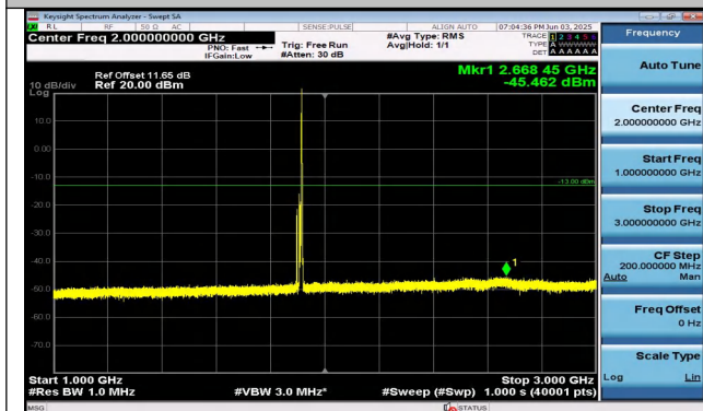
Band25-10MHz-QPSK-26640-1RB#49-1000~3000-PASS
