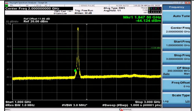
Band25-15MHz-QPSK-26365-75RB#0-1000~3000-PASS
