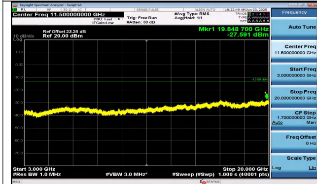
Band25-15MHz-QPSK-26365-75RB#0-3000~20000-PASS
