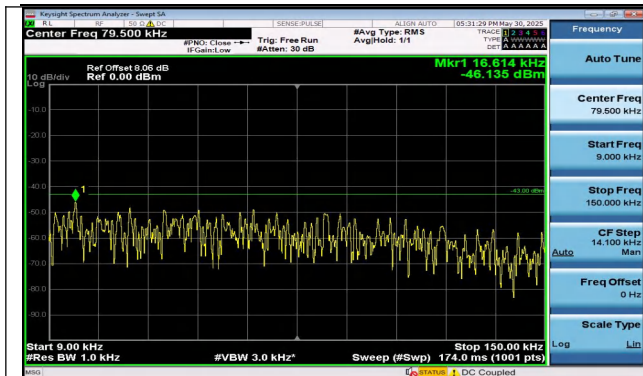
Band25-10MHz-QPSK-26640-50RB#0-0.009~0.15-PASS
