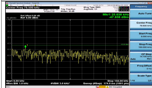
Band25-15MHz-QPSK-26115-1RB#74-0.009~0.15-PASS
