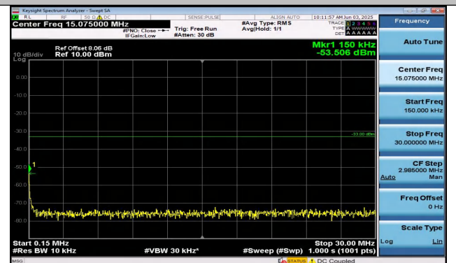
Band25-15MHz-16QAM-26115-1RB#0-0.15~30-PASS
