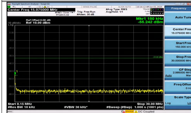
Band25-15MHz-QPSK-26365-1RB#74-0.15~30-PASS
