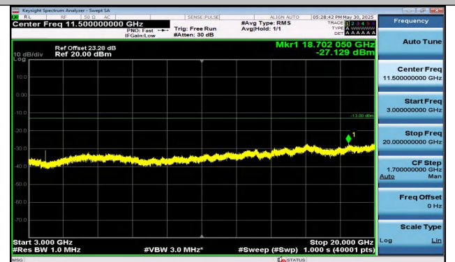
Band25-10MHz-QPSK-26640-1RB#49-3000~20000-PASS
