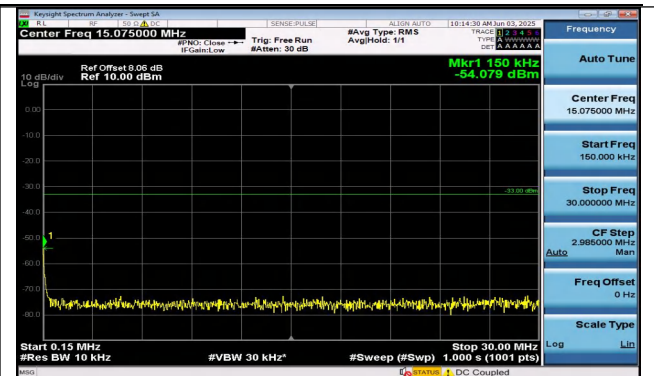
Band25-15MHz-QPSK-26365-1RB#0-0.15~30-PASS
