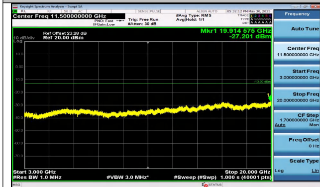
Band25-10MHz-QPSK-26640-50RB#0-3000~20000-PASS
