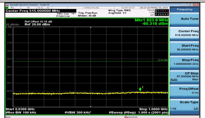
Band25-10MHz-16QAM-26640-1RB#0-30~1000-PASS
