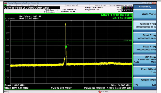
Band25-10MHz-QPSK-26640-50RB#0-1000~3000-PASS
