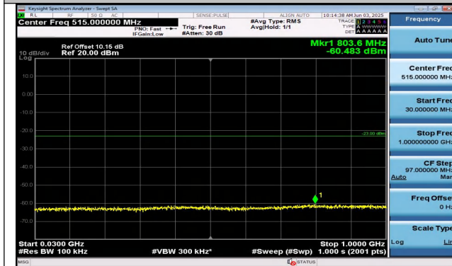
Band25-15MHz-QPSK-26365-1RB#0-30~1000-PASS
