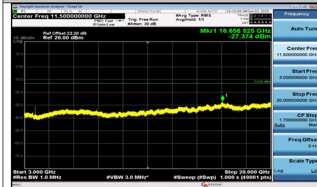
Band25-15MHz-QPSK-26365-1RB#0-3000~20000-PASS
