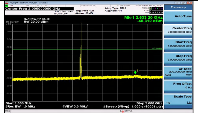
Band25-10MHz-16QAM-26640-1RB#49-1000~3000-PASS
