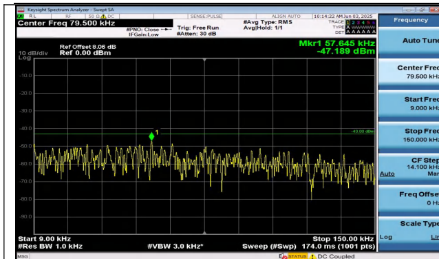
Band25-15MHz-QPSK-26365-1RB#0-0.009~0.15-PASS
