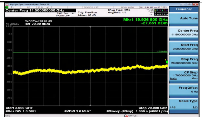
Band25-15MHz-QPSK-26365-1RB#74-3000~20000-PASS
