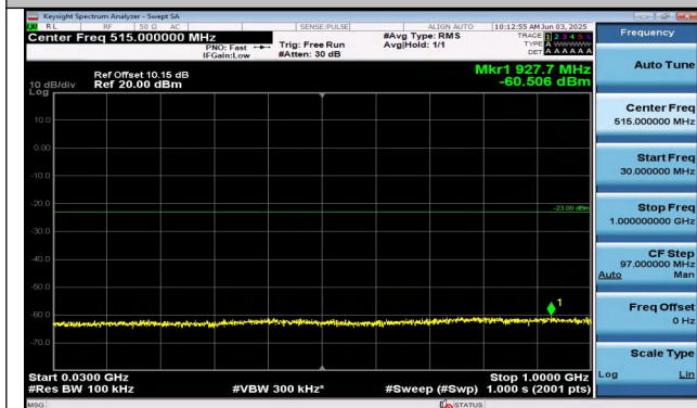
Band25-15MHz-QPSK-26115-1RB#74-30~1000-PASS
