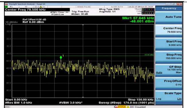
Band25-15MHz-QPSK-26115-75RB#0-0.009~0.15-PASS
