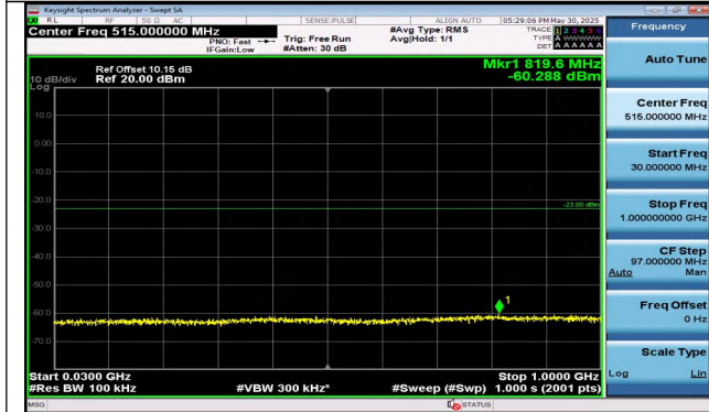
Band25-10MHz-16QAM-26640-1RB#49-30~1000-PASS
