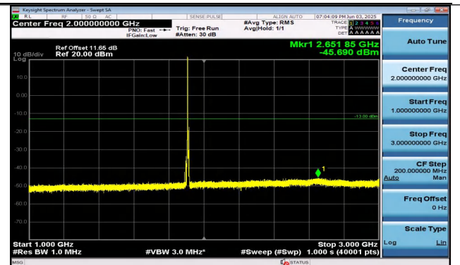
Band25-10MHz-QPSK-26640-1RB#0-1000~3000-PASS
