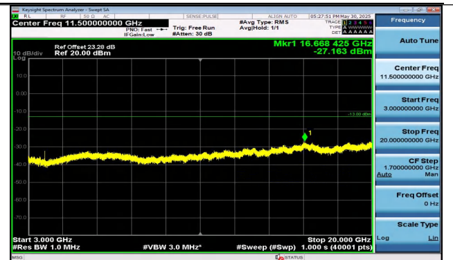
Band25-10MHz-16QAM-26640-1RB#0-3000~20000-PASS
