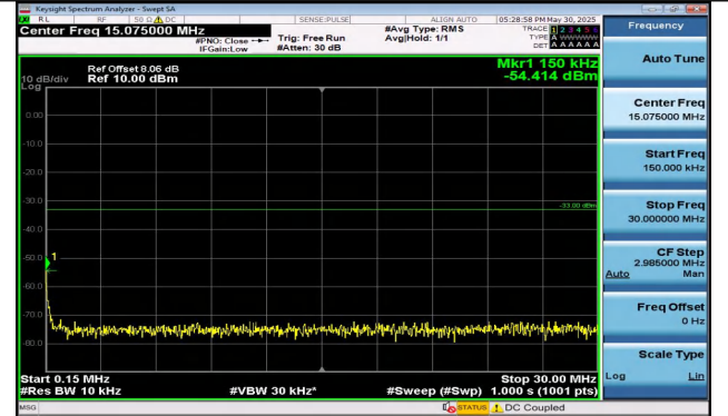
Band25-10MHz-16QAM-26640-1RB#49-0.15~30-PASS
