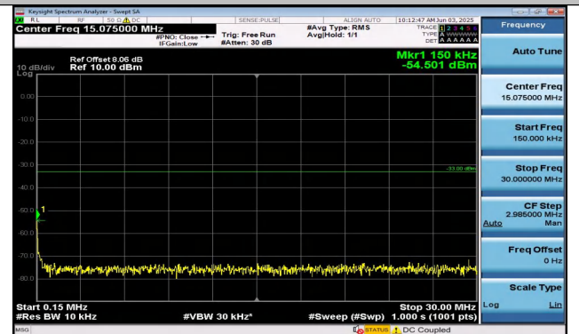
Band25-15MHz-QPSK-26115-1RB#74-0.15~30-PASS
