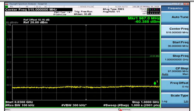
Band25-10MHz-QPSK-26640-1RB#49-30~1000-PASS
