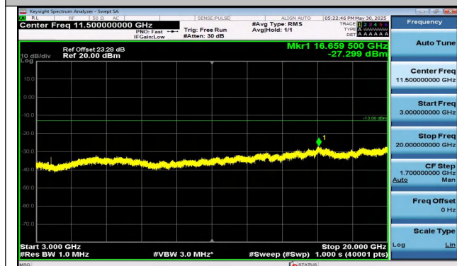
Band25-10MHz-16QAM-26090-1RB#49-3000~20000-PASS
