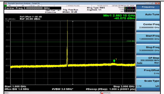
Band25-5MHz-16QAM-26665-1RB#24-1000~3000-PASS
