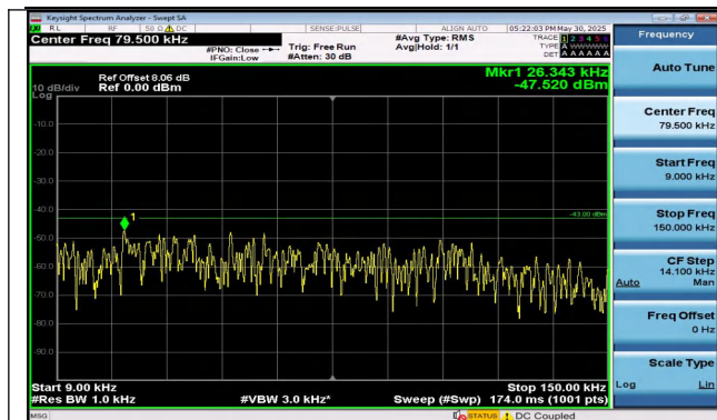
Band25-10MHz-16QAM-26090-1RB#49-0.009~0.15-PASS
