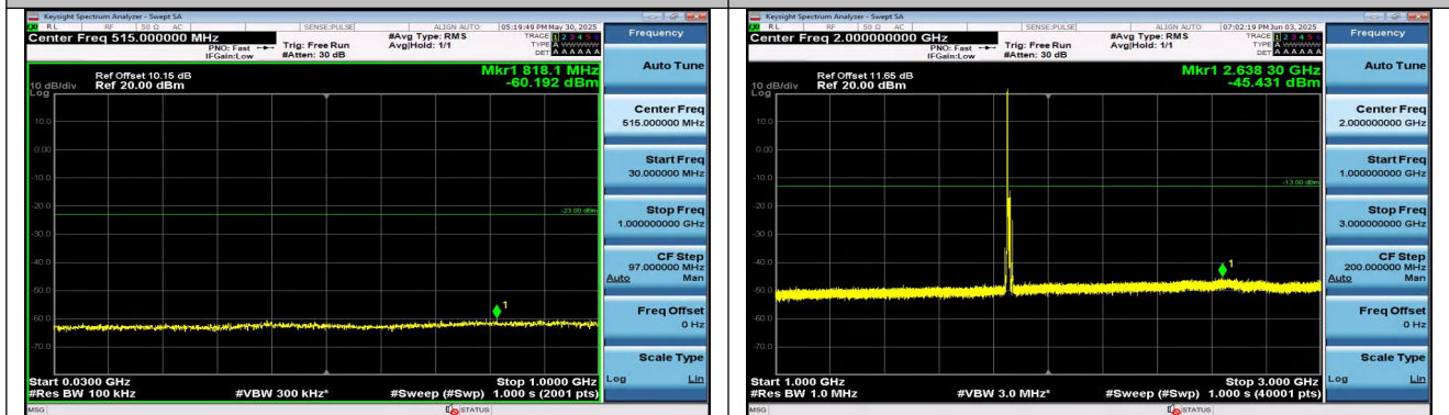
Band25-10MHz-QPSK-26090-1RB#0-30~1000-PASS
