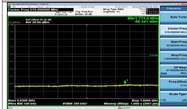
Band25-10MHz-16QAM-26090-1RB#49-30~1000-PASS
