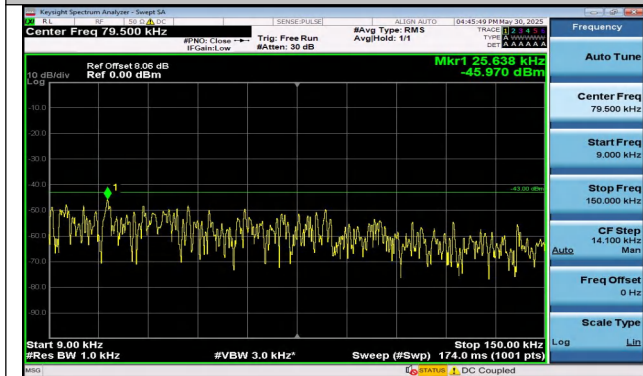
Band25-5MHz-16QAM-26665-1RB#24-0.009~0.15-PASS
