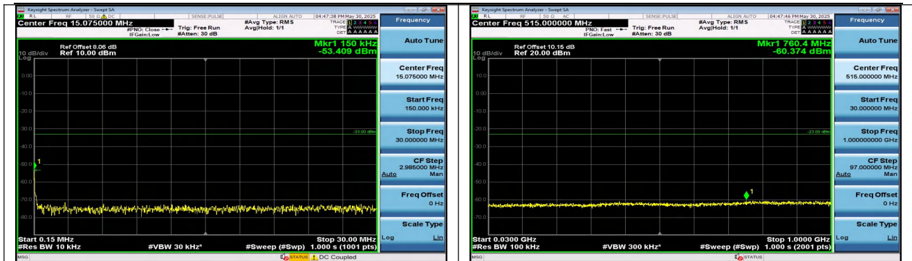
Band25-5MHz-16QAM-26665-25RB#0-0.15~30-PASS
