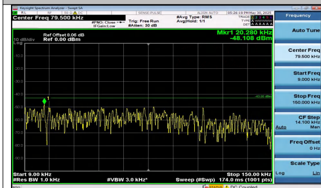
Band25-10MHz-QPSK-26640-1RB#0-0.009~0.15-PASS
