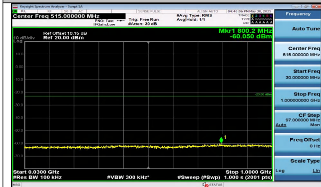
Band25-5MHz-16QAM-26665-1RB#24-30~1000-PASS
