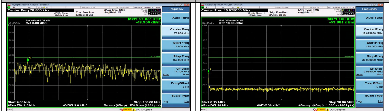
Band25-10MHz-16QAM-26365-1RB#0-0.009~0.15-PASS
