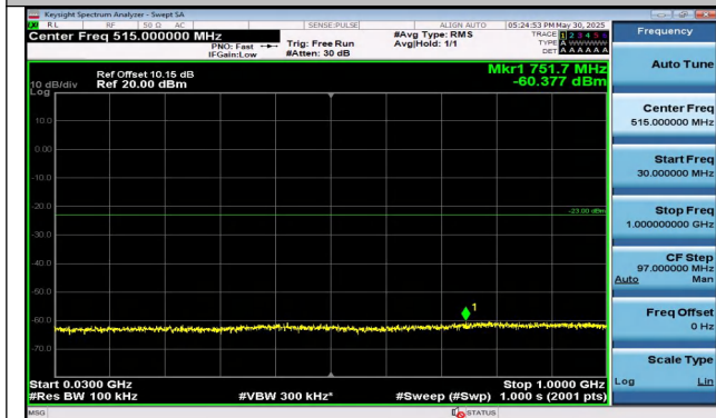
Band25-10MHz-QPSK-26365-1RB#49-30~1000-PASS
