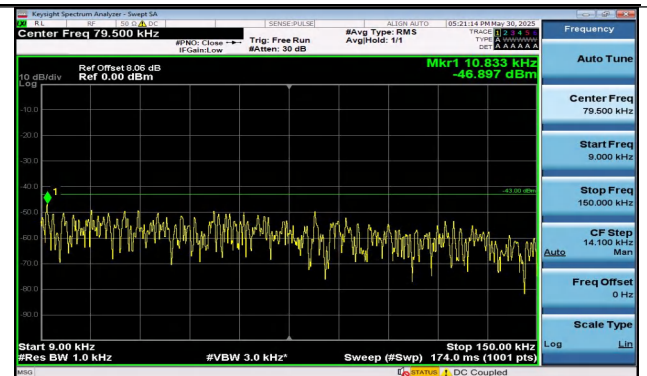
Band25-10MHz-QPSK-26090-1RB#49-0.009~0.15-PASS
