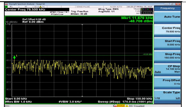
Band25-10MHz-16QAM-26365-1RB#49-0.009~0.15-PASS
