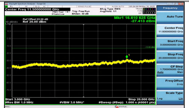
Band25-10MHz-16QAM-26365-1RB#49-3000~20000-PAS
