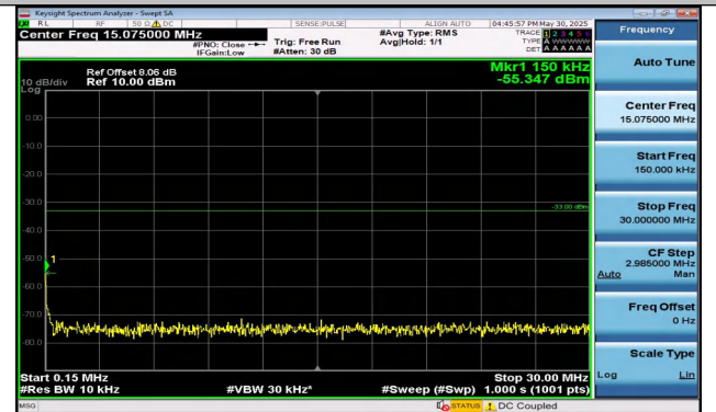
Band25-5MHz-16QAM-26665-1RB#24-0.15~30-PASS
