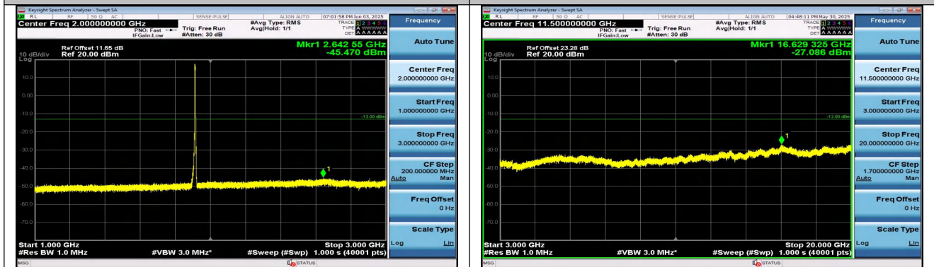
Band25-5MHz-16QAM-26665-25RB#0-1000~3000-PASS
