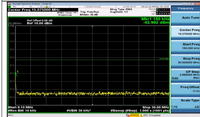
Band25-10MHz-QPSK-26090-1RB#49-0.15~30-PASS
