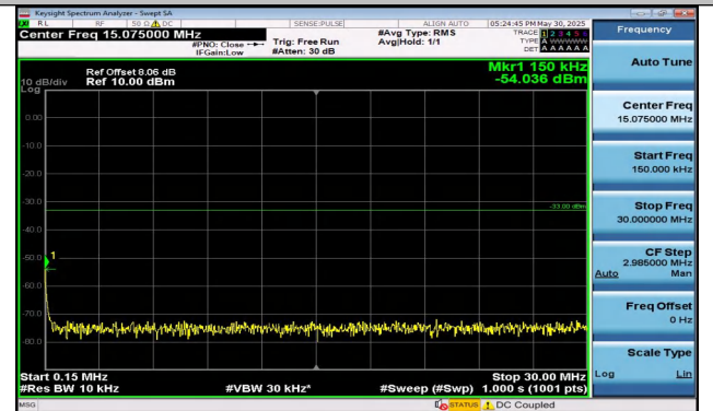
Band25-10MHz-QPSK-26365-1RB#49-0.15~30-PASS
