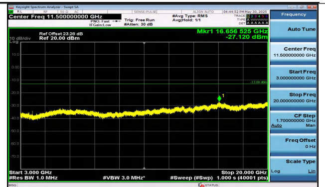
Band25-5MHz-16QAM-26665-1RB#0-3000~20000-PASS
