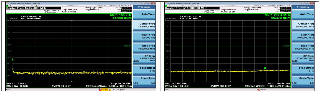
Band25-10MHz-QPSK-26365-50RB#0-0.15~30-PASS
