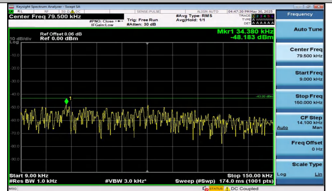
Band25-5MHz-16QAM-26665-25RB#0-0.009~0.15-PASS
