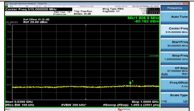
Band25-10MHz-16QAM-26365-1RB#49-30~1000-PASS
