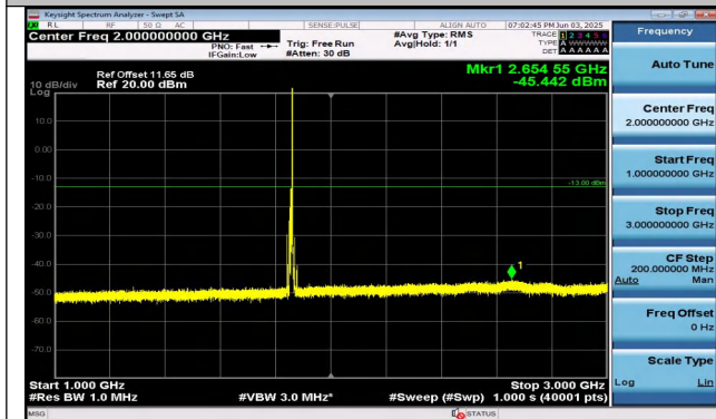
Band25-10MHz-QPSK-26090-1RB#49-1000~3000-PASS
