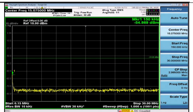
Band25-10MHz-16QAM-26090-1RB#49-0.15~30-PASS
