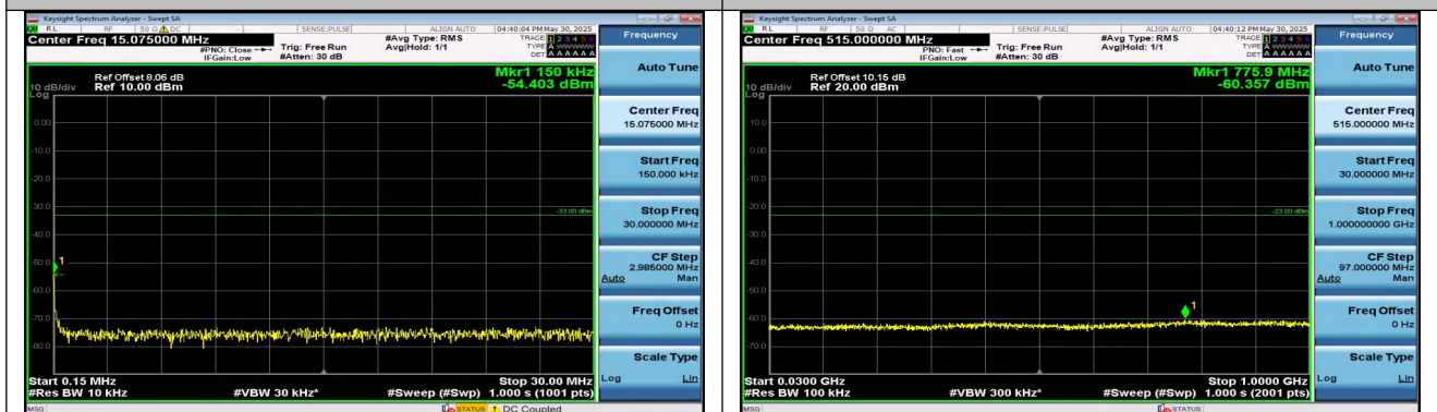
Band25-5MHz-QPSK-26365-1RB#24-0.15~30-PASS
