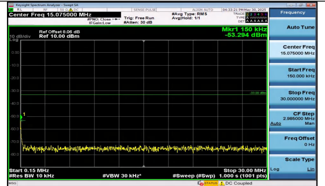
Band25-5MHz-QPSK-26065-1RB#0-0.15~30-PASS
