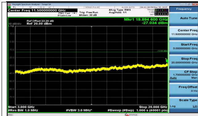
Band25-5MHz-16QAM-26365-1RB#24-3000~20000-PASS
