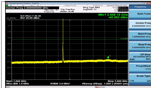
Band25-5MHz-QPSK-26365-1RB#24-1000~3000-PASS
