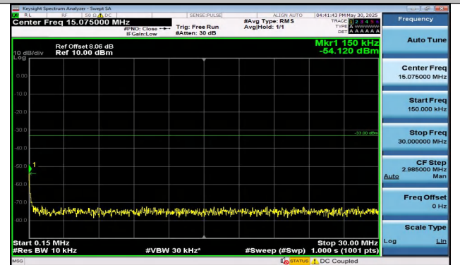
Band25-5MHz-QPSK-26365-25RB#0-0.15~30-PASS
