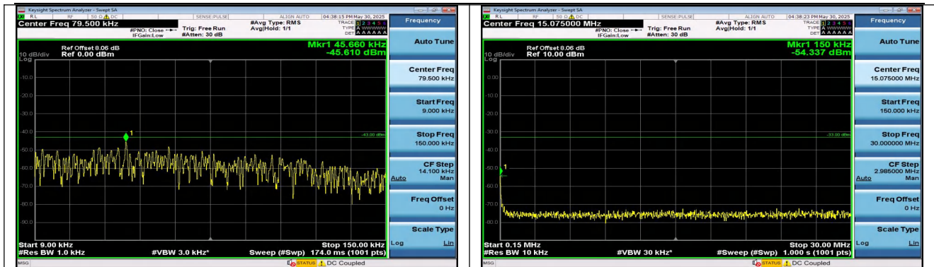
Band25-5MHz-QPSK-26365-1RB#0-0.009~0.15-PASS
