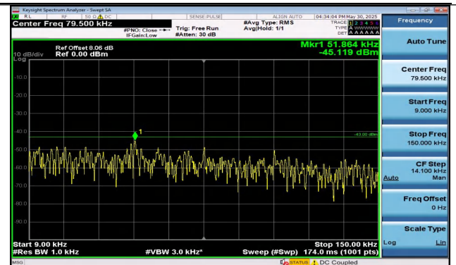
Band25-5MHz-16QAM-26065-1RB#0-0.009~0.15-PASS
