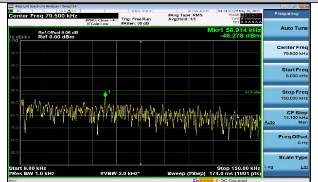
Band25-5MHz-QPSK-26065-1RB#24-0.009~0.15-PASS
