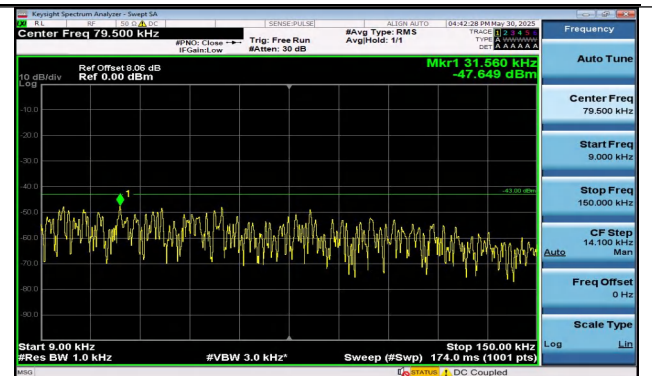
Band25-5MHz-16QAM-26365-25RB#0-0.009~0.15-PASS
