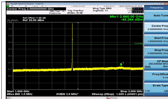
Band25-3MHz-16QAM-26675-15RB#0-1000~3000-PASS
