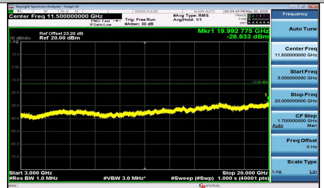
Band25-5MHz-16QAM-26065-1RB#0-3000~20000-PASS
