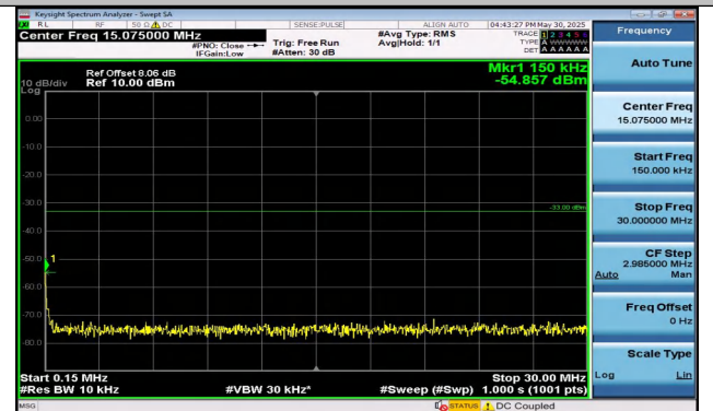
Band25-5MHz-QPSK-26665-1RB#0-0.15~30-PASS
