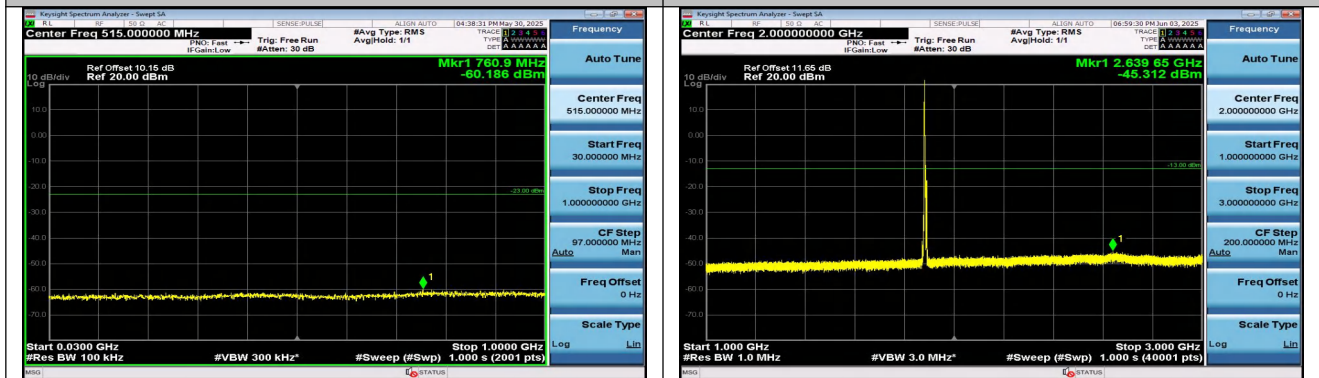
Band25-5MHz-QPSK-26365-1RB#0-30~1000-PASS
