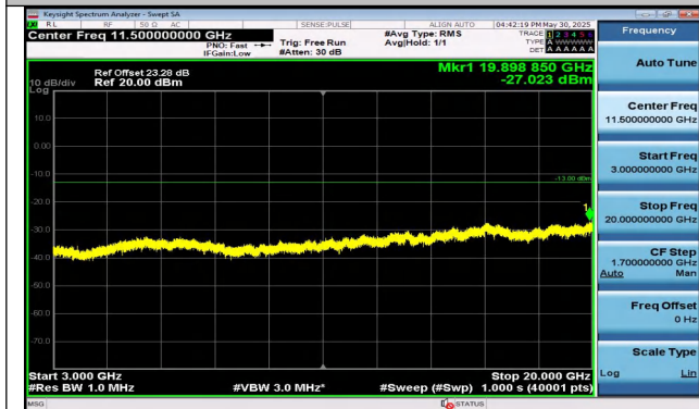
Band25-5MHz-QPSK-26365-25RB#0-3000~20000-PASS
