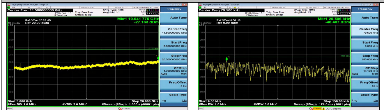
Band25-5MHz-QPSK-26365-1RB#0-3000~20000-PASS
