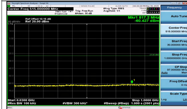
Band25-5MHz-QPSK-26065-1RB#0-30~1000-PASS
