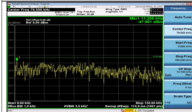
Band25-5MHz-QPSK-26665-1RB#0-0.009~0.15-PASS
