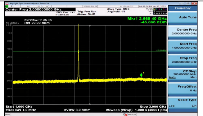
Band25-5MHz-QPSK-26065-1RB#0-1000~3000-PASS
