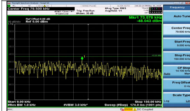
Band25-5MHz-QPSK-26065-1RB#0-0.009~0.15-PASS
