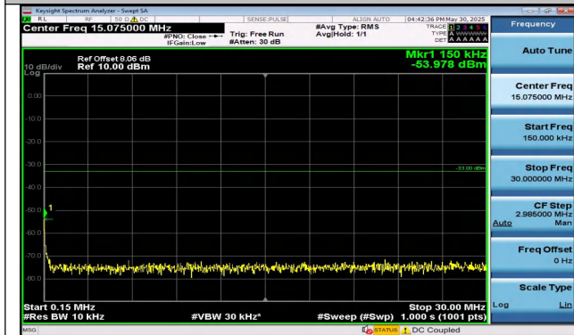
Band25-5MHz-16QAM-26365-25RB#0-0.15~30-PASS
