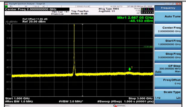
Band25-5MHz-QPSK-26365-25RB#0-1000~3000-PASS
