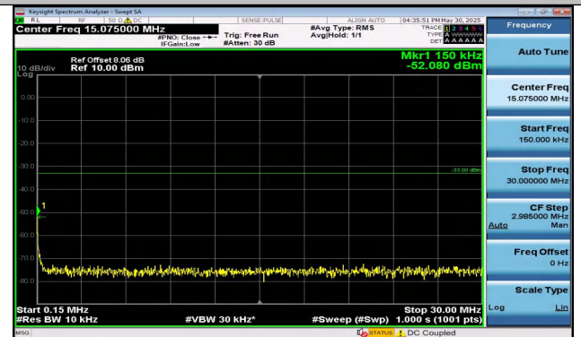
Band25-5MHz-16QAM-26065-1RB#24-0.15~30-PASS
