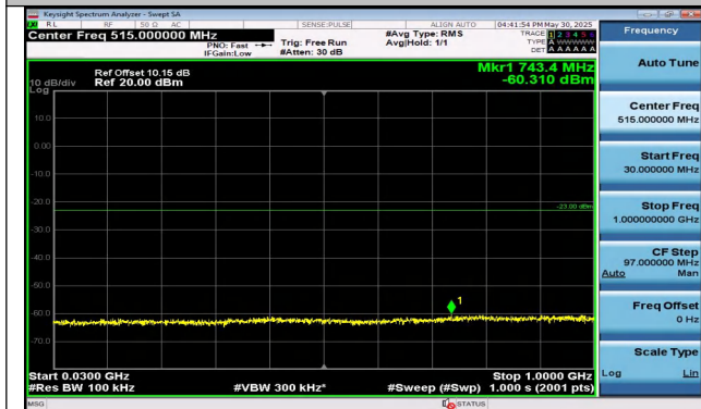
Band25-5MHz-QPSK-26365-25RB#0-0.30~1000-PASS
