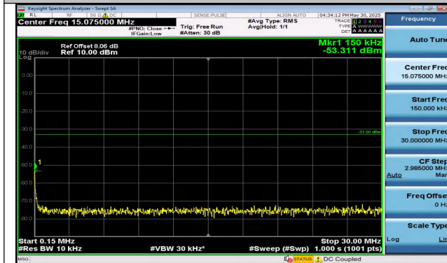
Band25-5MHz-16QAM-26065-1RB#0-0.15~30-PASS
