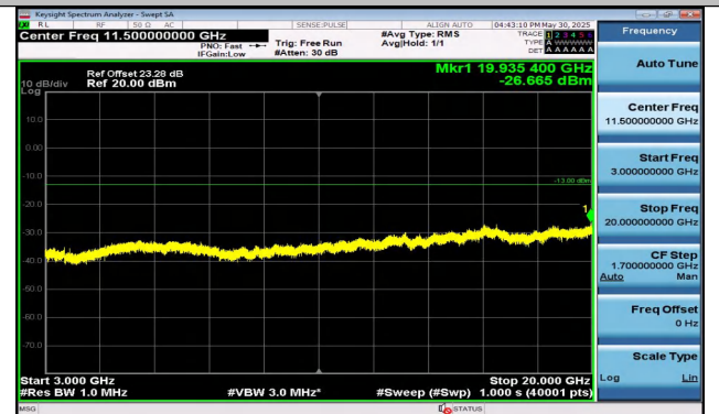
Band25-5MHz-16QAM-26365-25RB#0-3000~20000-PASS
