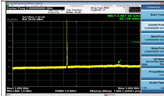
Band25-5MHz-16QAM-26065-1RB#0-1000~3000-PASS
