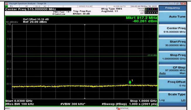
Band25-5MHz-16QAM-26365-25RB#0-30~1000-PASS
