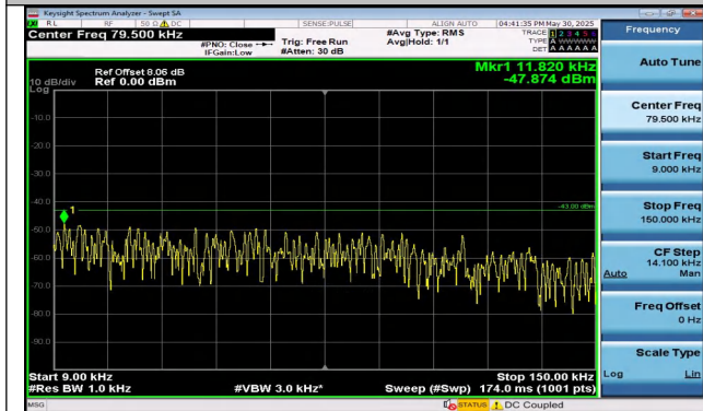
Band25-5MHz-QPSK-26365-25RB#0-0.009~0.15-PASS
