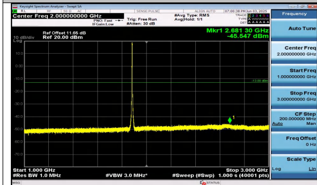
Band25-5MHz-16QAM-26365-25RB#0-1000~3000-PASS
