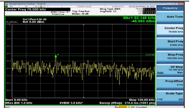
Band25-3MHz-16QAM-26365-15RB#0-0.009~0.15-PASS
