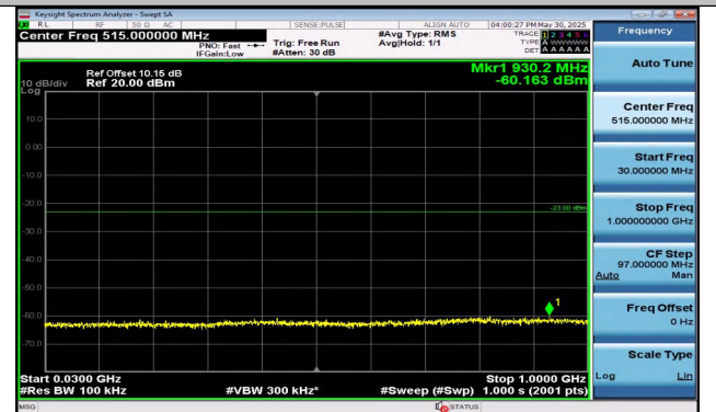
Band25-3MHz-16QAM-26675-15RB#0-30~1000-PASS
