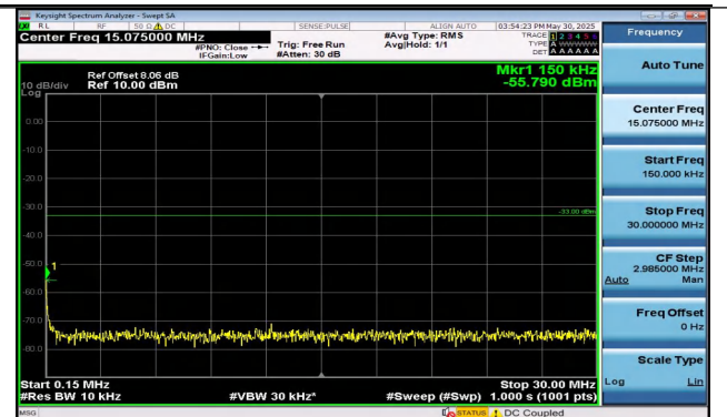
Band25-3MHz-QPSK-26365-15RB#0-0.15~30-PASS
