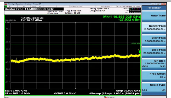
Band25-3MHz-QPSK-26365-1RB#14-3000~20000-PASS
