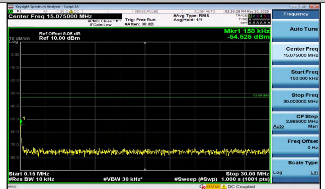
Band25-3MHz-QPSK-26675-15RB#0-0.15~30-PASS
