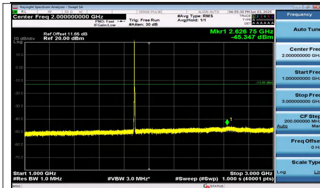
Band25-3MHz-16QAM-26365-1RB#0-1000~3000-PASS
