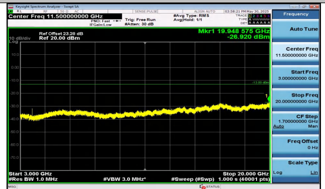
Band25-3MHz-QPSK-26675-1RB#14-3000~20000-PASS
