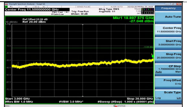
Band25-3MHz-16QAM-26365-1RB#0-3000~20000-PASS
