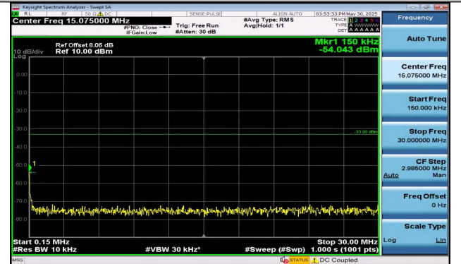
Band25-3MHz-16QAM-26365-1RB#14-0.15~30-PASS
