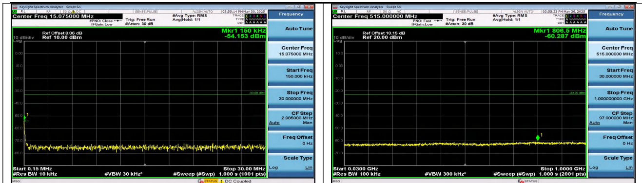
Band25-3MHz-16QAM-26365-15RB#0-0.15~30-PASS
