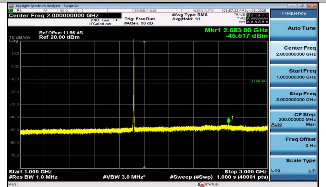
Band25-3MHz-16QAM-26675-1RB#14-1000~3000-PASS
