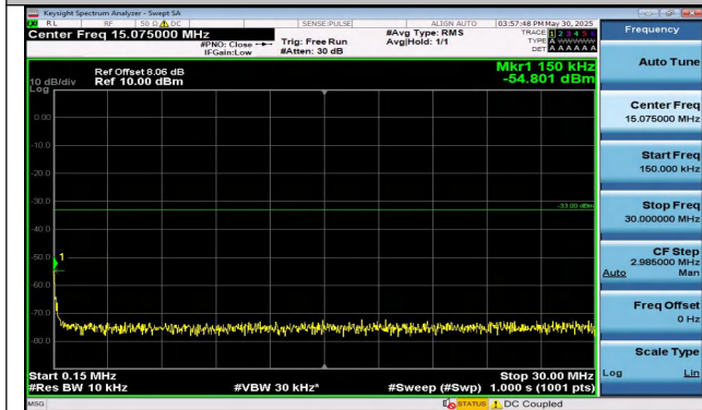
Band25-3MHz-QPSK-26675-1RB#14-0.15~30-PASS
