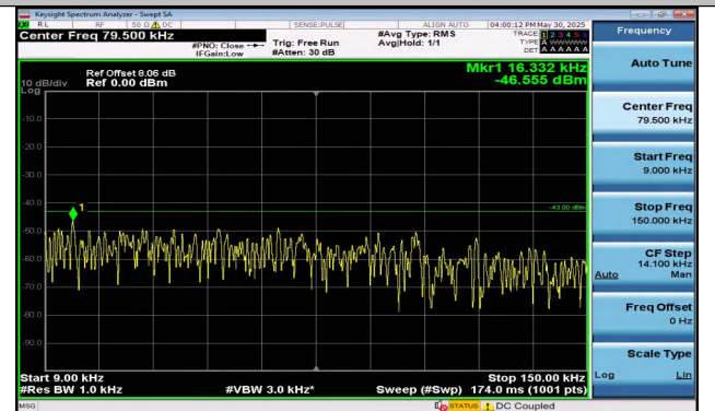
Band25-3MHz-16QAM-26675-15RB#0-0.009~0.15-PASS
