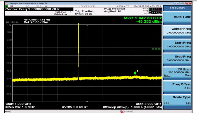
Band25-3MHz-16QAM-26365-1RB#14-1000~3000-PASS
