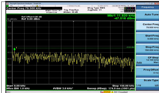
Band25-3MHz-16QAM-26675-1RB#14-0.009~0.15-PASS
