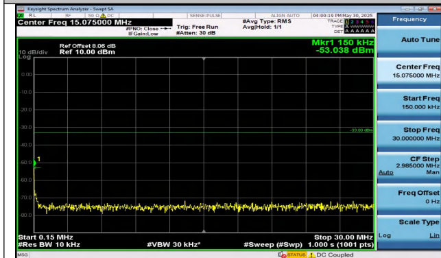
Band25-3MHz-16QAM-26675-15RB#0-0.15~30-PASS
