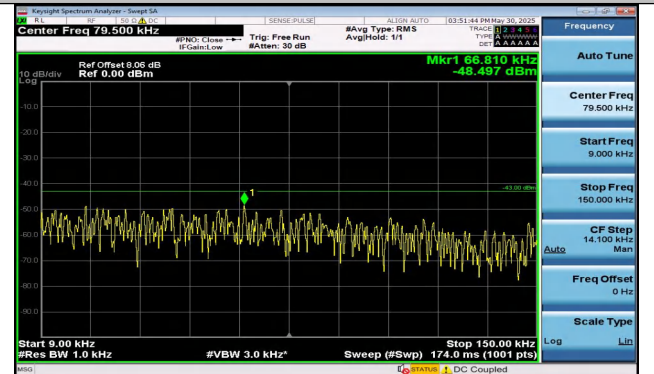
Band25-3MHz-16QAM-26365-1RB#0-0.009~0.15-PASS
