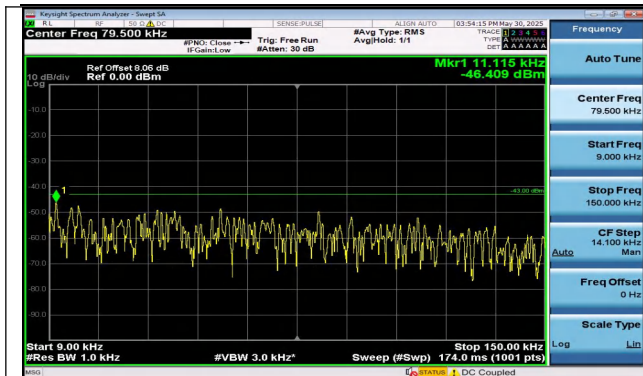
Band25-3MHz-QPSK-26365-15RB#0-0.009~0.15-PASS
