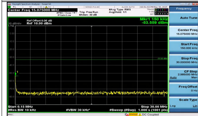
Band25-3MHz-16QAM-26365-1RB#0-0.15~30-PASS
