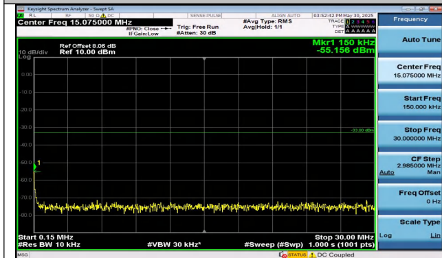
Band25-3MHz-QPSK-26365-1RB#14-0.15~30-PASS
