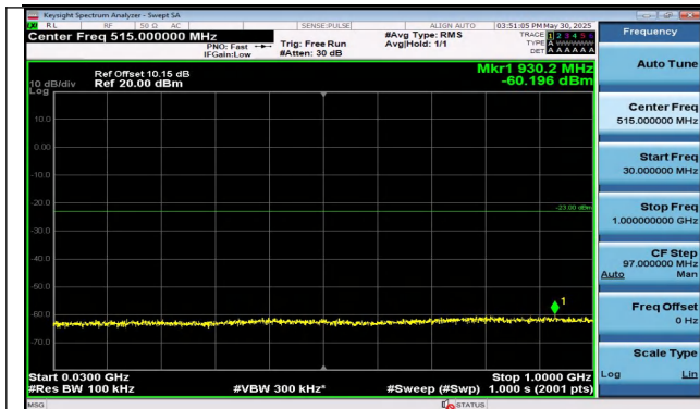
Band25-3MHz-QPSK-26365-1RB#0-30~1000-PASS
