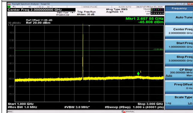
Band25-3MHz-QPSK-26675-1RB#14-1000~3000-PASS
