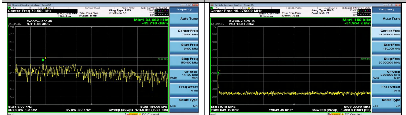
Band25-3MHz-QPSK-26675-1RB#0-0.009~0.15-PASS
