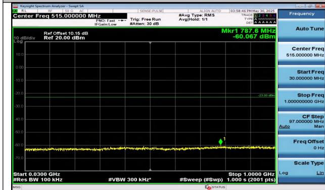
Band25-3MHz-16QAM-26675-1RB#14-30~1000-PASS
