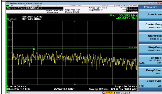
Band25-3MHz-QPSK-26675-15RB#0-0.009~0.15-PASS
