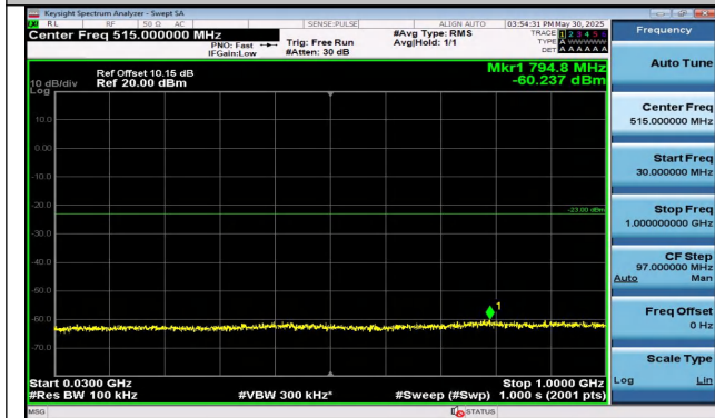
Band25-3MHz-QPSK-26365-15RB#0-0.30~1000-PASS
