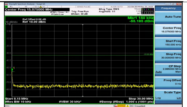
Band25-3MHz-16QAM-26675-1RB#14-0.15~30-PASS
