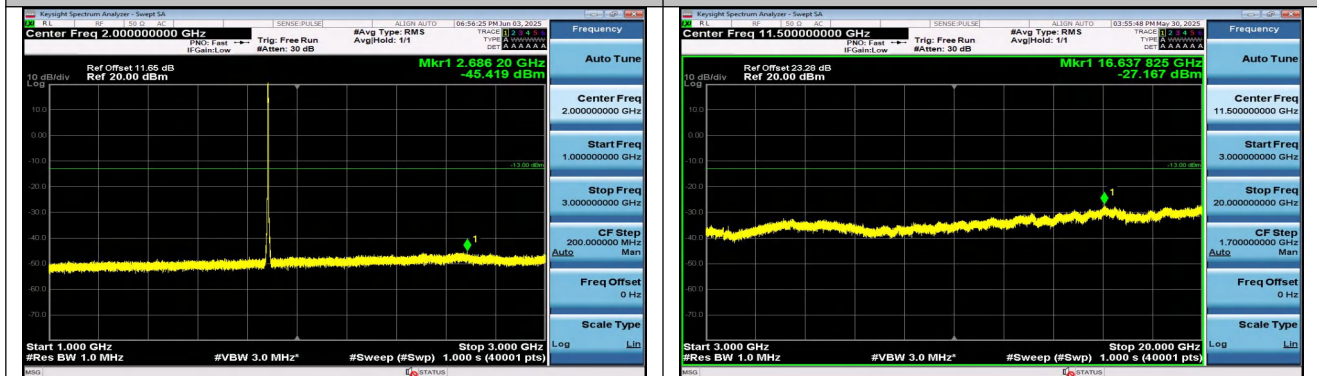
Band25-3MHz-16QAM-26365-15RB#0-1000~3000-PASS
