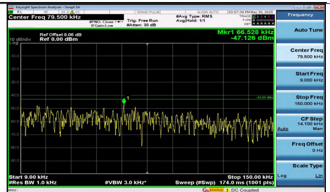
Band25-3MHz-QPSK-26675-1RB#14-0.009~0.15-PASS
