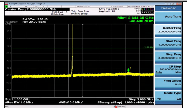
Band25-3MHz-QPSK-26055-15RB#0-1000~3000-PASS
