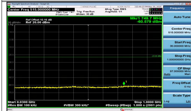
Band25-3MHz-QPSK-26055-15RB#0-0.30~1000-PASS
