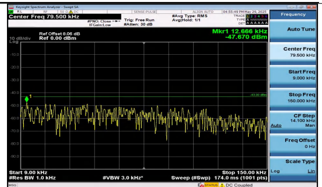
Band25-1.4MHz-16QAM-26683-1RB#0-0.009~0.15-PASS
