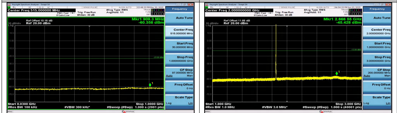
Band25-3MHz-16QAM-26055-1RB#14-30~1000-PASS
