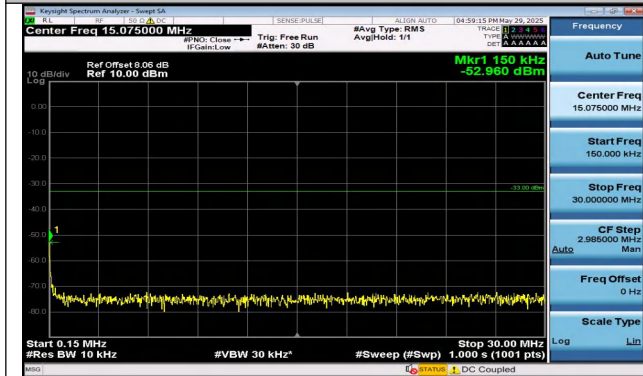
Band25-1.4MHz-16QAM-26683-6RB#0-0.15~30-PASS
