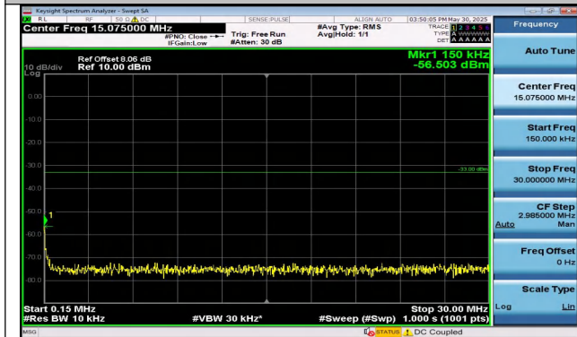
Band25-3MHz-16QAM-26055-15RB#0-0.15~30-PASS
