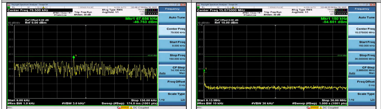
Band25-3MHz-16QAM-26055-1RB#14-0.009~0.15-PASS
