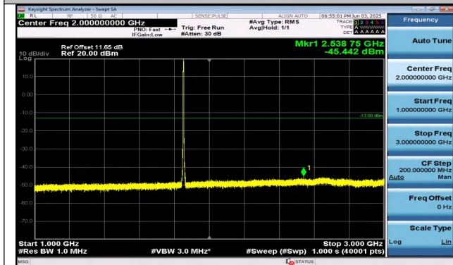
Band25-3MHz-16QAM-26055-15RB#0-1000~3000-PASS
