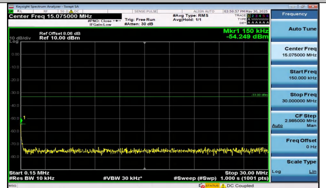
Band25-3MHz-QPSK-26365-1RB#0-0.15~30-PASS
