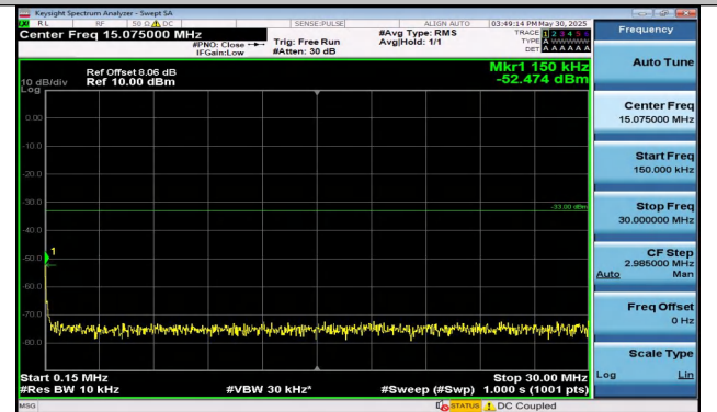
Band25-3MHz-QPSK-26055-15RB#0-0.15~30-PASS
