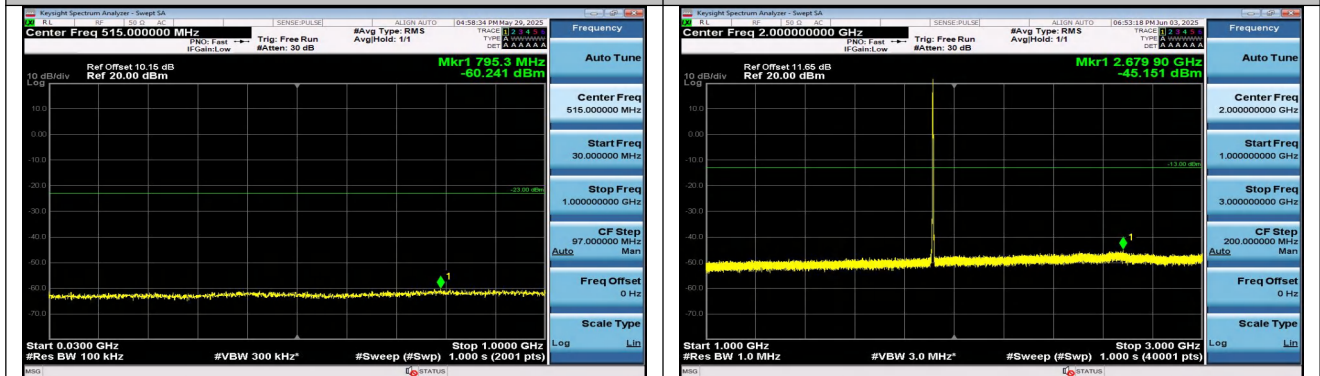
Band25-1.4MHz-QPSK-26683-6RB#0-30~1000-PASS
