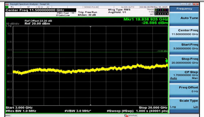
Band25-3MHz-16QAM-26055-15RB#0-3000~20000-PASS
