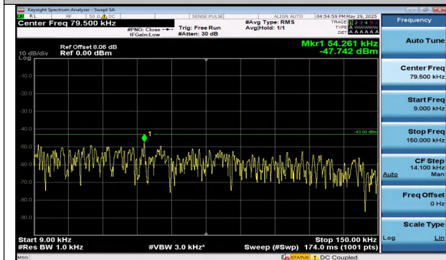
Band25-1.4MHz-QPSK-26683-1RB#0-0.009~0.15-PASS
