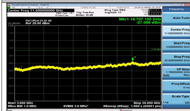
Band25-1.4MHz-QPSK-26683-1RB#0-3000~20000-PASS
