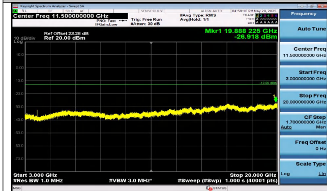
Band25-1.4MHz-16QAM-26683-1RB#5-3000~20000-PASS S
