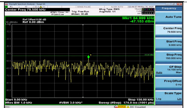
Band25-3MHz-16QAM-26055-15RB#0-0.009~0.15-PASS
