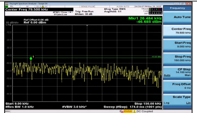
Band25-1.4MHz-16QAM-26683-6RB#0-0.009~0.15-PASS
