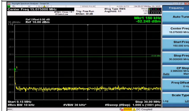
Band25-1.4MHz-16QAM-26683-1RB#0-0.15~30-PASS
