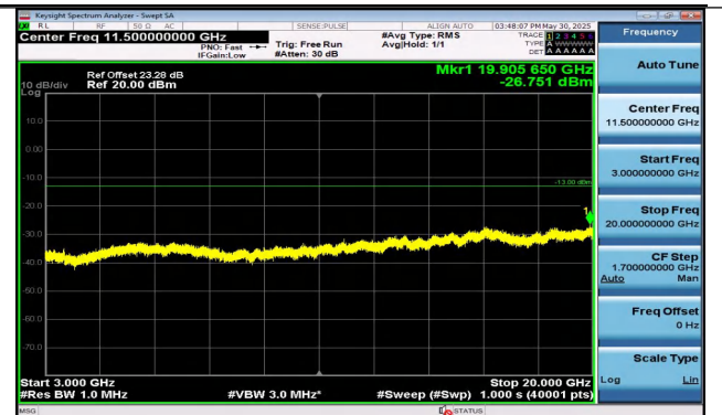
Band25-3MHz-QPSK-26055-1RB#14-3000~20000-PASS
