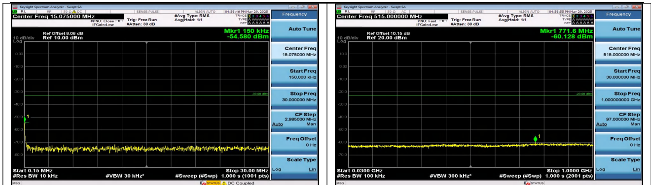
Band25-1.4MHz-QPSK-26683-1RB#5-0.15~30-PASS
