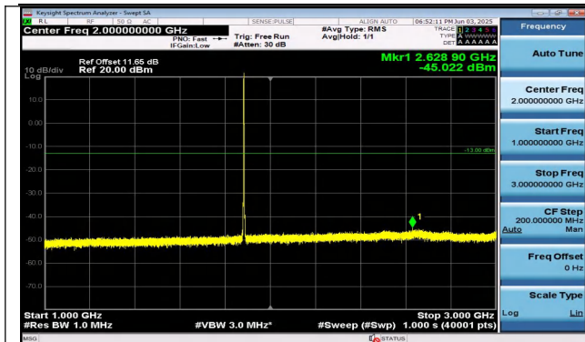
Band25-1.4MHz-16QAM-26365-6RB#0-1000~3000-PASS
