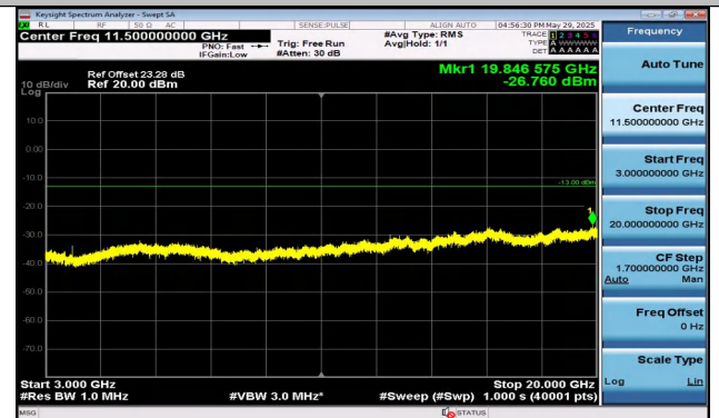
Band25-1.4MHz-16QAM-26683-1RB#0-3000~20000-PASS
