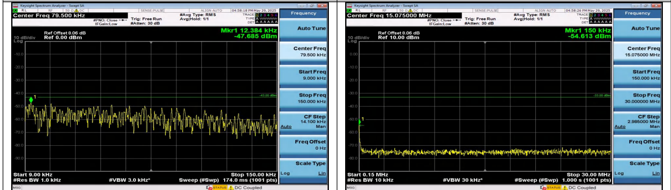
Band25-1.4MHz-QPSK-26683-6RB#0-0.009~0.15-PASS
