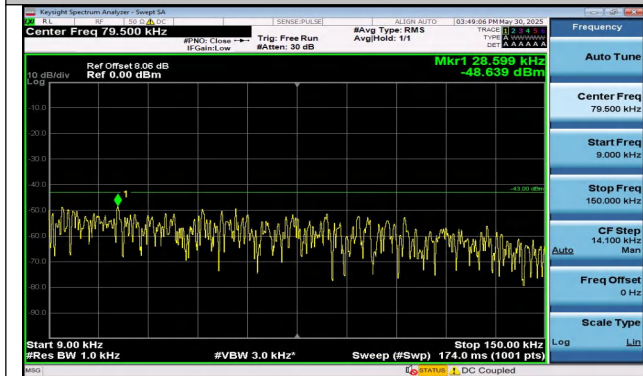
Band25-3MHz-QPSK-26055-15RB#0-0.009~0.15-PASS
