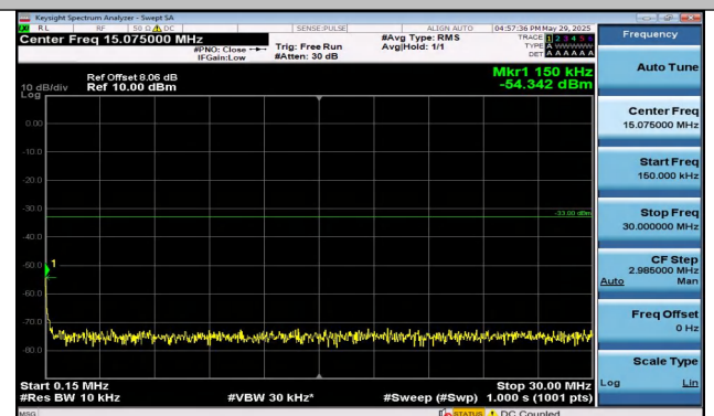
Band25-1.4MHz-16QAM-26683-1RB#5-0.15~30-PASS
