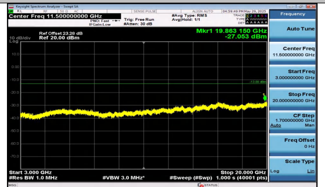
Band25-1.4MHz-16QAM-26683-6RB#0-3000~20000-PASS
