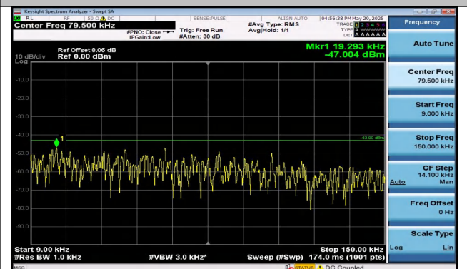
Band25-1.4MHz-QPSK-26683-1RB#5-0.009~0.15-PASS
