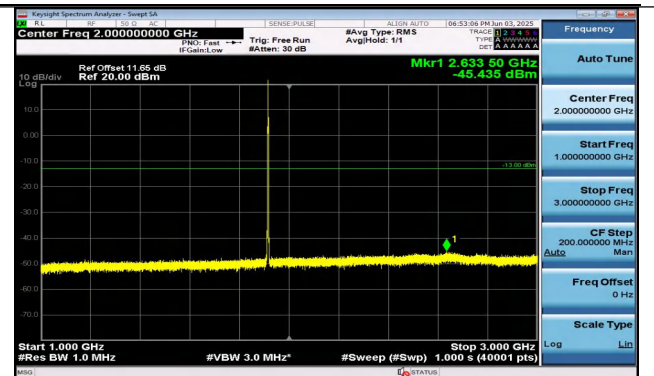
Band25-1.4MHz-16QAM-26683-1RB#5-1000~3000-PASS
