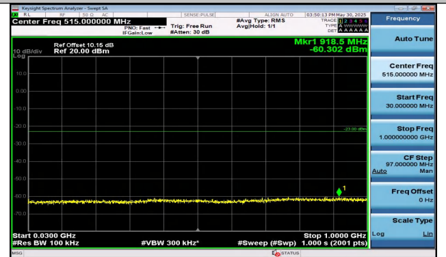
Band25-3MHz-16QAM-26055-15RB#0-30~1000-PASS
