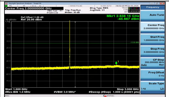
Band25-1.4MHz-QPSK-26683-1RB#0-1000~3000-PASS
