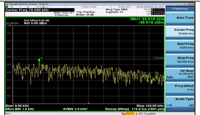
Band25-3MHz-16QAM-26055-1RB#0-0.009~0.15-PASS
