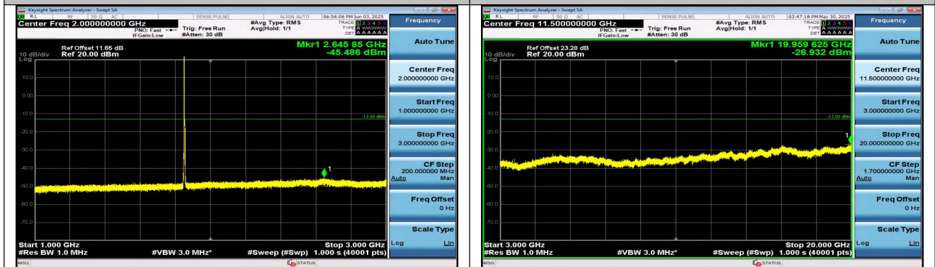
Band25-3MHz-16QAM-26055-1RB#0-1000~3000-PASS
