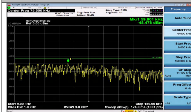
Band25-1.4MHz-16QAM-26683-1RB#5-0.009~0.15-PASS
