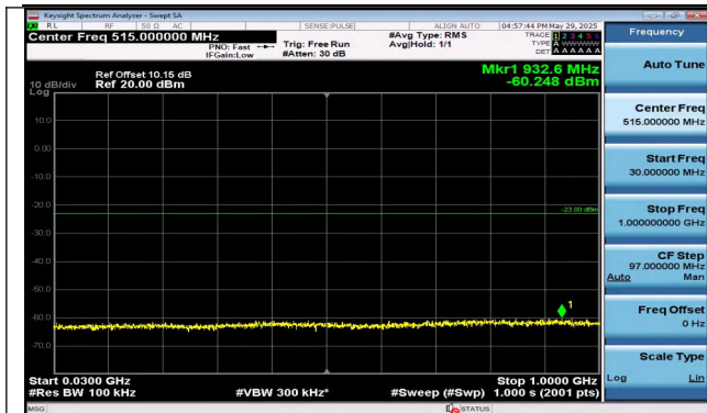
Band25-1.4MHz-16QAM-26683-1RB#5-30~1000-PASS
