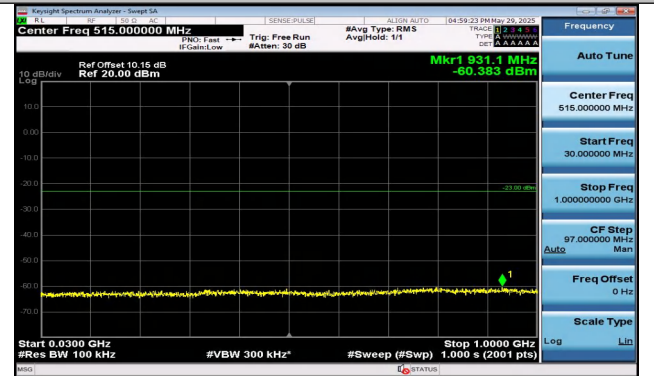
Band25-1.4MHz-16QAM-26683-6RB#0-30~1000-PASS
