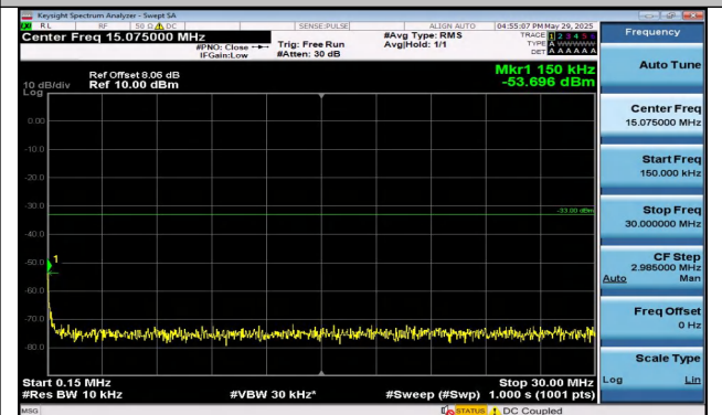
Band25-1.4MHz-QPSK-26683-1RB#0-0.15~30-PASS
