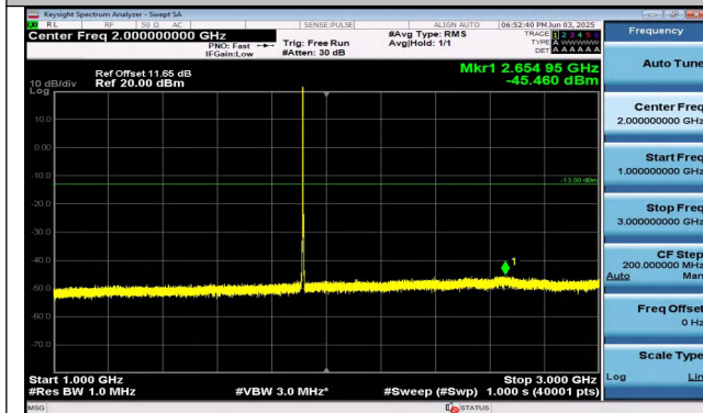
Band25-1.4MHz-16QAM-26683-1RB#0-1000~3000-PASS
