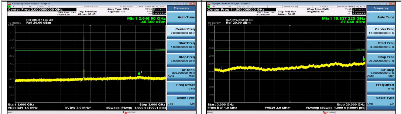
Band25-1.4MHz-QPSK-26683-1RB#5-1000~3000-PASS
