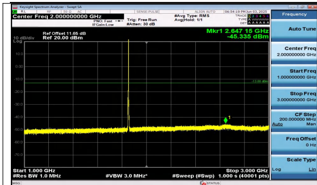
Band25-3MHz-QPSK-26055-1RB#14-1000~3000-PASS
