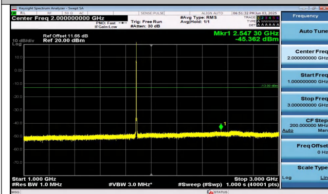
Band25-1.4MHz-QPSK-26365-1RB#5-1000~3000-PASS
