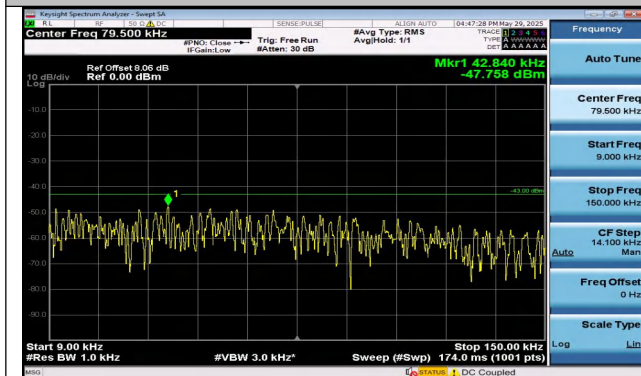
Band25-1.4MHz-16QAM-26047-1RB#5-0.009~0.15-PASS
