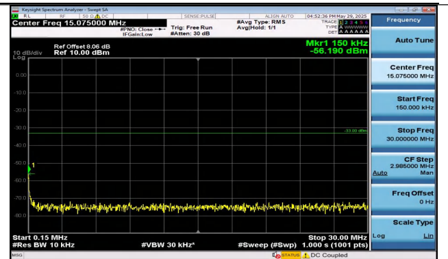
Band25-1.4MHz-16QAM-26365-1RB#5-0.15~30-PASS
