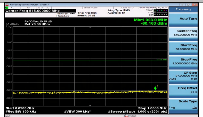
Band25-1.4MHz-16QAM-26047-1RB#0-30~1000-PASS
