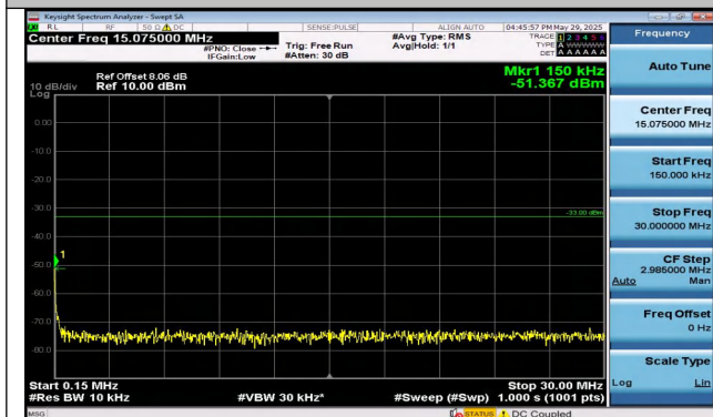
Band25-1.4MHz-16QAM-26047-1RB#0-0.15~30-PASS
