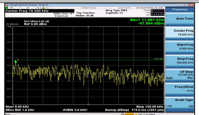
Band25-1.4MHz-16QAM-26047-6RB#0-0.009~0.15-PASS
