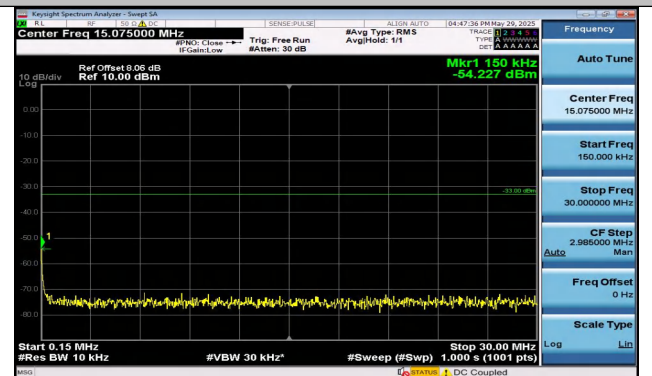
Band25-1.4MHz-16QAM-26047-1RB#5-0.15~30-PASS
