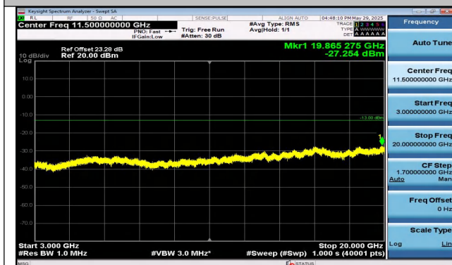
Band25-1.4MHz-16QAM-26047-1RB#5-3000~20000-PASS
