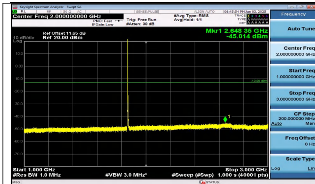
Band25-1.4MHz-16QAM-26047-1RB#0-1000~3000-PASS
