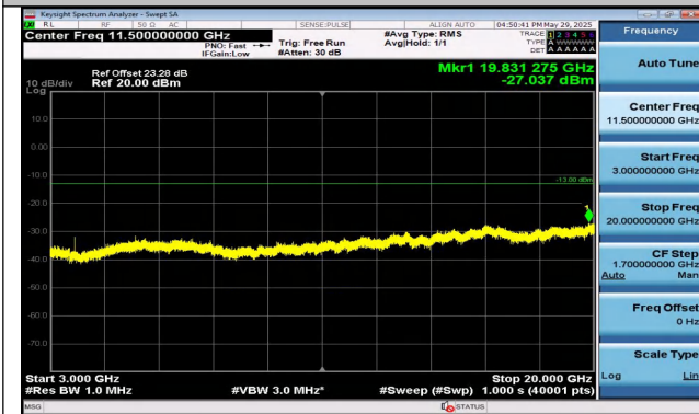
Band25-1.4MHz-QPSK-26365-1RB#0-3000~20000-PASS
