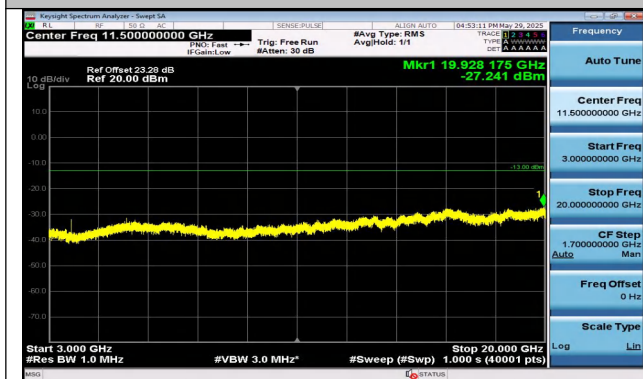
Band25-1.4MHz-16QAM-26365-1RB#5-3000~20000-PASS
