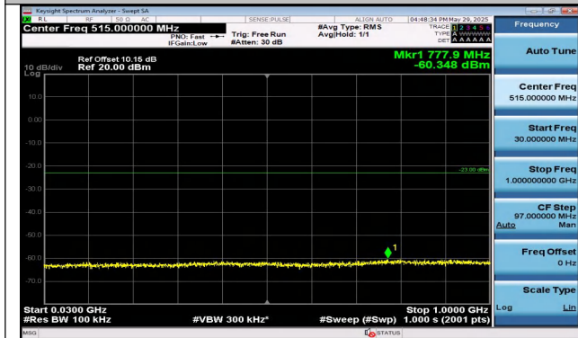
Band25-1.4MHz-QPSK-26047-6RB#0-30~1000-PASS
