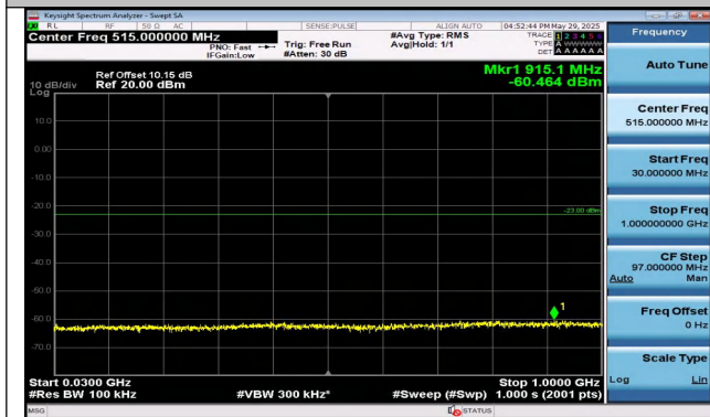
Band25-1.4MHz-16QAM-26365-1RB#5-30~1000-PASS
