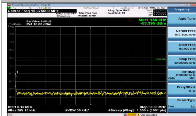
Band25-1.4MHz-16QAM-26365-6RB#0-0.15~30-PASS
