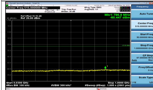
Band25-1.4MHz-16QAM-26047-1RB#5-30~1000-PASS
