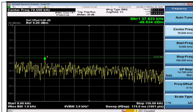
Band25-1.4MHz-QPSK-26047-6RB#0-0.009~0.15-PASS
