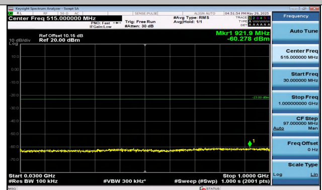
Band25-1.4MHz-QPSK-26365-1RB#5-30~1000-PASS
