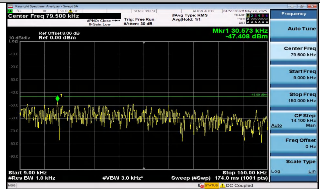
Band25-1.4MHz-QPSK-26365-1RB#5-0.009~0.15-PASS
