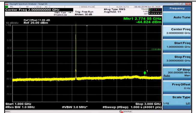
Band25-1.4MHz-16QAM-26047-1RB#5-1000~3000-PASS
