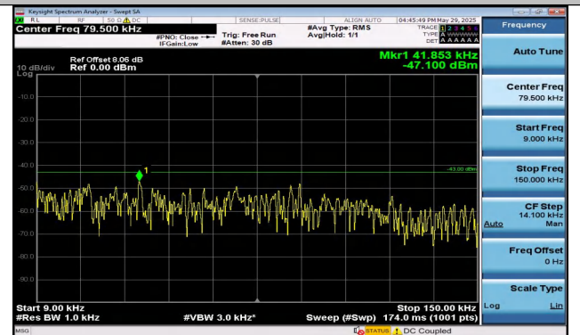
Band25-1.4MHz-16QAM-26047-1RB#0-0.009~0.15-PASS
