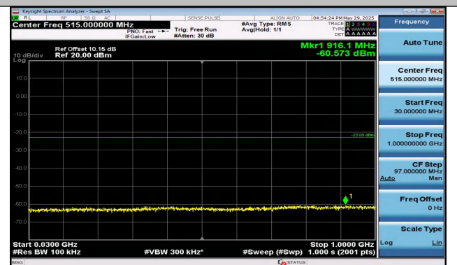
Band25-1.4MHz-16QAM-26365-6RB#0-30~1000-PASS
