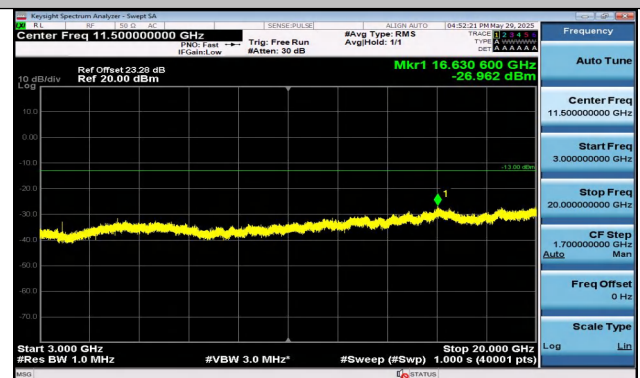
Band25-1.4MHz-QPSK-26365-1RB#5-3000~20000-PASS
