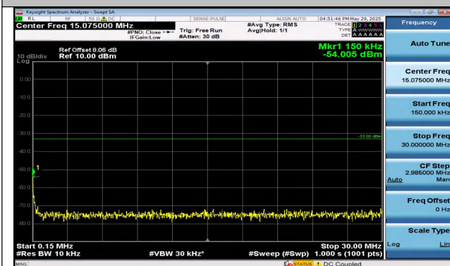
Band25-1.4MHz-QPSK-26365-1RB#5-0.15~30-PASS
