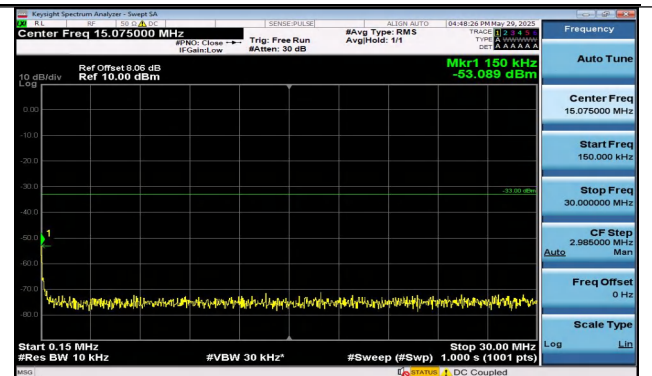
Band25-1.4MHz-QPSK-26047-6RB#0-0.15~30-PASS
