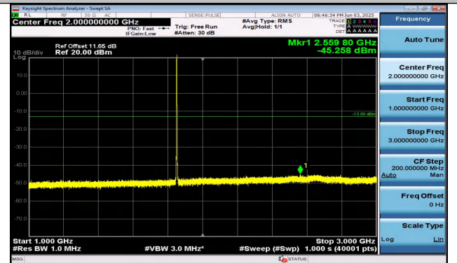
Band25-1.4MHz-QPSK-26047-6RB#0-1000~3000-PASS
