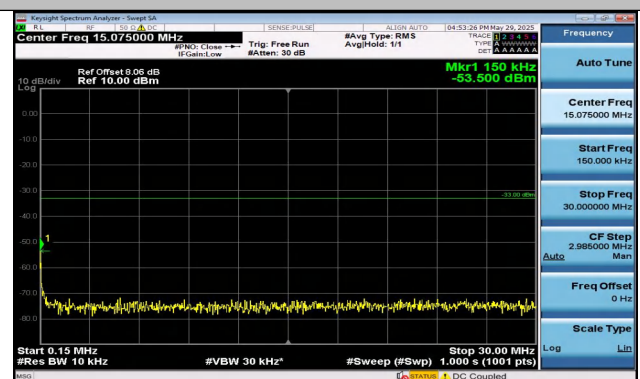
Band25-1.4MHz-QPSK-26365-6RB#0-0.15~30-PASS
