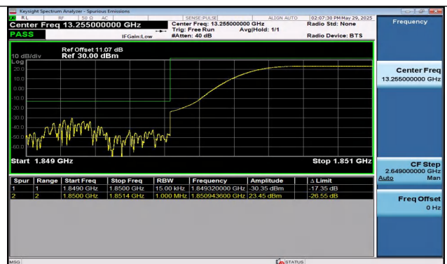
Band25-1.4MHz-QPSK-26047-1RB#5-PASS
