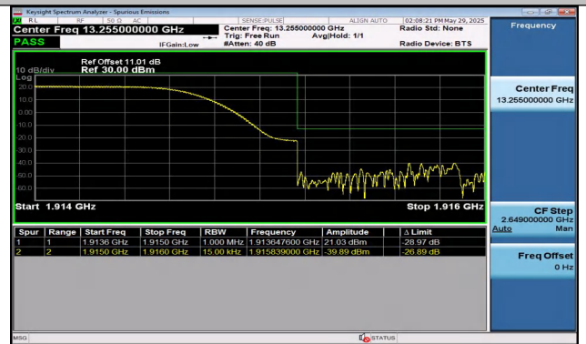
Band25-1.4MHz-16QAM-26683-1RB#0-PASS
