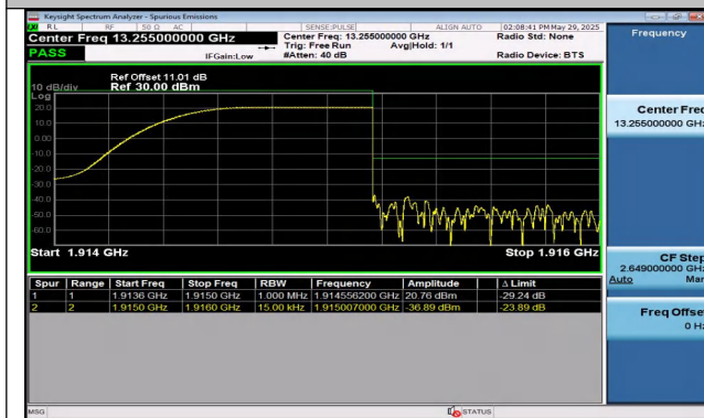
Band25-1.4MHz-16QAM-26683-1RB#5-PASS
