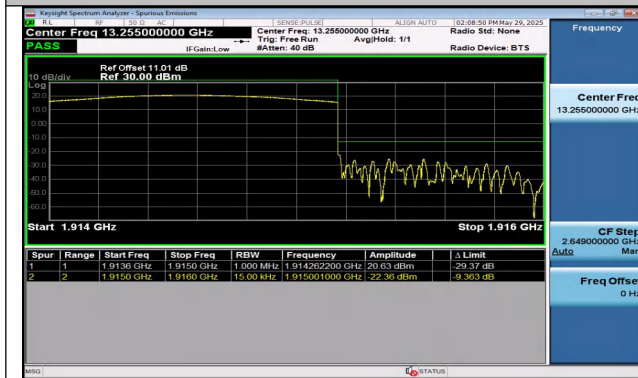
Band25-1.4MHz-QPSK-26683-6RB#0-PASS
