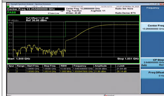
Band25-1.4MHz-16QAM-26047-1RB#5-PASS
