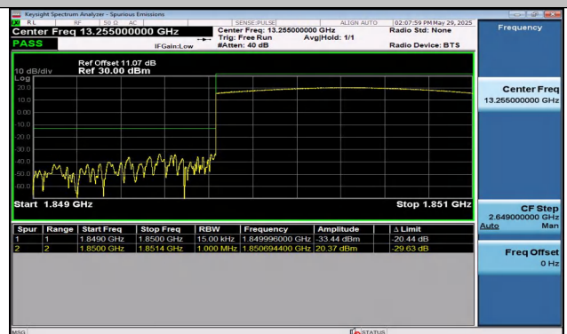
Band25-1.4MHz-16QAM-26047-6RB#0-PASS
