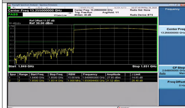
Band25-1.4MHz-QPSK-26047-6RB#0-PASS
