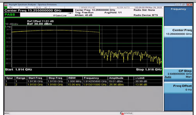
Band25-1.4MHz-16QAM-26683-6RB#0-PASS
