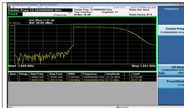
Band25-1.4MHz-QPSK-26047-1RB#0-PASS
