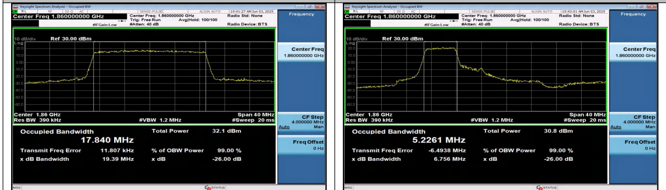
Band25-20MHz-QPSK-26140-100RB#0-PASS
