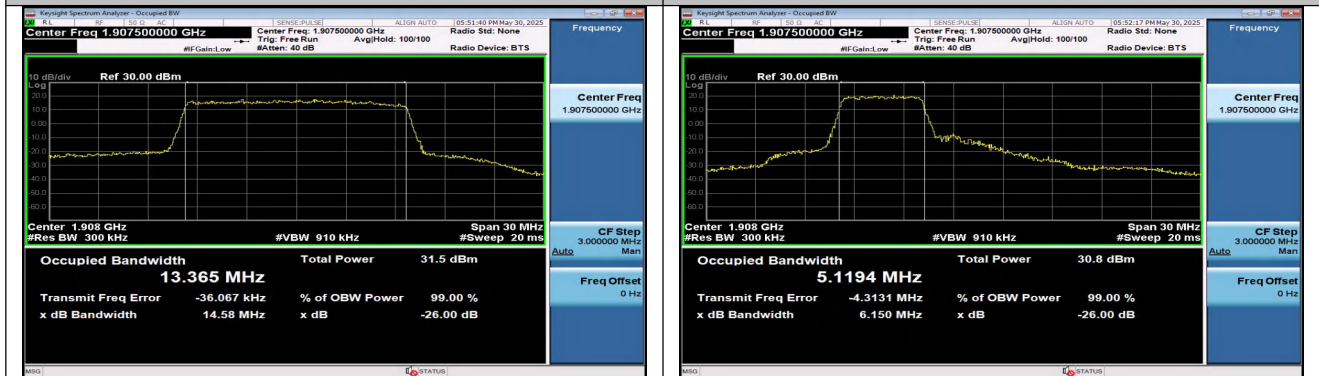
Band25-15MHz-QPSK-26615-75RB#0-PASS
