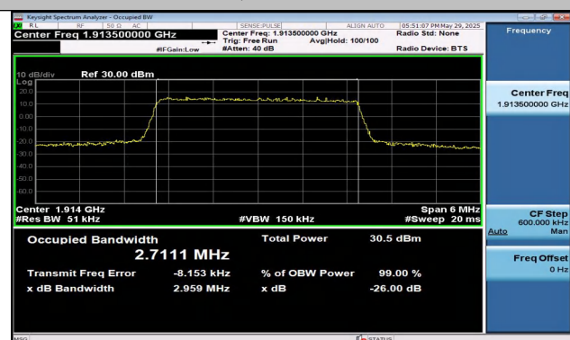
Band25-3MHz-QPSK-26675-15RB#0-PASS
