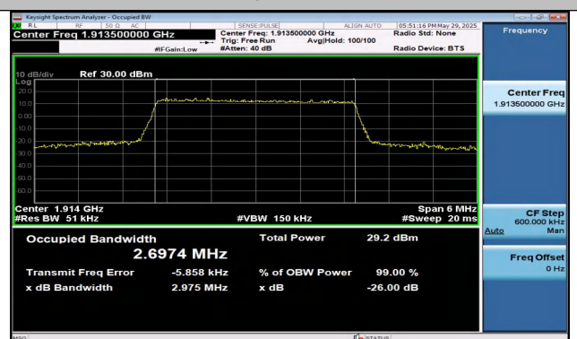
Band25-3MHz-16QAM-26675-15RB#0-PASS
