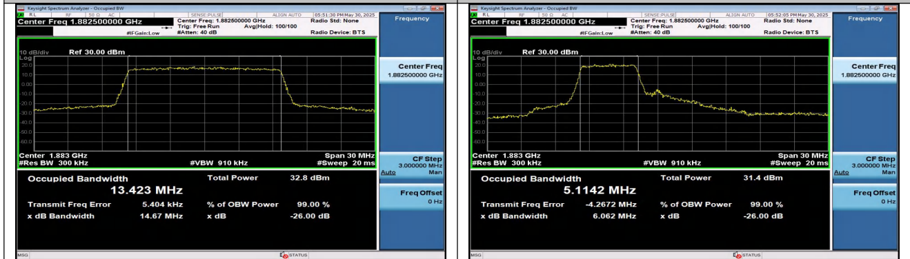
Band25-15MHz-QPSK-26365-75RB#0-PASS
