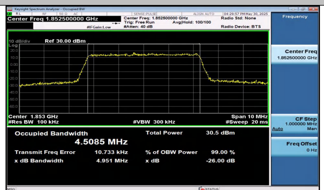
Band25-5MHz-16QAM-26065-25RB#0-PASS
