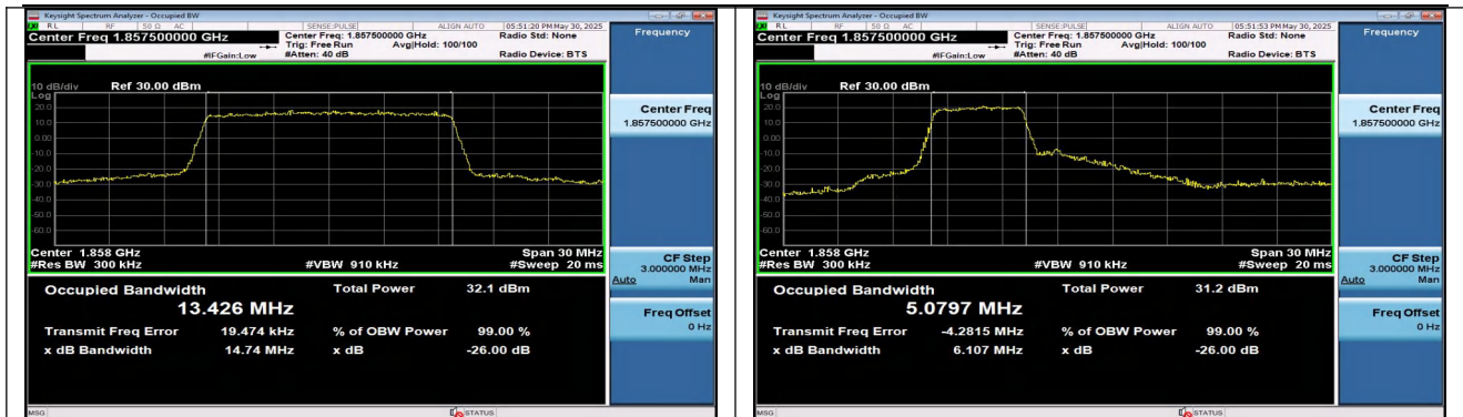
Band25-15MHz-QPSK-26115-75RB#0-PASS
