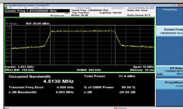
Band25-5MHz-QPSK-26065-25RB#0-PASS
