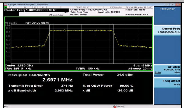
Band25-3MHz-16QAM-26365-15RB#0-PASS
