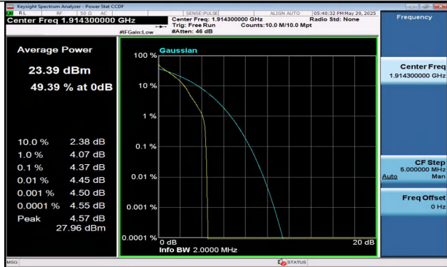
Band25-1.4MHz-QPSK-26683-1RB#0-PASS
