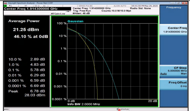
Band25-1.4MHz-16QAM-26683-6RB#0-PASS
