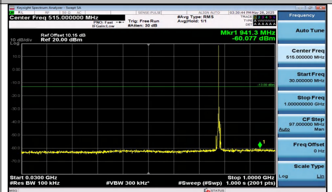
Band13-5MHz-16QAM-23255-1RB#0-30~1000-PASS
