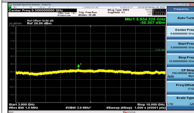
Band13-5MHz-16QAM-23255-1RB#24-3000~10000-PASS
