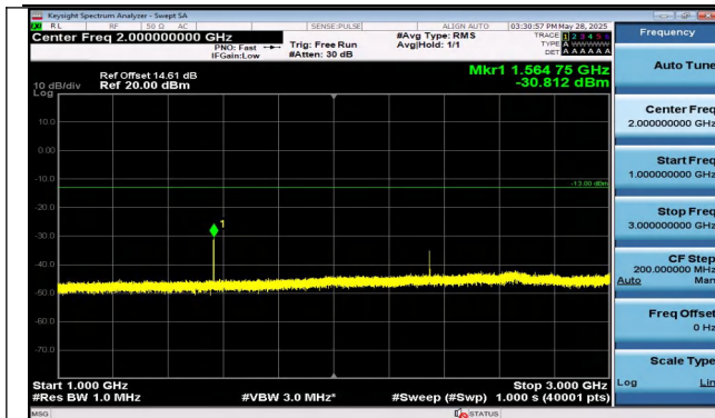
Band13-5MHz-16QAM-23255-1RB#0-1000~3000-PASS
