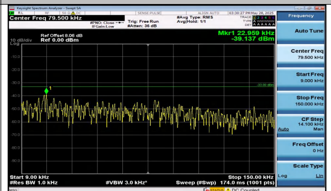
Band13-5MHz-16QAM-23255-1RB#0-0.009~0.15-PASS
