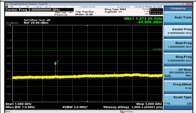
Band13-5MHz-16QAM-23255-1RB#24-1000~3000-PASS
