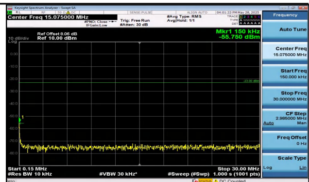
Band13-10MHz-16QAM-23230-1RB#49-0.15~30-PASS
