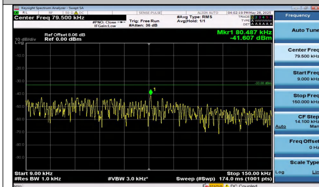
Band13-10MHz-QPSK-23230-50RB#0-0.009~0.15-PASS
