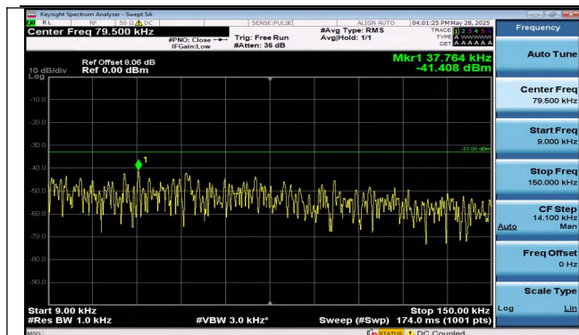
Band13-10MHz-16QAM-23230-1RB#49-0.009~0.15-PASS
