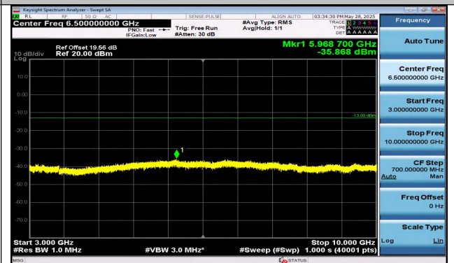
Band13-5MHz-16QAM-23255-25RB#0-3000~10000-PASS
