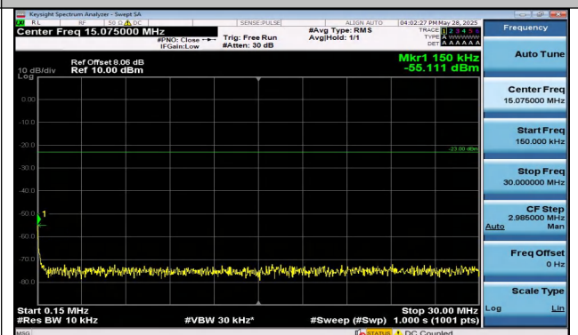
Band13-10MHz-QPSK-23230-50RB#0-0.15~30-PASS
