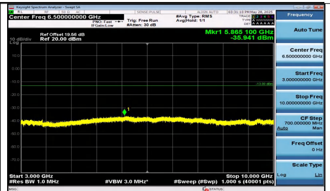
Band13-5MHz-16QAM-23255-1RB#0-3000~10000-PASS
