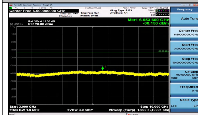
Band13-5MHz-QPSK-23255-25RB#0-3000~10000-PASS
