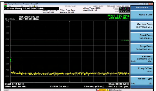
Band13-5MHz-QPSK-23255-25RB#0-0.15~30-PASS
