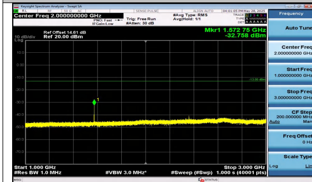
Band13-10MHz-QPSK-23230-1RB#49-1000~3000-PASS
