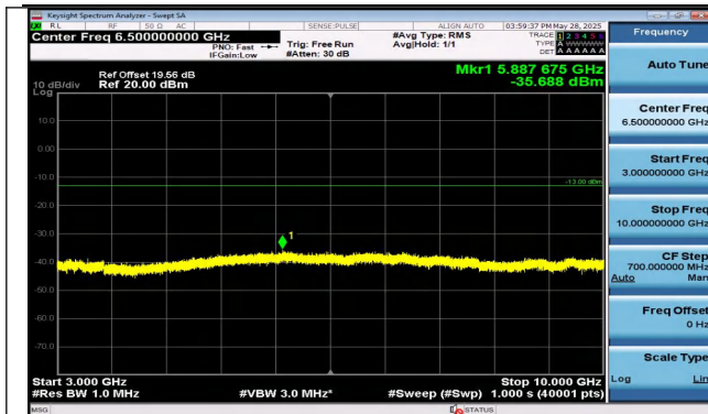
Band13-10MHz-QPSK-23230-1RB#0-3000~10000-PASS
