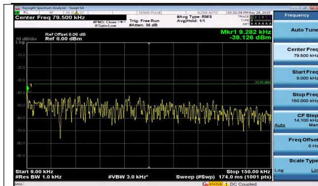
Band13-5MHz-QPSK-23255-25RB#0-0.009~0.15-PASS
