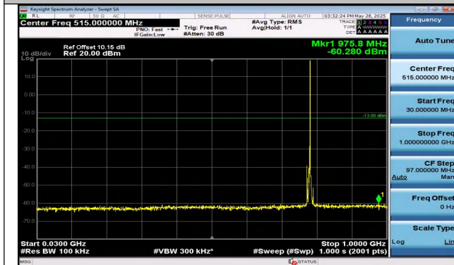
Band13-5MHz-16QAM-23255-1RB#24-30~1000-PASS
