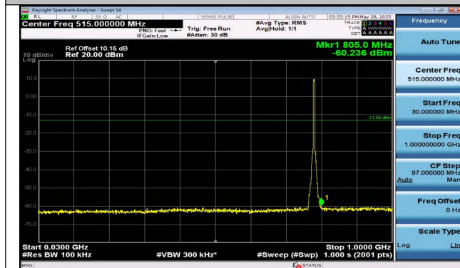
Band13-5MHz-QPSK-23255-25RB#0-30~1000-PASS
