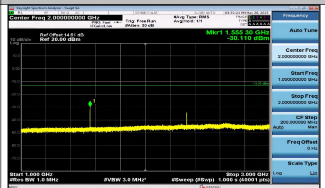
Band13-10MHz-QPSK-23230-1RB#0-1000~3000-PASS
