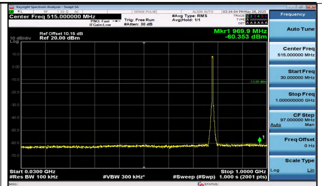
Band13-5MHz-16QAM-23255-25RB#0-30~1000-PASS
