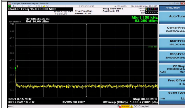
Band13-10MHz-QPSK-23230-1RB#49-0.15~30-PASS
