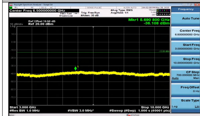
Band13-10MHz-16QAM-23230-1RB#49-3000~10000-PAS
