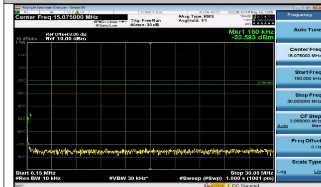
Band13-5MHz-16QAM-23255-1RB#0-0.15~30-PASS
