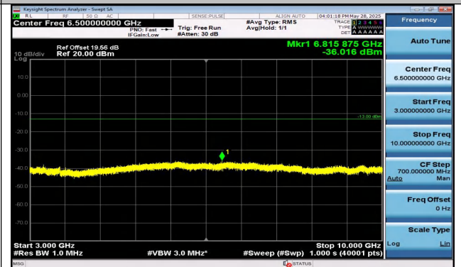
Band13-10MHz-QPSK-23230-1RB#49-3000~10000-PASS
