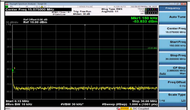
Band13-10MHz-QPSK-23230-1RB#0-0.15~30-PASS
