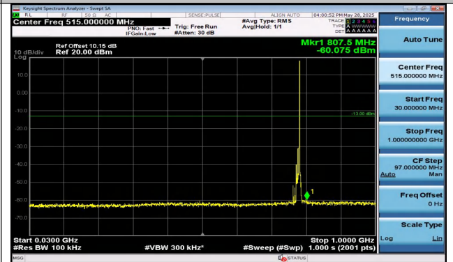
Band13-10MHz-QPSK-23230-1RB#49-30~1000-PASS
