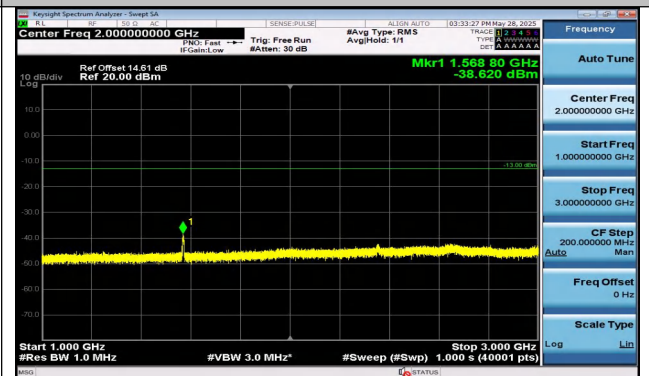
Band13-5MHz-QPSK-23255-25RB#0-1000~3000-PASS
