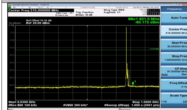
Band13-10MHz-QPSK-23230-1RB#0-0-30~1000-PASS
