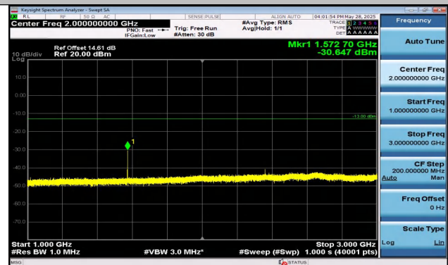
Band13-10MHz-16QAM-23230-1RB#49-1000~3000-PAS
