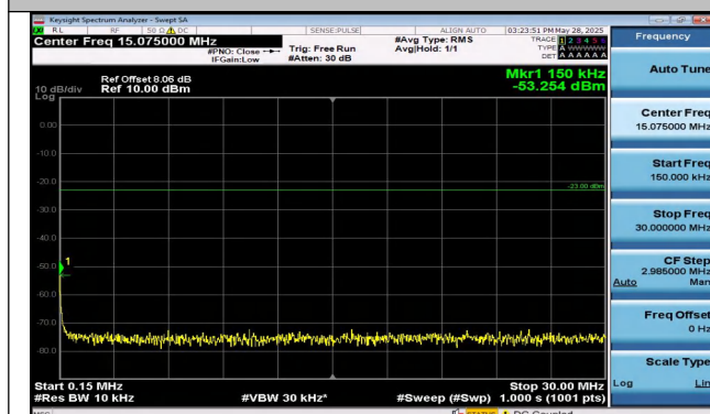
Band13-5MHz-16QAM-23205-25RB#0-0.15~30-PASS
