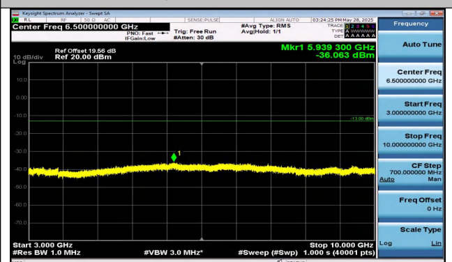
Band13-5MHz-16QAM-23205-25RB#0-3000~10000-PASS
