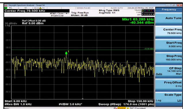
Band13-5MHz-16QAM-23205-1RB#0-0.009~0.15-PASS
