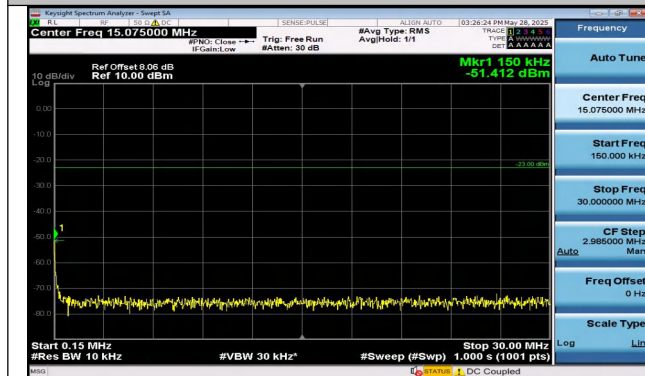
Band13-5MHz-QPSK-23230-1RB#24-0.15~30-PASS
