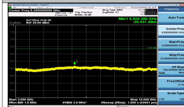
Band13-5MHz-16QAM-23205-1RB#24-3000~10000-PASS
