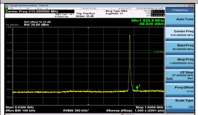
Band13-5MHz-16QAM-23205-25RB#0-30~1000-PASS
