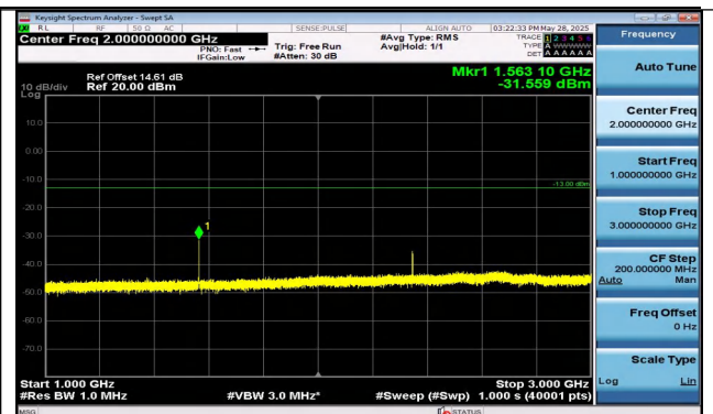
Band13-5MHz-16QAM-23205-1RB#24-1000~3000-PASS
