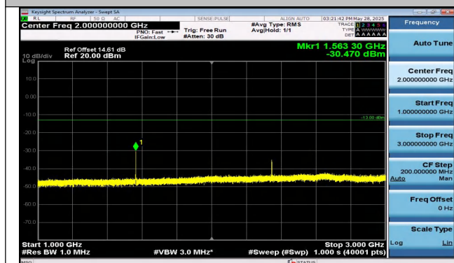
Band13-5MHz-QPSK-23205-1RB#24-1000~3000-PASS
