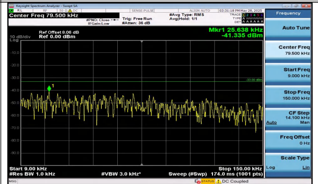
Band13-5MHz-QPSK-23255-1RB#24-0.009~0.15-PASS
