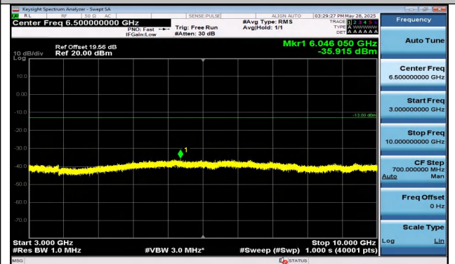
Band13-5MHz-16QAM-23230-25RB#0-3000~10000-PASS
