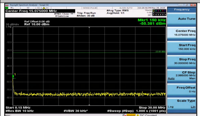
Band13-5MHz-QPSK-23255-1RB#0-0.15~30-PASS
