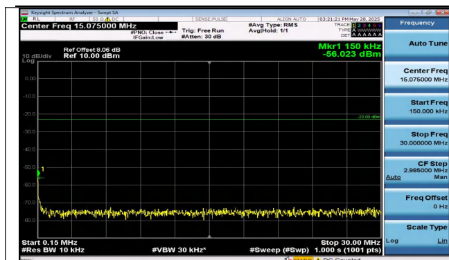
Band13-5MHz-QPSK-23205-1RB#24-0.15~30-PASS
