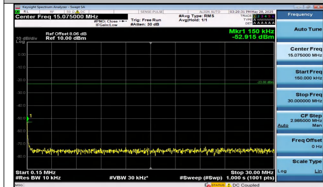
Band13-5MHz-16QAM-23205-1RB#0-0.15~30-PASS
