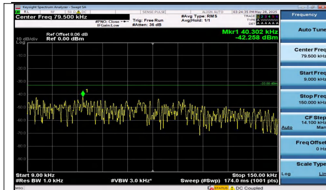
Band13-5MHz-QPSK-23230-1RB#0-0.009~0.15-PASS
