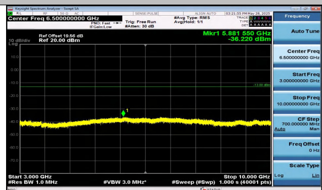
Band13-5MHz-QPSK-23205-1RB#24-3000~10000-PASS
