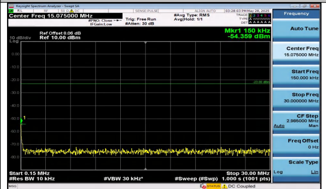
Band13-5MHz-QPSK-23230-25RB#0-0.15~30-PASS
