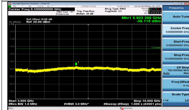
Band13-5MHz-QPSK-23255-1RB#0-3000~10000-PASS
