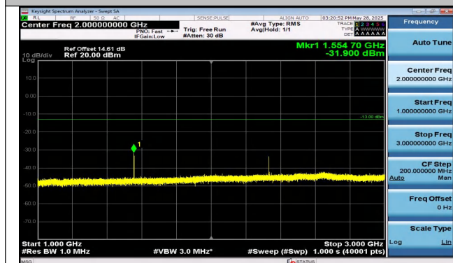
Band13-5MHz-16QAM-23205-1RB#0-1000~3000-PASS
