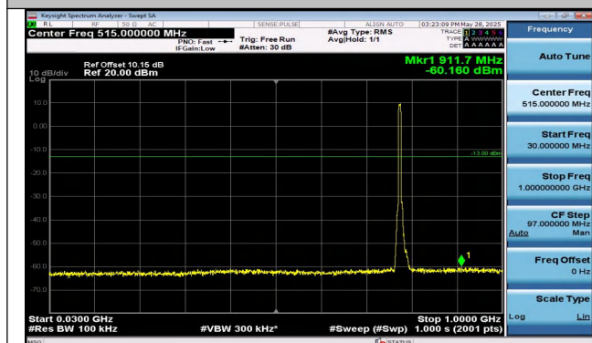
Band13-5MHz-QPSK-23205-25RB#0-30~1000-PASS
