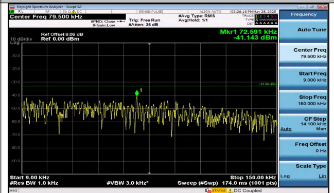
Band13-5MHz-QPSK-23230-1RB#24-0.009~0.15-PASS
