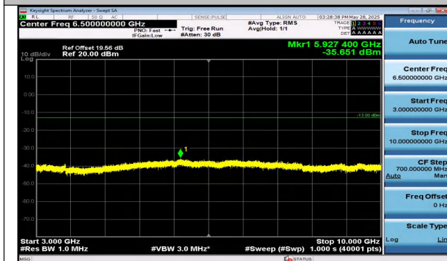
Band13-5MHz-QPSK-23230-25RB#0-3000~10000-PASS
