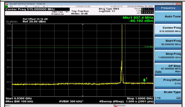
Band13-5MHz-QPSK-23230-1RB#24-30~1000-PASS
