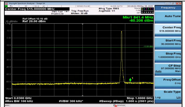
Band13-5MHz-16QAM-23230-25RB#0-30~1000-PASS
