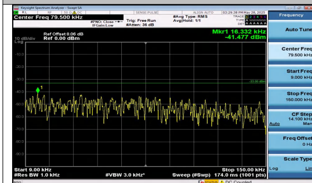
Band13-5MHz-QPSK-23255-1RB#0-0.009~0.15-PASS
