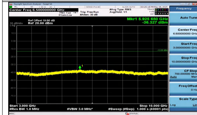
Band13-5MHz-QPSK-23230-1RB#0-3000~10000-PASS
