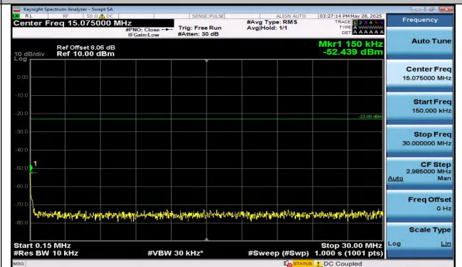
Band13-5MHz-16QAM-23230-1RB#24-0.15~30-PASS
