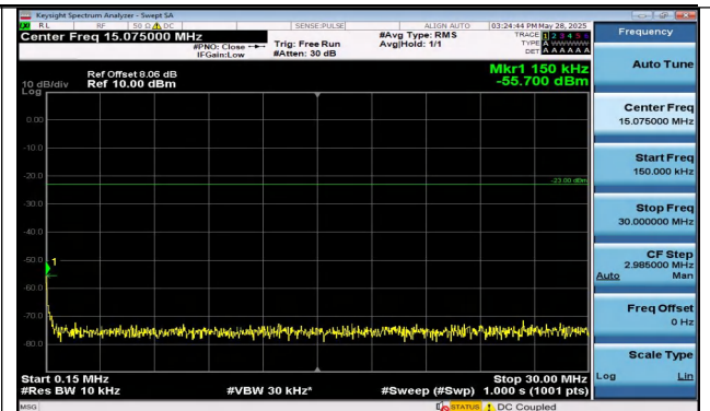
Band13-5MHz-QPSK-23230-1RB#0-0.15~30-PASS
