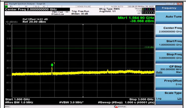
Band13-5MHz-QPSK-23230-25RB#0-1000~3000-PASS
