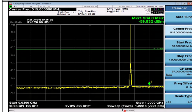
Band13-5MHz-QPSK-23230-1RB#0-30~1000-PASS
