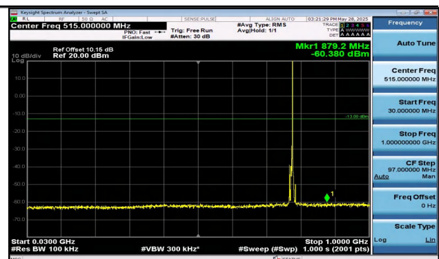
Band13-5MHz-QPSK-23205-1RB#24-30~1000-PASS
