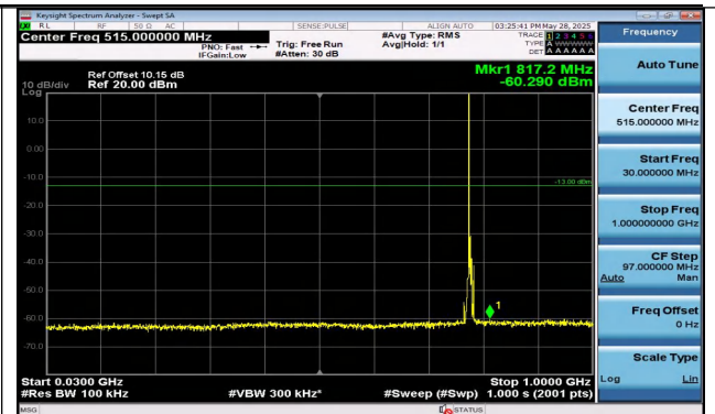
Band13-5MHz-16QAM-23230-1RB#0-30~1000-PASS
