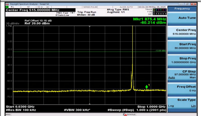
Band13-5MHz-QPSK-23255-1RB#24-30~1000-PASS
