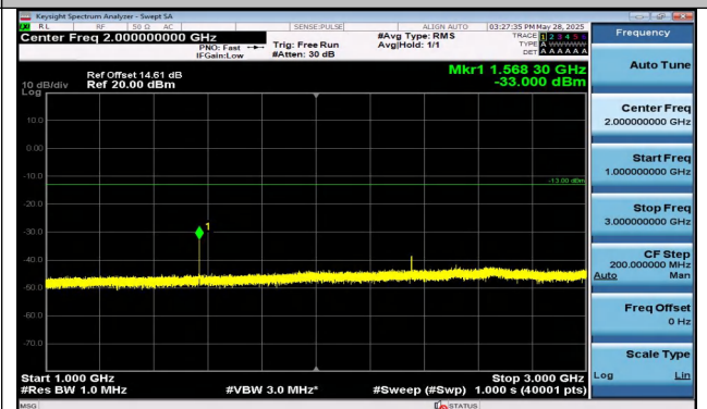
Band13-5MHz-16QAM-23230-1RB#24-1000~3000-PASS
