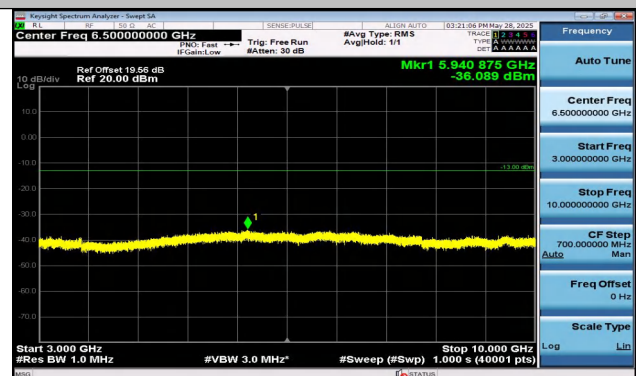
Band13-5MHz-16QAM-23205-1RB#0-3000~10000-PASS
