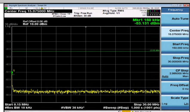
Band13-5MHz-QPSK-23205-25RB#0-0.15~30-PASS
