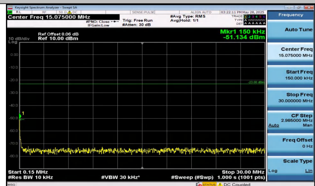
Band13-5MHz-16QAM-23205-1RB#24-0.15~30-PASS
