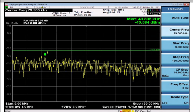
Band13-5MHz-16QAM-23230-1RB#0-0.009~0.15-PASS
