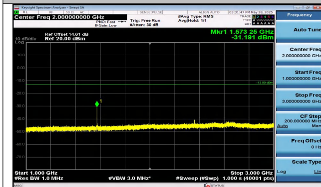
Band13-5MHz-QPSK-23255-1RB#24-1000~3000-PASS
