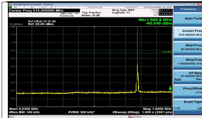
Band13-5MHz-QPSK-23255-1RB#0-30~1000-PASS
