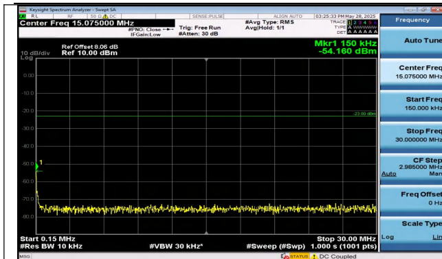
Band13-5MHz-16QAM-23230-1RB#0-0.15~30-PASS
