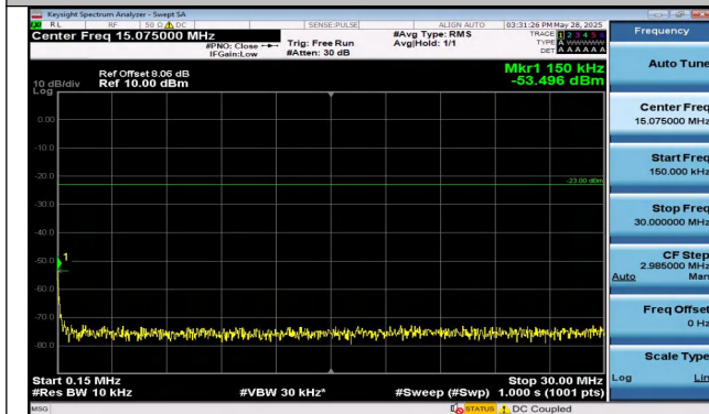
Band13-5MHz-QPSK-23255-1RB#24-0.15~30-PASS
