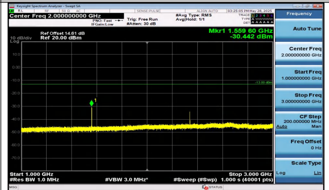
Band13-5MHz-QPSK-23230-1RB#0-1000~3000-PASS
