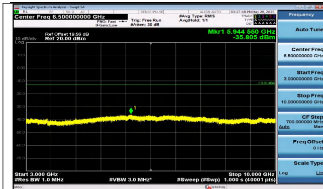
Band13-5MHz-16QAM-23230-1RB#24-3000~10000-PASS
