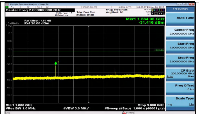
Band13-5MHz-QPSK-23255-1RB#0-1000~3000-PASS
