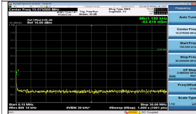
Band13-5MHz-16QAM-23230-25RB#0-0.15~30-PASS
