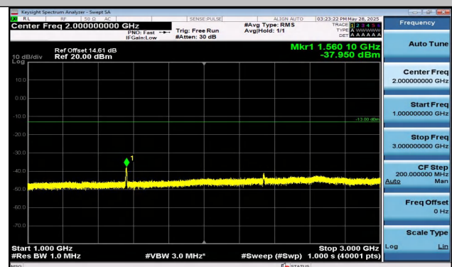
Band13-5MHz-QPSK-23205-25RB#0-1000~3000-PASS
