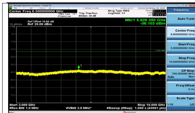
Band13-5MHz-QPSK-23205-25RB#0-3000~10000-PASS
