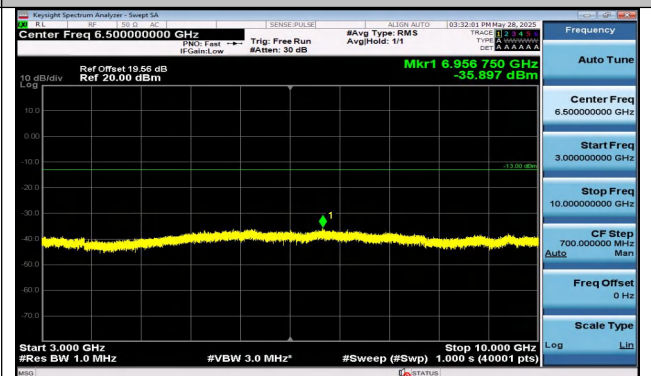
Band13-5MHz-QPSK-23255-1RB#24-3000~10000-PASS
