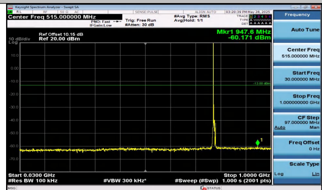
Band13-5MHz-16QAM-23205-1RB#0-30~1000-PASS
