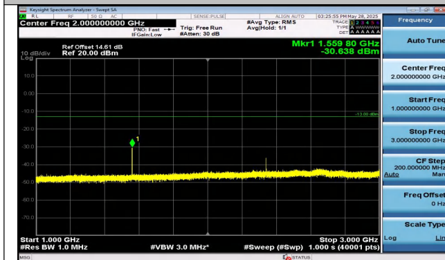
Band13-5MHz-16QAM-23230-1RB#0-1000~3000-PASS
