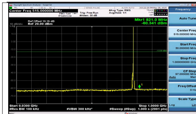
Band13-5MHz-16QAM-23205-1RB#24-30~1000-PASS
