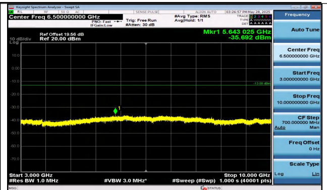
Band13-5MHz-QPSK-23230-1RB#24-3000~10000-PASS
