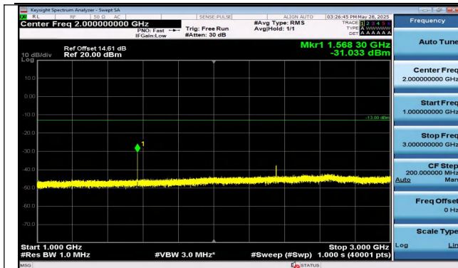
Band13-5MHz-QPSK-23230-1RB#24-1000~3000-PASS
