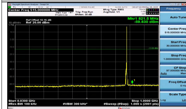
Band13-5MHz-16QAM-23230-1RB#24-30~1000-PASS
