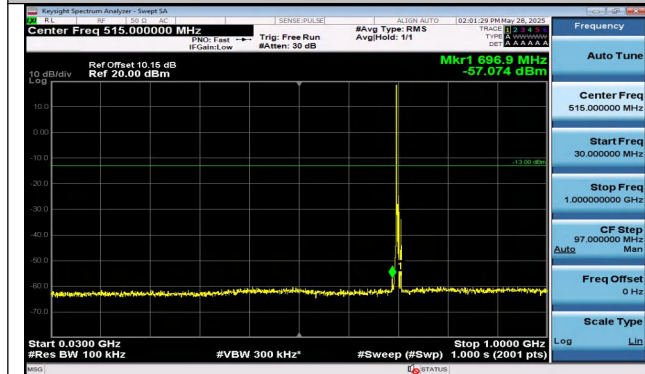
Band12-5MHz-QPSK-23095-1RB#0-30~1000-PASS
