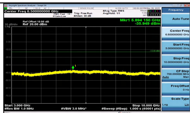
Band12-5MHz-16QAM-23035-25RB#0-3000~10000-PASS
