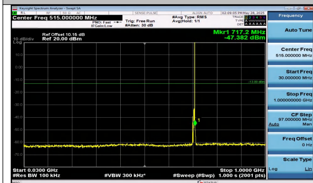
Band12-5MHz-16QAM-23155-1RB#24-30~1000-PASS
