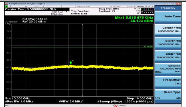
Band12-5MHz-16QAM-23095-1RB#0-3000~10000-PASS
