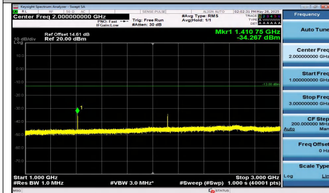
Band12-5MHz-16QAM-23095-1RB#0-1000~3000-PASS
