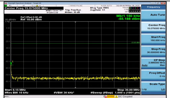
Band12-5MHz-QPSK-23155-25RB#0-0.15~30-PASS
