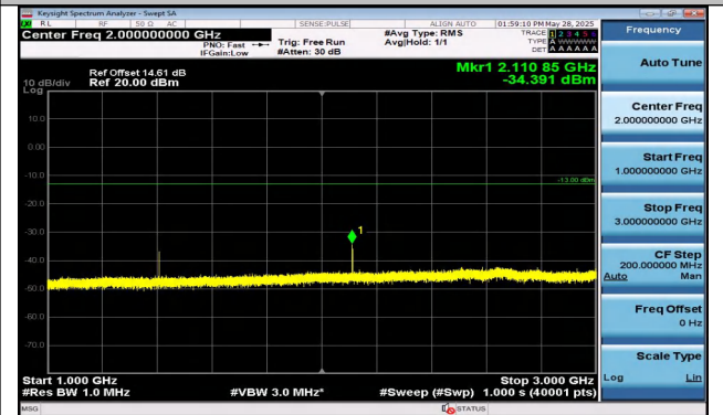
Band12-5MHz-16QAM-23035-1RB#24-1000~3000-PASS
