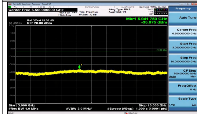
Band12-5MHz-QPSK-23095-1RB#0-3000~10000-PASS
