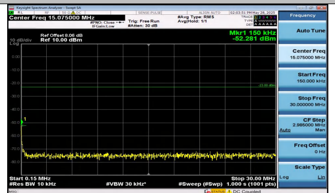
Band12-5MHz-16QAM-23095-1RB#24-0.15~30-PASS
