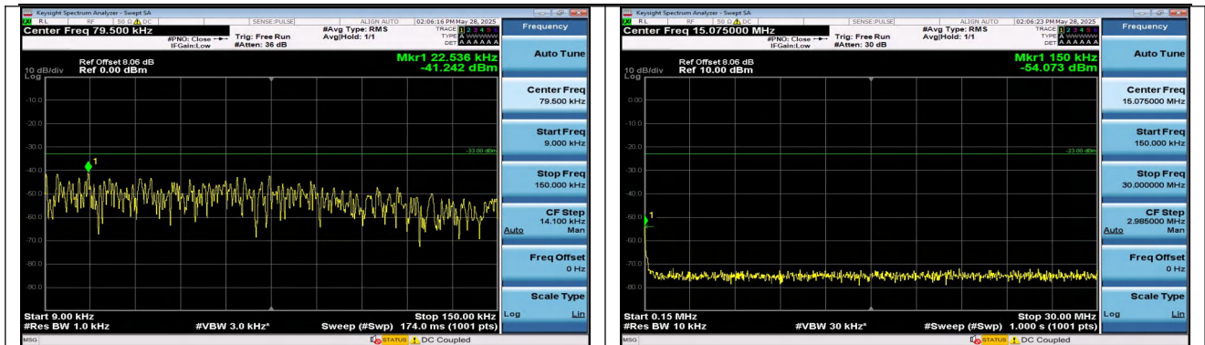
Band12-5MHz-QPSK-23155-1RB#0-0.009~0.15-PASS
