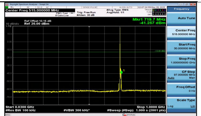
Band12-5MHz-16QAM-23155-1RB#0-30~1000-PASS
