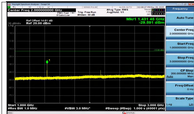
Band12-5MHz-QPSK-23155-1RB#24-1000~3000-PASS
