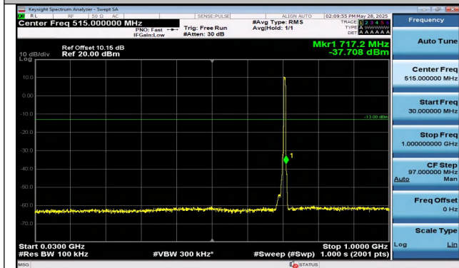
Band12-5MHz-QPSK-23155-25RB#0-30~1000-PASS
