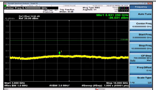
Band12-5MHz-16QAM-23155-1RB#0-3000~10000-PASS
