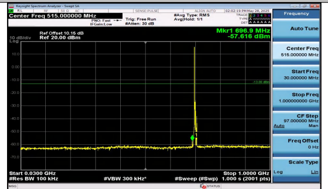
Band12-5MHz-16QAM-23095-1RB#0-30~1000-PASS
