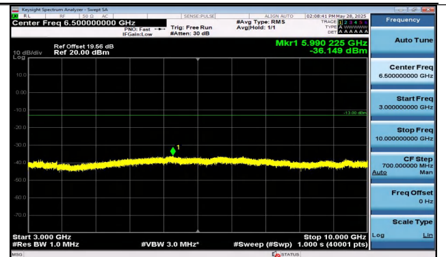
Band12-5MHz-QPSK-23155-1RB#24-3000~10000-PASS
