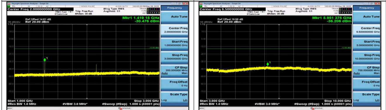
Band12-5MHz-QPSK-23095-1RB#24-1000~3000-PASS
