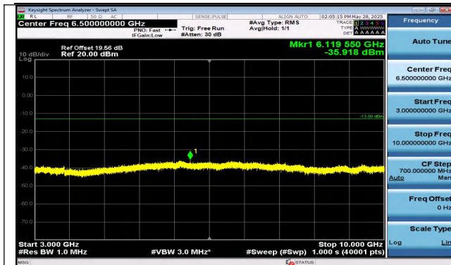
Band12-5MHz-QPSK-23095-25RB#0-3000~10000-PASS
