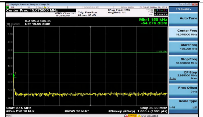
Band12-5MHz-16QAM-23035-1RB#24-0.15~30-PASS
