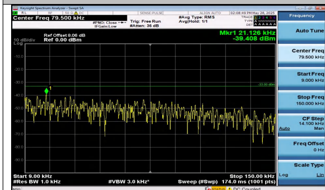
Band12-5MHz-16QAM-23155-1RB#24-0.009~0.15-PASS
