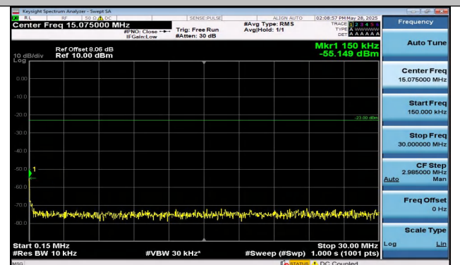
Band12-5MHz-16QAM-23155-1RB#24-0.15~30-PASS
