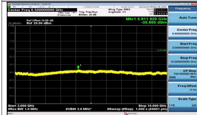
Band12-5MHz-QPSK-23155-25RB#0-3000~10000-PASS
