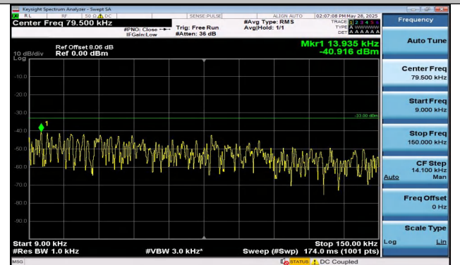
Band12-5MHz-16QAM-23155-1RB#0-0.009~0.15-PASS
