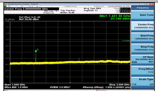
Band12-5MHz-16QAM-23155-1RB#24-1000~3000-PASS
