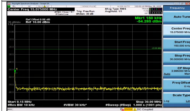
Band12-5MHz-16QAM-23095-1RB#0-0.15~30-PASS
