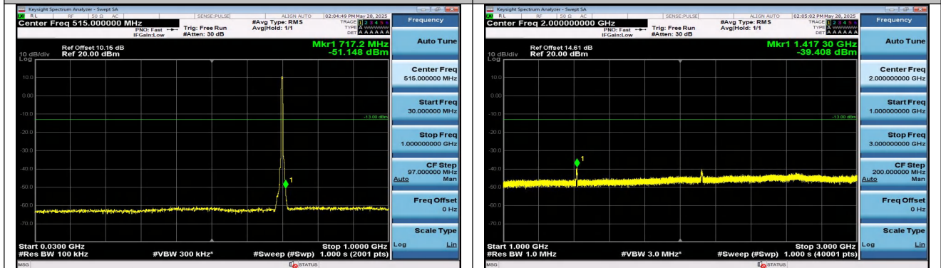
Band12-5MHz-QPSK-23095-25RB#0-30~1000-PASS
