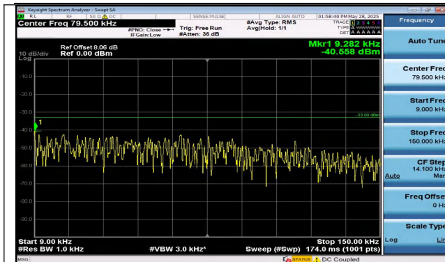
Band12-5MHz-16QAM-23035-1RB#24-0.009~0.15-PASS
