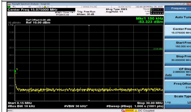
Band12-5MHz-16QAM-23035-25RB#0-0.15~30-PASS
