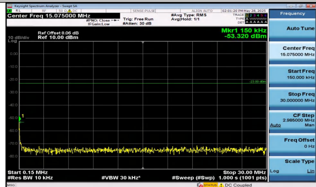
Band12-5MHz-QPSK-23095-1RB#0-0.15~30-PASS
