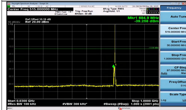
Band12-5MHz-16QAM-23035-1RB#24-30~1000-PASS
