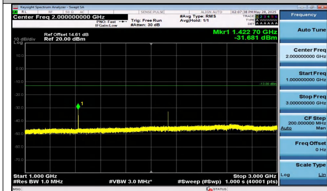
Band12-5MHz-16QAM-23155-1RB#0-1000~3000-PASS
