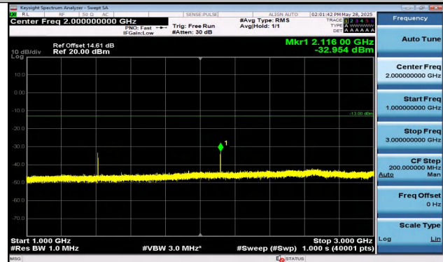
Band12-5MHz-QPSK-23095-1RB#0-1000~3000-PASS
