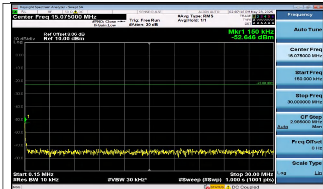
Band12-5MHz-16QAM-23155-1RB#0-0.15~30-PASS
