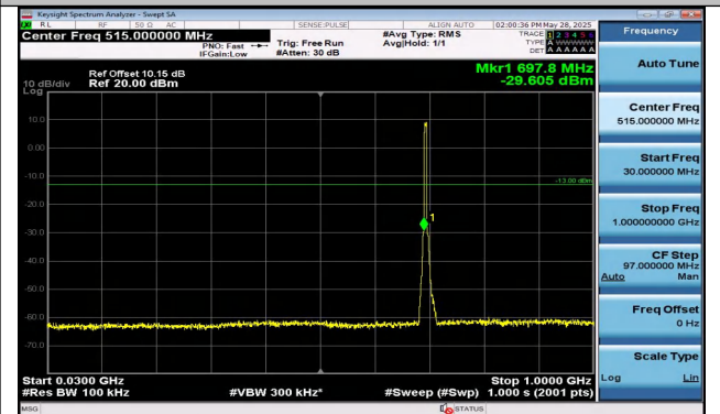
Band12-5MHz-16QAM-23035-25RB#0-30~1000-PASS
