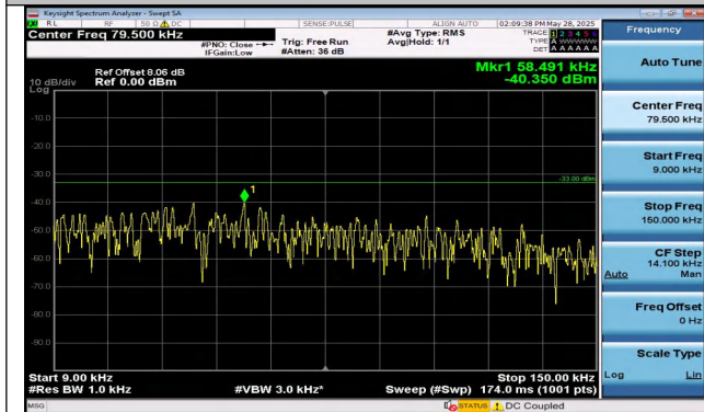
Band12-5MHz-QPSK-23155-25RB#0-0.009~0.15-PASS
