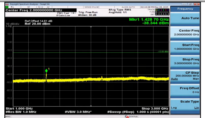
Band12-5MHz-QPSK-23155-25RB#0-1000~3000-PASS
