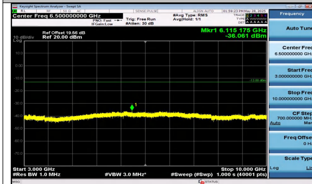
Band12-5MHz-16QAM-23035-1RB#24-3000~10000-PASS
