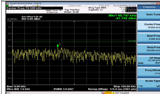
Band12-3MHz-QPSK-23165-1RB#0-0.009~0.15-PASS
