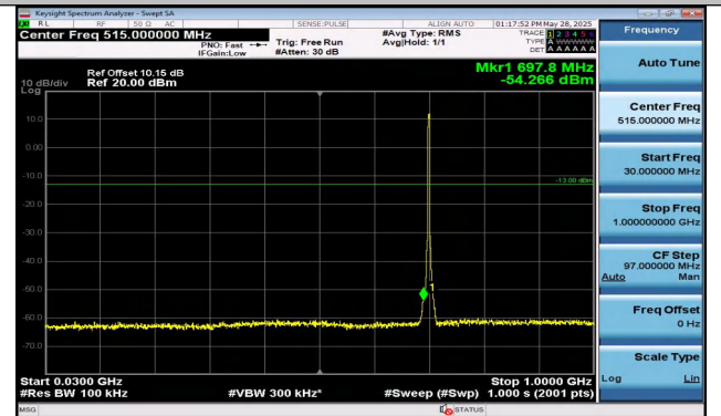
Band12-3MHz-16QAM-23095-15RB#0-30~1000-PASS
