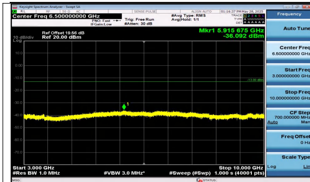
Band12-3MHz-16QAM-23095-1RB#14-3000~10000-PASS
