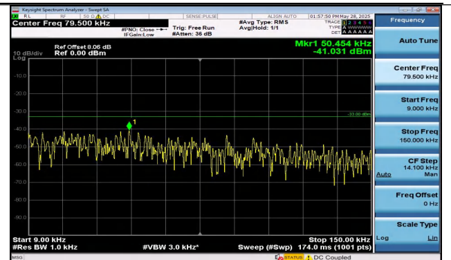
Band12-5MHz-QPSK-23035-1RB#24-0.009~0.15-PASS
