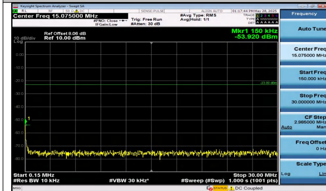
Band12-3MHz-16QAM-23095-15RB#0-0.15~30-PASS
