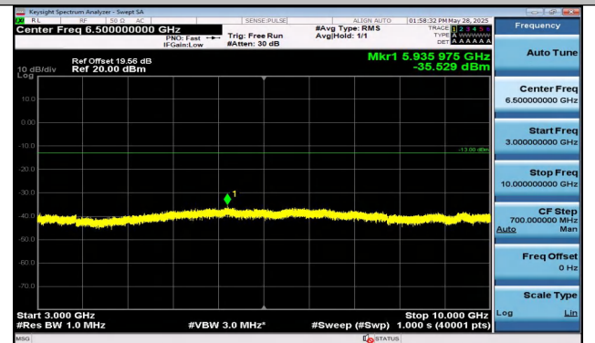
Band12-5MHz-QPSK-23035-1RB#24-3000~10000-PASS
