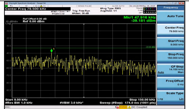
Band12-3MHz-16QAM-23165-1RB#0-0.009~0.15-PASS
