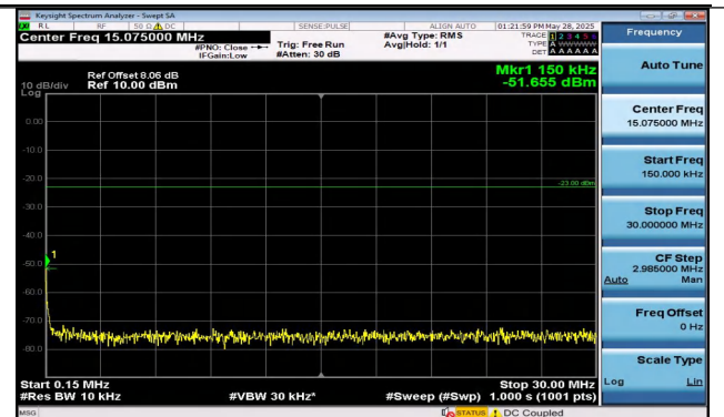
Band12-3MHz-QPSK-23165-15RB#0-0.15~30-PASS
