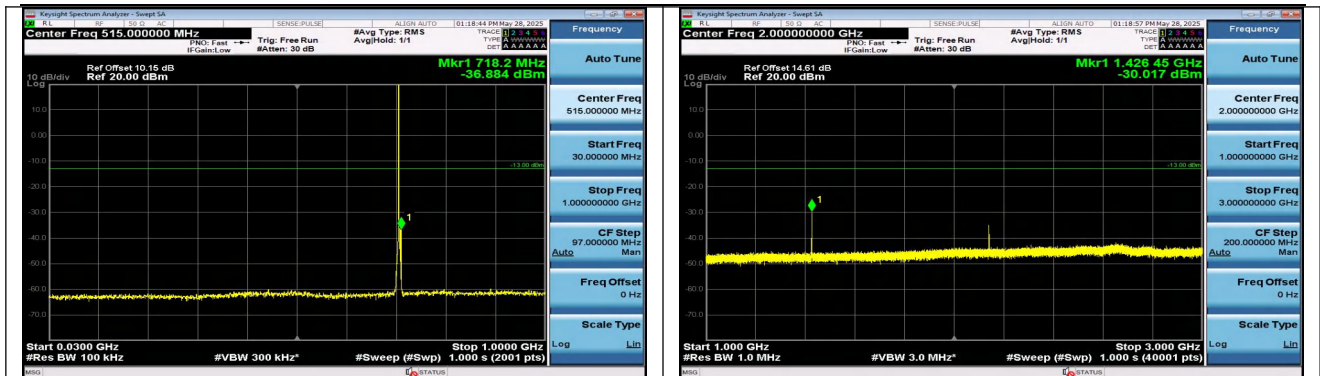
Band12-3MHz-QPSK-23165-1RB#0-30~1000-PASS
