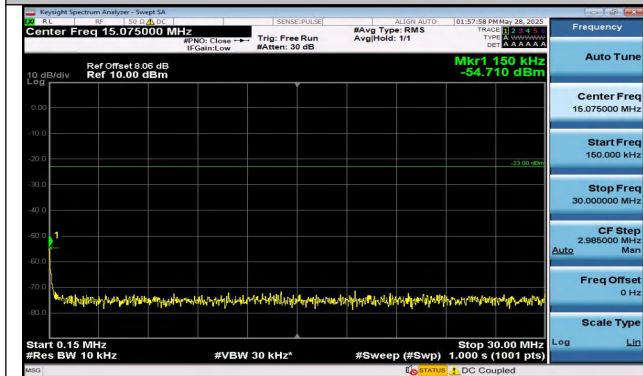
Band12-5MHz-QPSK-23035-1RB#24-0.15~30-PASS
