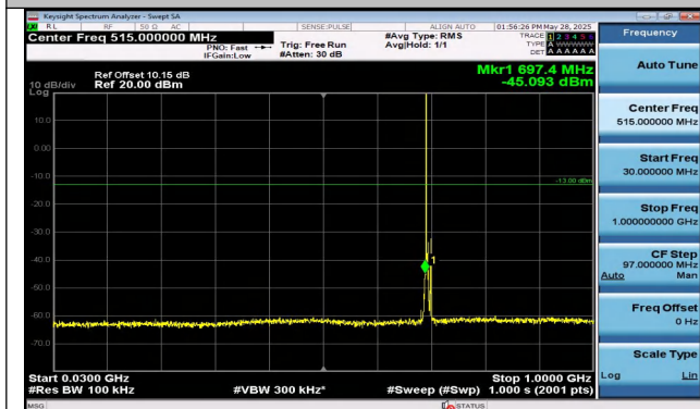
Band12-5MHz-QPSK-23035-1RB#0-30~1000-PASS
