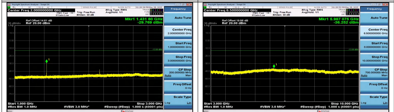
Band12-3MHz-QPSK-23165-1RB#14-1000~3000-PASS
