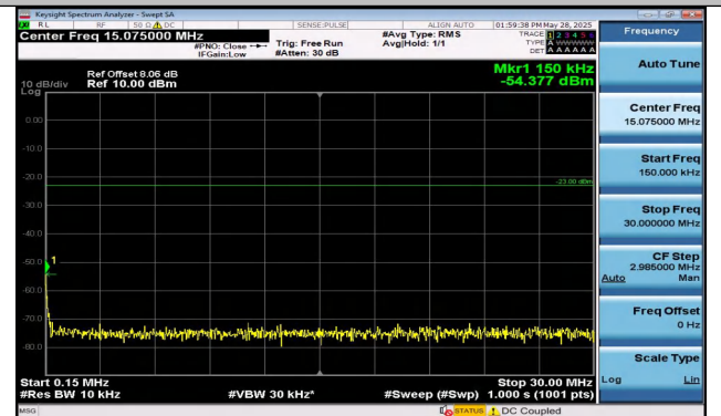
Band12-5MHz-QPSK-23035-25RB#0-0.15~30-PASS
