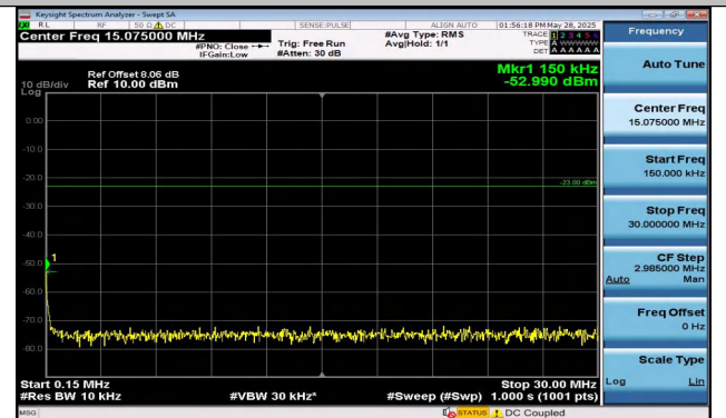
Band12-5MHz-QPSK-23035-1RB#0-0.15~30-PASS
