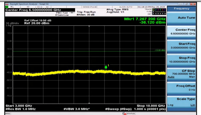
Band12-3MHz-16QAM-23095-15RB#0-3000~10000-PASS
