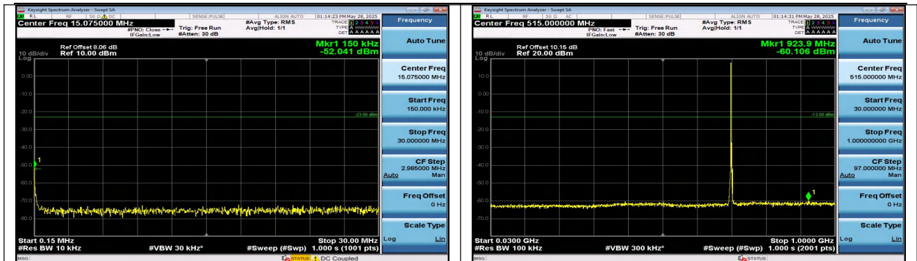
Band12-3MHz-16QAM-23095-1RB#0-0.15~30-PASS
