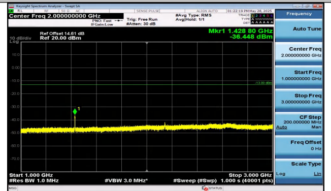
Band12-3MHz-QPSK-23165-15RB#0-1000~3000-PASS
