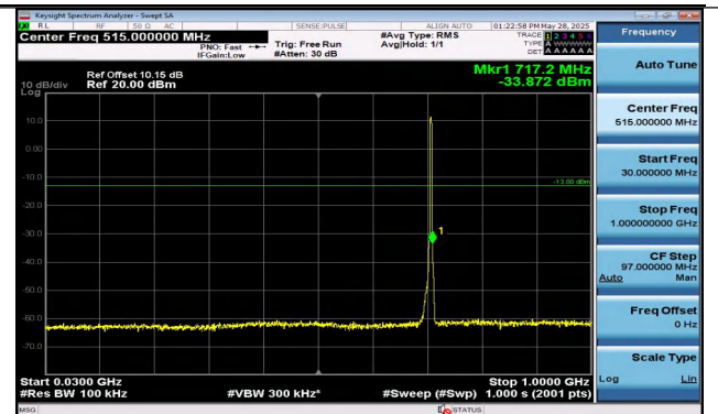
Band12-3MHz-16QAM-23165-15RB#0-30~1000-PASS
