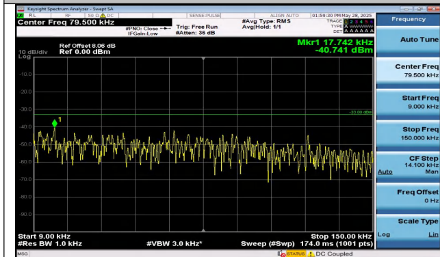
Band12-5MHz-QPSK-23035-25RB#0-0.009~0.15-PASS
