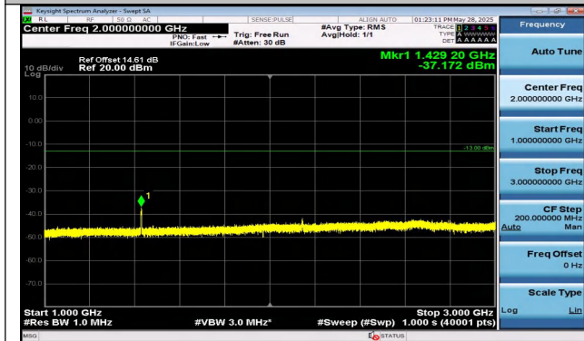
Band12-3MHz-16QAM-23165-15RB#0-1000~3000-PASS
