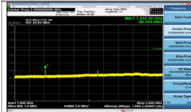
Band12-3MHz-16QAM-23095-15RB#0-1000~3000-PASS
