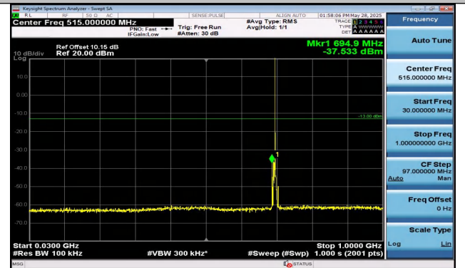
Band12-5MHz-QPSK-23035-1RB#24-30~1000-PASS
