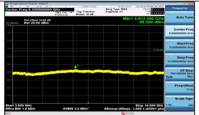
Band12-3MHz-16QAM-23165-15RB#0-3000~10000-PASS
