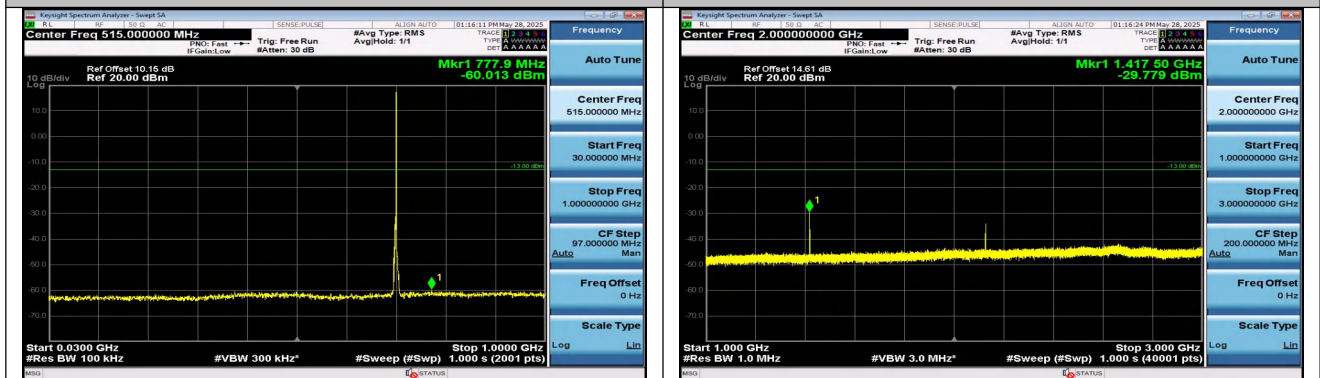
Band12-3MHz-16QAM-23095-1RB#14-30~1000-PASS
