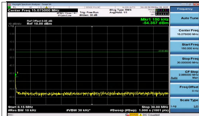
Band12-3MHz-16QAM-23165-15RB#0-0.15~30-PASS
