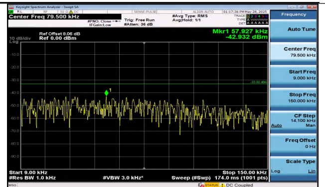
Band12-3MHz-16QAM-23095-15RB#0-0.009~0.15-PASS
