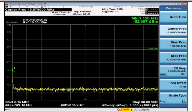
Band12-3MHz-QPSK-23165-1RB#0-0.15~30-PASS
