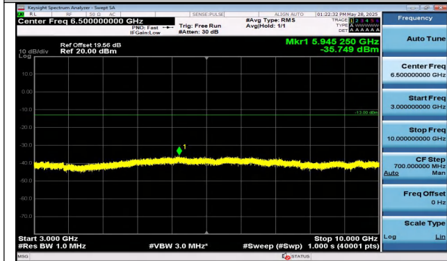
Band12-3MHz-QPSK-23165-15RB#0-3000~10000-PASS
