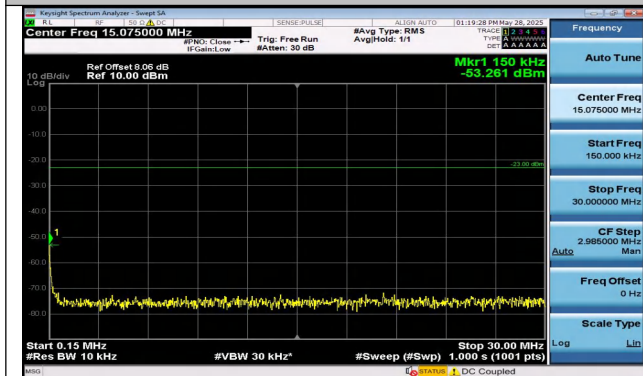
Band12-3MHz-16QAM-23165-1RB#0-0.15~30-PASS
