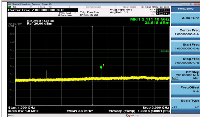
Band12-5MHz-QPSK-23035-1RB#24-1000~3000-PASS
