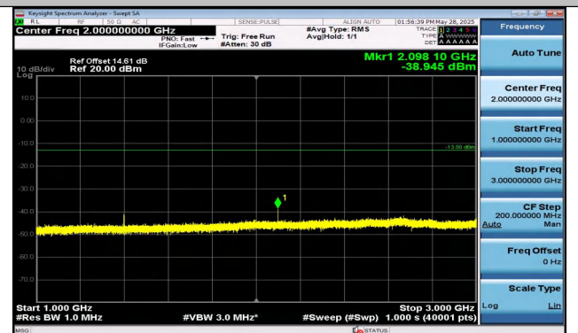
Band12-5MHz-QPSK-23035-1RB#0-1000~3000-PASS
