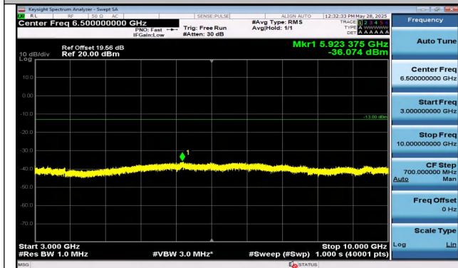
Band12-1.4MHz-16QAM-23173-1RB#5-3000~10000-PASS
