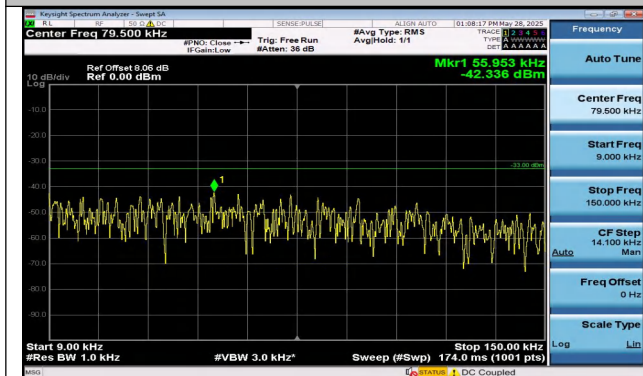
Band12-3MHz-QPSK-23025-1RB#0-0.009~0.15-PASS
