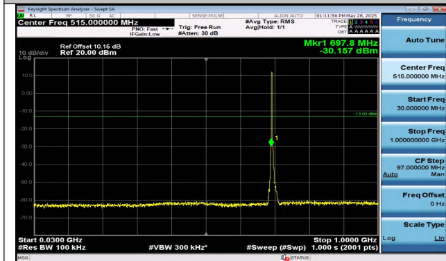
Band12-3MHz-QPSK-23025-15RB#0-30~1000-PASS
