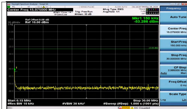
Band12-3MHz-QPSK-23025-1RB#14-0.15~30-PASS
