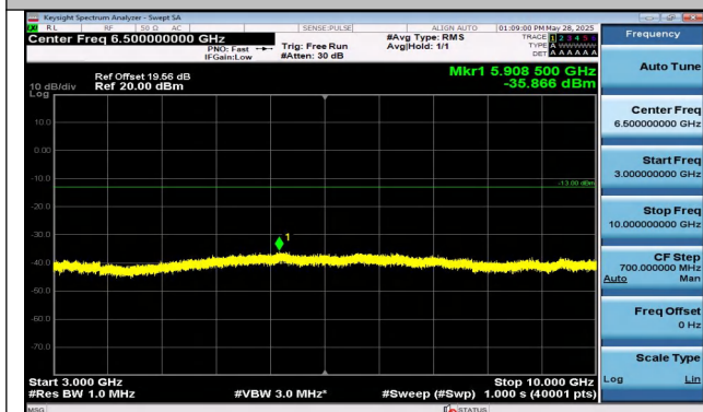
Band12-3MHz-QPSK-23025-1RB#0-3000~10000-PASS
