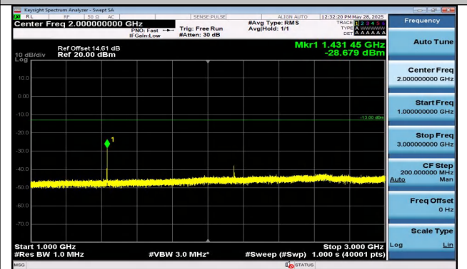
Band12-1.4MHz-16QAM-23173-1RB#5-1000~3000-PASS
