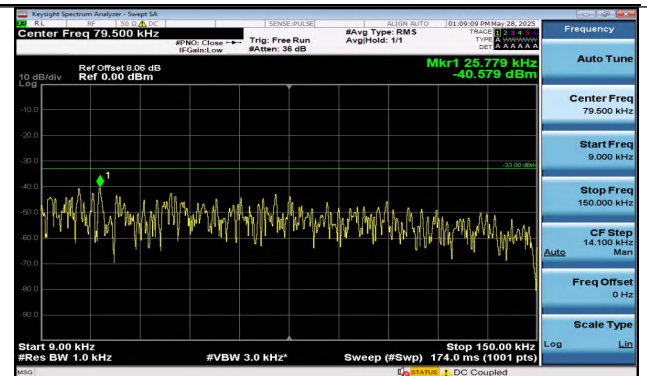
Band12-3MHz-16QAM-23025-1RB#0-0.009~0.15-PASS
