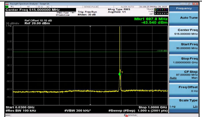
Band12-3MHz-16QAM-23025-1RB#0-30~1000-PASS
