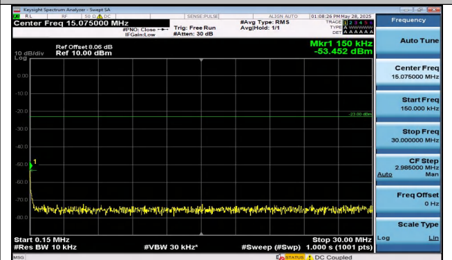
Band12-3MHz-QPSK-23025-1RB#0-0.15~30-PASS
