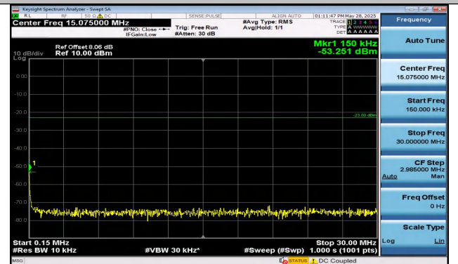
Band12-3MHz-QPSK-23025-15RB#0-0.15~30-PASS
