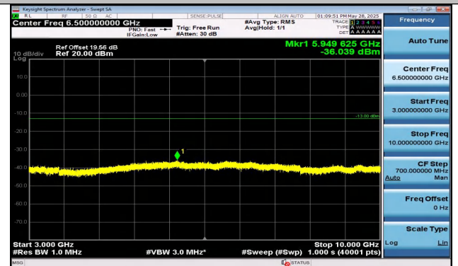
Band12-3MHz-16QAM-23025-1RB#0-3000~10000-PASS
