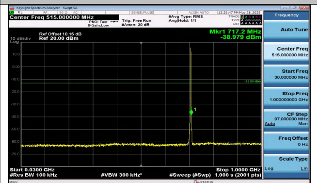
Band12-1.4MHz-16QAM-23173-6RB#0-30~1000-PASS
