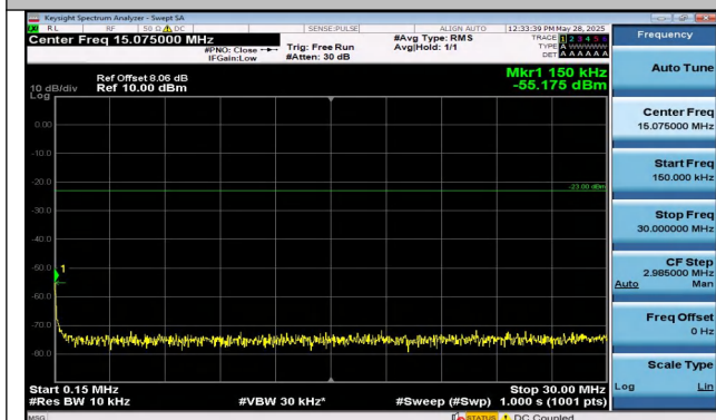
Band12-1.4MHz-16QAM-23173-6RB#0-0.15~30-PASS
