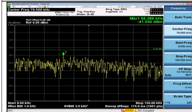
Band12-3MHz-QPSK-23025-15RB#0-0.009~0.15-PASS
