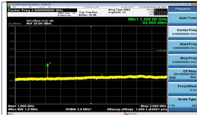
Band12-1.4MHz-16QAM-23173-6RB#0-1000~3000-PASS
