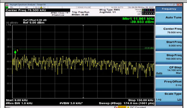
Band12-3MHz-QPSK-23025-1RB#14-0.009~0.15-PASS
