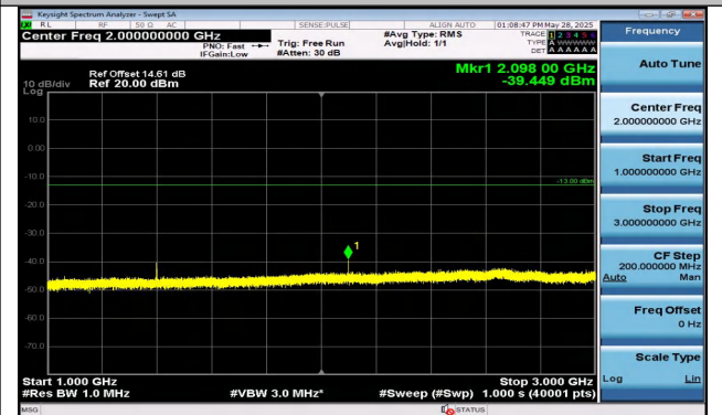
Band12-3MHz-QPSK-23025-1RB#0-1000~3000-PASS
