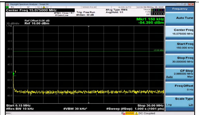
Band12-1.4MHz-16QAM-23173-1RB#5-0.15~30-PASS
