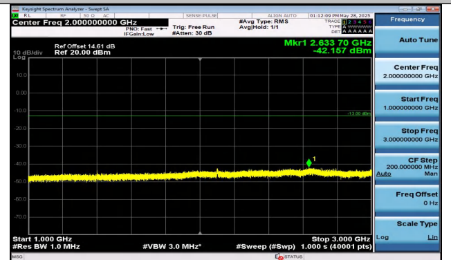
Band12-3MHz-QPSK-23025-15RB#0-1000~3000-PASS
