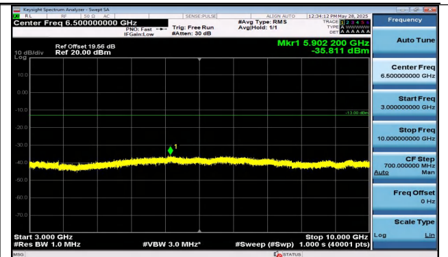
Band12-1.4MHz-16QAM-23173-6RB#0-3000~10000-PASS S
