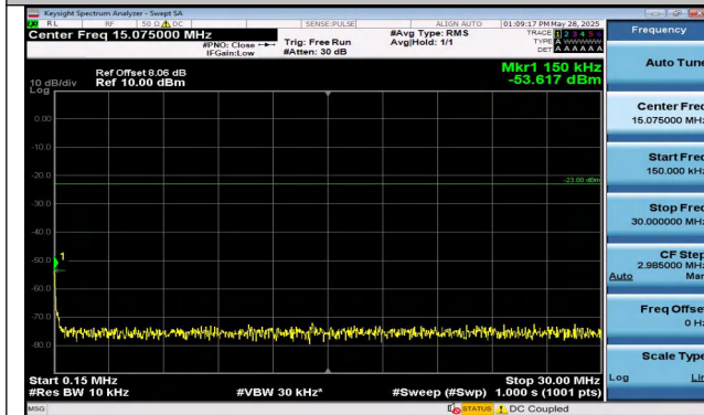
Band12-3MHz-16QAM-23025-1RB#0-0.15~30-PASS
