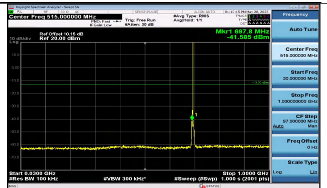
Band12-3MHz-QPSK-23025-1RB#14-30~1000-PASS
