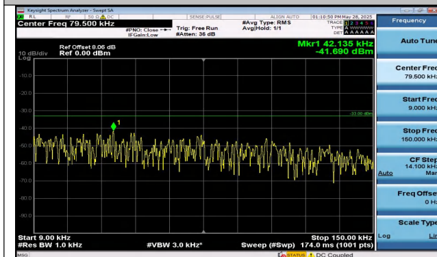
Band12-3MHz-16QAM-23025-1RB#14-0.009~0.15-PASS
