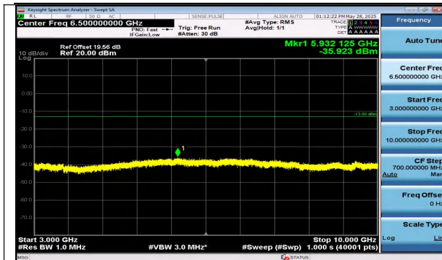
Band12-3MHz-QPSK-23025-15RB#0-3000~10000-PASS
