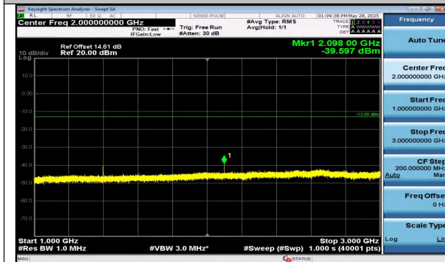
Band12-3MHz-16QAM-23025-1RB#0-1000~3000-PASS
