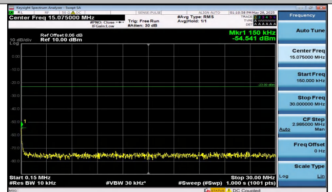
Band12-3MHz-16QAM-23025-1RB#14-0.15~30-PASS
