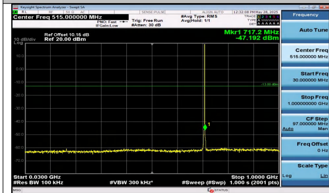
Band12-1.4MHz-16QAM-23173-1RB#5-30~1000-PASS
