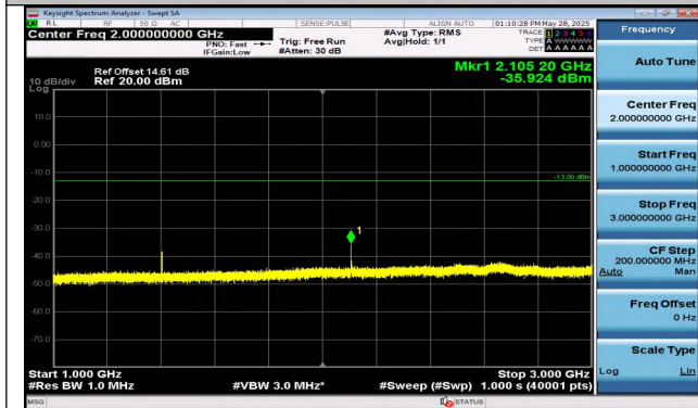
Band12-3MHz-QPSK-23025-1RB#14-1000~3000-PASS
