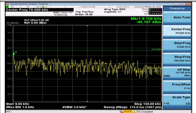
Band12-1.4MHz-16QAM-23173-6RB#0-0.009~0.15-PASS
