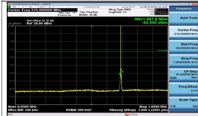
Band12-3MHz-QPSK-23025-1RB#0-30~1000-PASS
