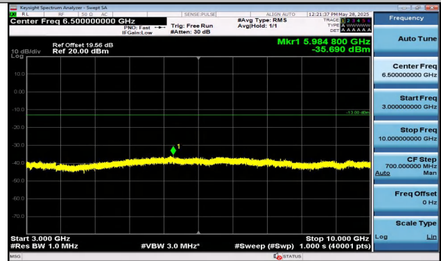
Band12-1.4MHz-QPSK-23017-1RB#5-3000~10000-PASS
