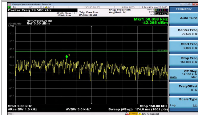
Band12-1.4MHz-16QAM-23095-1RB#5-0.009~0.15-PASS
