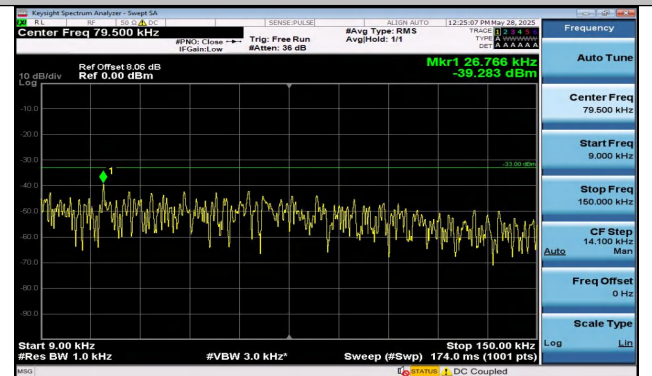
Band12-1.4MHz-16QAM-23095-1RB#0-0.009~0.15-PASS
