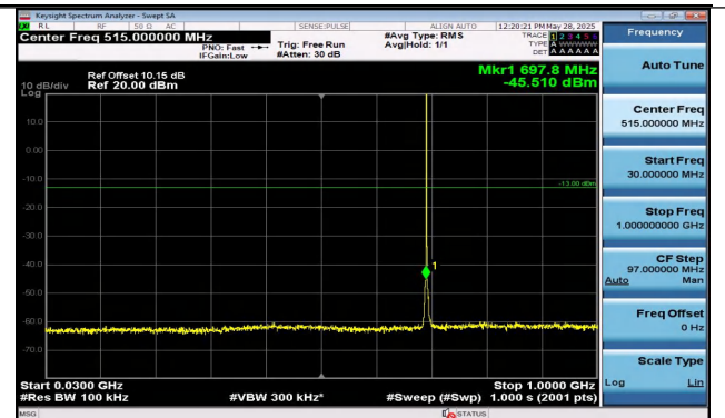
Band12-1.4MHz-16QAM-23017-1RB#0-30~1000-PASS
