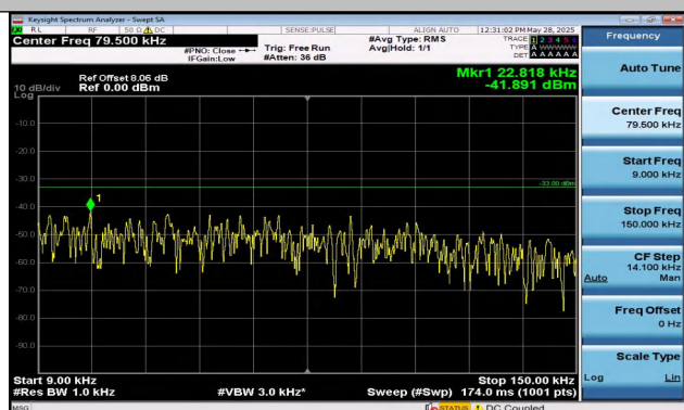
Band12-1.4MHz-QPSK-23173-1RB#5-0.009~0.15-PASS
