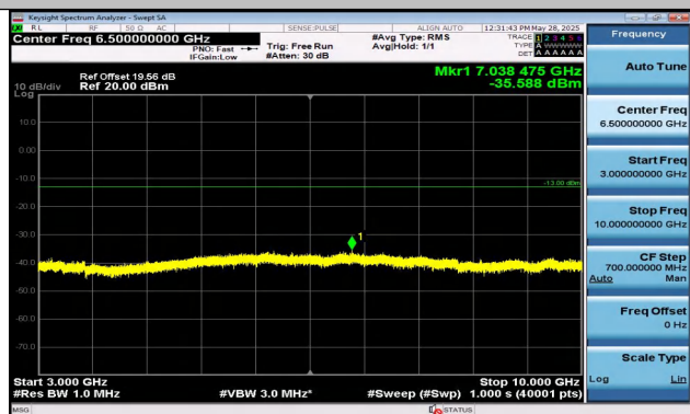
Band12-1.4MHz-QPSK-23173-1RB#5-3000~10000-PASS
