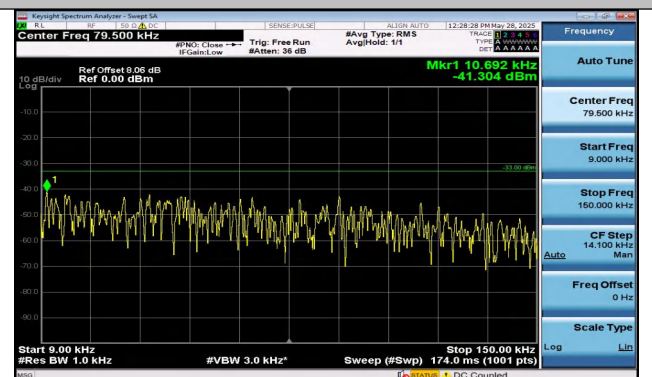
Band12-1.4MHz-16QAM-23095-6RB#0-0.009~0.15-PASS
