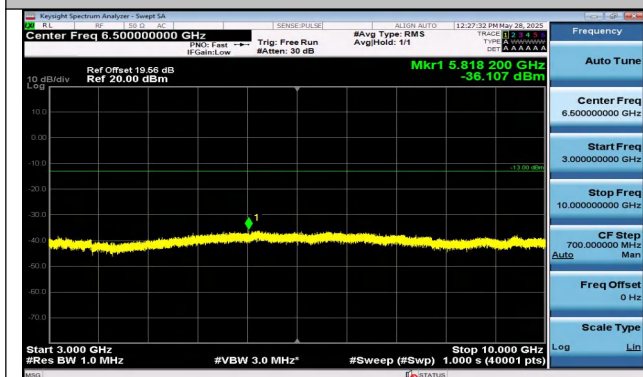
Band12-1.4MHz-16QAM-23095-1RB#5-3000~10000-PASS
