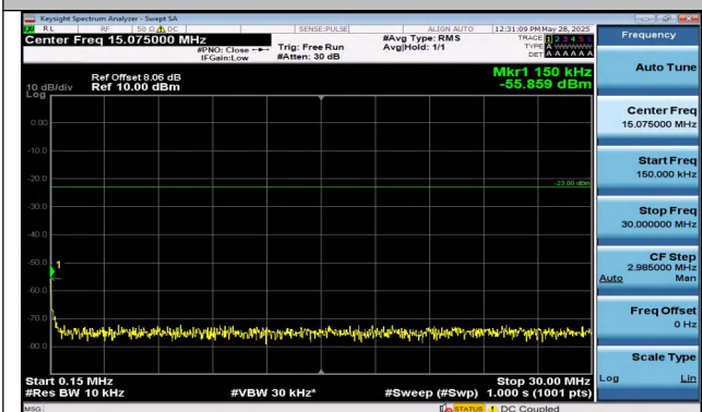
Band12-1.4MHz-QPSK-23173-1RB#5-0.15~30-PASS
