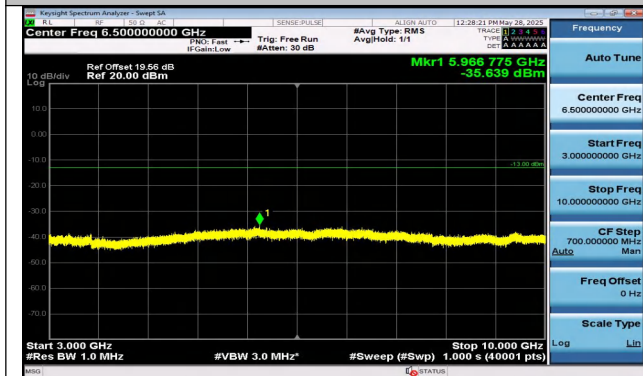
Band12-1.4MHz-QPSK-23095-6RB#0-3000~10000-PASS
