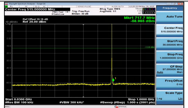
Band12-1.4MHz-16QAM-23095-1RB#0-30~1000-PASS
