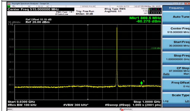
Band12-1.4MHz-QPSK-23095-6RB#0-30~1000-PASS
