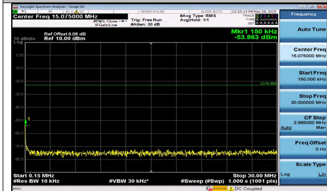
Band12-1.4MHz-16QAM-23095-1RB#0-0.15~30-PASS
