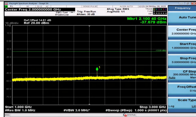
Band12-1.4MHz-QPSK-23017-1RB#5-1000~3000-PASS
