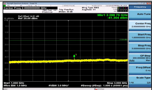
Band12-1.4MHz-QPSK-23017-6RB#0-1000~3000-PASS
