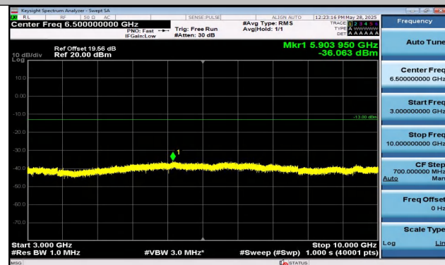
Band12-1.4MHz-QPSK-23017-6RB#0-3000~10000-PASS
