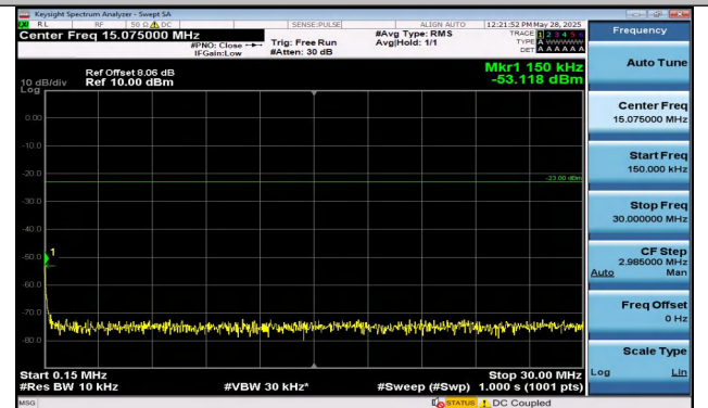
Band12-1.4MHz-16QAM-23017-1RB#5-0.15~30-PASS
