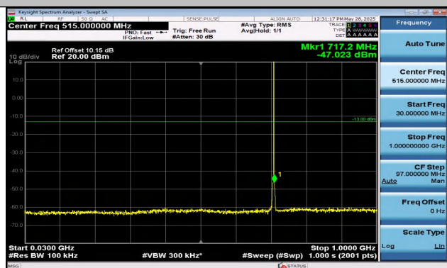
Band12-1.4MHz-QPSK-23173-1RB#5-30~1000-PASS
