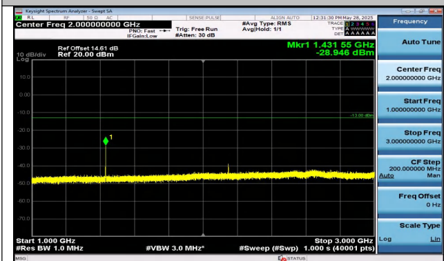
Band12-1.4MHz-QPSK-23173-1RB#5-1000~3000-PASS
