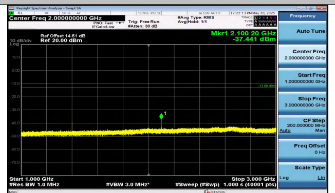
Band12-1.4MHz-16QAM-23017-1RB#5-1000~3000-PASS
