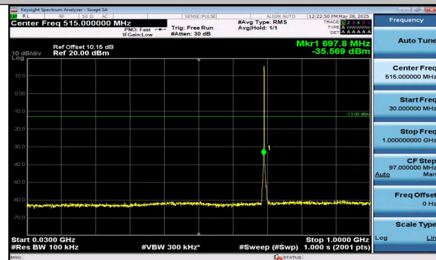
Band12-1.4MHz-QPSK-23017-6RB#0-30~1000-PASS
