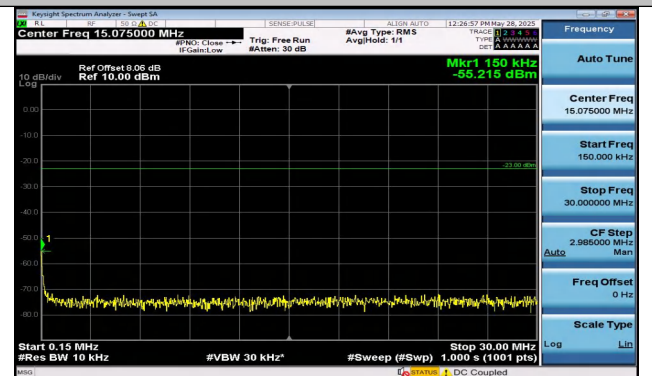
Band12-1.4MHz-16QAM-23095-1RB#5-0.15~30-PASS
