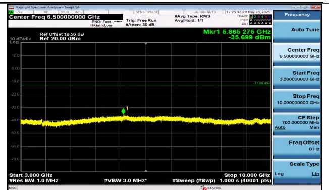
Band12-1.4MHz-16QAM-23095-1RB#0-3000~10000-PASS S
