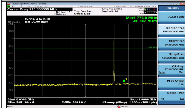
Band12-1.4MHz-16QAM-23095-1RB#5-30~1000-PASS
