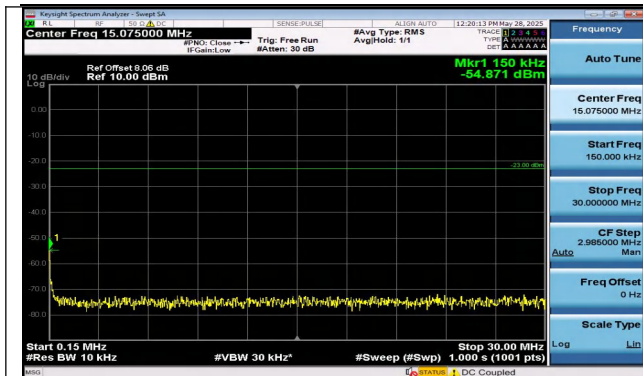
Band12-1.4MHz-16QAM-23017-1RB#0-0.15~30-PASS
