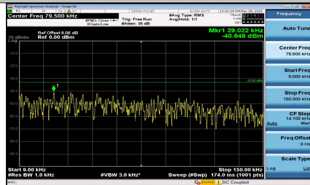
Band12-1.4MHz-QPSK-23017-6RB#0-0.009~0.15-PASS
