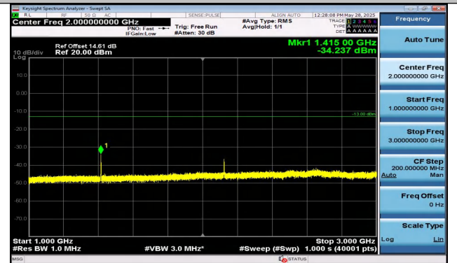
Band12-1.4MHz-QPSK-23095-6RB#0-1000~3000-PASS
