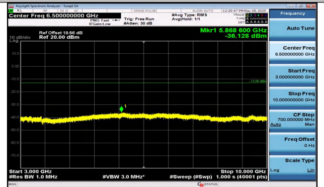
Band12-1.4MHz-16QAM-23017-1RB#0-3000~10000-PASS S
