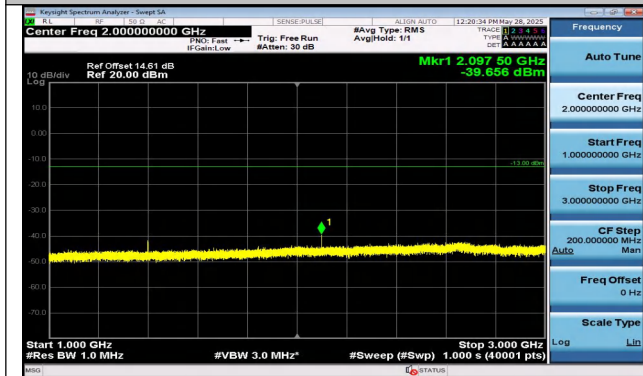
Band12-1.4MHz-16QAM-23017-1RB#0-1000~3000-PASS
