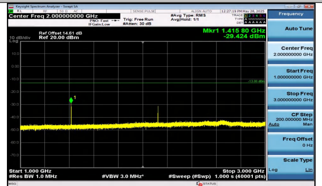
Band12-1.4MHz-16QAM-23095-1RB#5-1000~3000-PASS
