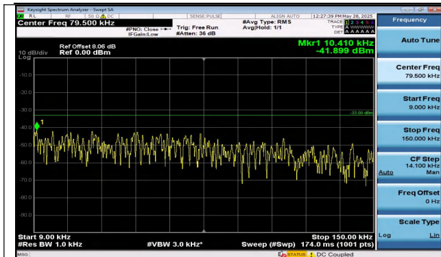
Band12-1.4MHz-QPSK-23095-6RB#0-0.009~0.15-PASS
