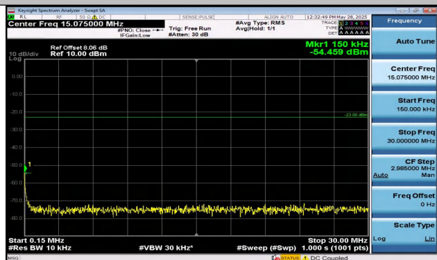
Band12-1.4MHz-QPSK-23173-6RB#0-0.15~30-PASS
