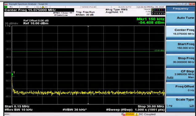
Band12-1.4MHz-QPSK-23017-6RB#0-0.15~30-PASS
