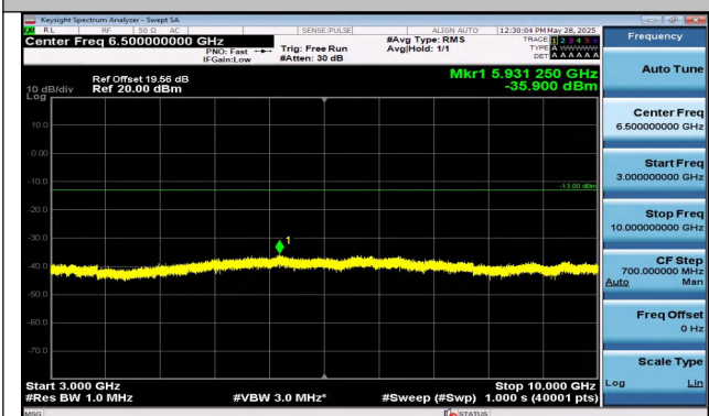
Band12-1.4MHz-QPSK-23173-1RB#0-3000~10000-PASS
