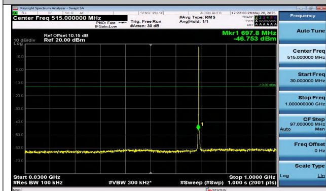
Band12-1.4MHz-16QAM-23017-1RB#5-30~1000-PASS
