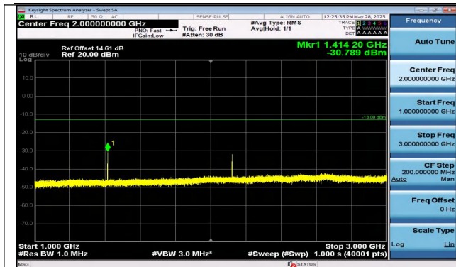
Band12-1.4MHz-16QAM-23095-1RB#0-1000~3000-PASS
