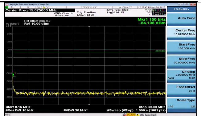
Band12-1.4MHz-QPSK-23095-6RB#0-0.15~30-PASS
