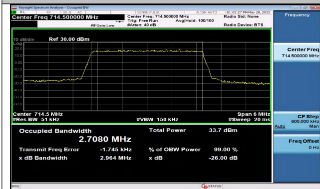
Band12-3MHz-QPSK-23165-15RB#0-PASS
