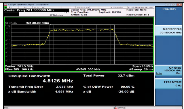
Band12-5MHz-16QAM-23035-25RB#0-PASS
