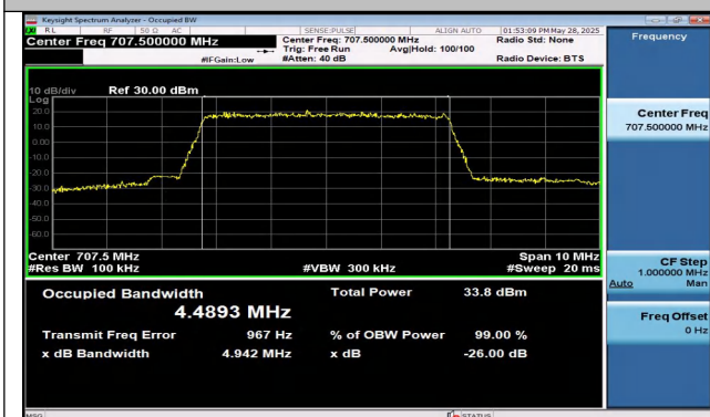
Band12-5MHz-QPSK-23095-25RB#0-PASS
