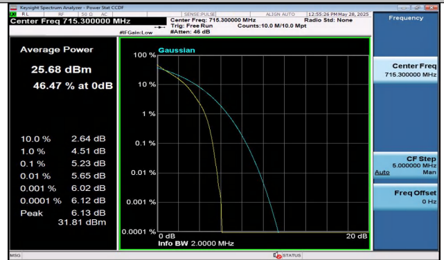
Band12-1.4MHz-QPSK-23173-6RB#0-PASS
