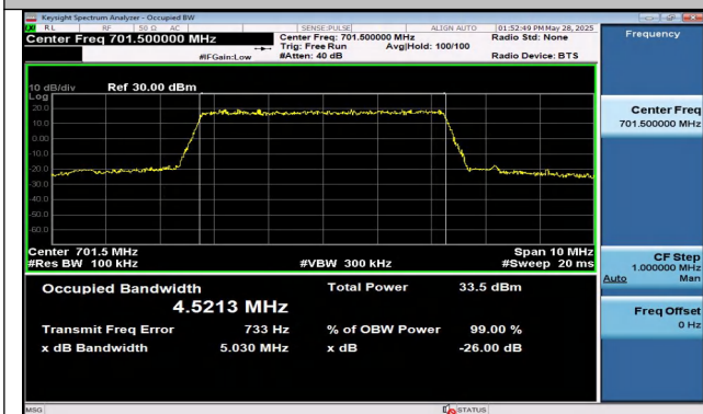
Band12-5MHz-QPSK-23035-25RB#0-PASS
