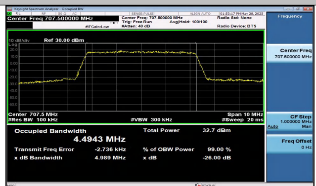
Band12-5MHz-16QAM-23095-25RB#0-PASS
