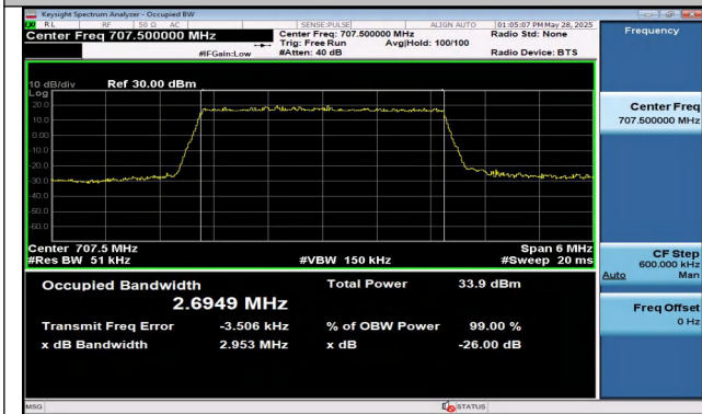
Band12-3MHz-QPSK-23095-15RB#0-PASS
