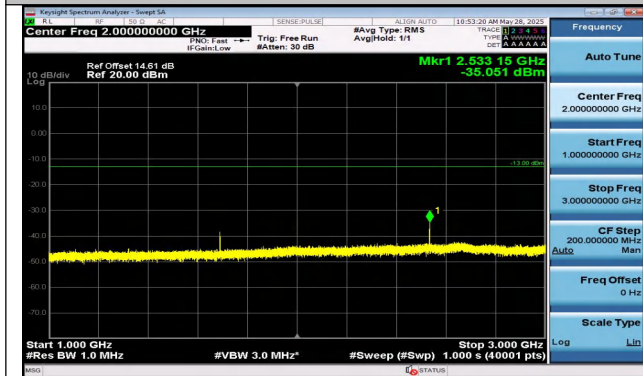
Band5-5MHz-16QAM-20625-1RB#0-1000~3000-PASS
