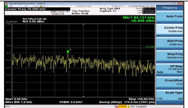
Band5-10MHz-QPSK-20450-1RB#49-0.009~0.15-PASS
