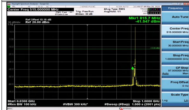
Band5-10MHz-16QAM-20450-1RB#49-30~1000-PASS
