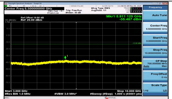
Band5-10MHz-QPSK-20525-50RB#0-3000~10000-PASS
