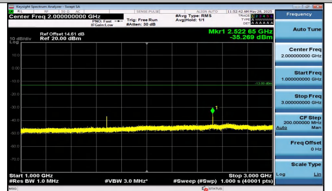
Band5-10MHz-QPSK-20525-1RB#49-1000~3000-PASS
