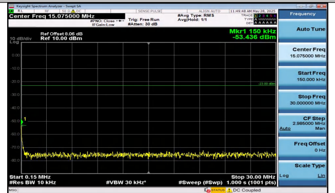
Band5-10MHz-16QAM-20450-1RB#49-0.15~30-PASS
