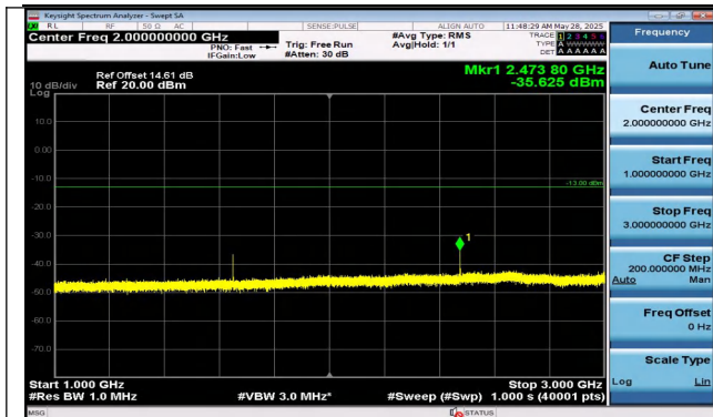
Band5-10MHz-16QAM-20450-1RB#0-1000~3000-PASS
