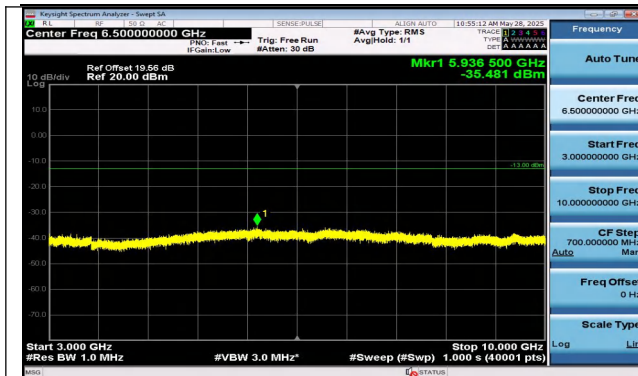
Band5-5MHz-16QAM-20625-1RB#24-3000~10000-PASS
