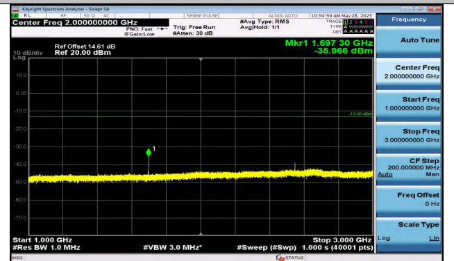
Band5-5MHz-16QAM-20625-1RB#24-1000~3000-PASS
