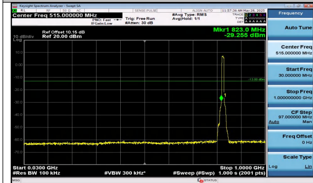
Band5-10MHz-QPSK-20450-50RB#0-30~1000-PASS
