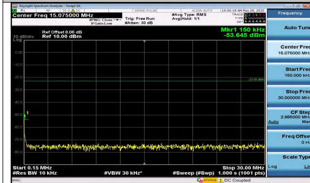
Band5-5MHz-16QAM-20625-25RB#0-0.15~30-PASS
