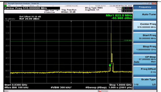
Band5-10MHz-QPSK-20525-1RB#0-30~1000-PASS
