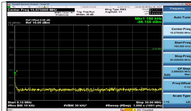
Band5-5MHz-16QAM-20625-1RB#0-0.15~30-PASS
