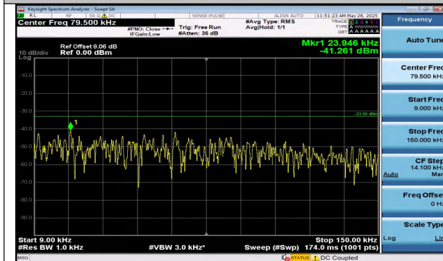
Band5-10MHz-16QAM-20525-1RB#0-0.009~0.15-PASS
