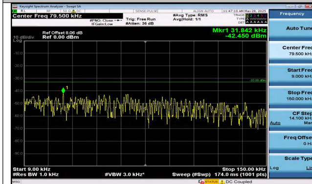
Band5-10MHz-QPSK-20450-1RB#0-0.009~0.15-PASS
