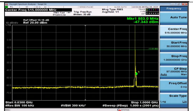
Band5-5MHz-16QAM-20625-1RB#0-30~1000-PASS
