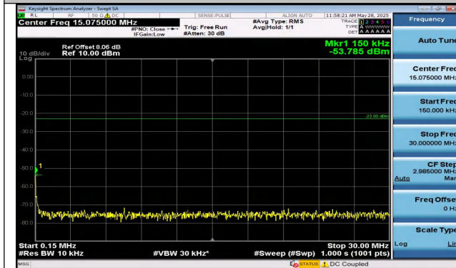
Band5-10MHz-QPSK-20525-50RB#0-0.15~30-PASS
