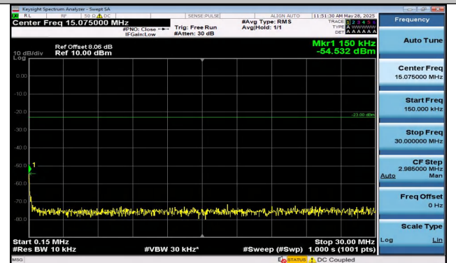
Band5-10MHz-16QAM-20525-1RB#0-0.15~30-PASS
