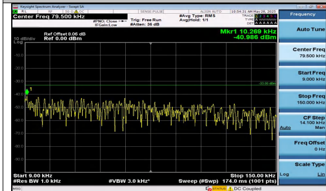
Band5-5MHz-16QAM-20625-1RB#24-0.009~0.15-PASS
