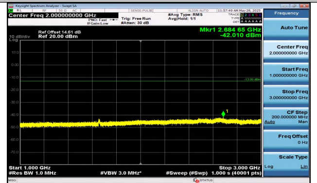
Band5-10MHz-QPSK-20450-50RB#0-1000~3000-PASS
