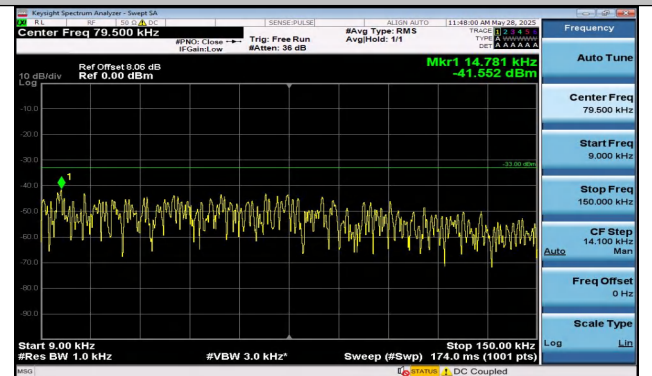
Band5-10MHz-16QAM-20450-1RB#0-0.009~0.15-PASS
