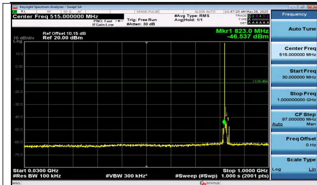
Band5-10MHz-QPSK-20450-1RB#0-30~1000-PASS
