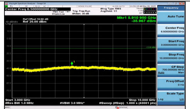
Band5-10MHz-QPSK-20525-1RB#0-3000~10000-PASS
