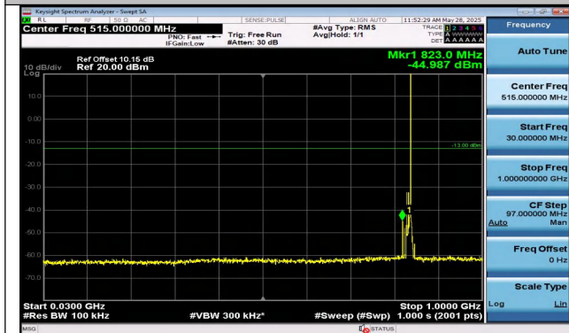
Band5-10MHz-QPSK-20525-1RB#49-30~1000-PASS
