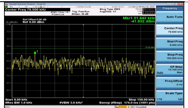
Band5-10MHz-QPSK-20525-50RB#0-0.009~0.15-PASS
