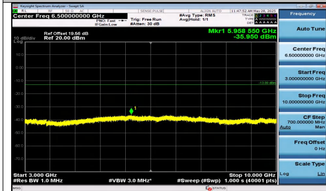
Band5-10MHz-QPSK-20450-1RB#0-3000~10000-PASS
