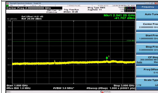
Band5-5MHz-16QAM-20625-25RB#0-1000~3000-PASS
