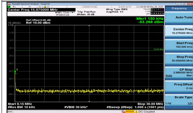
Band5-10MHz-16QAM-20450-1RB#0-0.15~30-PASS
