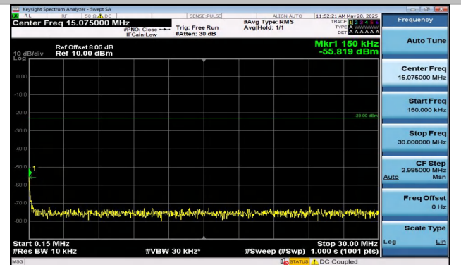
Band5-10MHz-QPSK-20525-1RB#49-0.15~30-PASS
