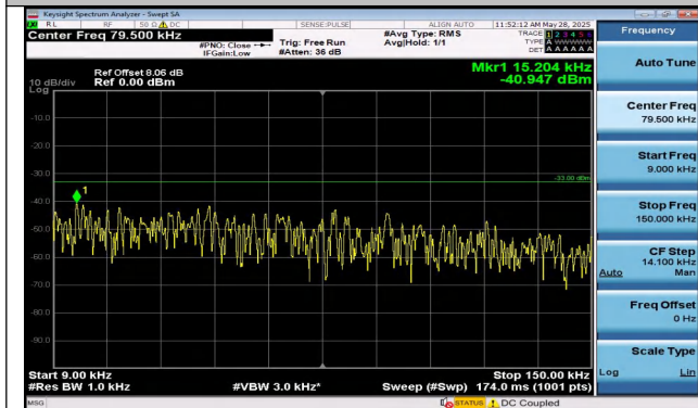
Band5-10MHz-QPSK-20525-1RB#49-0.009~0.15-PASS
