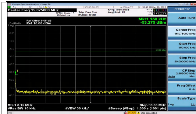
Band5-10MHz-QPSK-20525-1RB#0-0.15~30-PASS
