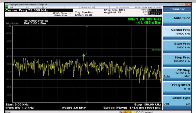
Band5-10MHz-QPSK-20525-1RB#0-0.009~0.15-PASS
