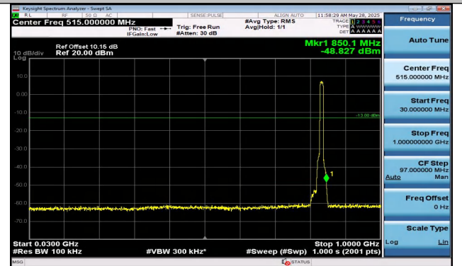
Band5-10MHz-QPSK-20525-50RB#0-0.30~1000-PASS
