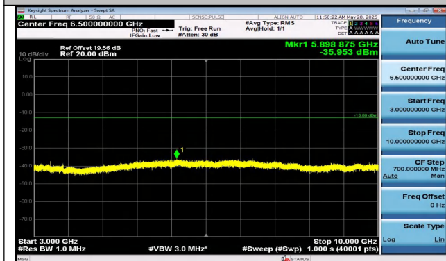
Band5-10MHz-16QAM-20450-1RB#49-3000~10000-PASS
