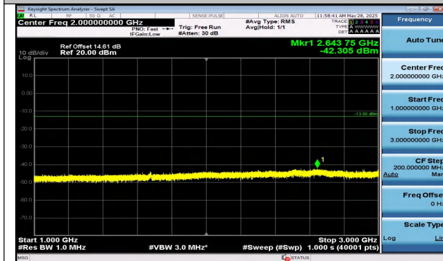
Band5-10MHz-QPSK-20525-50RB#0-1000~3000-PASS
