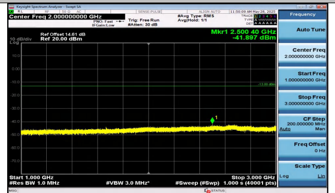
Band5-10MHz-16QAM-20450-1RB#49-1000~3000-PASS
