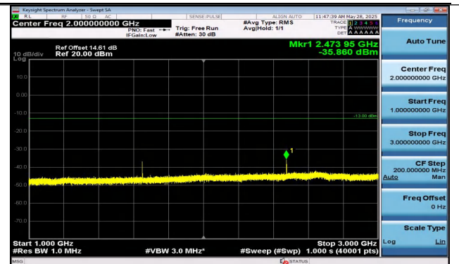
Band5-10MHz-QPSK-20450-1RB#0-1000~3000-PASS
