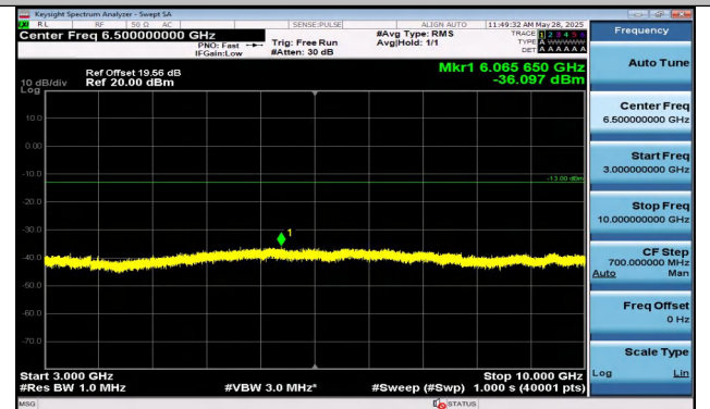
Band5-10MHz-QPSK-20450-1RB#49-3000~10000-PASS
