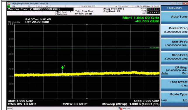
Band5-10MHz-QPSK-20525-1RB#0-1000~3000-PASS
