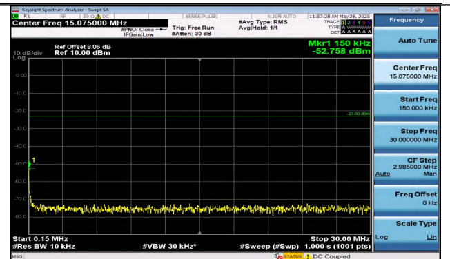
Band5-10MHz-QPSK-20450-50RB#0-0.15~30-PASS
