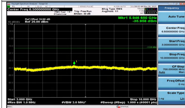
Band5-10MHz-QPSK-20450-50RB#0-3000~10000-PASS
