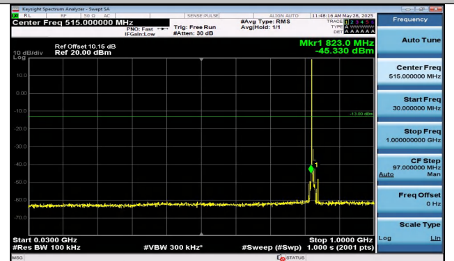
Band5-10MHz-16QAM-20450-1RB#0-30~1000-PASS
