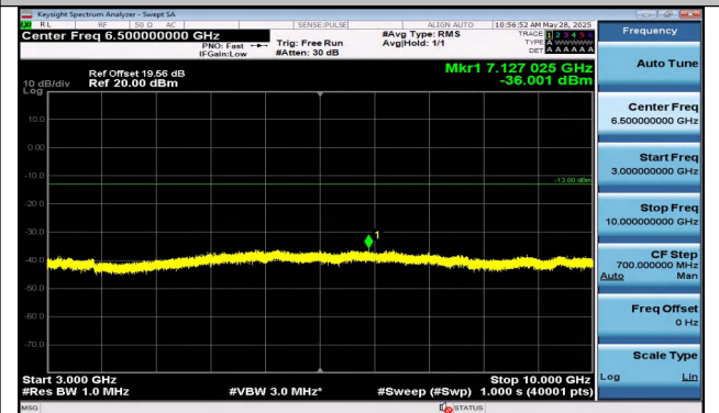
Band5-5MHz-16QAM-20625-25RB#0-3000~10000-PASS
