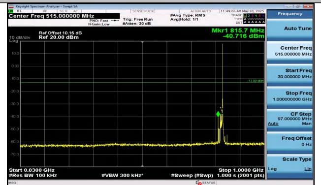
Band5-10MHz-QPSK-20450-1RB#49-30~1000-PASS
