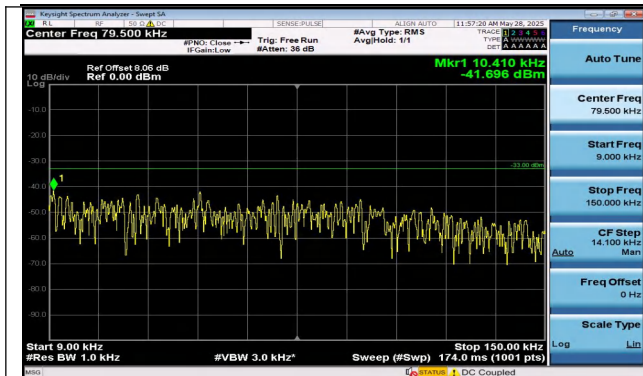
Band5-10MHz-QPSK-20450-50RB#0-0.009~0.15-PASS
