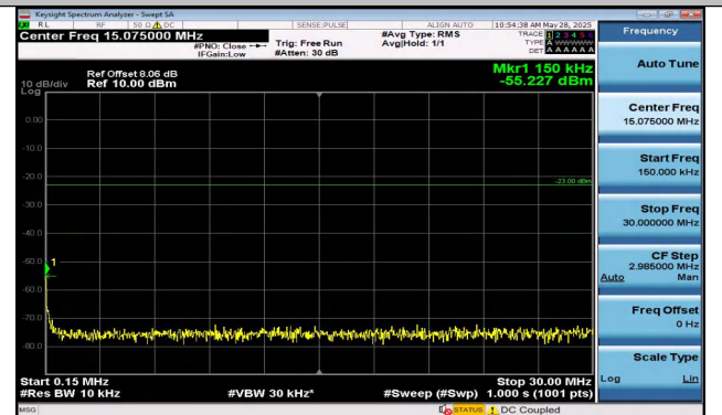
Band5-5MHz-16QAM-20625-1RB#24-0.15~30-PASS
