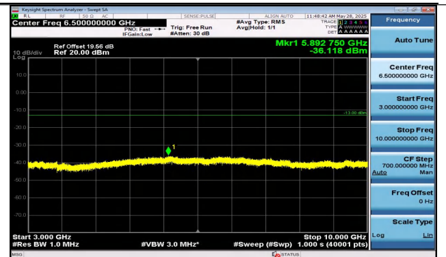
Band5-10MHz-16QAM-20450-1RB#0-3000~10000-PASS
