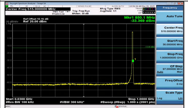
Band5-5MHz-16QAM-20625-25RB#0-30~1000-PASS
