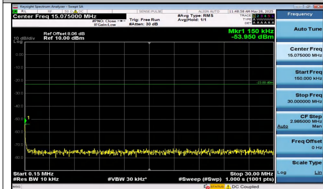
Band5-10MHz-QPSK-20450-1RB#49-0.15~30-PASS
