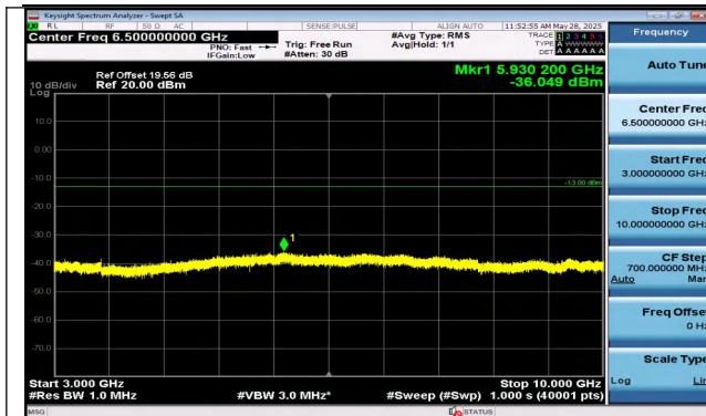
Band5-10MHz-QPSK-20525-1RB#49-3000~10000-PASS
