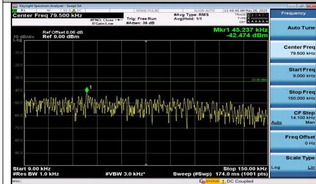
Band5-10MHz-16QAM-20450-1RB#49-0.009~0.15-PASS
