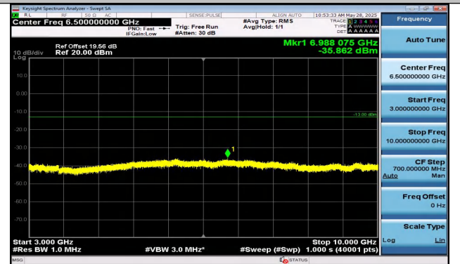
Band5-5MHz-16QAM-20625-1RB#0-3000~10000-PASS
