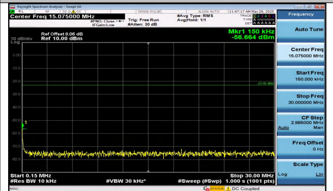
Band5-10MHz-QPSK-20450-1RB#0-0.15~30-PASS
