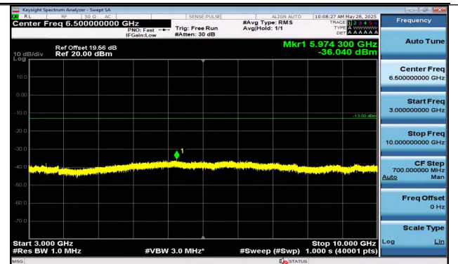
Band5-3MHz-QPSK-20525-1RB#14-3000~10000-PASS
