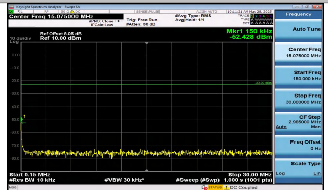
Band5-3MHz-QPSK-20635-1RB#0-0.15~30-PASS
