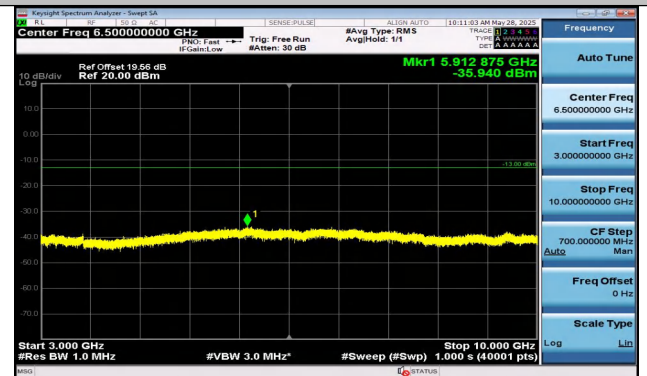
Band5-3MHz-16QAM-20525-15RB#0-3000~10000-PASS
