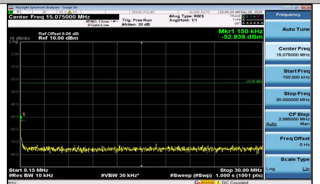
Band5-5MHz-QPSK-20425-25RB#0-0.15~30-PASS
