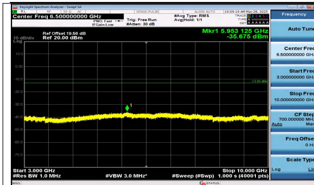
Band5-3MHz-16QAM-20525-1RB#14-3000~10000-PASS
