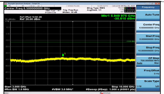
Band5-3MHz-16QAM-20635-1RB#0-3000~10000-PASS
