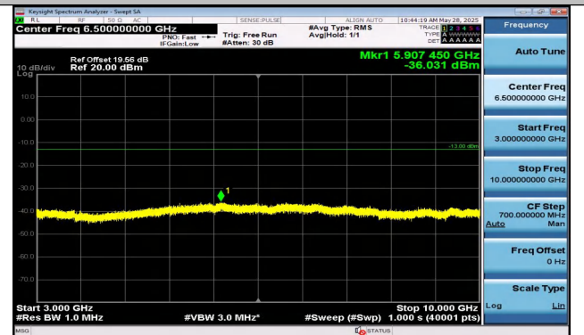
Band5-5MHz-QPSK-20425-1RB#24-3000~10000-PASS
