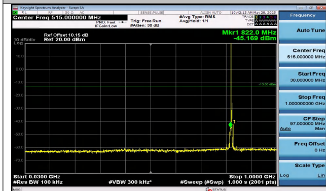
Band5-5MHz-QPSK-20425-1RB#0-30~1000-PASS
