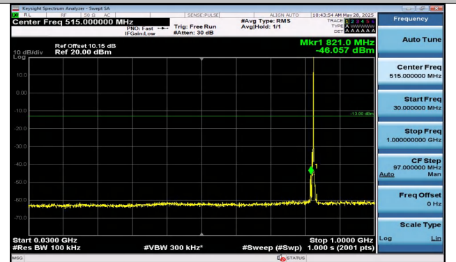
Band5-5MHz-QPSK-20425-1RB#24-30~1000-PASS
