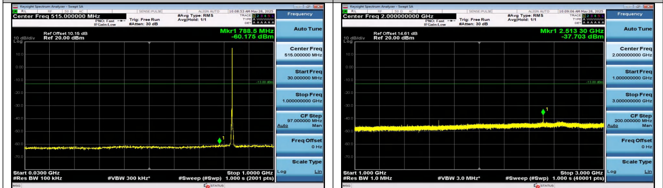
Band5-3MHz-16QAM-20525-1RB#14-30~1000-PASS
