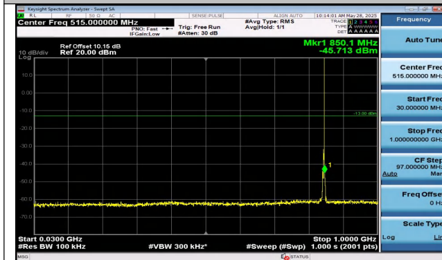
Band5-3MHz-16QAM-20635-1RB#14-30~1000-PASS
