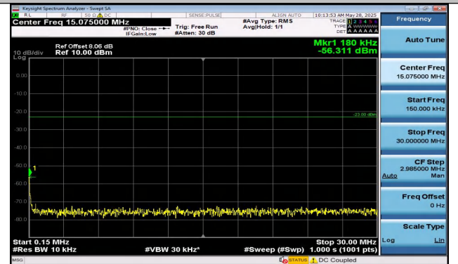
Band5-3MHz-16QAM-20635-1RB#14-0.15~30-PASS
