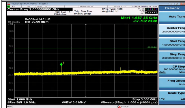
Band5-5MHz-QPSK-20425-1RB#24-1000~3000-PASS
