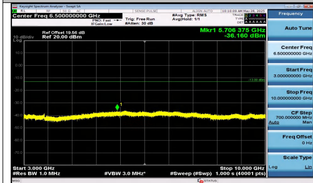
Band5-3MHz-QPSK-20525-15RB#0-3000~10000-PASS
