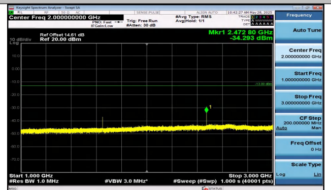
Band5-5MHz-QPSK-20425-1RB#0-1000~3000-PASS
