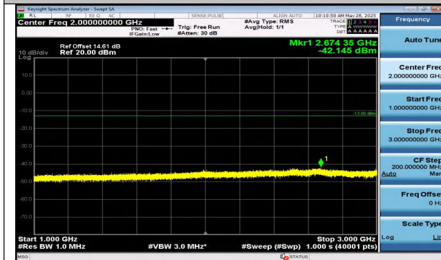
Band5-3MHz-16QAM-20525-15RB#0-1000~3000-PASS
