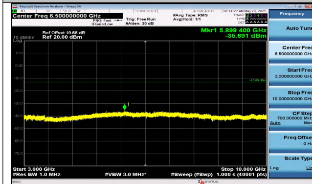
Band5-3MHz-16QAM-20635-1RB#14-3000~10000-PASS
