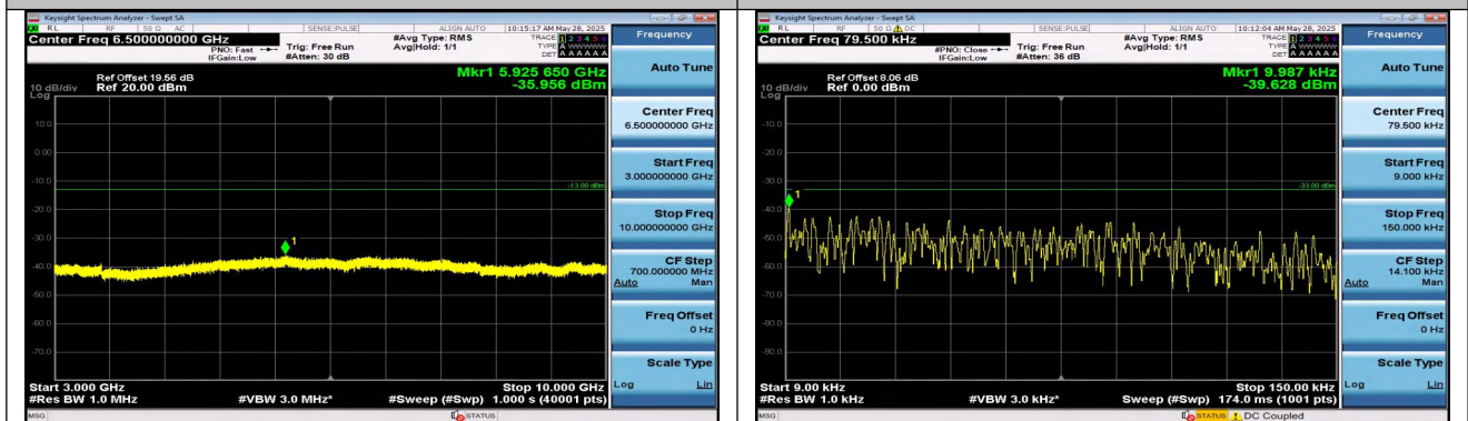
Band5-3MHz-QPSK-20635-15RB#0-3000~10000-PASS
