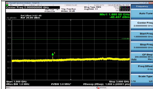
Band5-3MHz-16QAM-20635-15RB#0-1000~3000-PASS
