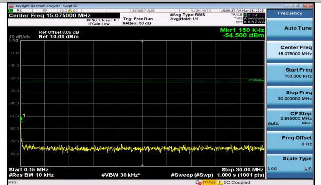
Band5-3MHz-QPSK-20525-15RB#0-0.15~30-PASS
