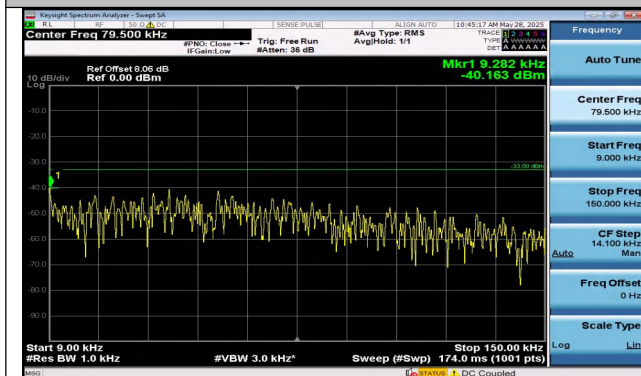
Band5-5MHz-QPSK-20425-25RB#0-0.009~0.15-PASS
