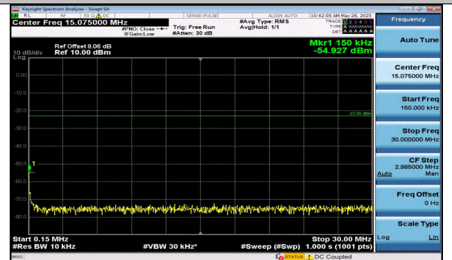
Band5-5MHz-QPSK-20425-1RB#0-0.15~30-PASS
