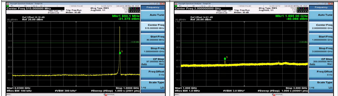
Band5-3MHz-QPSK-20635-15RB#0-30~1000-PASS
