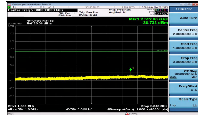
Band5-3MHz-QPSK-20525-1RB#14-1000~3000-PASS
