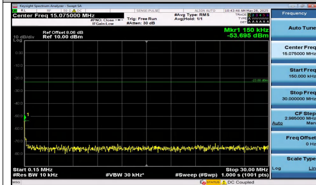
Band5-5MHz-QPSK-20425-1RB#24-0.15~30-PASS
