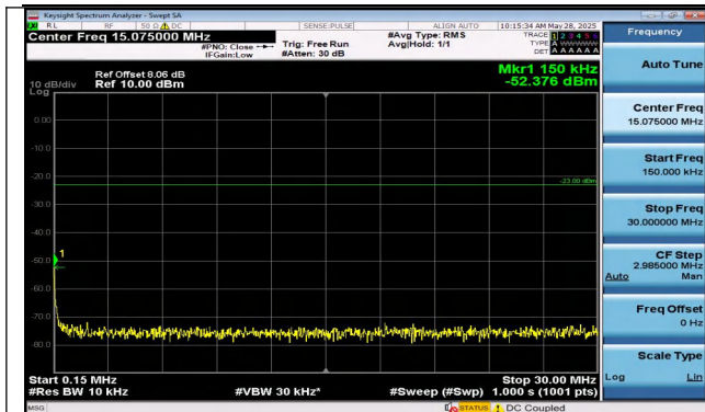
Band5-3MHz-16QAM-20635-15RB#0-0.15~30-PASS
