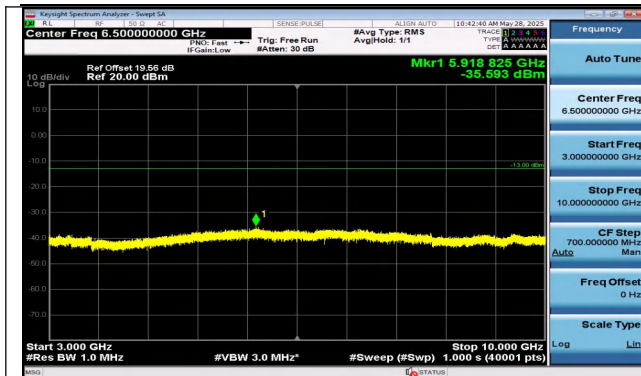
Band5-5MHz-QPSK-20425-1RB#0-3000~10000-PASS
