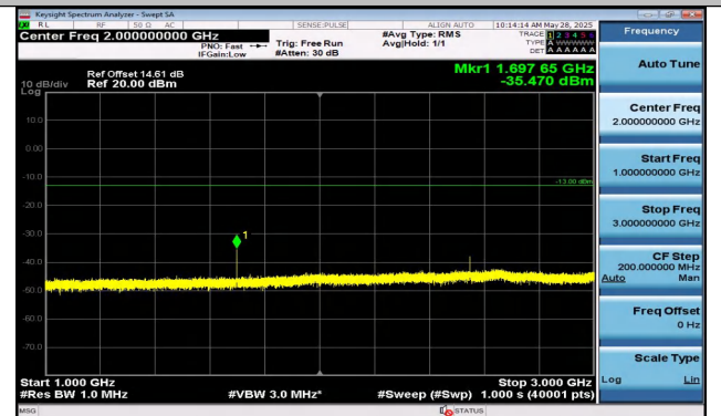
Band5-3MHz-16QAM-20635-1RB#14-1000~3000-PASS
