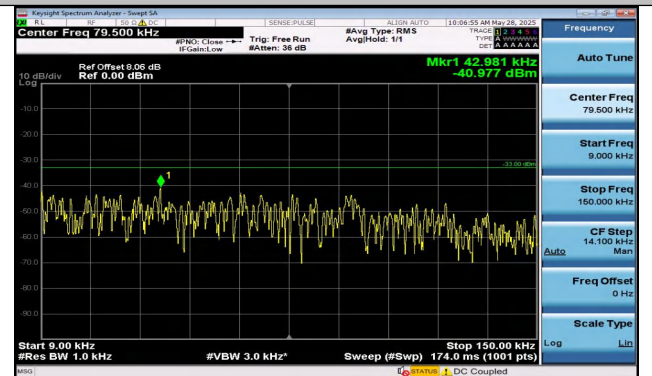
Band5-3MHz-16QAM-20525-1RB#0-0.009~0.15-PASS
