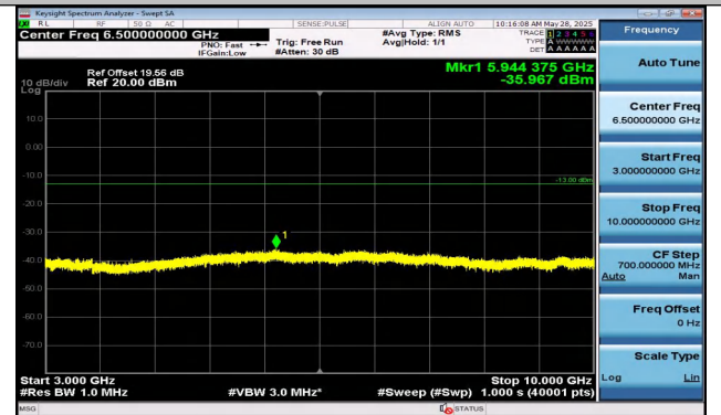
Band5-3MHz-16QAM-20635-15RB#0-3000~10000-PASS
