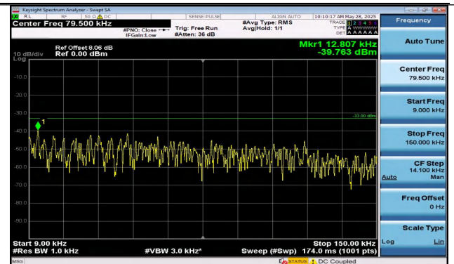
Band5-3MHz-16QAM-20525-15RB#0-0.009~0.15-PASS
