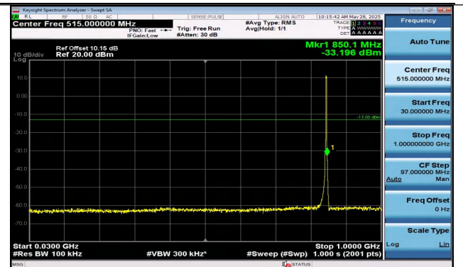
Band5-3MHz-16QAM-20635-15RB#0-30~1000-PASS
