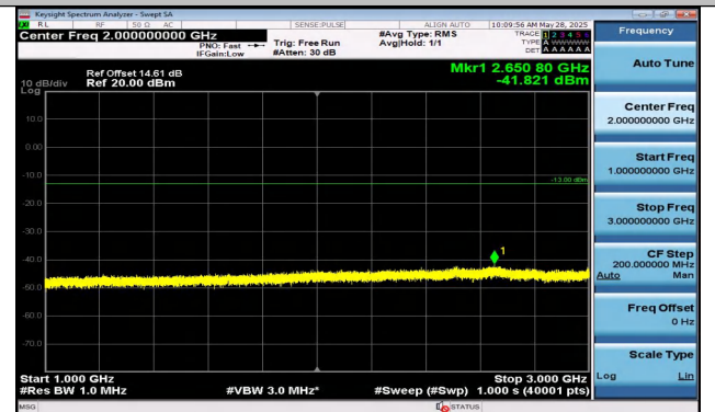
Band5-3MHz-QPSK-20525-15RB#0-1000~3000-PASS
