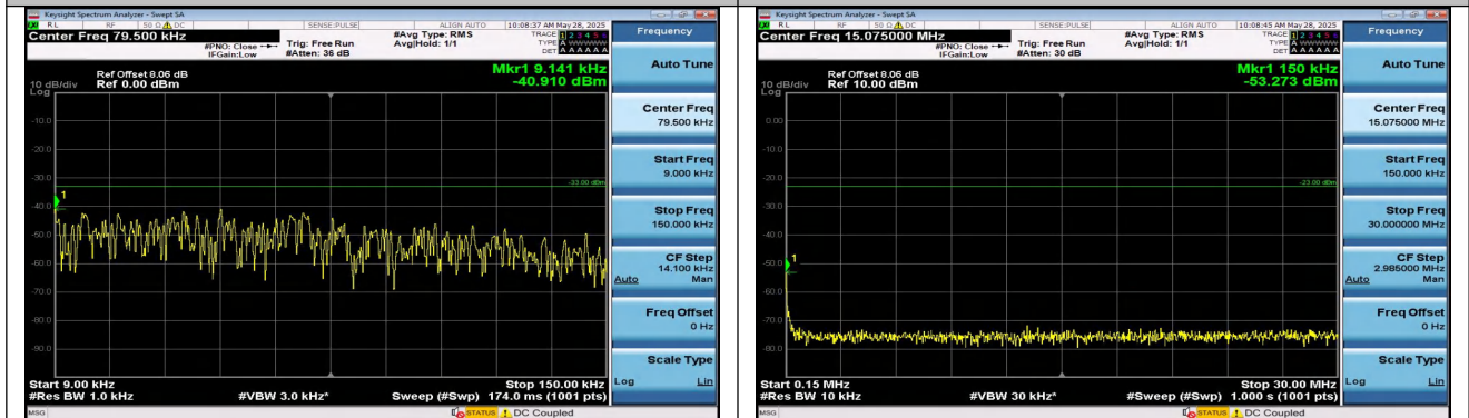
Band5-3MHz-16QAM-20525-1RB#14-0.009~0.15-PASS
