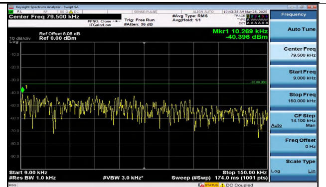
Band5-5MHz-QPSK-20425-1RB#24-0.009~0.15-PASS
