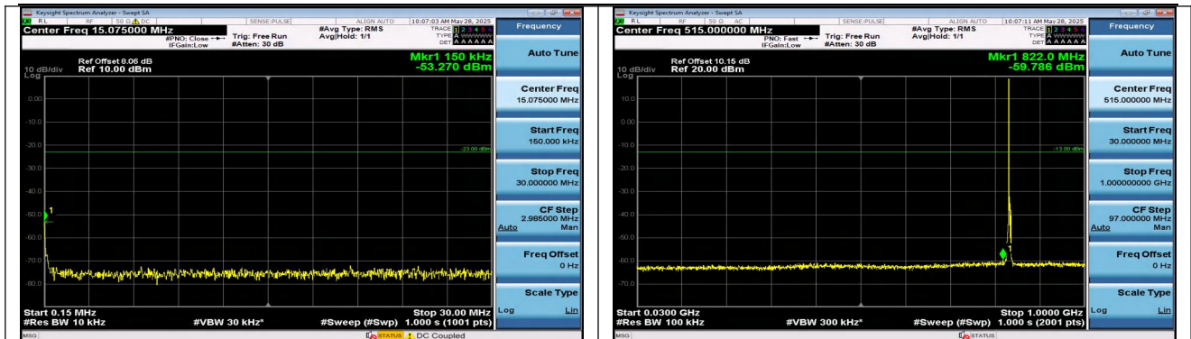
Band5-3MHz-16QAM-20525-1RB#0-0.15~30-PASS
