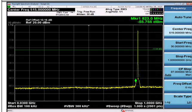
Band5-3MHz-QPSK-20525-15RB#0-0.30~1000-PASS
