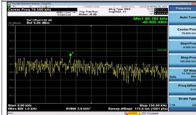
Band5-3MHz-16QAM-20635-1RB#14-0.009~0.15-PASS
