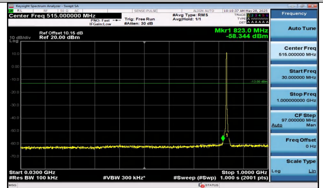
Band5-3MHz-16QAM-20525-15RB#0-30~1000-PASS
