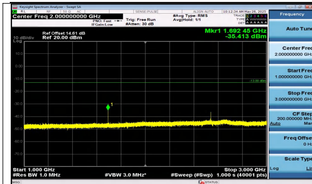
Band5-3MHz-16QAM-20635-1RB#0-1000~3000-PASS
