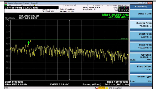
Band5-1.4MHz-16QAM-20643-6RB#0-0.009~0.15-PASS
