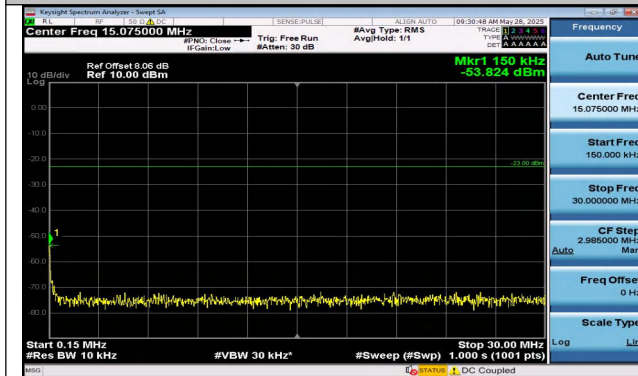
Band5-1.4MHz-QPSK-20643-1RB#5-0.15~30-PASS
