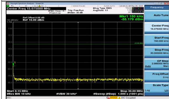
Band5-3MHz-16QAM-20415-15RB#0-0.15~30-PASS
