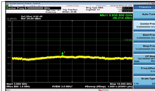
Band5-1.4MHz-QPSK-20643-1RB#0-3000~10000-PASS
