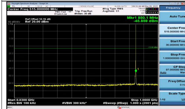
Band5-1.4MHz-16QAM-20643-1RB#5-30~1000-PASS
