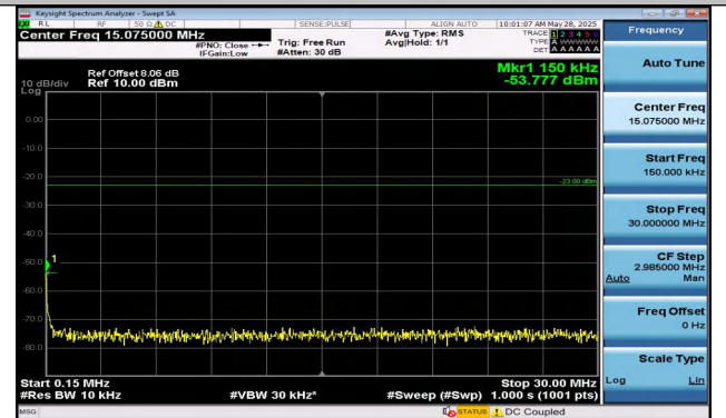
Band5-3MHz-QPSK-20415-1RB#0-0.15~30-PASS
