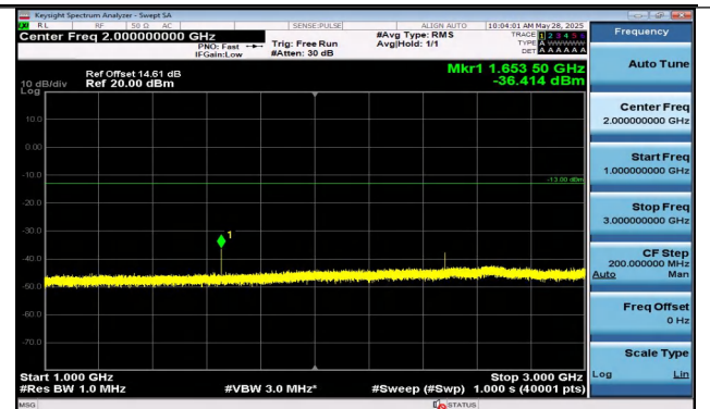
Band5-3MHz-16QAM-20415-1RB#14-1000~3000-PASS
