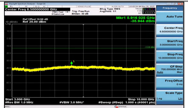
Band5-3MHz-16QAM-20415-15RB#0-3000~10000-PASS
