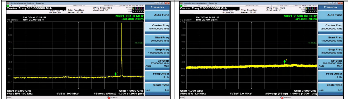
Band5-3MHz-QPSK-20525-1RB#0-30~1000-PASS
