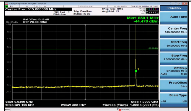
Band5-1.4MHz-QPSK-20643-1RB#5-30~1000-PASS
