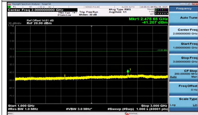
Band5-3MHz-16QAM-20415-15RB#0-1000~3000-PASS
