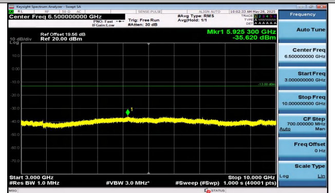
Band5-3MHz-16QAM-20415-1RB#0-3000~10000-PASS
