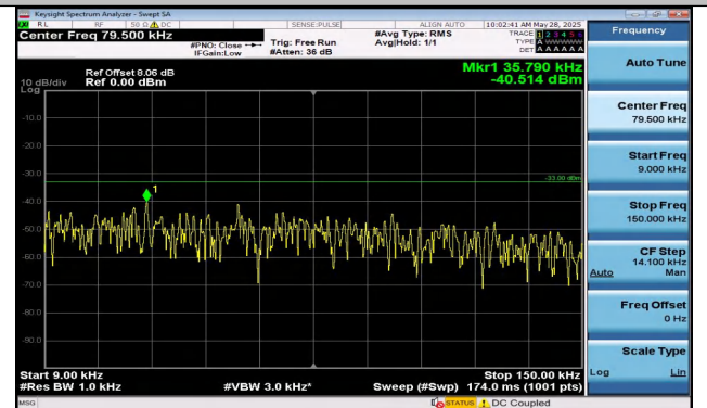
Band5-3MHz-QPSK-20415-1RB#14-0.009~0.15-PASS
