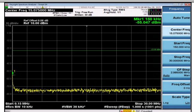
Band5-1.4MHz-QPSK-20643-6RB#0-0.15~30-PASS
