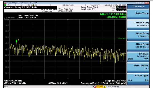
Band5-3MHz-16QAM-20415-15RB#0-0.009~0.15-PASS
