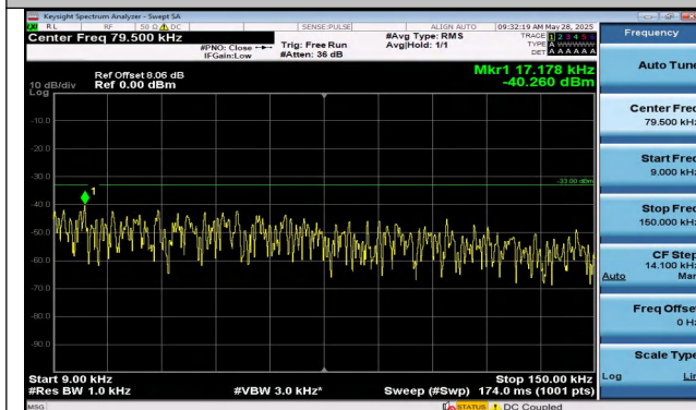
Band5-1.4MHz-QPSK-20643-6RB#0-0.009~0.15-PASS
