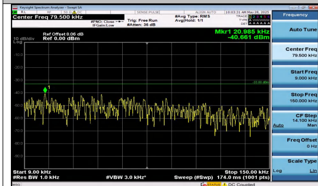
Band5-3MHz-16QAM-20415-1RB#14-0.009~0.15-PASS
