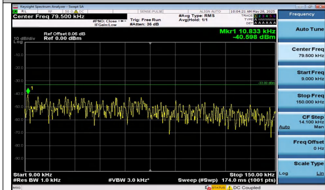
Band5-3MHz-QPSK-20415-15RB#0-0.009~0.15-PASS
