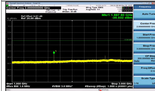
Band5-1.4MHz-QPSK-20643-1RB#5-1000~3000-PASS
