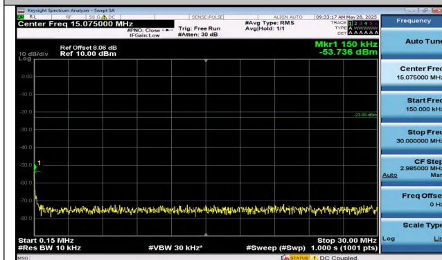
Band5-1.4MHz-16QAM-20643-6RB#0-0.15~30-PASS
