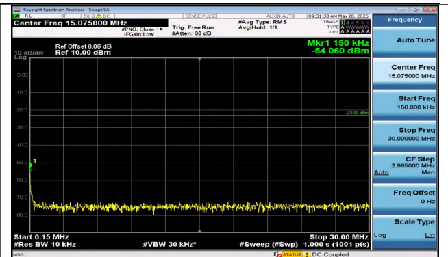
Band5-1.4MHz-16QAM-20643-1RB#5-0.15~30-PASS
