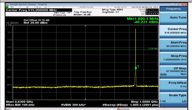
Band5-1.4MHz-16QAM-20643-6RB#0-30~1000-PASS
