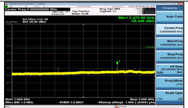
Band5-3MHz-QPSK-20415-1RB#0-1000~3000-PASS
