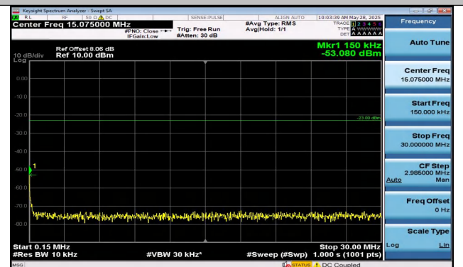
Band5-3MHz-16QAM-20415-1RB#14-0.15~30-PASS
