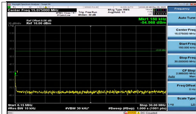
Band5-3MHz-QPSK-20415-1RB#14-0.15~30-PASS
