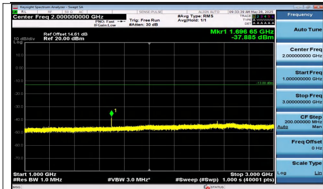
Band5-1.4MHz-16QAM-20643-6RB#0-1000~3000-PASS
