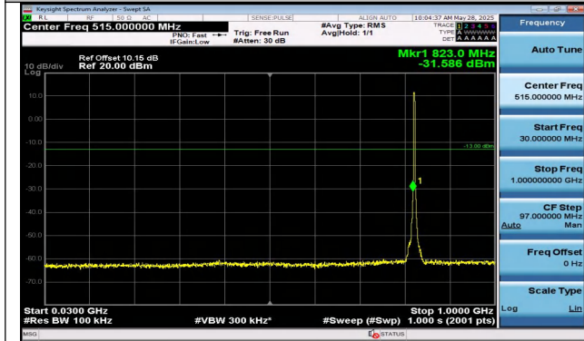
Band5-3MHz-QPSK-20415-15RB#0-30~1000-PASS
