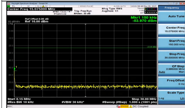
Band5-3MHz-16QAM-20415-1RB#0-0.15~30-PASS
