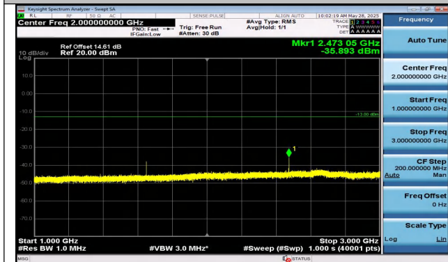
Band5-3MHz-16QAM-20415-1RB#0-1000~3000-PASS
