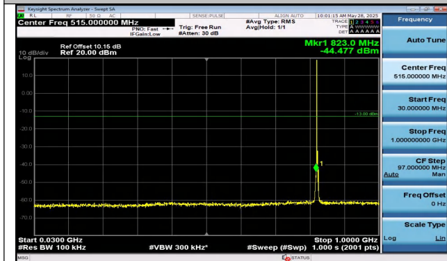
Band5-3MHz-QPSK-20415-1RB#0-30~1000-PASS
