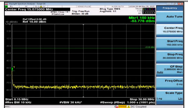
Band5-3MHz-QPSK-20415-15RB#0-0.15~30-PASS
