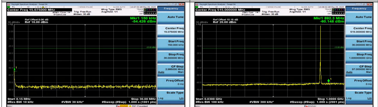
Band5-3MHz-QPSK-20525-1RB#14-0.15~30-PASS
