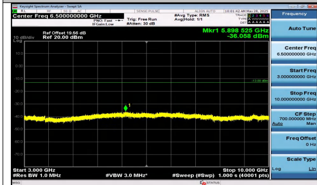
Band5-3MHz-QPSK-20415-1RB#0-3000~10000-PASS
