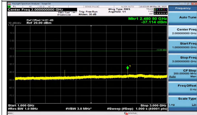
Band5-3MHz-QPSK-20415-1RB#14-1000~3000-PASS
