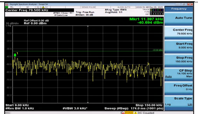
Band5-3MHz-16QAM-20415-1RB#0-0.009~0.15-PASS
