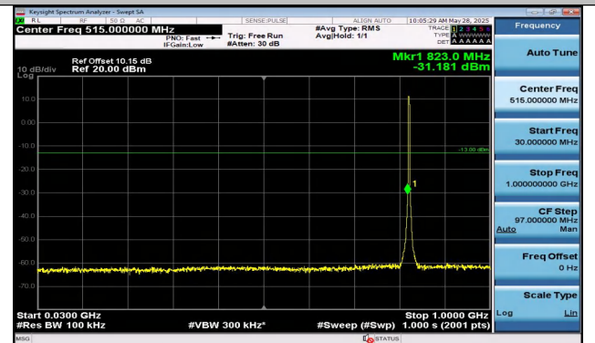
Band5-3MHz-16QAM-20415-15RB#0-30~1000-PASS
