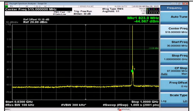
Band5-3MHz-16QAM-20415-1RB#0-30~1000-PASS
