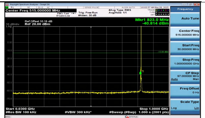
Band5-3MHz-QPSK-20415-1RB#14-30~1000-PASS
