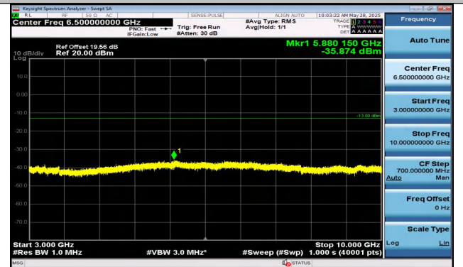
Band5-3MHz-QPSK-20415-1RB#14-3000~10000-PASS
