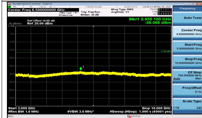
Band5-3MHz-16QAM-20415-1RB#14-3000~10000-PASS
