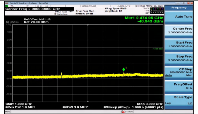
Band5-3MHz-QPSK-20415-15RB#0-1000~3000-PASS
