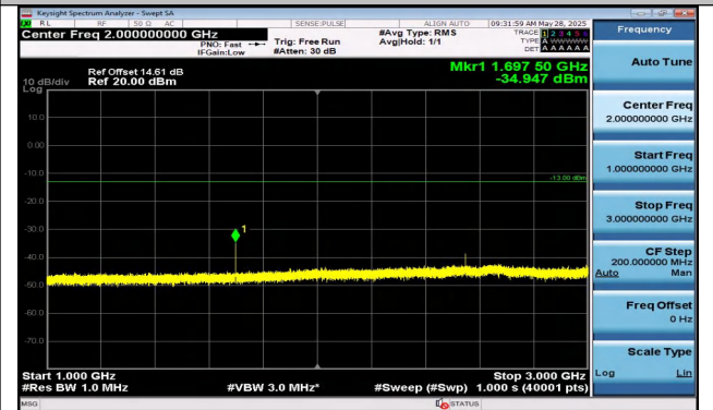
Band5-1.4MHz-16QAM-20643-1RB#5-1000~3000-PASS
