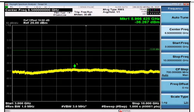
Band5-1.4MHz-16QAM-20643-6RB#0-3000~10000-PASS
