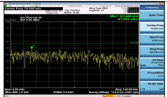
Band5-1.4MHz-QPSK-20643-1RB#5-0.009~0.15-PASS
