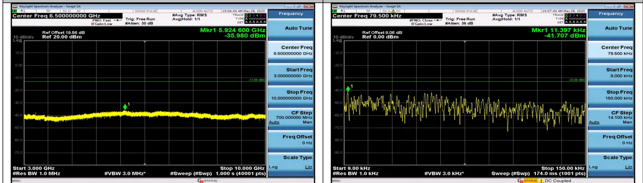
Band5-3MHz-QPSK-20525-1RB#0-3000~10000-PASS
