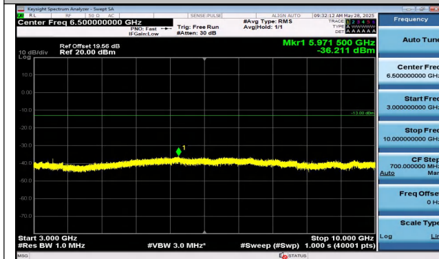
Band5-1.4MHz-16QAM-20643-1RB#5-3000~10000-PASS
