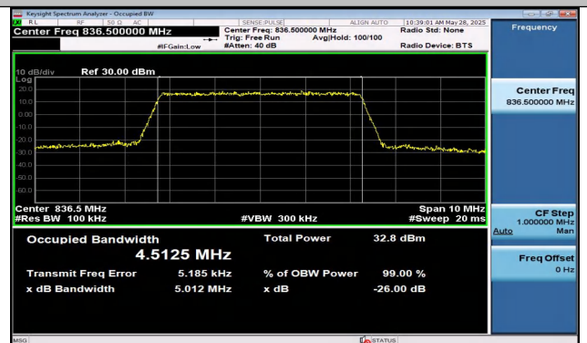
Band5-5MHz-16QAM-20525-25RB#0-PASS
