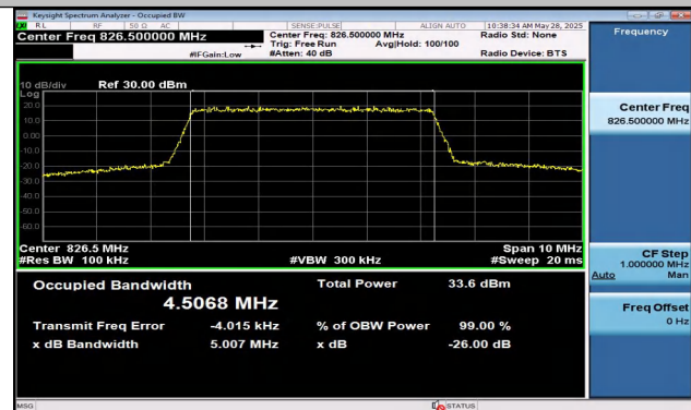
Band5-5MHz-QPSK-20425-25RB#0-PASS
