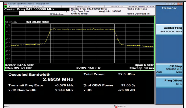
Band5-3MHz-16QAM-20635-15RB#0-PASS
