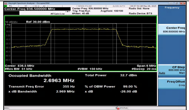
Band5-3MHz-16QAM-20525-15RB#0-PASS
