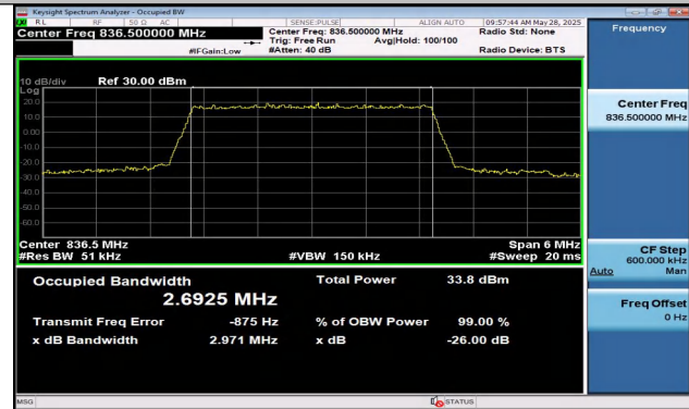
Band5-3MHz-QPSK-20525-15RB#0-PASS
