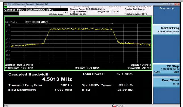
Band5-5MHz-16QAM-20425-25RB#0-PASS
