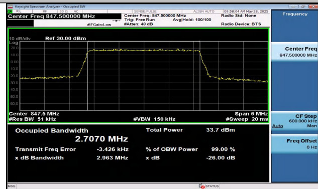
Band5-3MHz-QPSK-20635-15RB#0-PASS
