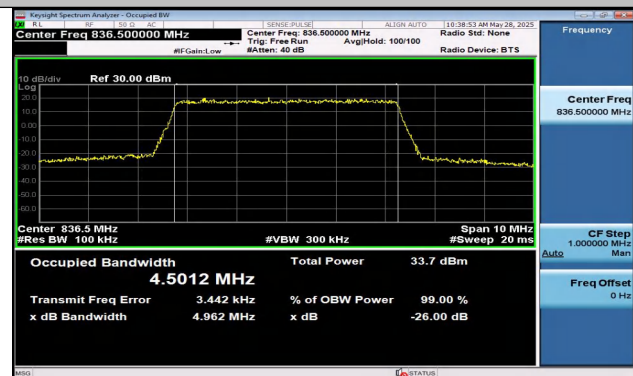
Band5-5MHz-QPSK-20525-25RB#0-PASS
