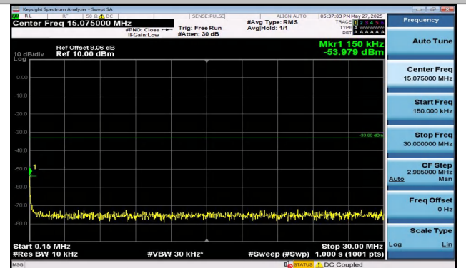
Band4-20MHz-16QAM-20050-1RB#99-0.15~30-PASS
