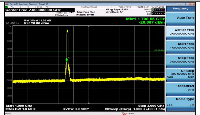
Band4-20MHz-QPSK-20050-100RB#0-1000~3000-PASS
