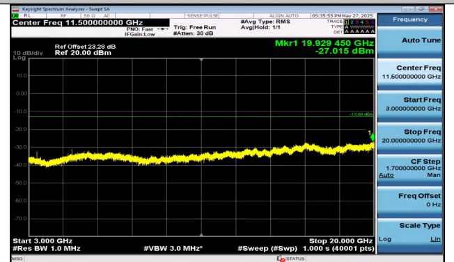
Band4-20MHz-16QAM-20050-1RB#0-3000~20000-PASS
