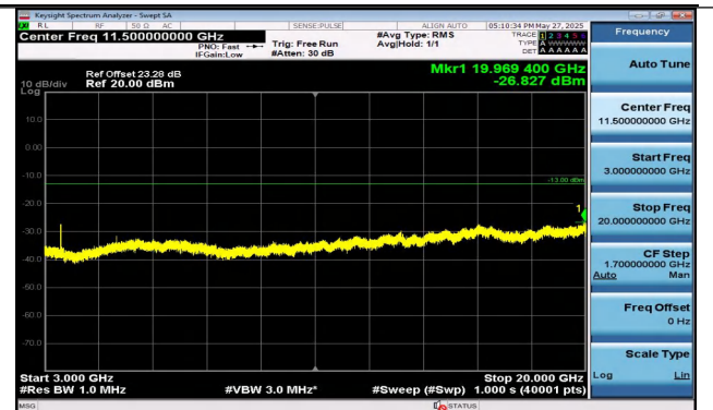
Band4-15MHz-16QAM-20325-1RB#74-3000~20000-PASS
