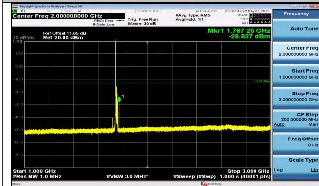
Band4-15MHz-QPSK-20325-1RB#0-1000~3000-PASS
