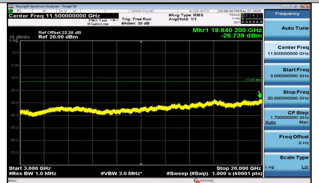
Band4-15MHz-QPSK-20325-1RB#0-3000~20000-PASS
