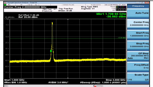
Band4-15MHz-QPSK-20175-75RB#0-1000~3000-PASS
