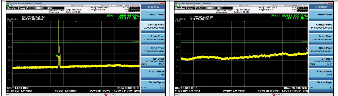
Band4-15MHz-16QAM-20175-1RB#0-1000~3000-PASS
