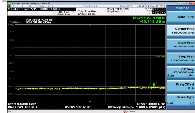
Band4-15MHz-QPSK-20175-75RB#0-30~1000-PASS
