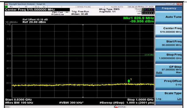
Band4-20MHz-QPSK-20050-1RB#99-30~1000-PASS
