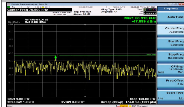
Band4-15MHz-QPSK-20325-1RB#74-0.009~0.15-PASS
