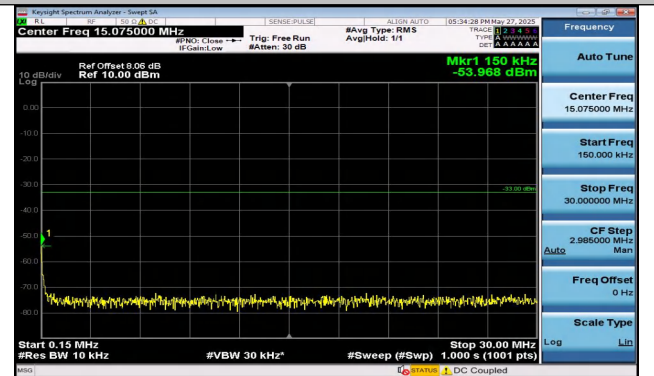
Band4-20MHz-QPSK-20050-1RB#0-0.15~30-PASS
