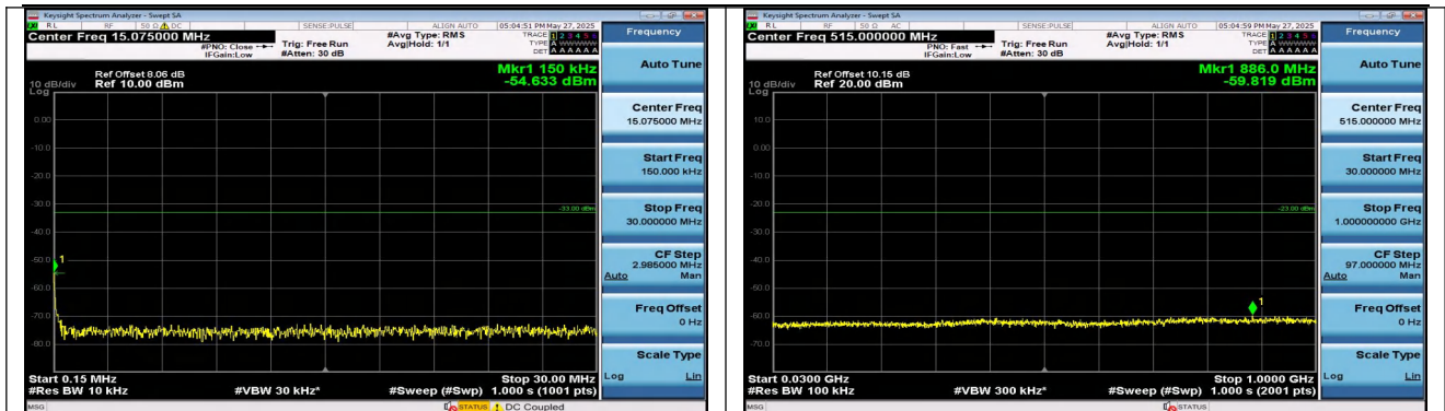
Band4-15MHz-16QAM-20175-1RB#0-0.15~30-PASS
