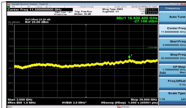
Band4-20MHz-QPSK-20050-100RB#0-3000~20000-PASS
