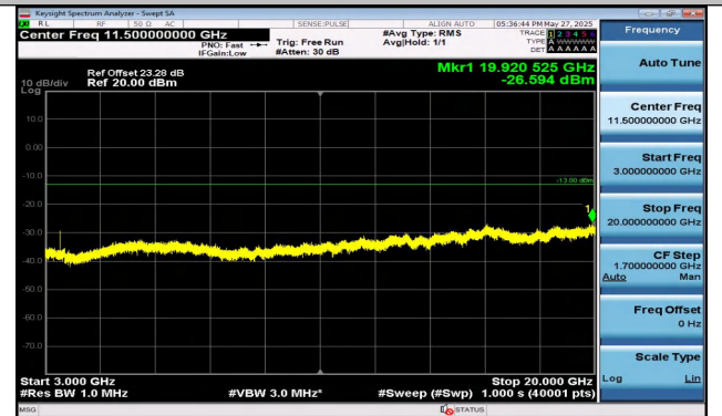
Band4-20MHz-QPSK-20050-1RB#99-3000~20000-PASS
