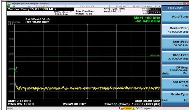
Band4-15MHz-QPSK-20325-1RB#0-0.15~30-PASS
