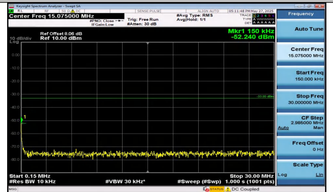
Band4-15MHz-QPSK-20175-75RB#0-0.15~30-PASS
