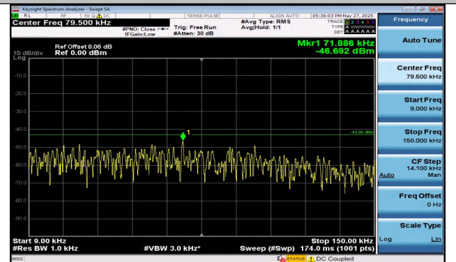
Band4-20MHz-QPSK-20050-1RB#99-0.009~0.15-PASS
