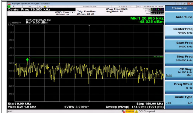
Band4-15MHz-QPSK-20175-75RB#0-0.009~0.15-PASS
