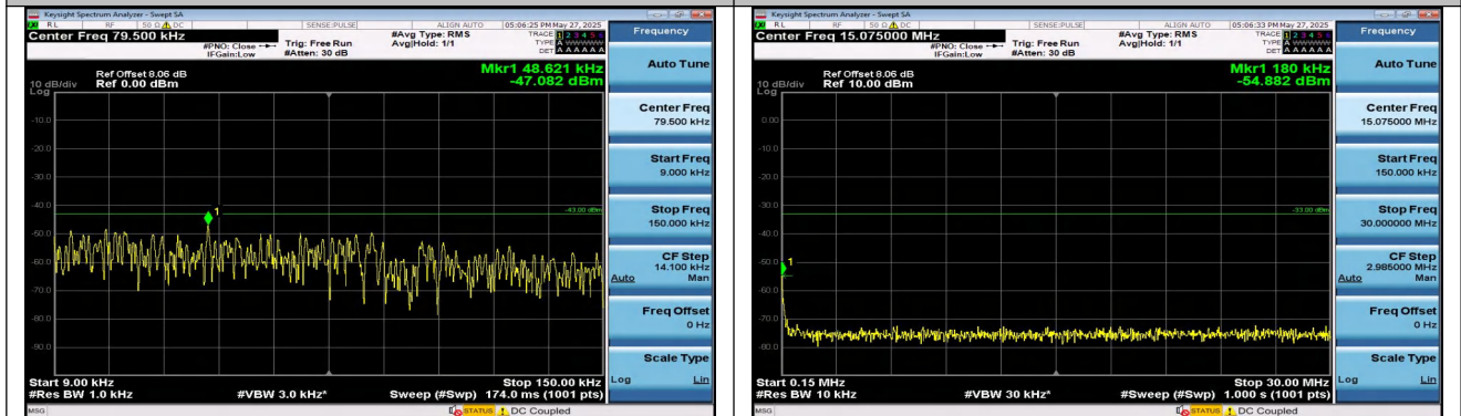
Band4-15MHz-16QAM-20175-1RB#74-0.009~0.15-PASS
