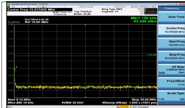
Band4-20MHz-QPSK-20050-1RB#99-0.15~30-PASS
