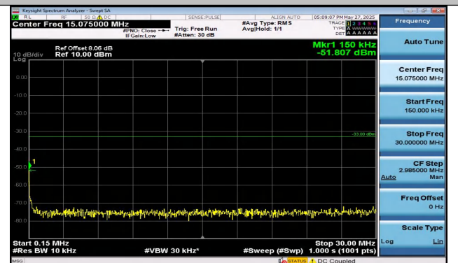
Band4-15MHz-QPSK-20325-1RB#74-0.15~30-PASS
