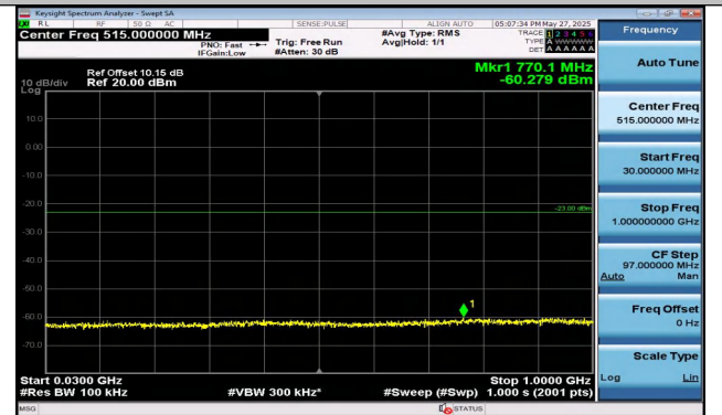
Band4-15MHz-QPSK-20325-1RB#0-30~1000-PASS
