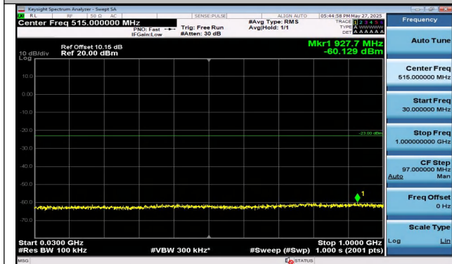
Band4-20MHz-QPSK-20050-100RB#0-30~1000-PASS
