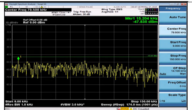
Band4-15MHz-QPSK-20325-1RB#0-0.009~0.15-PASS
