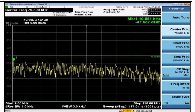
Band4-20MHz-16QAM-20050-1RB#0-0.009~0.15-PASS
