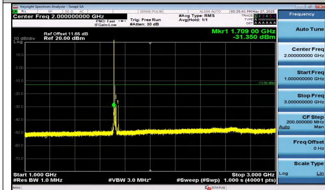
Band4-20MHz-16QAM-20050-1RB#0-1000~3000-PASS
