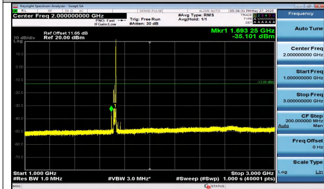
Band4-20MHz-QPSK-20050-1RB#99-1000~3000-PASS
