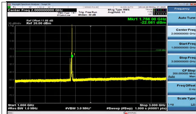
Band4-15MHz-16QAM-20325-1RB#74-1000~3000-PASS
