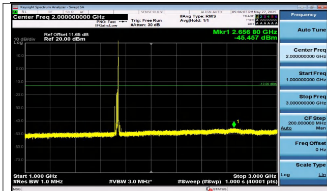
Band4-15MHz-QPSK-20175-1RB#74-1000~3000-PASS
