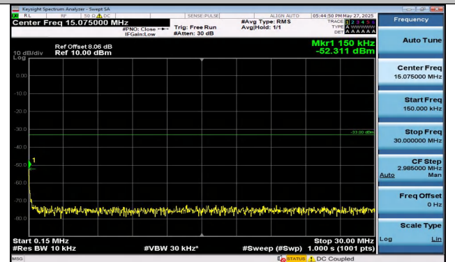
Band4-20MHz-QPSK-20050-100RB#0-0.15~30-PASS
