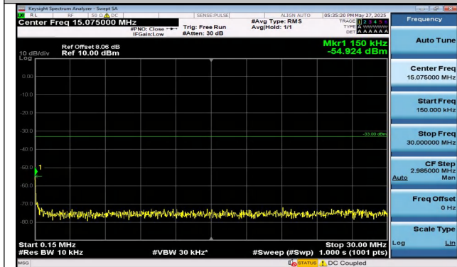
Band4-20MHz-16QAM-20050-1RB#0-0.15~30-PASS
