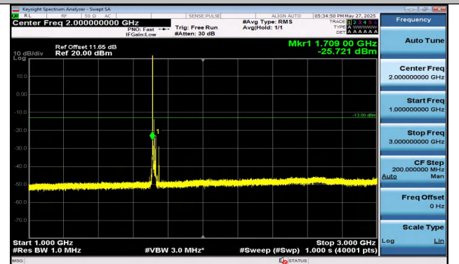
Band4-20MHz-QPSK-20050-1RB#0-1000~3000-PASS
