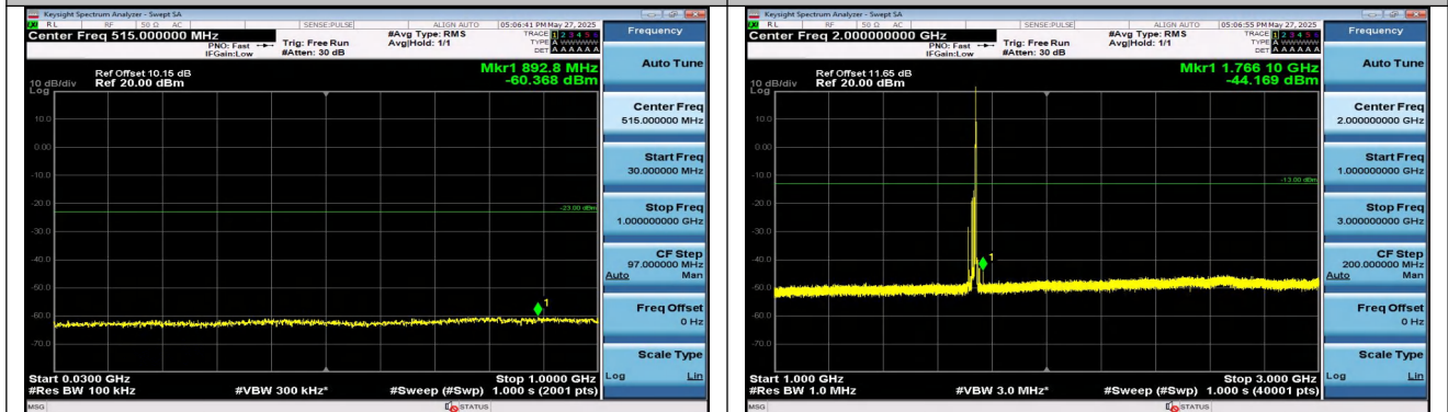
Band4-15MHz-16QAM-20175-1RB#74-30~1000-PASS
