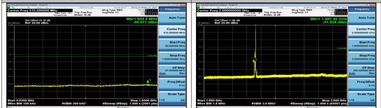
Band4-15MHz-QPSK-2025-1RB#74-30~1000-PASS
