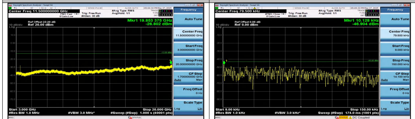
Band4-15MHz-QPSK-20175-1RB#0-3000~20000-PASS
