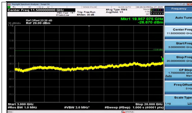
Band4-10MHz-16QAM-20175-1RB#0-3000~20000-PASS
