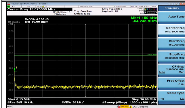
Band4-10MHz-QPSK-20350-1RB#49-0.15~30-PASS
