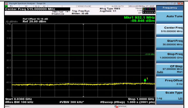
Band4-15MHz-QPSK-20025-75RB#0-30~1000-PASS
