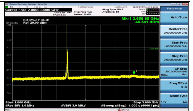
Band4-10MHz-QPSK-20350-1RB#0-1000~3000-PASS
