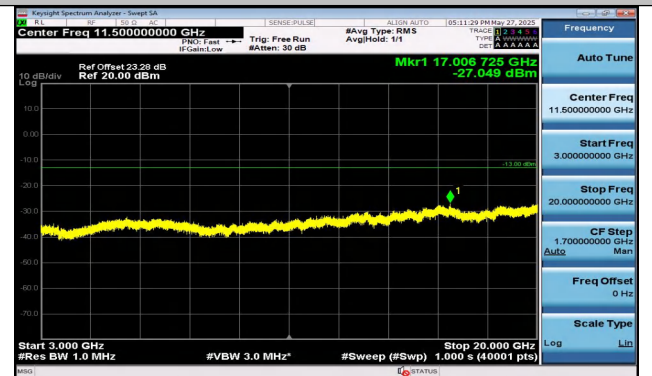
Band4-15MHz-QPSK-20025-75RB#0-3000~20000-PASS
