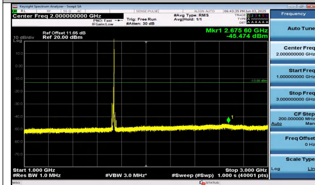
Band4-10MHz-16QAM-20175-1RB#49-1000~3000-PASS
