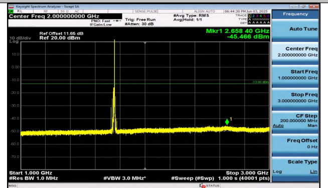
Band4-10MHz-16QAM-20350-1RB#49-1000~3000-PASS
