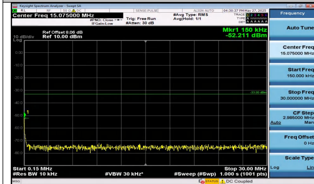
Band4-10MHz-16QAM-20175-1RB#49-0.15~30-PASS
