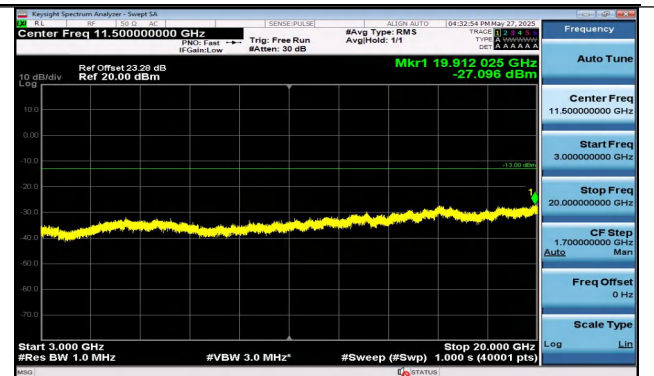
Band4-10MHz-16QAM-20350-1RB#0-3000~20000-PASS
