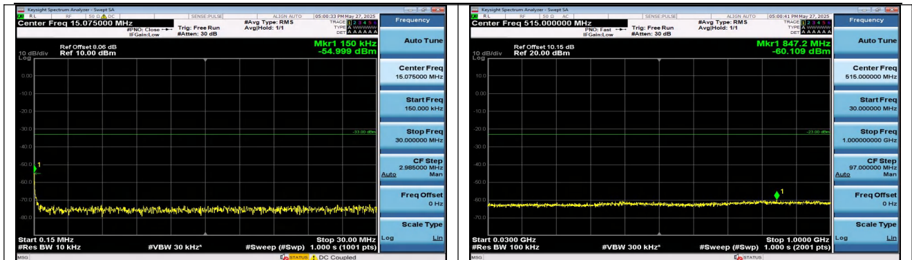
Band4-15MHz-QPSK-2025-1RB#0-0.15~30-PASS
