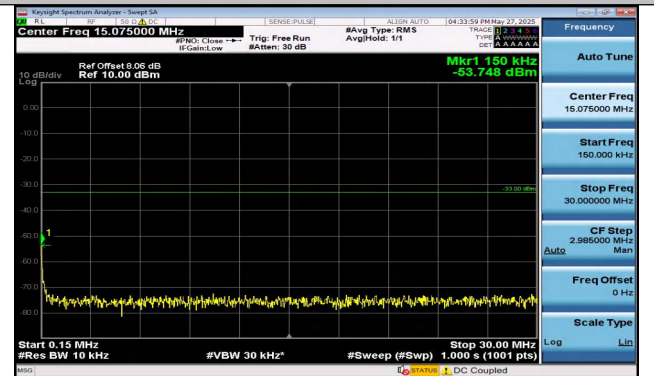
Band4-10MHz-16QAM-20350-1RB#49-0.15~30-PASS
