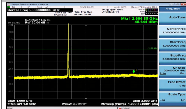
Band4-10MHz-QPSK-20350-1RB#49-1000~3000-PASS
