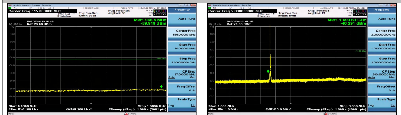
Band4-15MHz-QPSK-20175-1RB#0-30~1000-PASS
