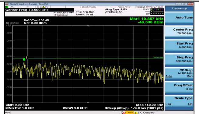
Band4-15MHz-QPSK-20025-1RB#0-0.009~0.15-PASS
