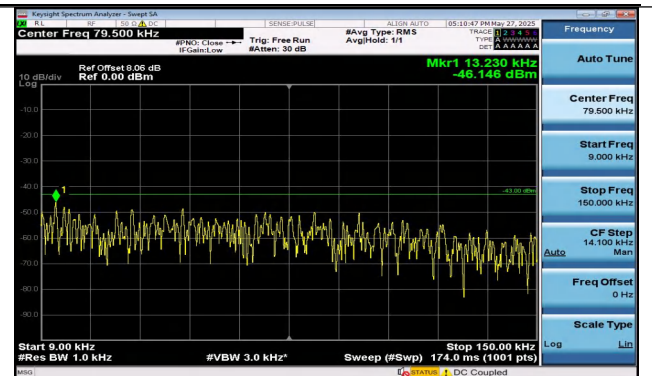
Band4-15MHz-QPSK-20025-75RB#0-0.009~0.15-PASS
