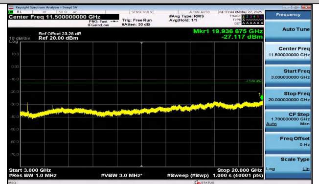
Band4-10MHz-QPSK-20350-1RB#49-3000~20000-PASS
