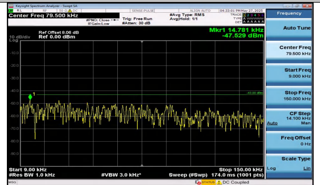
Band4-10MHz-QPSK-20350-1RB#49-0.009~0.15-PASS
