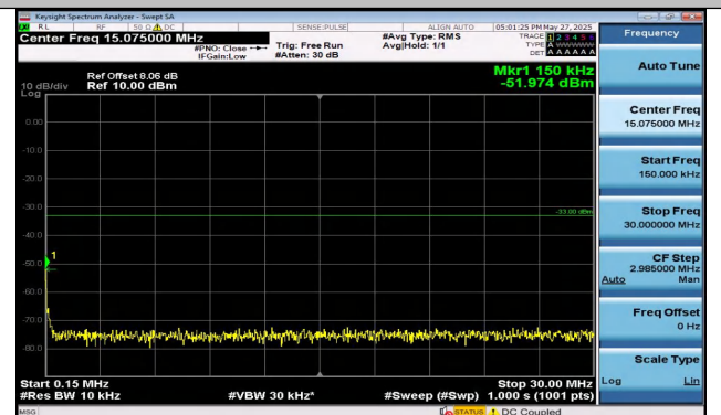
Band4-15MHz-16QAM-20025-1RB#0-0.15~30-PASS
