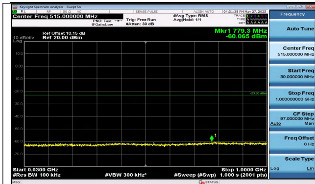
Band4-10MHz-QPSK-20350-1RB#0-30~1000-PASS
