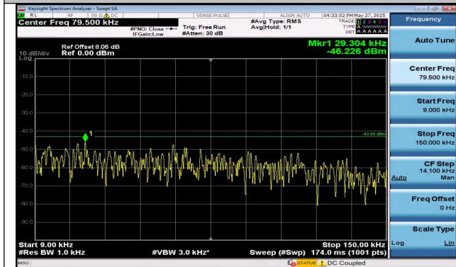
Band4-10MHz-16QAM-20350-1RB#49-0.009~0.15-PASS
