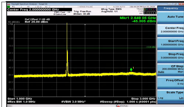
Band4-10MHz-16QAM-20350-1RB#0-1000~3000-PASS
