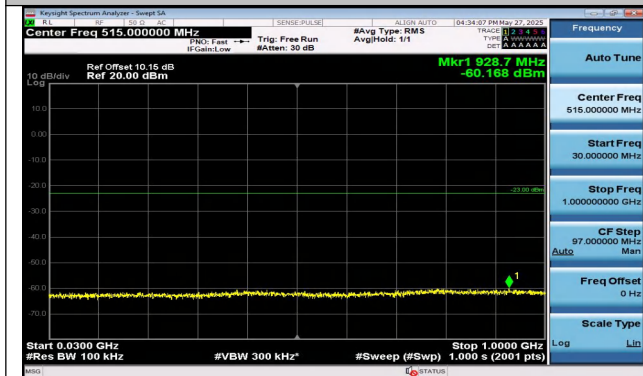
Band4-10MHz-16QAM-20350-1RB#49-30~1000-PASS
