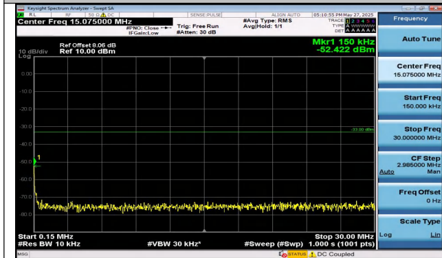
Band4-15MHz-QPSK-20025-75RB#0-0.15~30-PASS
