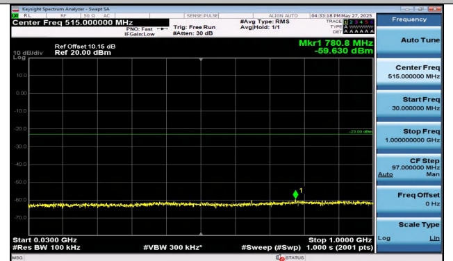
Band4-10MHz-QPSK-20350-1RB#49-30~1000-PASS
