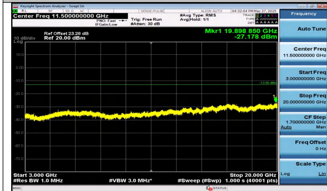
Band4-10MHz-QPSK-20350-1RB#0-3000~20000-PASS
