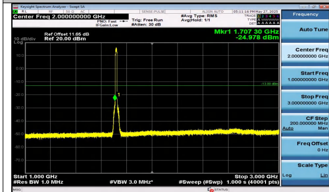
Band4-15MHz-QPSK-20025-75RB#0-1000~3000-PASS
