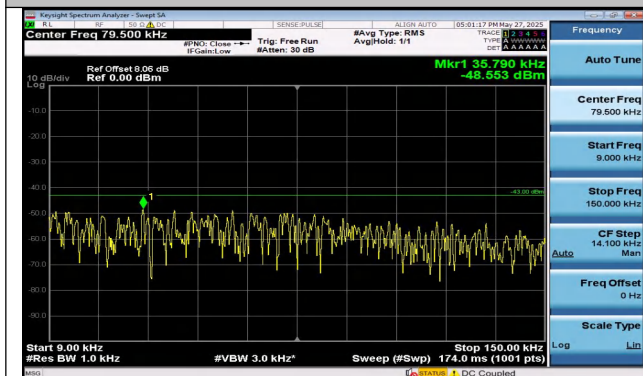
Band4-15MHz-16QAM-20025-1RB#0-0.009~0.15-PASS
