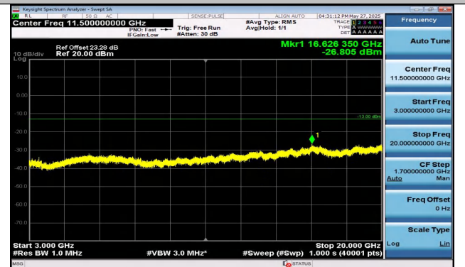
Band4-10MHz-16QAM-20175-1RB#49-3000~20000-PASS
