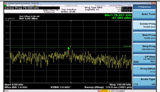
Band4-10MHz-QPSK-20175-50RB#0-0.009~0.15-PASS
