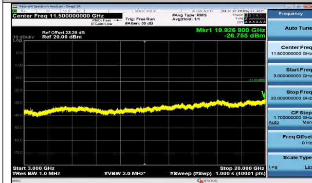
Band4-10MHz-QPSK-20175-1RB#49-3000~20000-PASS
