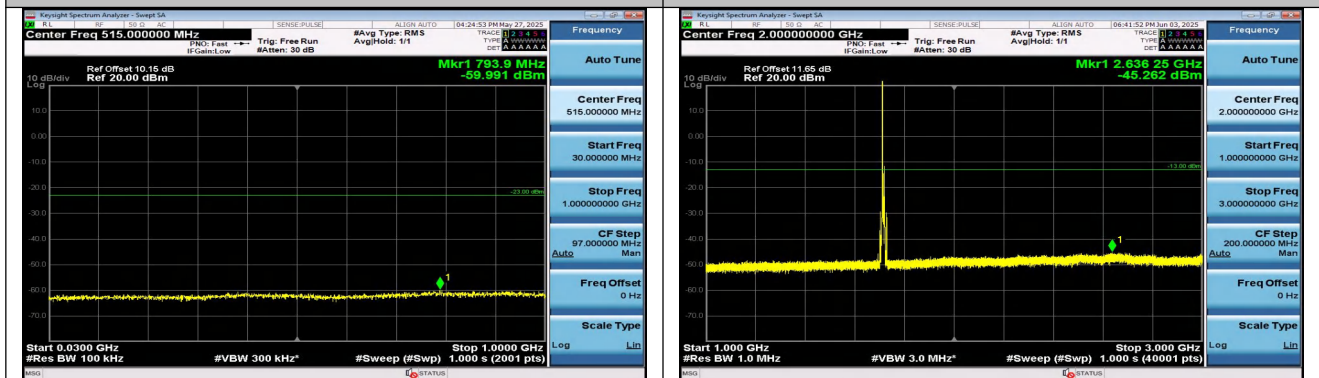
Band4-10MHz-QPSK-20000-1RB#0-30~1000-PASS
