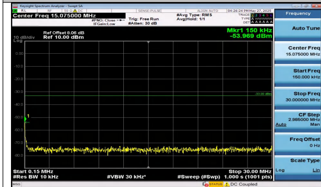
Band4-10MHz-QPSK-20000-1RB#49-0.15~30-PASS
