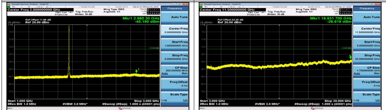
Band4-5MHz-16QAM-20375-25RB#0-1000~3000-PASS
