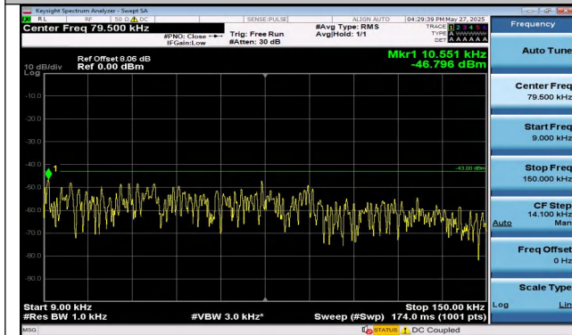
Band4-10MHz-QPSK-20175-1RB#49-0.009~0.15-PASS
