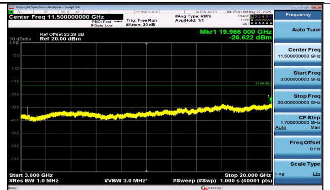
Band4-10MHz-QPSK-20175-1RB#0-3000~20000-PASS
