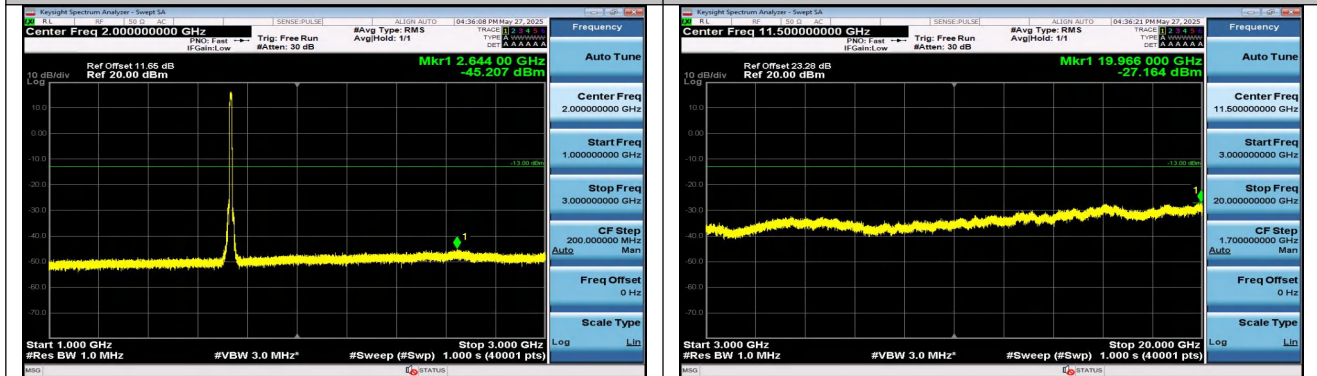
Band4-10MHz-QPSK-20175-50RB#0-1000~3000-PASS
