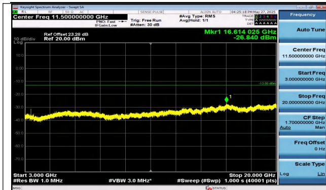
Band4-10MHz-QPSK-20000-1RB#0-3000~20000-PASS
