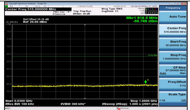
Band4-10MHz-QPSK-20000-1RB#49-30~1000-PASS
