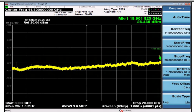
Band4-10MHz-QPSK-20000-1RB#49-3000~20000-PASS
