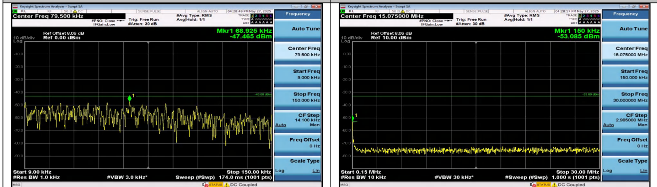
Band4-10MHz-16QAM-20175-1RB#0-0.009~0.15-PASS
