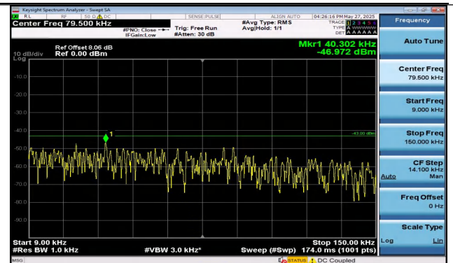
Band4-10MHz-QPSK-20000-1RB#49-0.009~0.15-PASS
