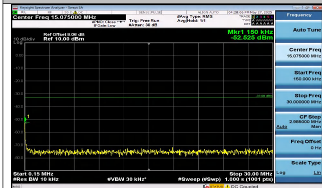
Band4-10MHz-QPSK-20175-1RB#0-0.15~30-PASS
