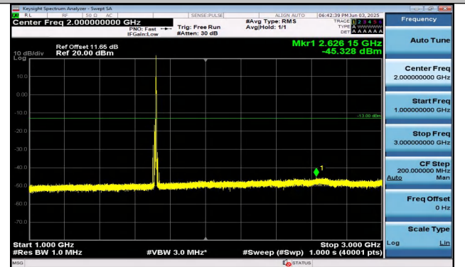
Band4-10MHz-16QAM-20000-1RB#49-1000~3000-PASS
