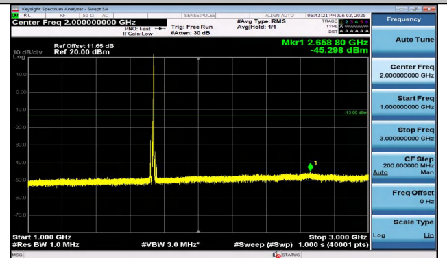
Band4-10MHz-QPSK-20175-1RB#49-1000~3000-PASS
