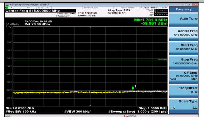
Band4-10MHz-QPSK-20175-1RB#0-30~1000-PASS
