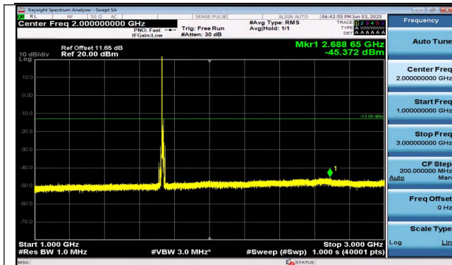
Band4-10MHz-QPSK-20175-1RB#0-1000~3000-PASS
