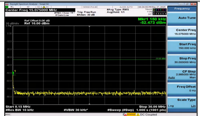
Band4-10MHz-QPSK-20000-50RB#0-0.15~30-PASS
