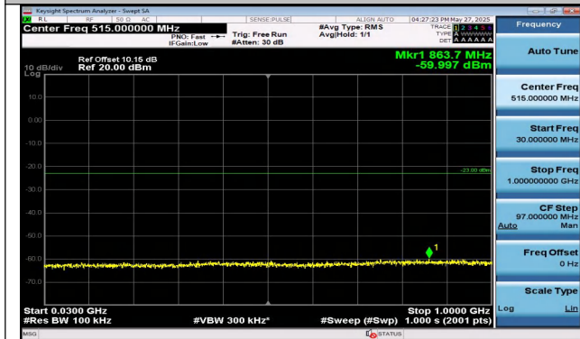
Band4-10MHz-16QAM-20000-1RB#49-30~1000-PASS
