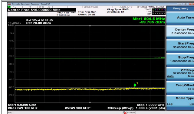
Band4-10MHz-QPSK-20175-1RB#49-30~1000-PASS
