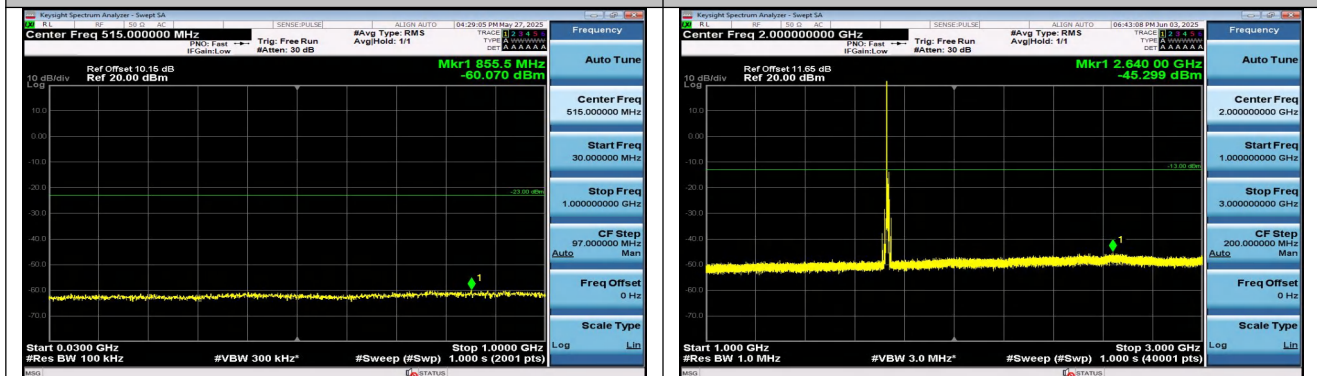
Band4-10MHz-16QAM-20175-1RB#0-30~1000-PASS
