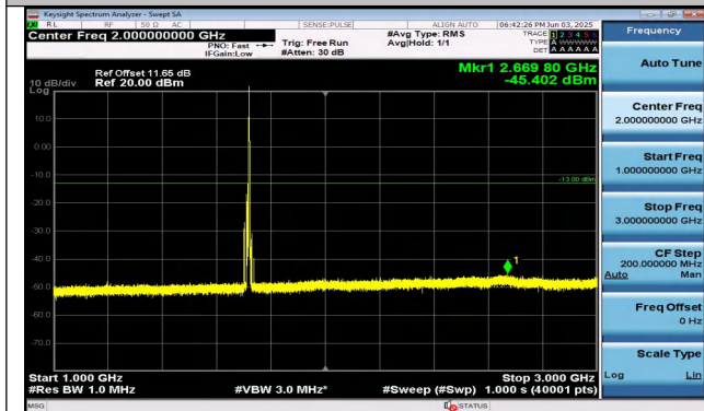
Band4-10MHz-QPSK-20000-1RB#49-1000~3000-PASS
