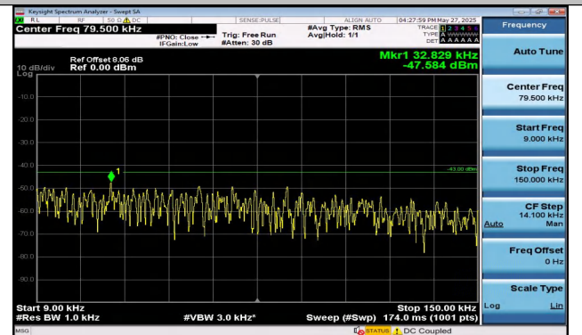
Band4-10MHz-QPSK-20175-1RB#0-0.009~0.15-PASS
