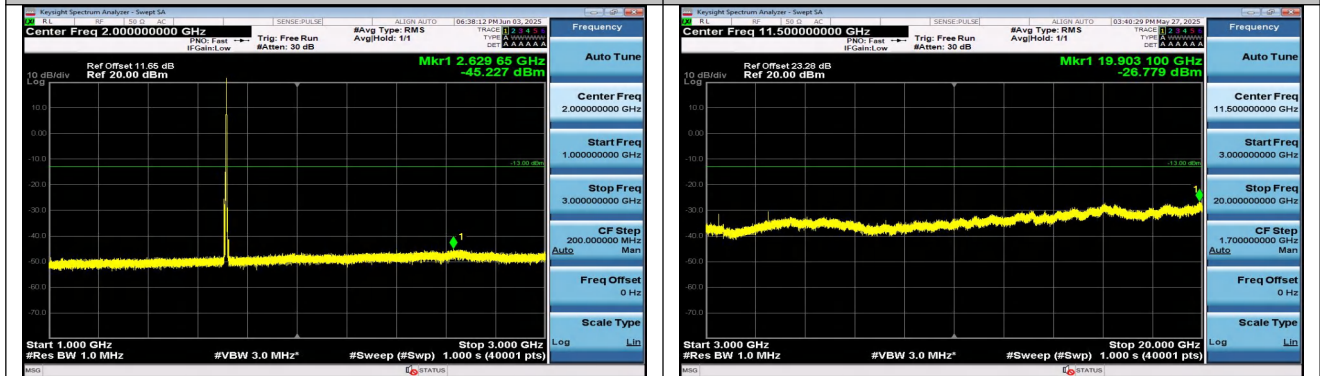
Band4-5MHz-QPSK-19975-1RB#24-1000~3000-PASS
