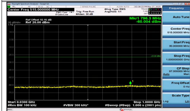
Band4-5MHz-QPSK-19975-1RB#0-0.30~1000-PASS
