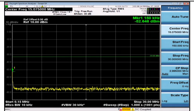
Band4-5MHz-QPSK-19975-1RB#0-0.15~30-PASS
