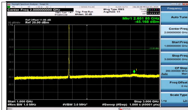
Band4-3MHz-16QAM-20385-15RB#0-1000~3000-PASS
