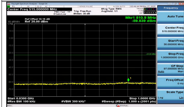
Band4-5MHz-QPSK-20175-25RB#0-30~1000-PASS
