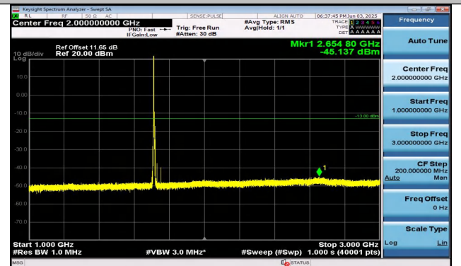
Band4-5MHz-QPSK-19975-1RB#0-1000~3000-PASS
