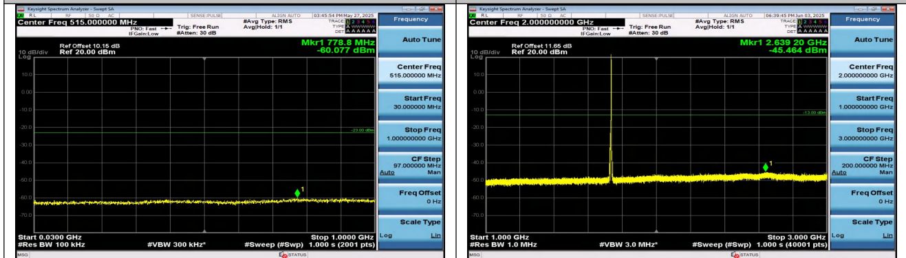
Band4-5MHz-16QAM-20175-1RB#24-30~1000-PASS
