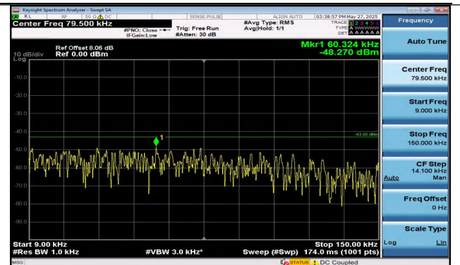
Band4-5MHz-16QAM-19975-1RB#0-0.009~0.15-PASS
