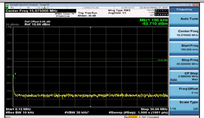
Band4-5MHz-16QAM-19975-1RB#24-0.15~30-PASS
