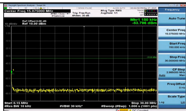
Band4-3MHz-16QAM-20385-1RB#14-0.15~30-PASS
