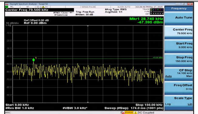
Band4-5MHz-QPSK-19975-1RB#24-0.009~0.15-PASS
