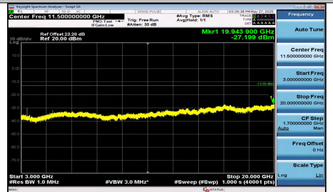
Band4-5MHz-16QAM-19975-1RB#0-3000~20000-PASS
