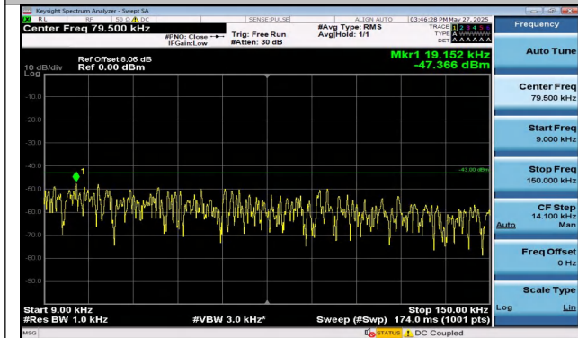
Band4-5MHz-QPSK-20175-25RB#0-0.009~0.15-PASS
