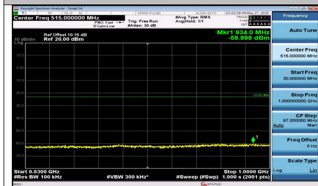
Band4-3MHz-16QAM-20385-1RB#14-30~1000-PASS
