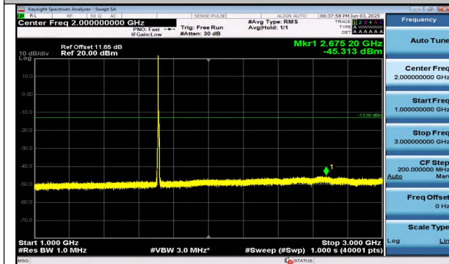
Band4-5MHz-16QAM-19975-1RB#0-1000~3000-PASS
