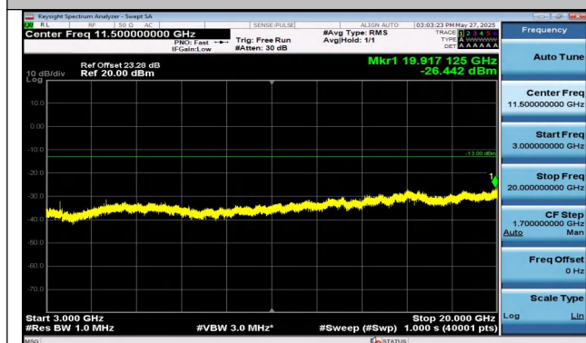
Band4-3MHz-16QAM-20385-1RB#14-3000~20000-PASS
