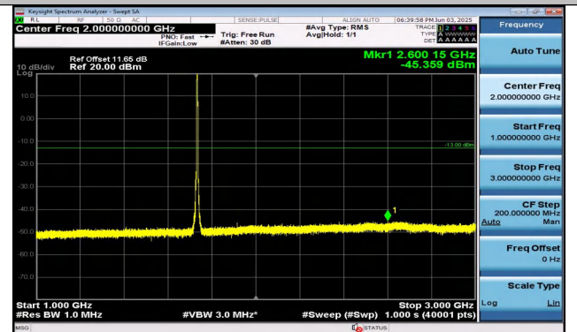
Band4-5MHz-QPSK-20175-25RB#0-1000~3000-PASS
