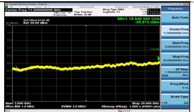
Band4-5MHz-QPSK-20175-1RB#24-3000~20000-PASS
