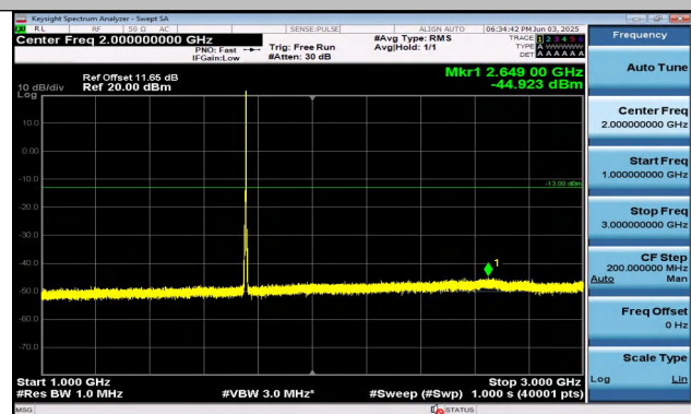
Band4-3MHz-16QAM-20385-1RB#14-1000~3000-PASS
