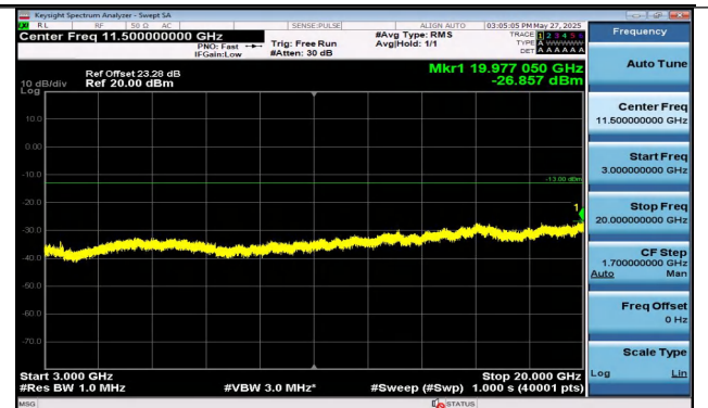
Band4-3MHz-16QAM-20385-15RB#0-3000~20000-PASS
