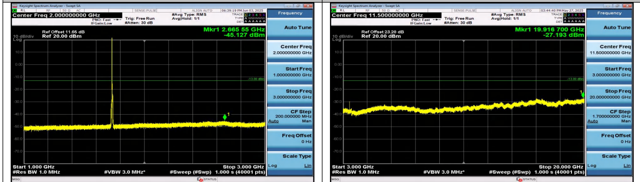
Band4-5MHz-16QAM-20175-1RB#0-1000~3000-PASS
