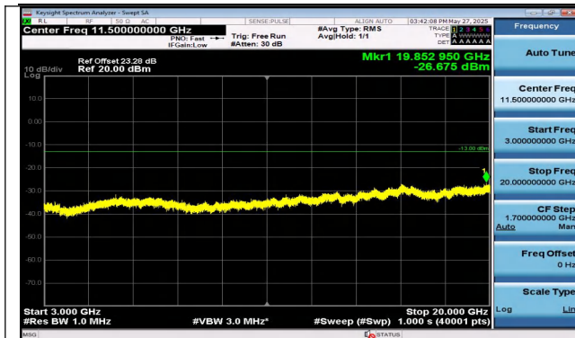
Band4-5MHz-QPSK-19975-25RB#0-3000~20000-PASS
