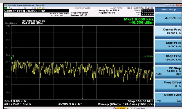
Band4-3MHz-16QAM-20385-15RB#0-0.009~0.15-PASS
