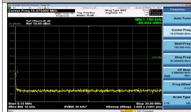
Band4-3MHz-16QAM-20385-15RB#0-0.15~30-PASS
