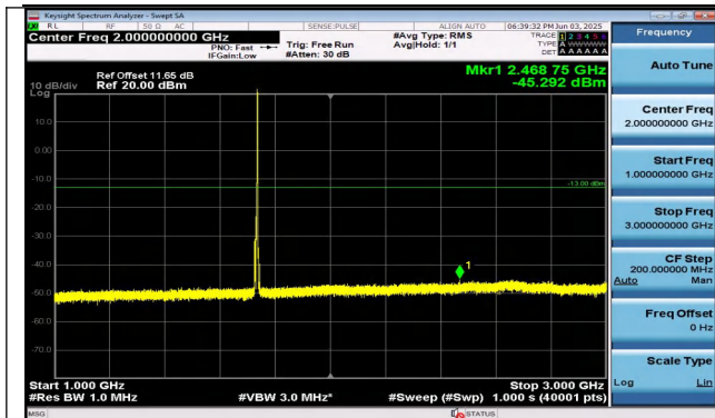
Band4-5MHz-QPSK-20175-1RB#24-1000~3000-PASS
