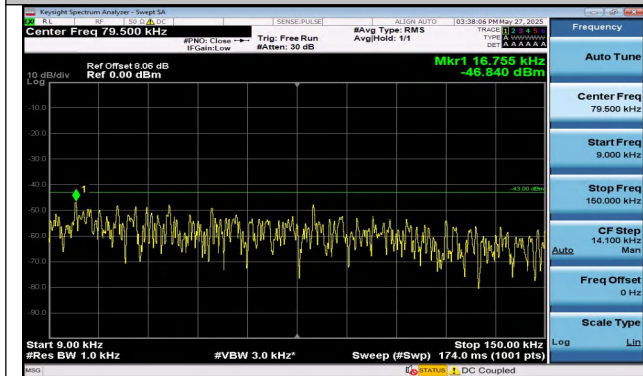
Band4-5MHz-QPSK-19975-1RB#0-0.009~0.15-PASS
