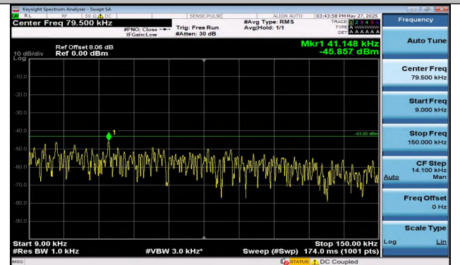
Band4-5MHz-16QAM-20175-1RB#0-0.009~0.15-PASS
