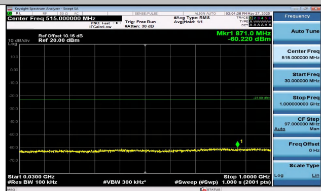
Band4-3MHz-16QAM-20385-15RB#0-30~1000-PASS
