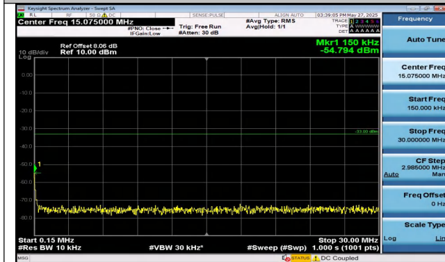
Band4-5MHz-16QAM-19975-1RB#0-0.15~30-PASS
