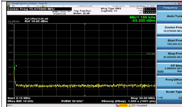
Band4-3MHz-QPSK-20385-1RB#14-0.15~30-PASS
