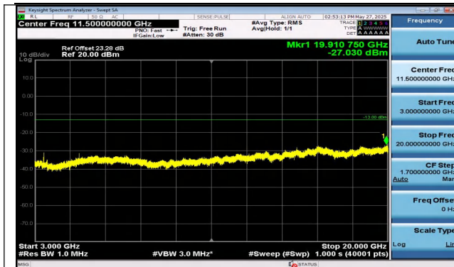
Band4-3MHz-16QAM-19965-1RB#14-3000~20000-PASS
