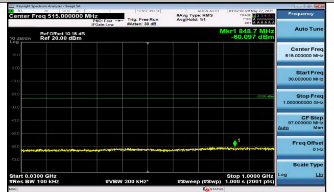
Band4-3MHz-QPSK-20385-1RB#14-30~1000-PASS
