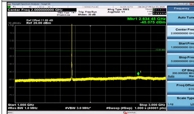
Band4-3MHz-QPSK-20385-1RB#14-1000~3000-PASS
