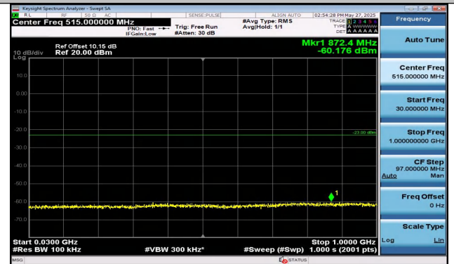
Band4-3MHz-16QAM-19965-15RB#0-30~1000-PASS
