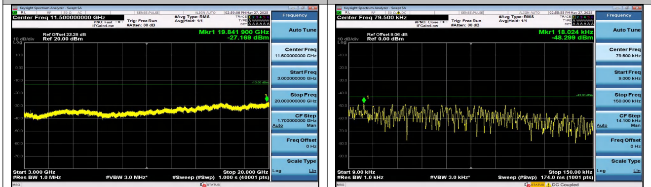
Band4-3MHz-QPSK-20175-15RB#0-3000~20000-PASS
