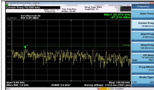
Band4-3MHz-16QAM-20175-1RB#14-0.009~0.15-PASS
