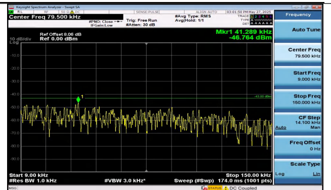
Band4-3MHz-QPSK-20385-1RB#14-0.009~0.15-PASS
