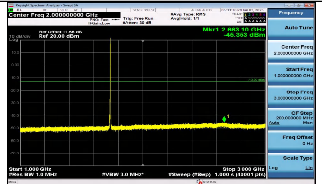
Band4-3MHz-16QAM-20175-1RB#14-1000~3000-PASS
