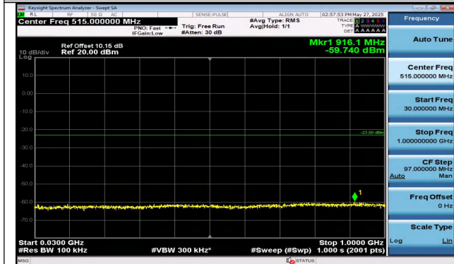
Band4-3MHz-16QAM-20175-1RB#14-30~1000-PASS
