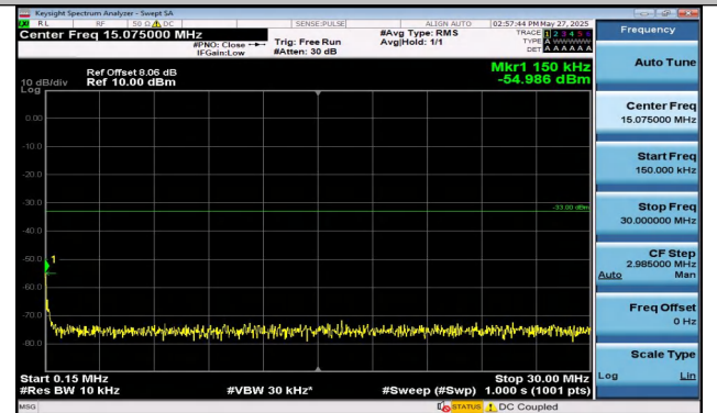
Band4-3MHz-16QAM-20175-1RB#14-0.15~30-PASS
