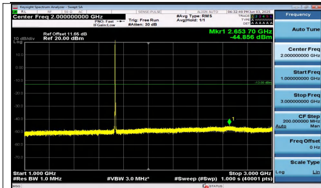
Band4-3MHz-16QAM-20175-1RB#0-1000~3000-PASS
