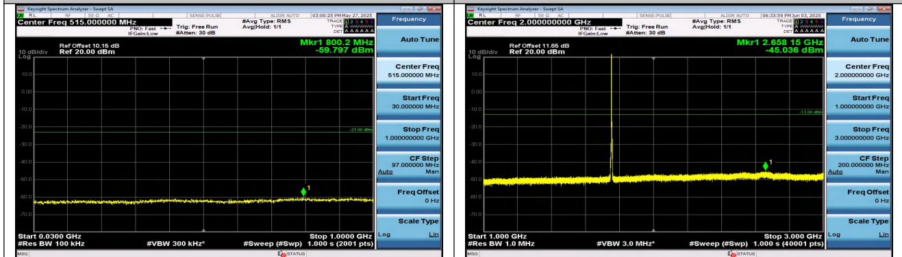
Band4-3MHz-QPSK-20385-1RB#0-30~1000-PASS
