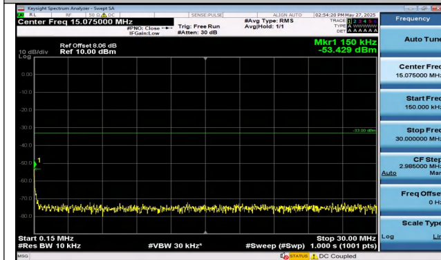
Band4-3MHz-16QAM-19965-15RB#0-0.15~30-PASS
