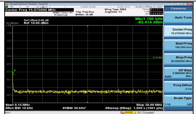
Band4-3MHz-QPSK-20175-1RB#0-0.15~30-PASS
