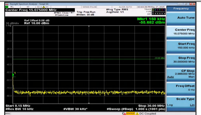
Band4-3MHz-QPSK-20385-15RB#0-0.15~30-PASS
