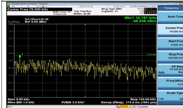
Band4-3MHz-QPSK-20175-1RB#0-0.009~0.15-PASS
