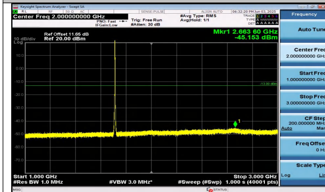
Band4-3MHz-16QAM-19965-15RB#0-1000~3000-PASS
