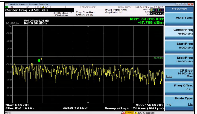
Band4-3MHz-16QAM-19965-15RB#0-0.009~0.15-PASS
