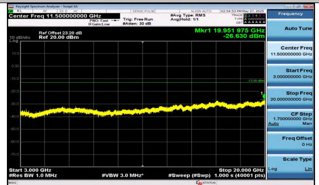
Band4-3MHz-16QAM-19965-15RB#0-3000~20000-PASS
