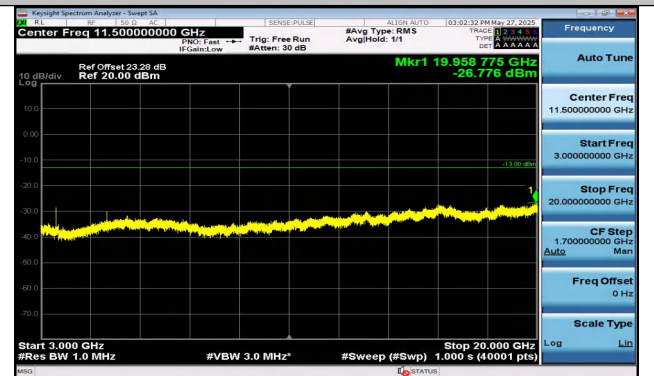
Band4-3MHz-QPSK-20385-1RB#14-3000~20000-PASS
