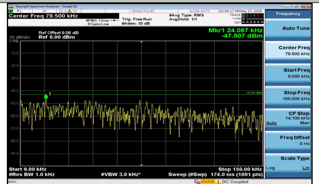
Band4-3MHz-16QAM-20175-15RB#0-0.009~0.15-PASS
