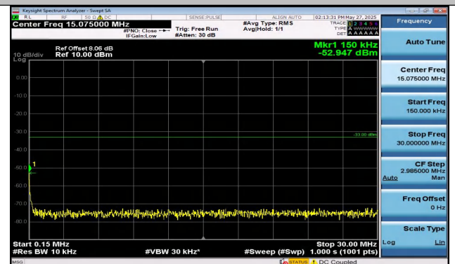
Band4-1.4MHz-16QAM-20393-1RB#5-0.15~30-PASS
