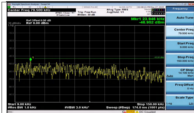
Band4-1.4MHz-16QAM-20175-1RB#5-0.009~0.15-PASS
