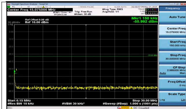
Band4-3MHz-16QAM-19965-1RB#0-0.15~30-PASS
