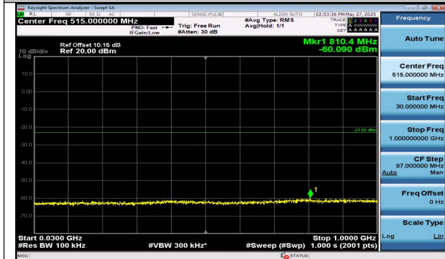
Band4-3MHz-QPSK-19965-15RB#0-30~1000-PASS
