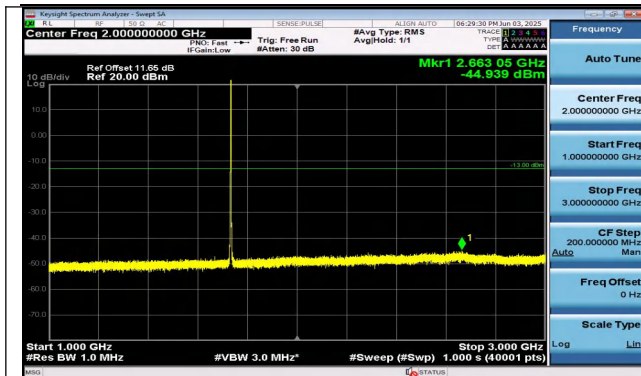
Band4-1.4MHz-16QAM-20175-6RB#0-1000~3000-PASS
