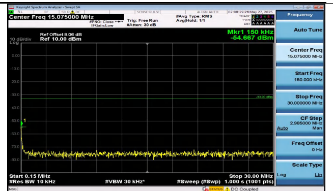
Band4-1.4MHz-16QAM-20175-1RB#5-0.15~30-PASS
