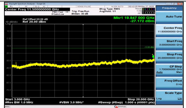
Band4-1.4MHz-16QAM-20393-1RB#0-3000~20000-PASS
