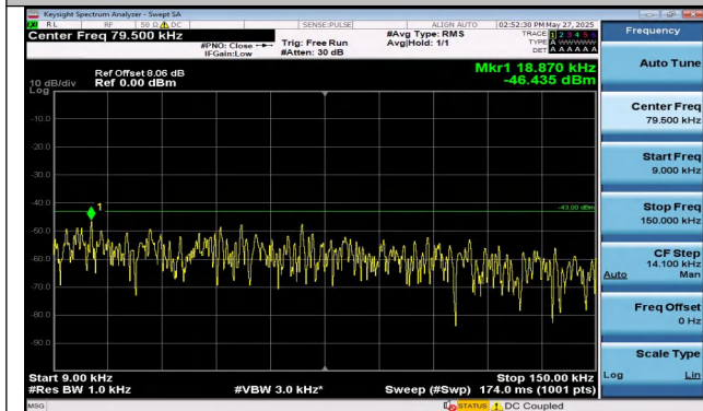
Band4-3MHz-16QAM-19965-1RB#14-0.009~0.15-PASS
