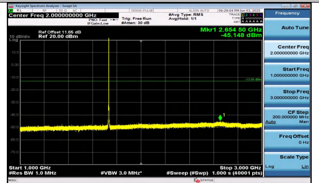
Band4-1.4MHz-16QAM-20175-1RB#5-1000~3000-PASS
