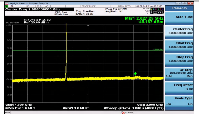
Band4-3MHz-QPSK-19965-15RB#0-1000~3000-PASS
