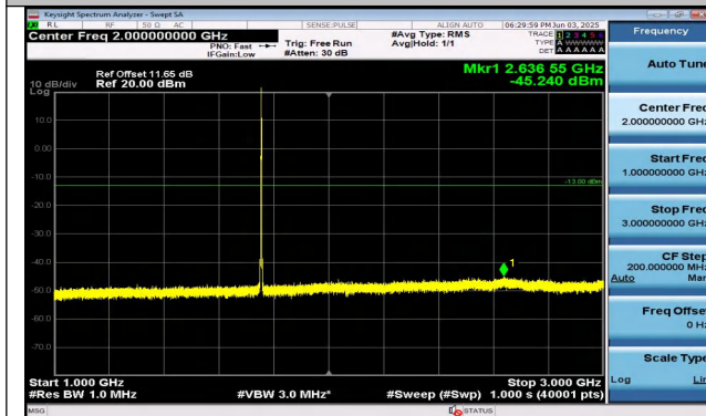
Band4-1.4MHz-16QAM-20393-1RB#0-1000~3000-PASS
