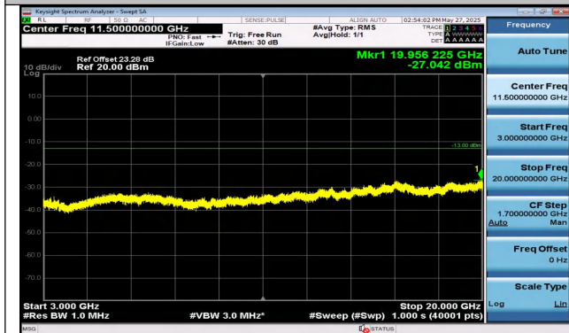
Band4-3MHz-QPSK-19965-15RB#0-3000~20000-PASS
