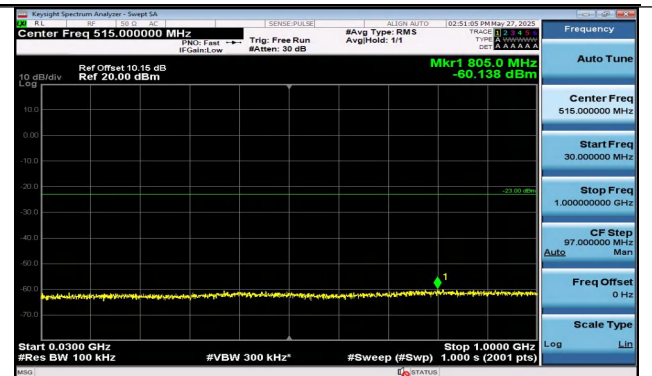
Band4-3MHz-16QAM-19965-1RB#0-30~1000-PASS
