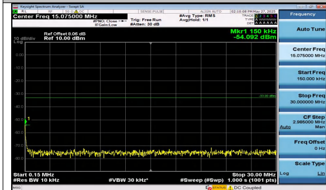
Band4-1.4MHz-16QAM-20175-6RB#0-0.15~30-PASS
