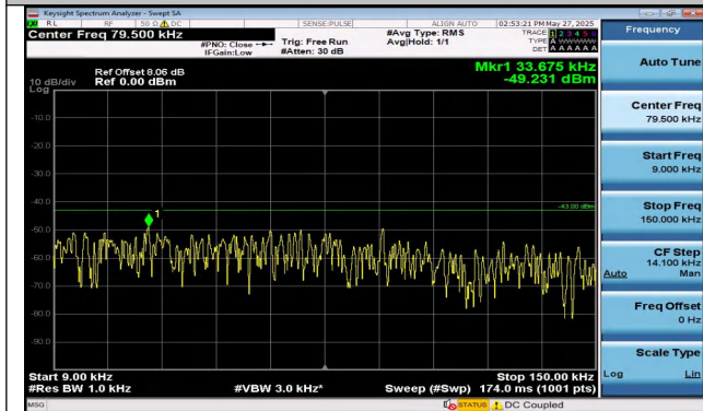
Band4-3MHz-QPSK-19965-15RB#0-0.009~0.15-PASS
