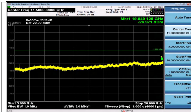
Band4-1.4MHz-QPSK-20393-6RB#0-3000~20000-PASS
