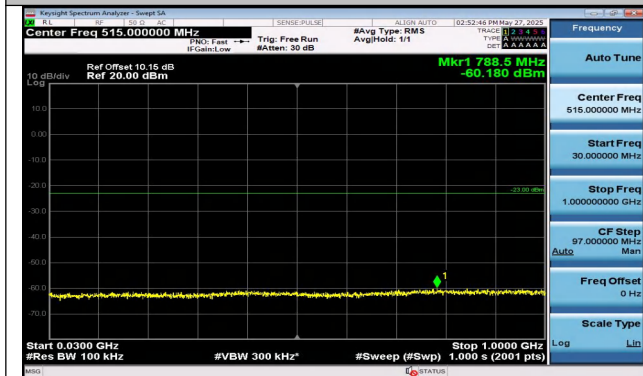
Band4-3MHz-16QAM-19965-1RB#14-30~1000-PASS
