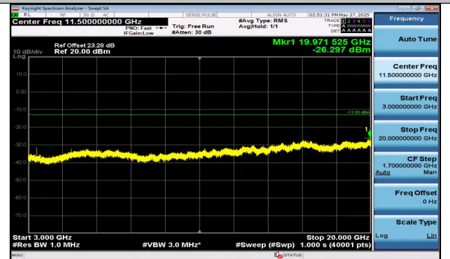
Band4-3MHz-16QAM-19965-1RB#0-3000~20000-PASS
