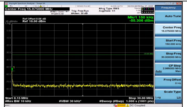
Band4-3MHz-QPSK-19965-15RB#0-0.15~30-PASS
