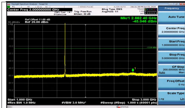
Band4-3MHz-QPSK-19965-1RB#14-1000~3000-PASS
