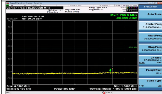
Band4-1.4MHz-16QAM-20175-1RB#5-30~1000-PASS
