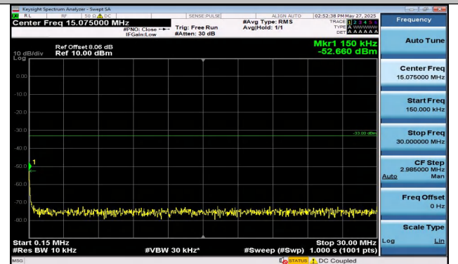
Band4-3MHz-16QAM-19965-1RB#14-0.15~30-PASS
