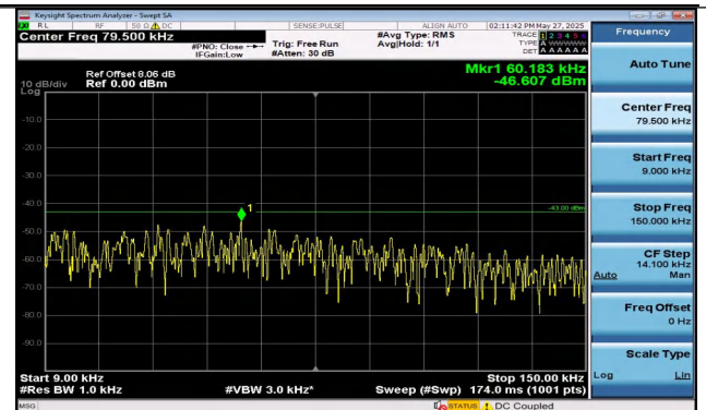
Band4-1.4MHz-16QAM-20393-1RB#0-0.009~0.15-PASS
