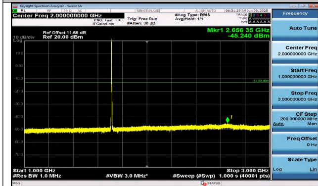
Band4-3MHz-16QAM-19965-1RB#0-1000~3000-PASS
