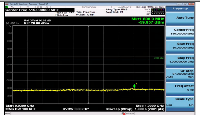
Band4-1.4MHz-16QAM-20175-6RB#0-30~1000-PASS
