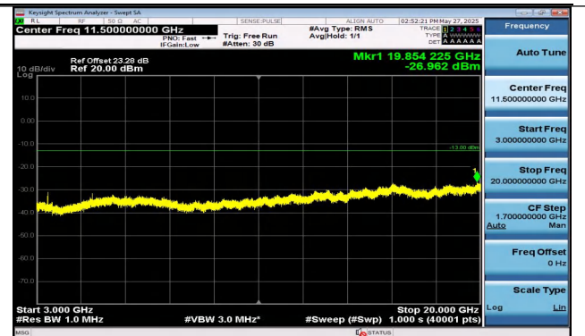
Band4-3MHz-QPSK-19965-1RB#14-3000~20000-PASS
