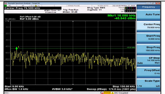
Band4-1.4MHz-16QAM-20175-6RB#0-0.009~0.15-PASS
