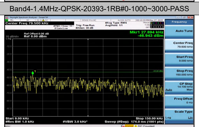
Band4-1.4MHz-QPSK-20393-1RB#0-1000~3000-PASS
