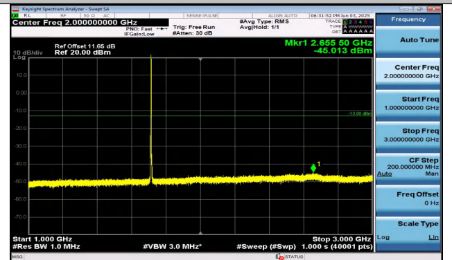
Band4-3MHz-16QAM-19965-1RB#14-1000~3000-PASS
