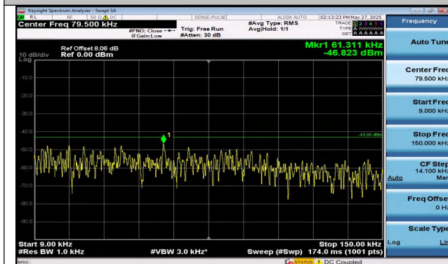
Band4-1.4MHz-16QAM-20393-1RB#5-0.009~0.15-PASS
