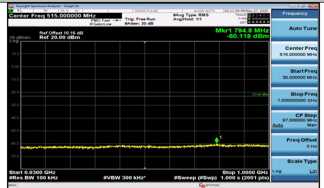
Band4-1.4MHz-16QAM-20393-1RB#0-30~1000-PASS
