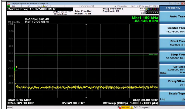
Band4-1.4MHz-16QAM-20393-1RB#0-0.15~30-PASS
