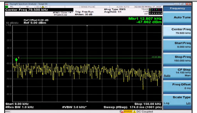
Band4-3MHz-16QAM-19965-1RB#0-0.009~0.15-PASS
