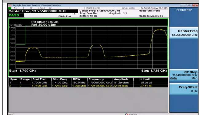
Band4-15MHz-16QAM-20025-1RB#74-PASS
