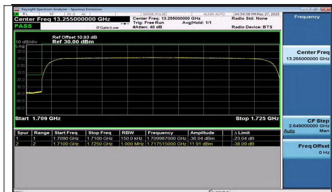
Band4-15MHz-QPSK-20025-75RB#0-PASS
