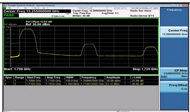
Band4-15MHz-16QAM-20025-1RB#0-PASS
