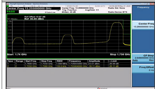
Band4-15MHz-QPSK-20325-1RB#74-PASS
