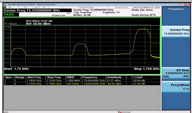
Band4-15MHz-16QAM-20325-1RB#74-PASS
