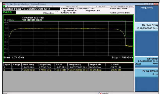
Band4-15MHz-QPSK-20325-75RB#0-PASS
