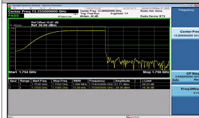
Band4-1.4MHz-16QAM-20393-1RB#5-PASS
