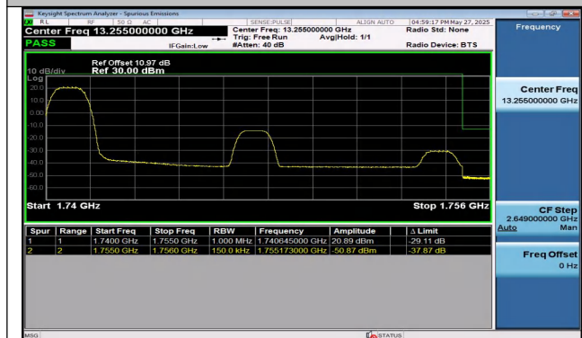
Band4-15MHz-16QAM-20325-1RB#0-PASS
