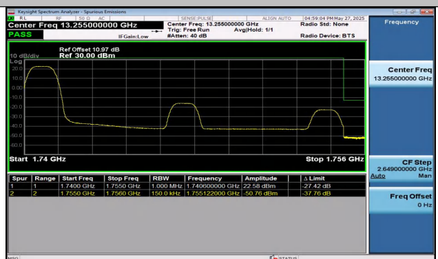
Band4-15MHz-QPSK-20325-1RB#0-PASS
