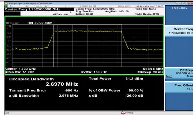
Band4-3MHz-QPSK-20175-15RB#0-PASS
