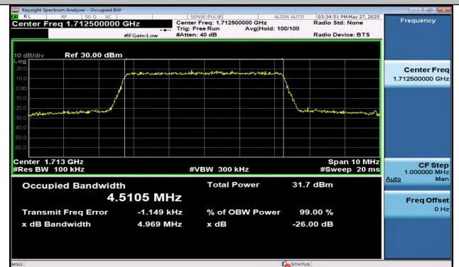
Band4-5MHz-16QAM-19975-25RB#0-PASS
