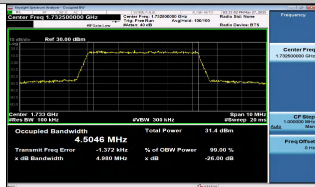
Band4-5MHz-QPSK-20175-25RB#0-PASS
