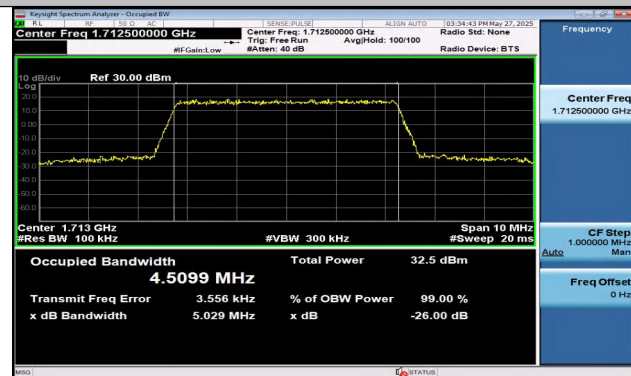
Band4-5MHz-QPSK-19975-25RB#0-PASS
