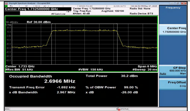
Band4-3MHz-16QAM-20175-15RB#0-PASS
