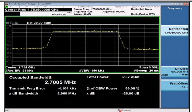
Band4-3MHz-16QAM-20385-15RB#0-PASS
