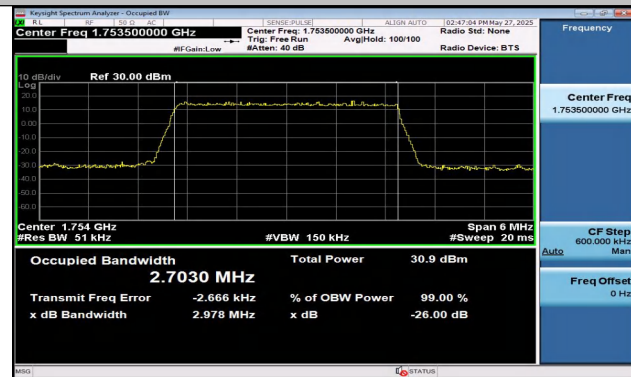
Band4-3MHz-QPSK-20385-15RB#0-PASS
