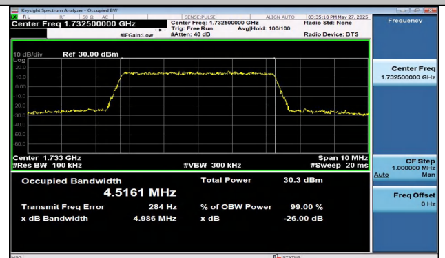
Band4-5MHz-16QAM-20175-25RB#0-PASS
