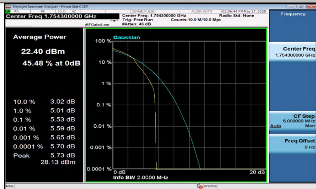
Band4-1.4MHz-16QAM-20393-1RB#0-PASS
