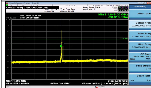
Band2-20MHz-16QAM-18700-1RB#0-1000~3000-PASS
