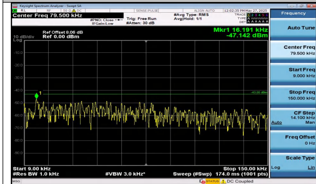
Band2-20MHz-QPSK-18700-1RB#0-0.009~0.15-PASS
