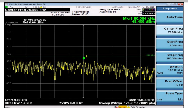
Band2-20MHz-QPSK-18700-1RB#99-0.009~0.15-PASS
