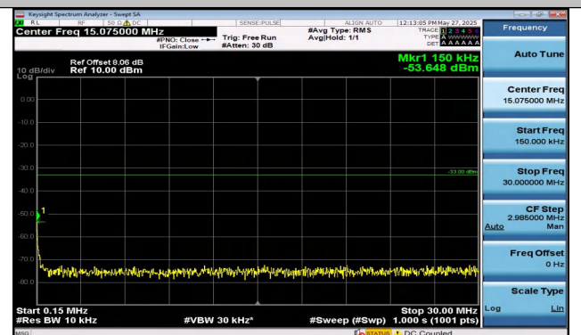
Band2-20MHz-QPSK-18700-100RB#0-0.15~30-PASS
