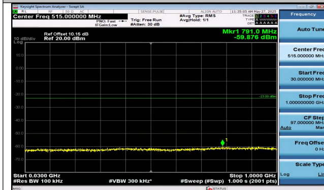
Band2-15MHz-16QAM-18900-1RB#74-30~1000-PASS
