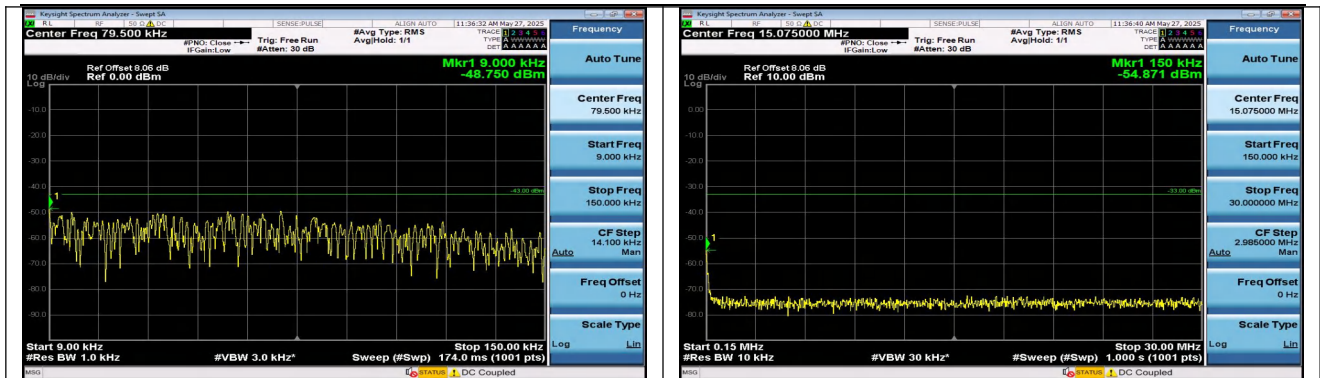
Band2-15MHz-16QAM-19125-1RB#0-0.009~0.15-PASS
