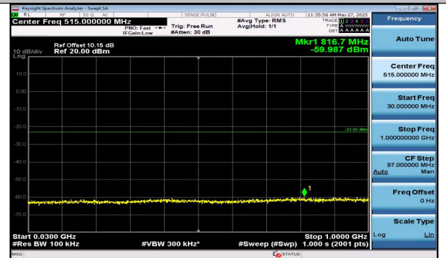
Band2-15MHz-QPSK-19125-1RB#0-30~1000-PASS
