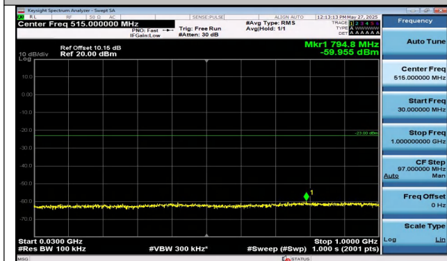
Band2-20MHz-QPSK-18700-100RB#0-30~1000-PASS
