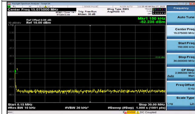
Band2-15MHz-QPSK-19125-1RB#0-0.15~30-PASS
