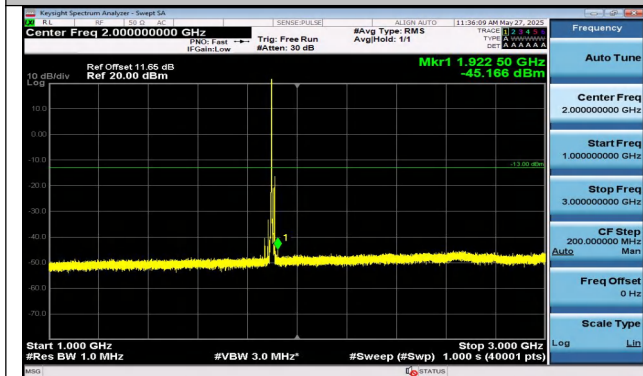
Band2-15MHz-QPSK-19125-1RB#0-1000~3000-PASS
