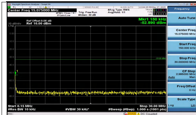
Band2-20MHz-QPSK-18700-1RB#99-0.15~30-PASS
