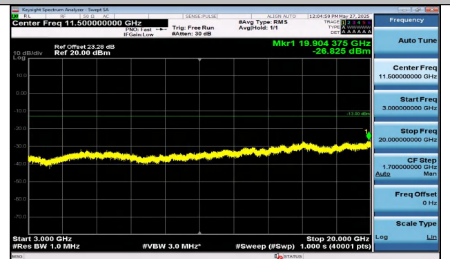
Band2-20MHz-QPSK-18700-1RB#99-3000~20000-PASS
