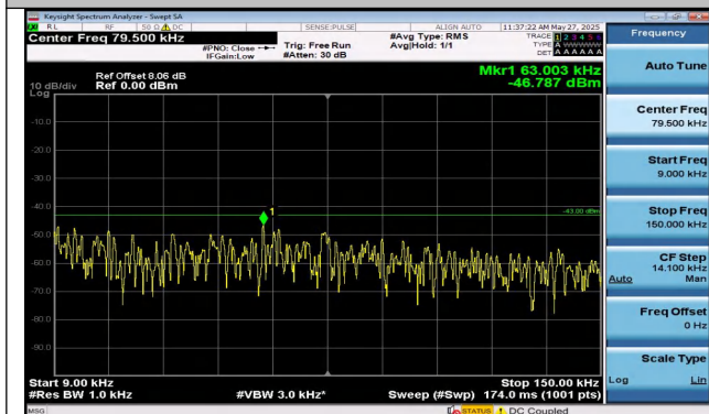
Band2-15MHz-QPSK-19125-1RB#74-0.009~0.15-PASS
