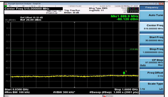
Band2-20MHz-QPSK-18700-1RB#99-30~1000-PASS
