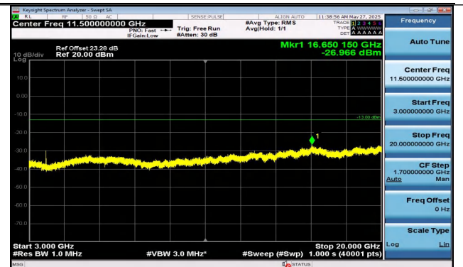
Band2-15MHz-16QAM-19125-1RB#74-3000~20000-PASS
