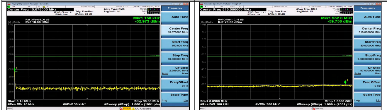
Band2-15MHz-16QAM-19125-1RB#74-0.15~30-PASS
