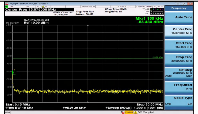
Band2-20MHz-QPSK-18700-1RB#0-0.15~30-PASS
