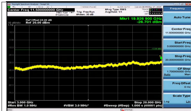
Band2-20MHz-QPSK-18700-100RB#0-3000~20000-PASS
