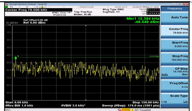
Band2-20MHz-16QAM-18700-1RB#0-0.009~0.15-PASS
