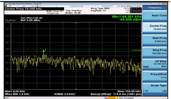
Band2-15MHz-QPSK-19125-1RB#0-0.009~0.15-PASS
