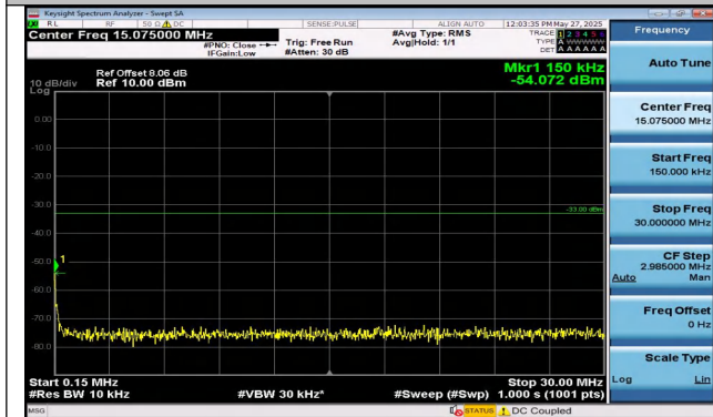
Band2-20MHz-16QAM-18700-1RB#0-0.15~30-PASS
