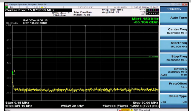
Band2-20MHz-16QAM-18700-1RB#99-0.15~30-PASS
