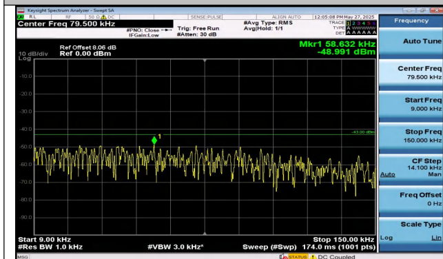
Band2-20MHz-16QAM-18700-1RB#99-0.009~0.15-PASS
