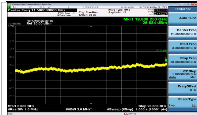
Band2-15MHz-16QAM-18900-1RB#74-3000~20000-PASS
