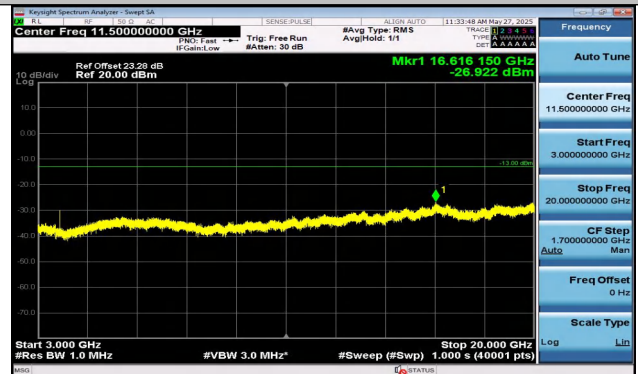
Band2-15MHz-16QAM-18900-1RB#0-3000~20000-PASS
