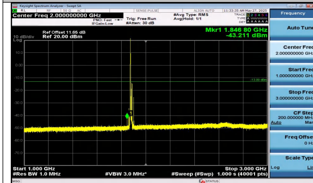
Band2-15MHz-16QAM-18900-1RB#0-1000~3000-PASS
