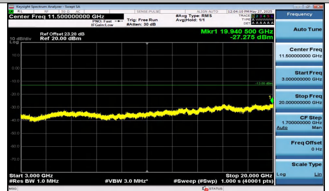
Band2-20MHz-16QAM-18700-1RB#0-3000~20000-PASS
