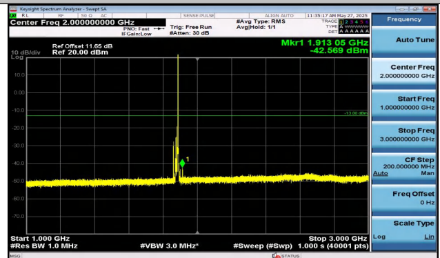
Band2-15MHz-16QAM-18900-1RB#74-1000~3000-PASS
