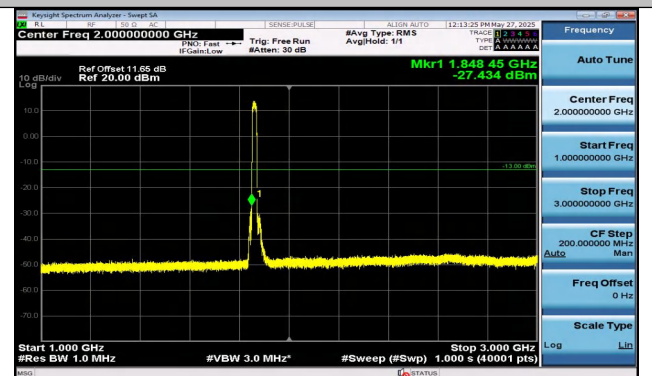
Band2-20MHz-QPSK-18700-100RB#0-1000~3000-PASS
