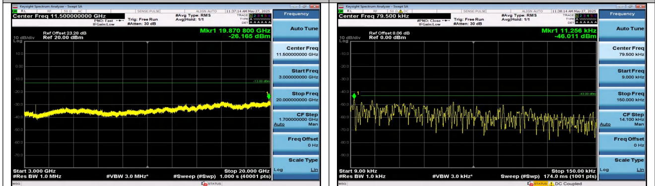
Band2-15MHz-16QAM-19125-1RB#0-3000~20000-PASS
