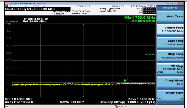
Band2-20MHz-16QAM-18700-1RB#0-30~1000-PASS
