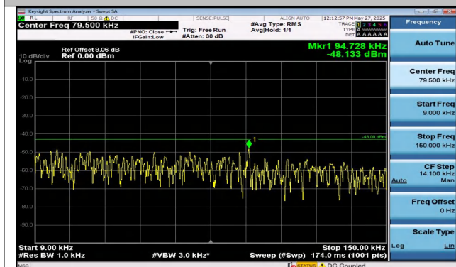
Band2-20MHz-QPSK-18700-100RB#0-0.009~0.15-PASS
