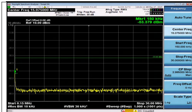
Band2-5MHz-16QAM-19175-25RB#0-0.15~30-PASS
