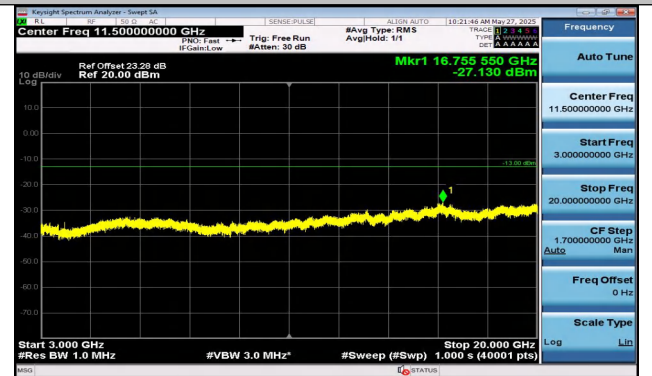
Band2-5MHz-16QAM-19175-25RB#0-3000~20000-PASS
