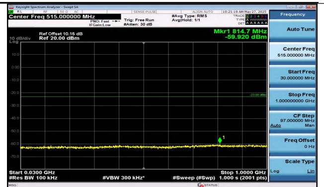
Band2-5MHz-16QAM-19175-25RB#0-30~1000-PASS
