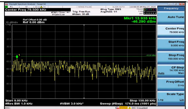
Band2-10MHz-16QAM-18900-1RB#49-0.009~0.15-PASS
