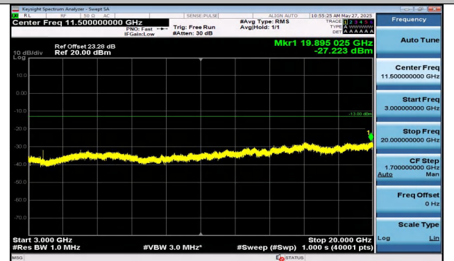
Band2-10MHz-QPSK-18650-1RB#49-3000~20000-PASS
