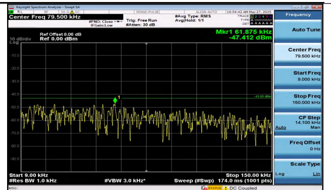
Band2-10MHz-QPSK-18650-1RB#49-0.009~0.15-PASS
