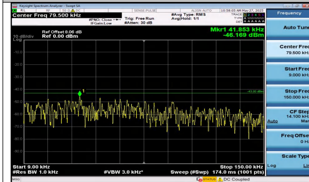
Band2-10MHz-QPSK-18900-1RB#49-0.009~0.15-PASS
