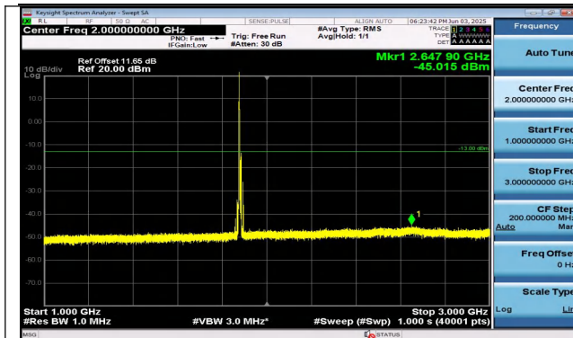
Band2-10MHz-QPSK-18900-1RB#0-1000~3000-PASS
