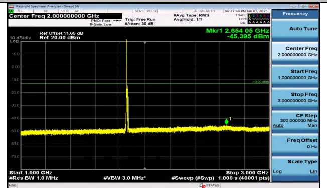
Band2-10MHz-QPSK-18650-1RB#0-1000~3000-PASS
