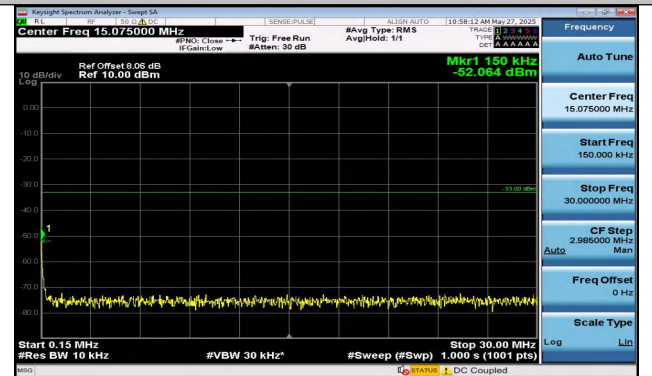
Band2-10MHz-QPSK-18900-1RB#49-0.15~30-PASS
