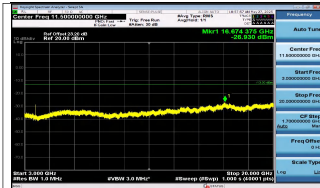
Band2-10MHz-16QAM-18900-1RB#0-3000~20000-PASS
