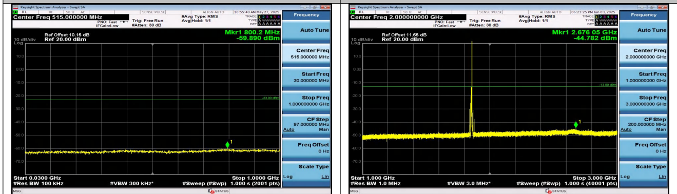
Band2-10MHz-16QAM-18650-1RB#49-30~1000-PASS
