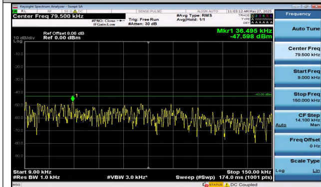
Band2-10MHz-QPSK-18650-50RB#0-0.009~0.15-PASS
