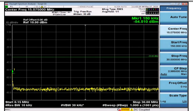
Band2-10MHz-QPSK-18650-50RB#0-0.15~30-PASS
