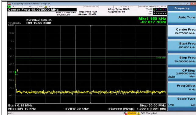
Band2-10MHz-QPSK-18650-1RB#49-0.15~30-PASS
