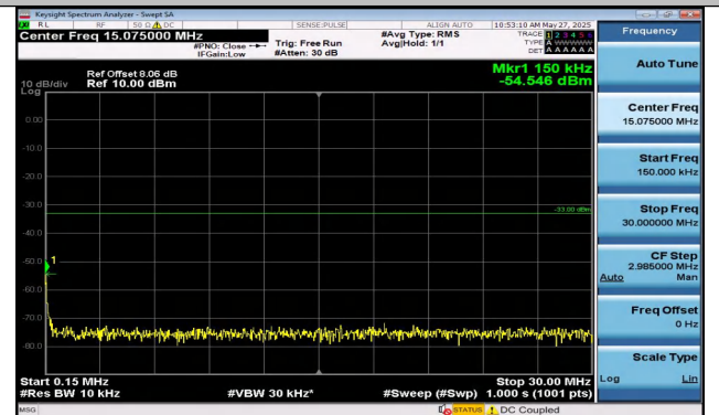
Band2-10MHz-QPSK-18650-1RB#0-0.15~30-PASS
