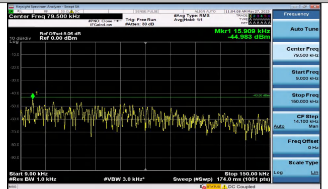
Band2-10MHz-QPSK-18900-50RB#0-0.009~0.15-PASS
