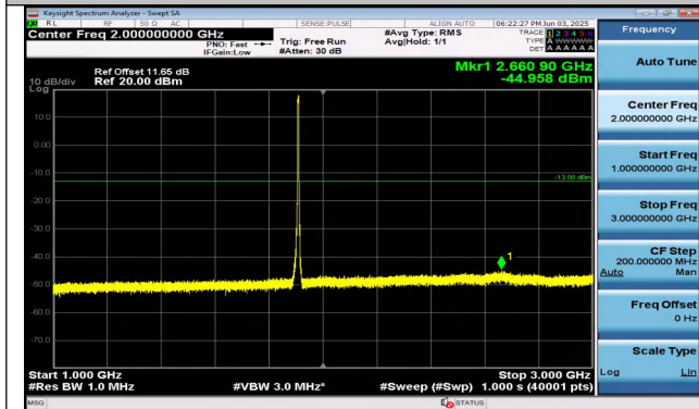
Band2-5MHz-16QAM-19175-25RB#0-1000~3000-PASS
