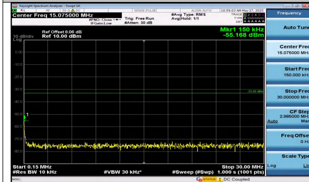
Band2-10MHz-16QAM-18900-1RB#49-0.15~30-PASS
