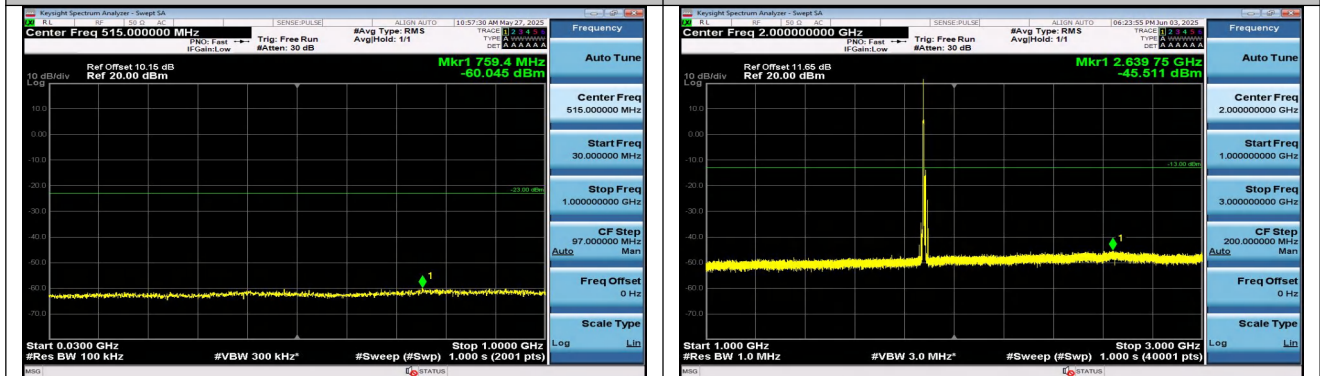
Band2-10MHz-16QAM-18900-1RB#0-30~1000-PASS
