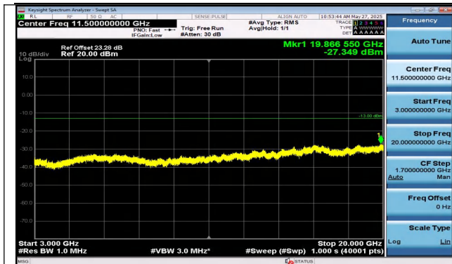
Band2-10MHz-QPSK-18650-1RB#0-3000~20000-PASS
