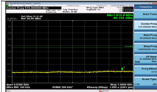
Band2-10MHz-QPSK-18650-1RB#0-30~1000-PASS
