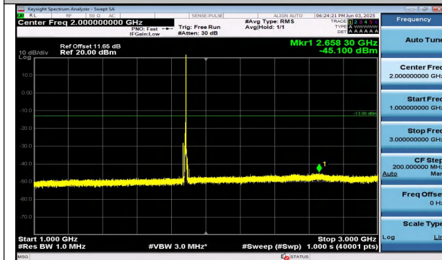
Band2-10MHz-16QAM-18900-1RB#49-1000~3000-PASS
