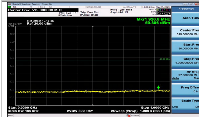
Band2-10MHz-QPSK-18900-1RB#49-30~1000-PASS
