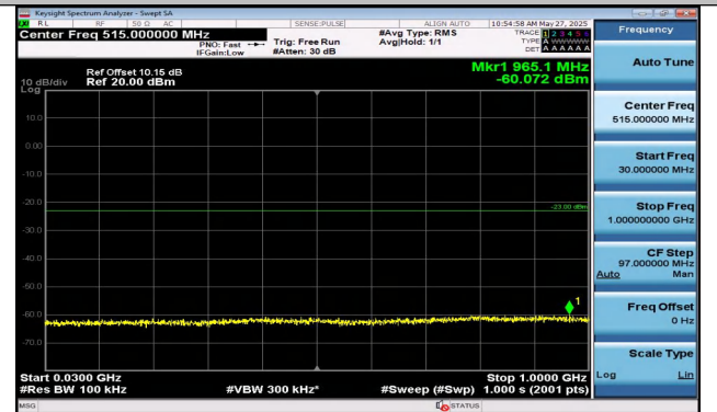
Band2-10MHz-QPSK-18650-1RB#49-30~1000-PASS
