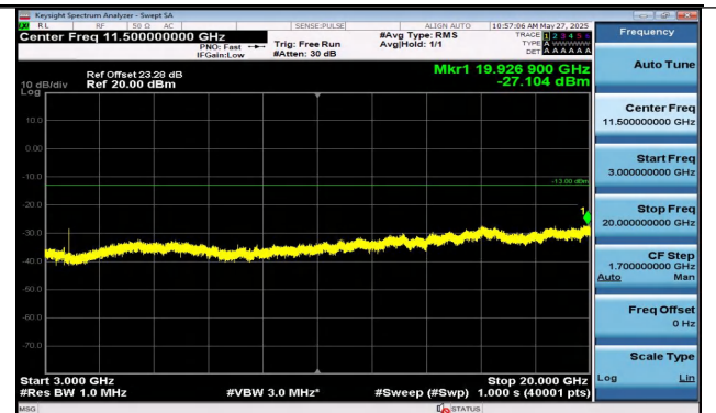
Band2-10MHz-QPSK-18900-1RB#0-3000~20000-PASS
