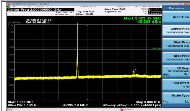
Band2-10MHz-QPSK-18650-1RB#49-1000~3000-PASS
