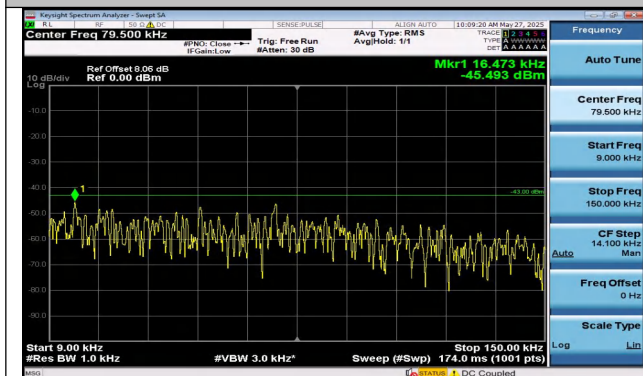
Band2-5MHz-16QAM-18625-1RB#24-0.009~0.15-PASS
