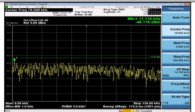
Band2-5MHz-16QAM-18625-25RB#0-0.009~0.15-PASS
