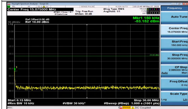
Band2-5MHz-QPSK-18900-1RB#24-0.15~30-PASS
