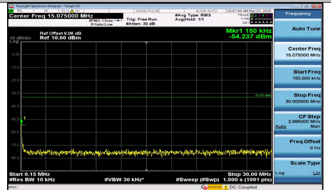
Band2-5MHz-QPSK-18625-1RB#0-0.15~30-PASS
