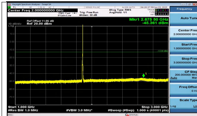
Band2-5MHz-QPSK-18900-1RB#24-1000~3000-PASS
