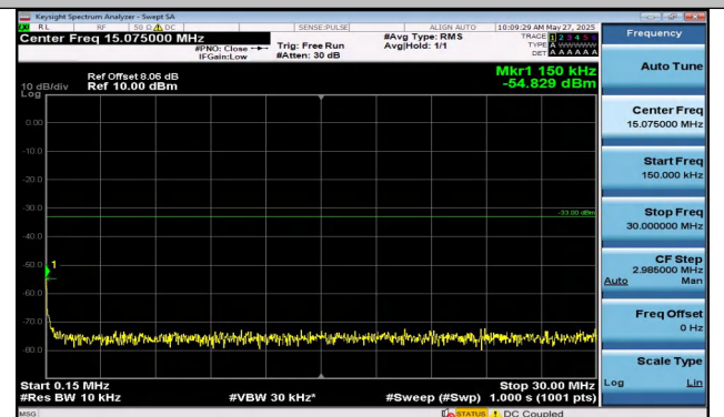
Band2-5MHz-16QAM-18625-1RB#24-0.15~30-PASS
