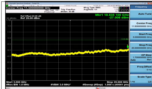
Band2-5MHz-QPSK-18625-25RB#0-3000~20000-PASS
