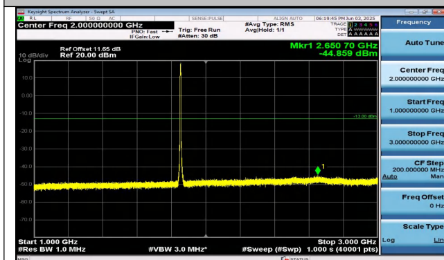
Band2-5MHz-16QAM-18625-25RB#0-1000~3000-PASS
