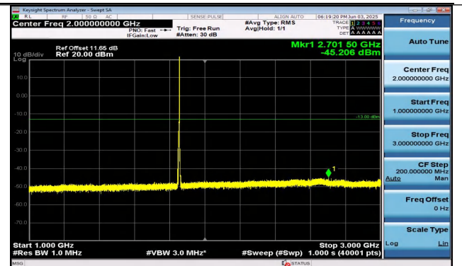
Band2-5MHz-16QAM-18625-1RB#24-1000~3000-PASS
