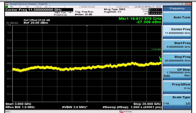
Band2-5MHz-16QAM-18625-1RB#0-3000~20000-PASS
