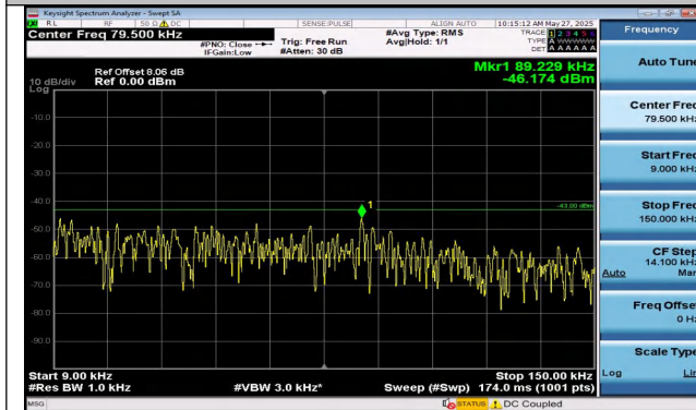
Band2-5MHz-QPSK-18900-25RB#0-0.009~0.15-PASS
