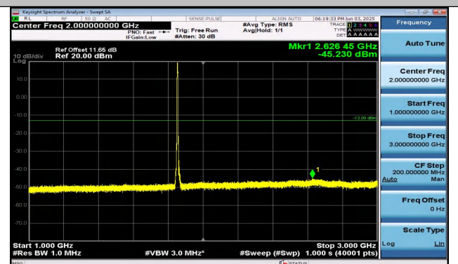
Band2-5MHz-QPSK-18625-25RB#0-1000~3000-PASS
