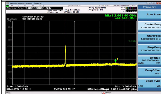
Band2-5MHz-16QAM-18625-1RB#0-1000~3000-PASS
