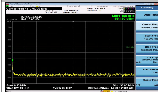
Band2-5MHz-16QAM-18625-25RB#0-0.15~30-PASS
