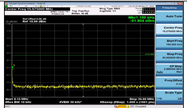
Band2-5MHz-QPSK-18900-25RB#0-0.15~30-PASS
