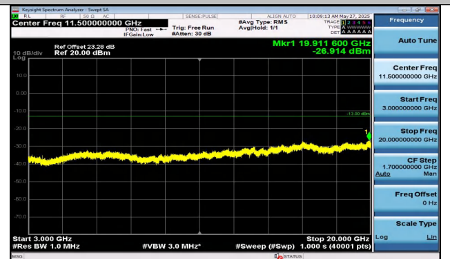
Band2-5MHz-QPSK-18625-1RB#24-3000~20000-PASS
