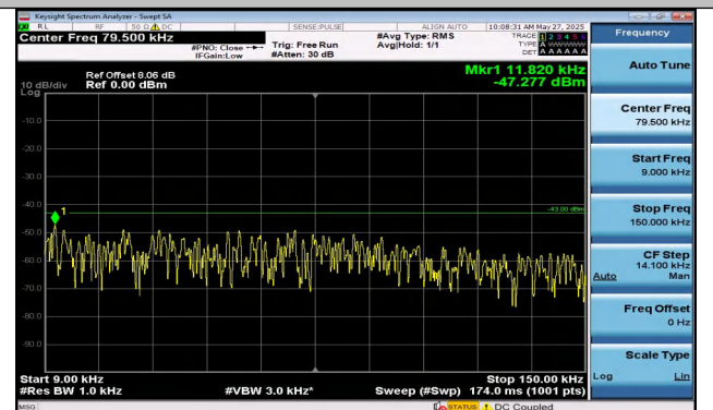
Band2-5MHz-QPSK-18625-1RB#24-0.009~0.15-PASS
