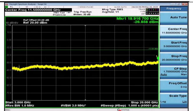
Band2-3MHz-16QAM-19185-15RB#0-3000~20000-PASS
