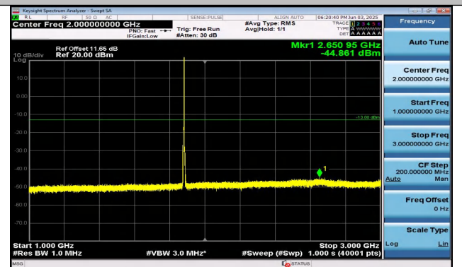
Band2-5MHz-16QAM-18900-1RB#24-1000~3000-PASS
