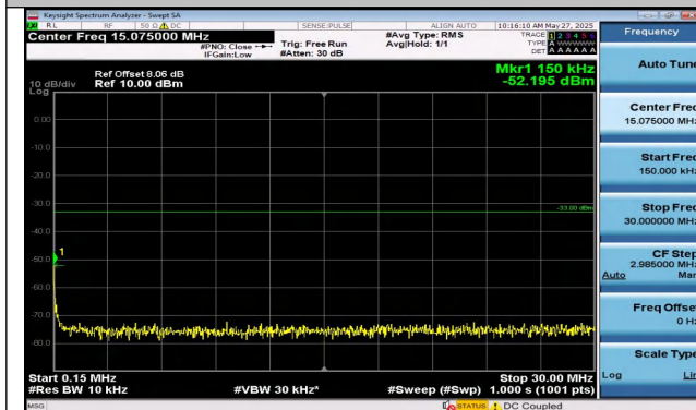
Band2-5MHz-16QAM-18900-25RB#0-0.15~30-PASS
