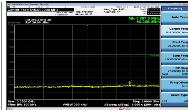
Band2-5MHz-16QAM-18625-1RB#24-30~1000-PASS
