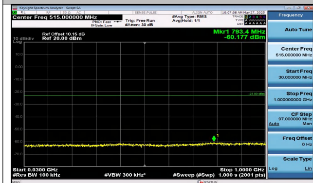
Band2-5MHz-QPSK-18625-1RB#0-30~1000-PASS
