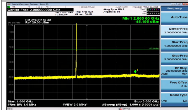
Band2-5MHz-QPSK-18625-1RB#24-1000~3000-PASS
