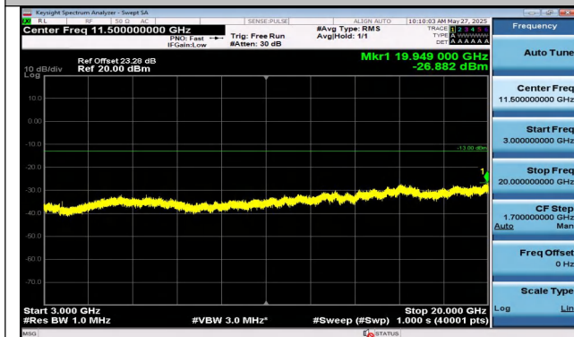
Band2-5MHz-16QAM-18625-1RB#24-3000~20000-PASS
