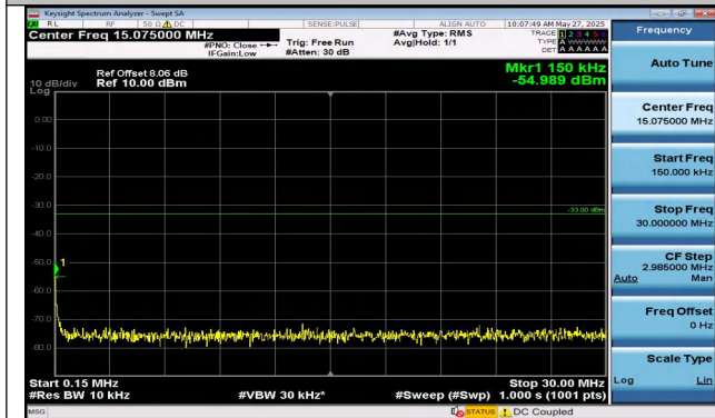
Band2-5MHz-16QAM-18625-1RB#0-0.15~30-PASS
