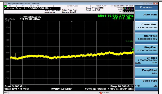
Band2-5MHz-16QAM-18900-1RB#0-3000~20000-PASS
