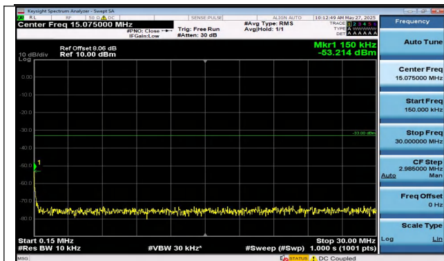
Band2-5MHz-16QAM-18900-1RB#0-0.15~30-PASS
