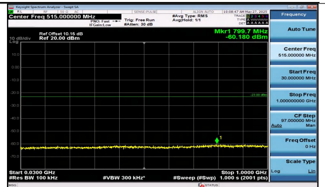
Band2-5MHz-QPSK-18625-1RB#24-30~1000-PASS
