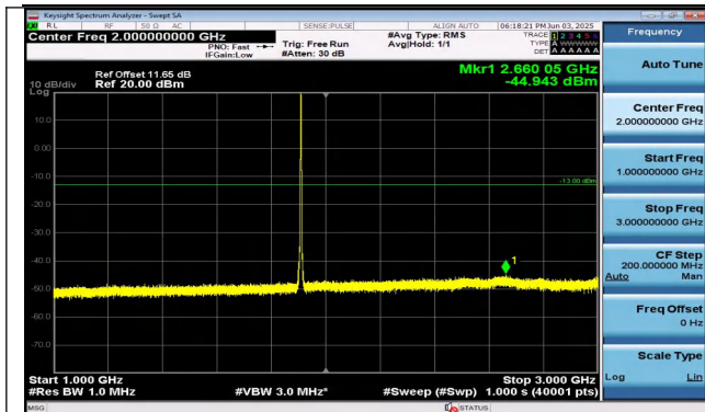
Band2-3MHz-16QAM-19185-15RB#0-1000~3000-PASS
