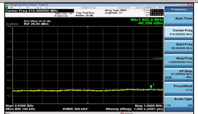
Band2-5MHz-16QAM-18625-25RB#0-30~1000-PASS
