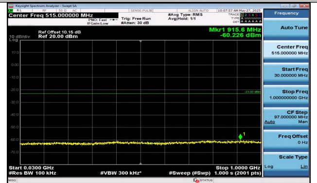
Band2-5MHz-16QAM-18625-1RB#0-30~1000-PASS
