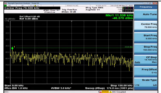
Band2-5MHz-16QAM-18900-1RB#0-0.009~0.15-PASS
