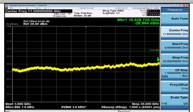
Band2-5MHz-16QAM-18900-25RB#0-3000~20000-PASS
