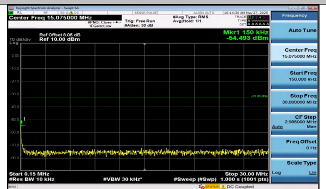
Band2-5MHz-16QAM-18900-1RB#24-0.15~30-PASS
