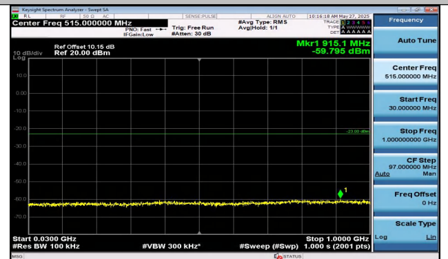
Band2-5MHz-16QAM-18900-25RB#0-30~1000-PASS
