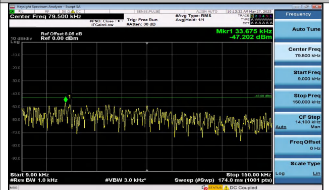
Band2-5MHz-QPSK-18900-1RB#24-0.009~0.15-PASS
