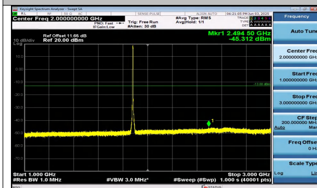
Band2-5MHz-16QAM-18900-25RB#0-1000~3000-PASS
