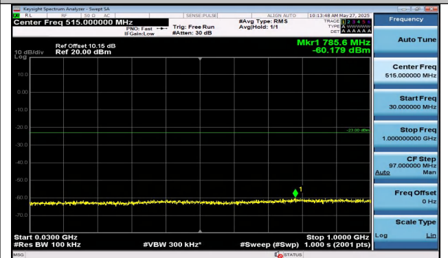
Band2-5MHz-QPSK-18900-1RB#24-30~1000-PASS
