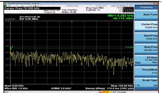
Band2-5MHz-16QAM-18625-1RB#0-0.009~0.15-PASS
