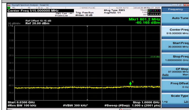
Band2-5MHz-QPSK-18625-25RB#0-30~1000-PASS
