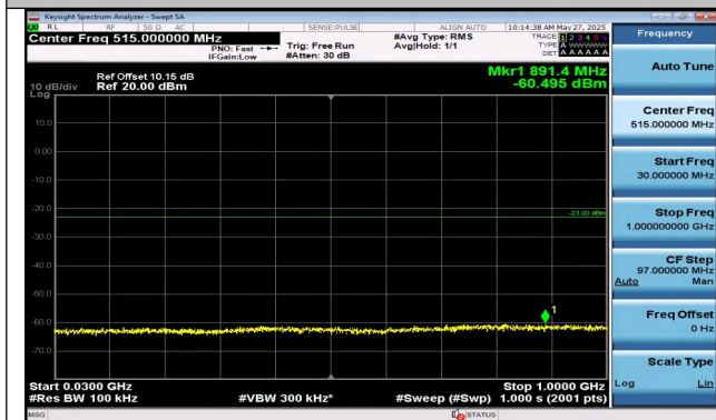
Band2-5MHz-16QAM-18900-1RB#24-30~1000-PASS
