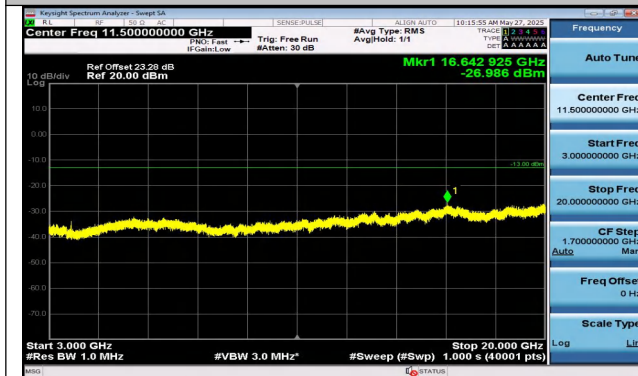
Band2-5MHz-QPSK-18900-25RB#0-3000~20000-PASS
