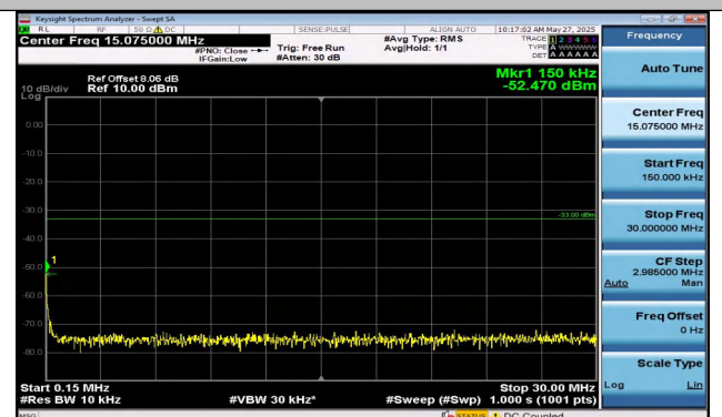
Band2-5MHz-QPSK-19175-1RB#0-0.15~30-PASS
