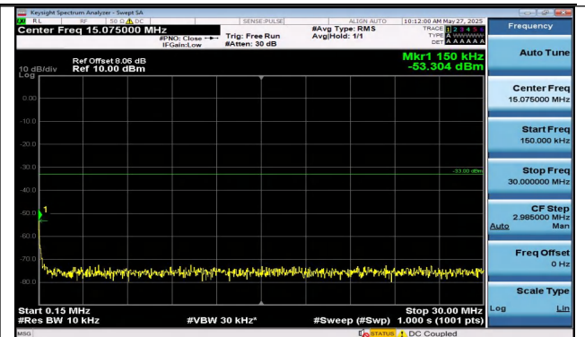
Band2-5MHz-QPSK-18900-1RB#0-0.15~30-PASS
