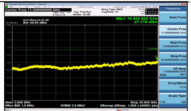
Band2-5MHz-QPSK-18900-1RB#24-3000~20000-PASS
