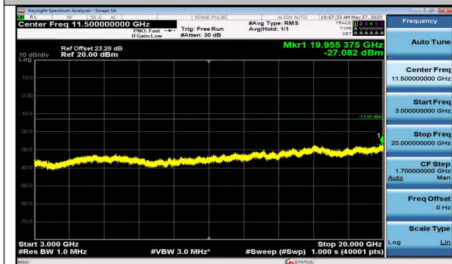
Band2-5MHz-QPSK-18625-1RB#0-3000~20000-PASS
