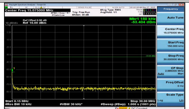
Band2-5MHz-QPSK-18625-25RB#0-0.15~30-PASS
