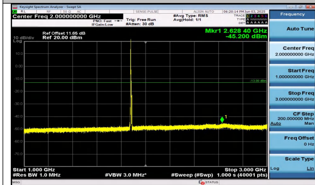
Band2-5MHz-16QAM-18900-1RB#0-1000~3000-PASS
