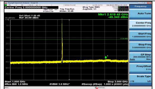
Band2-5MHz-QPSK-18900-1RB#0-1000~3000-PASS
