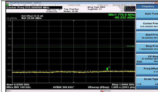
Band2-5MHz-QPSK-18900-25RB#0-30~1000-PASS
