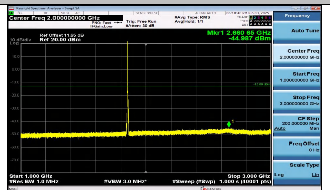
Band2-5MHz-QPSK-18625-1RB#0-1000~3000-PASS
