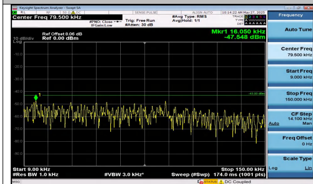
Band2-5MHz-16QAM-18900-1RB#24-0.009~0.15-PASS
