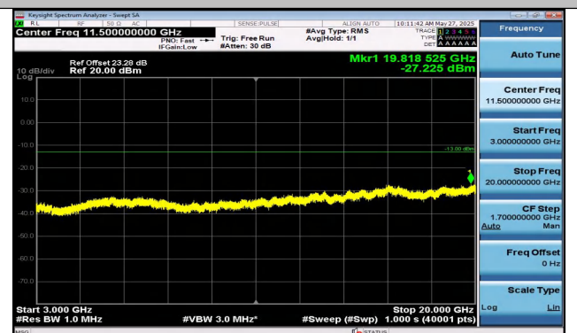
Band2-5MHz-16QAM-18625-25RB#0-3000~20000-PASS
