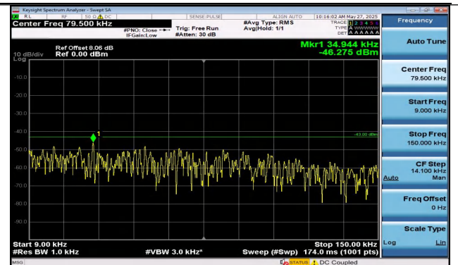
Band2-5MHz-16QAM-18900-25RB#0-0.009~0.15-PASS
