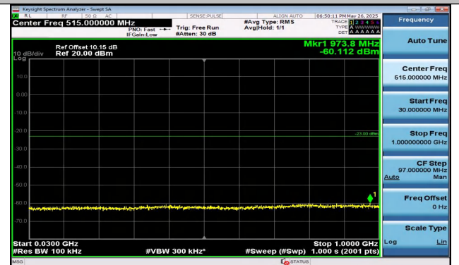
Band2-3MHz-16QAM-19185-1RB#0-30~1000-PASS
