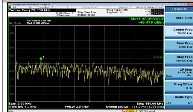
Band2-3MHz-QPSK-19185-15RB#0-0.009~0.15-PASS
