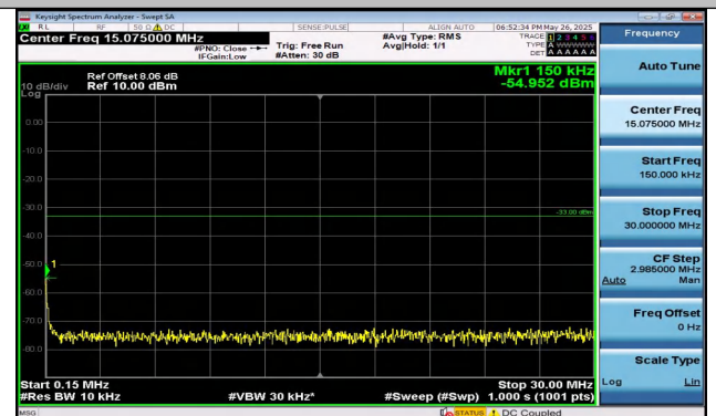
Band2-3MHz-QPSK-19185-15RB#0-0.15~30-PASS
