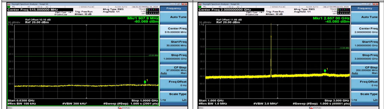
Band2-3MHz-16QAM-19185-1RB#14-30~1000-PASS
