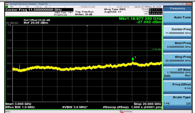
Band2-3MHz-QPSK-19185-1RB#14-3000~20000-PASS
