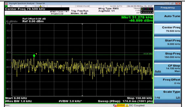
Band2-3MHz-16QAM-19185-1RB#0-0.009~0.15-PASS
