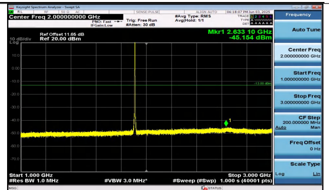
Band2-3MHz-QPSK-19185-15RB#0-1000~3000-PASS
