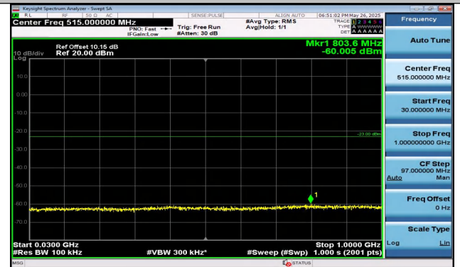
Band2-3MHz-QPSK-19185-1RB#14-0.30~1000-PASS
