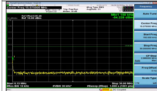
Band2-3MHz-QPSK-19185-1RB#14-0.15~30-PASS
