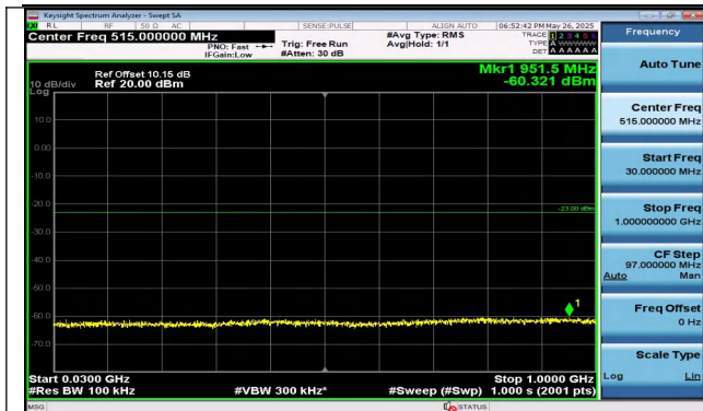
Band2-3MHz-QPSK-19185-15RB#0-30~1000-PASS
