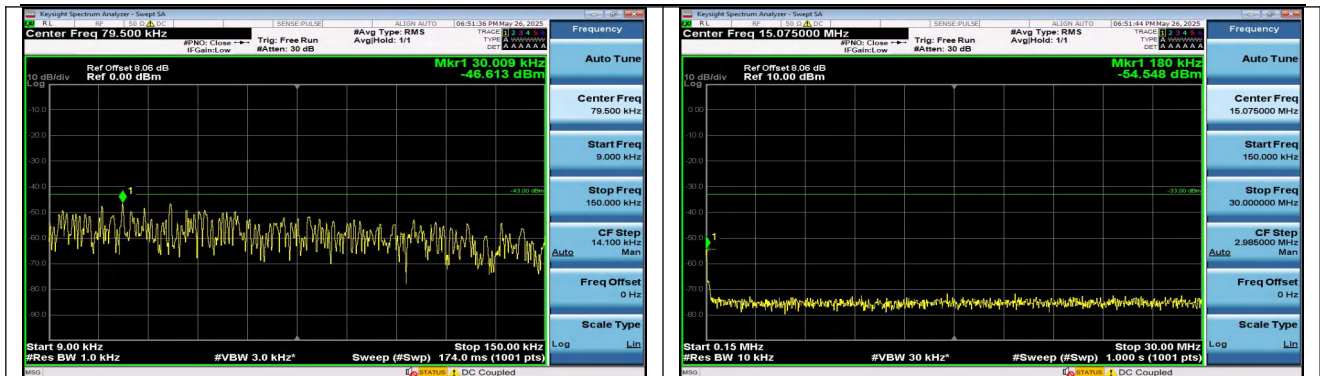
Band2-3MHz-16QAM-19185-1RB#14-0.009~0.15-PASS
