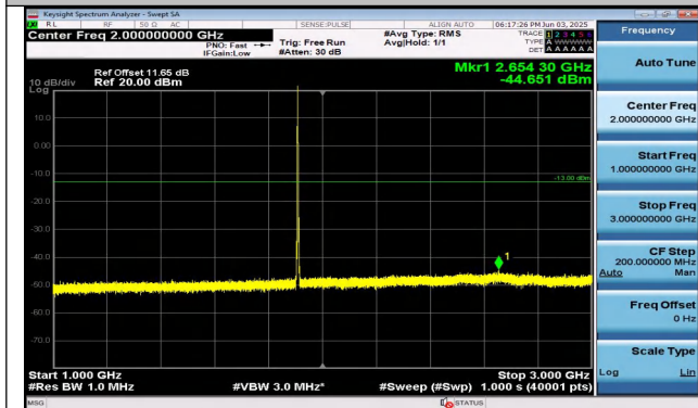
Band2-3MHz-16QAM-19185-1RB#0-1000~3000-PASS
