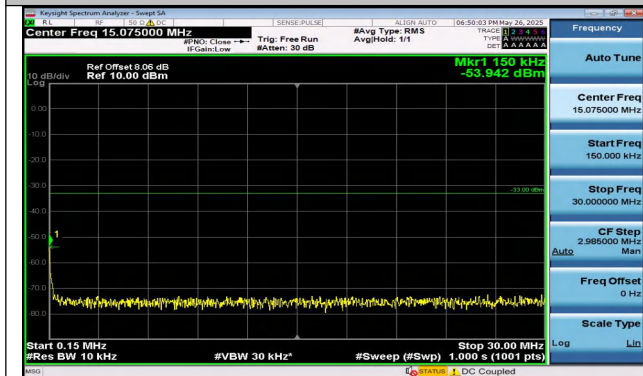
Band2-3MHz-16QAM-19185-1RB#0-0.15~30-PASS
