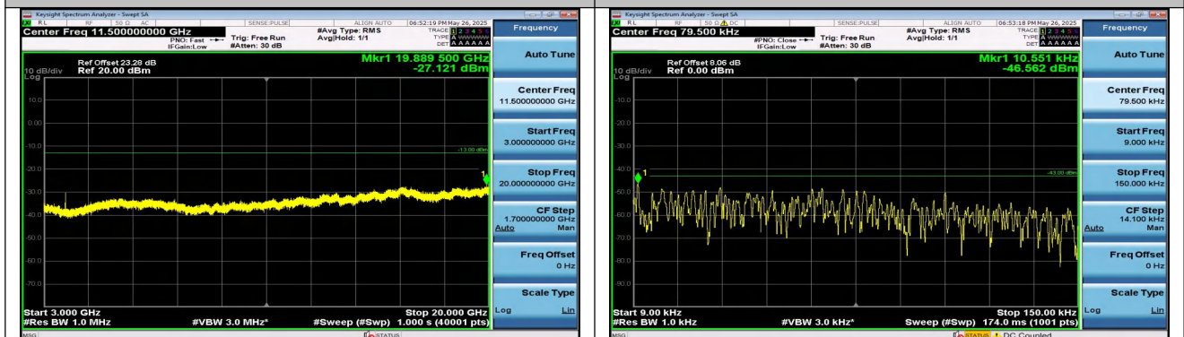
Band2-3MHz-16QAM-19185-1RB#14-3000~20000-PASS
