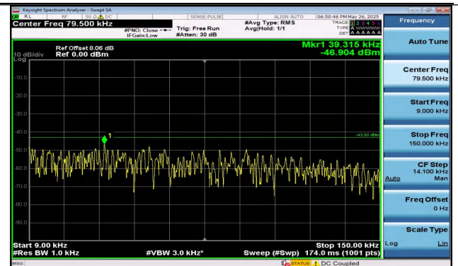
Band2-3MHz-QPSK-19185-1RB#14-0.009~0.15-PASS
