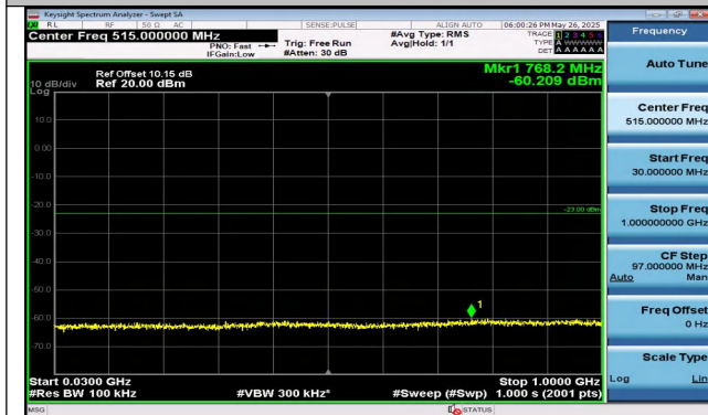
Band2-1.4MHz-QPSK-19193-1RB#0-30~1000-PASS
