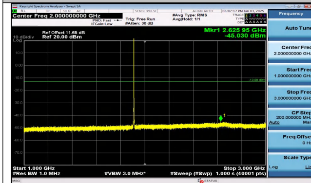
Band2-1.4MHz-16QAM-19193-1RB#0-1000~3000-PASS
