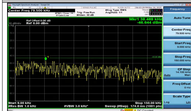
Band2-1.4MHz-QPSK-19193-6RB#0-0.009~0.15-PASS
