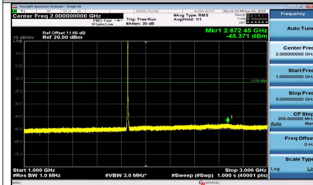
Band2-3MHz-16QAM-18615-15RB#0-1000~3000-PASS
