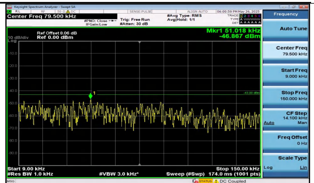
Band2-1.4MHz-16QAM-19193-1RB#0-0.009~0.15-PASS
