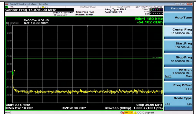
Band2-3MHz-QPSK-18900-1RB#0-0.15~30-PASS
