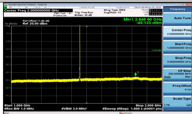
Band2-1.4MHz-QPSK-19193-6RB#0-1000~3000-PASS
