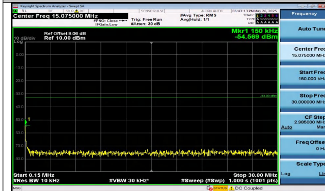
Band2-3MHz-16QAM-18615-15RB#0-0.15~30-PASS
