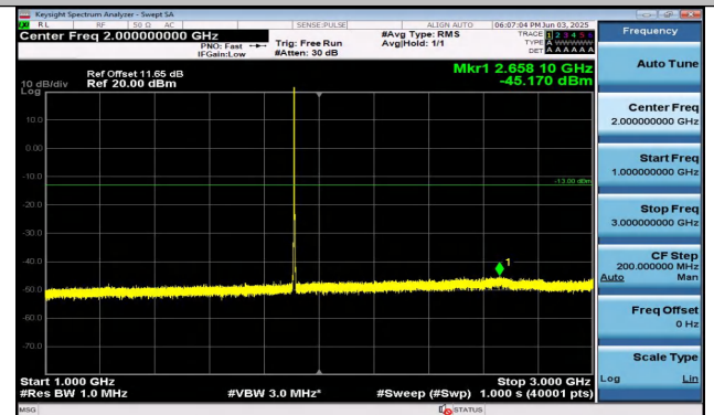
Band2-1.4MHz-QPSK-19193-1RB#0-1000~3000-PASS
