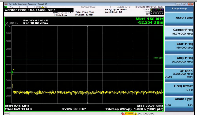
Band2-1.4MHz-16QAM-19193-1RB#5-0.15~30-PASS
