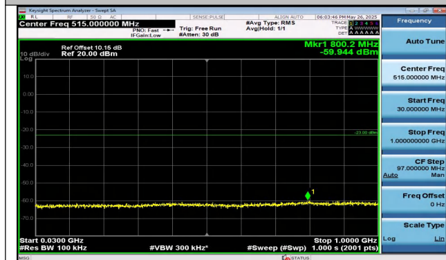
Band2-1.4MHz-QPSK-19193-6RB#0-30~1000-PASS
