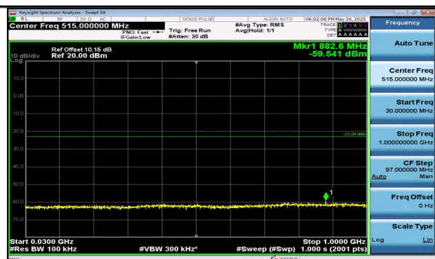
Band2-1.4MHz-QPSK-19193-1RB#5-30~1000-PASS
