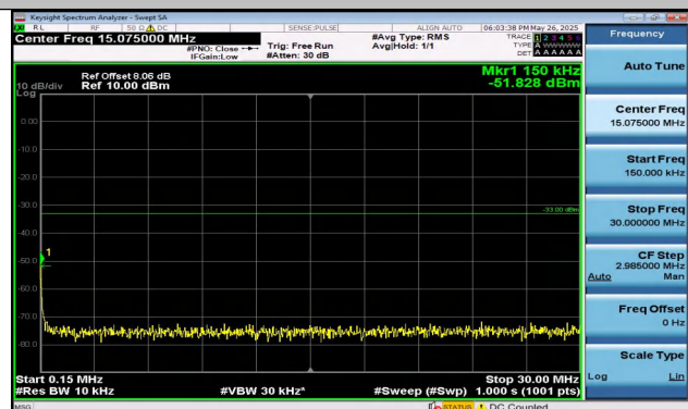
Band2-1.4MHz-QPSK-19193-6RB#0-0.15~30-PASS
