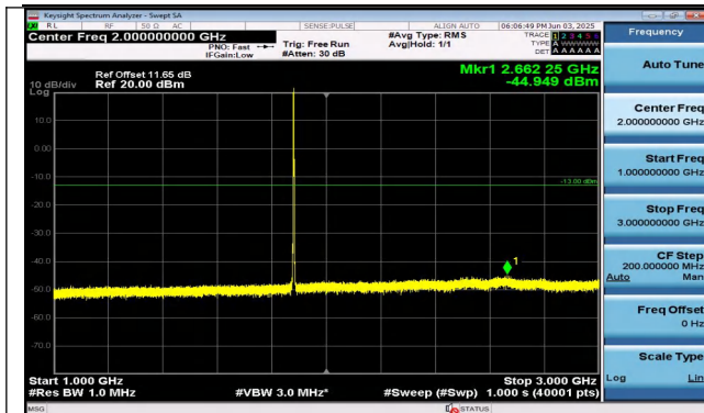
Band2-1.4MHz-16QAM-18900-6RB#0-1000~3000-PASS
