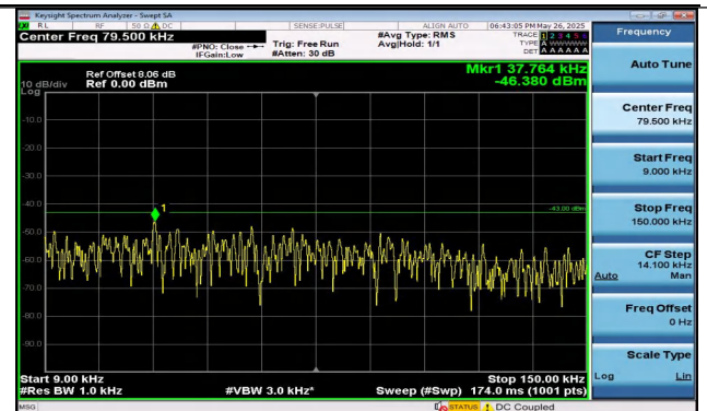
Band2-3MHz-16QAM-18615-15RB#0-0.009~0.15-PASS
