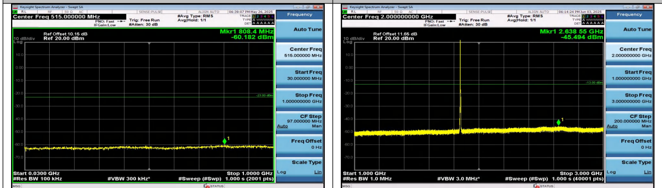
Band2-3MHz-QPSK-18615-1RB#0-30~1000-PASS
