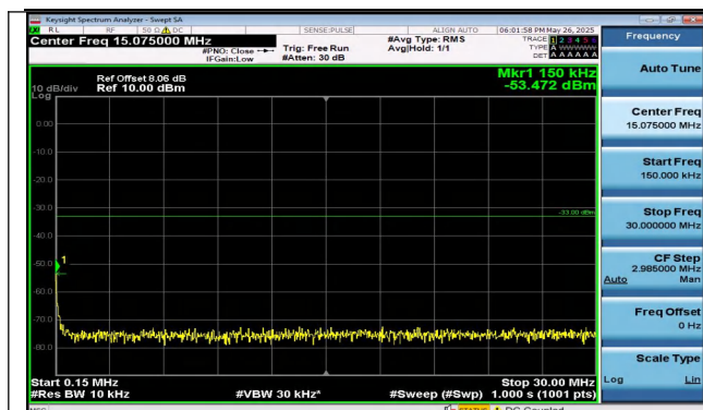
Band2-1.4MHz-QPSK-19193-1RB#5-0.15~30-PASS
