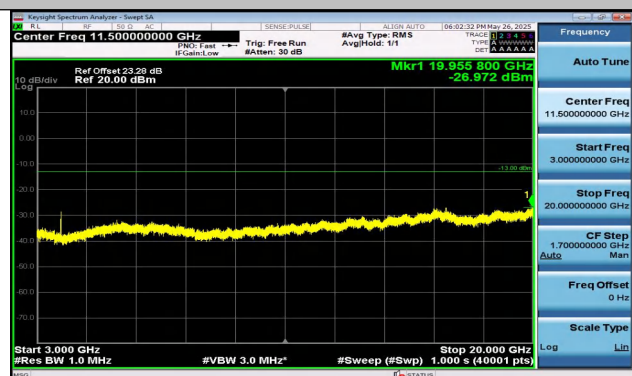
Band2-1.4MHz-QPSK-19193-1RB#5-3000~20000-PASS
