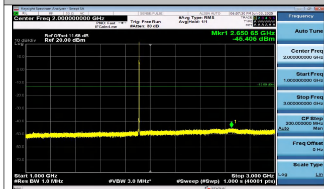
Band2-1.4MHz-QPSK-19193-1RB#5-1000~3000-PASS
