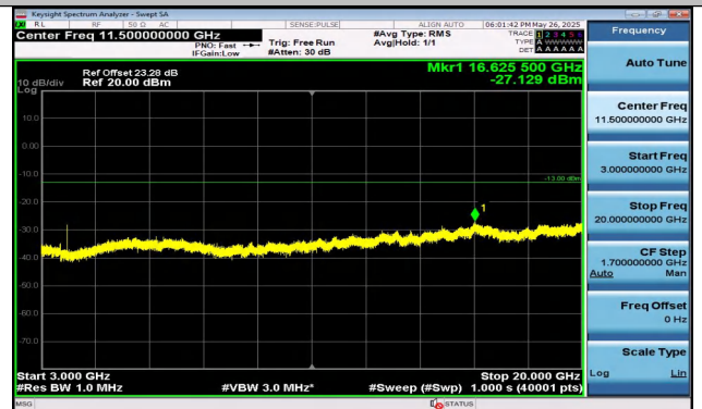
Band2-1.4MHz-16QAM-19193-1RB#0-3000~20000-PASS
