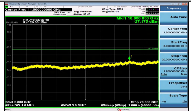
Band2-3MHz-16QAM-18615-15RB#0-3000~20000-PASS
