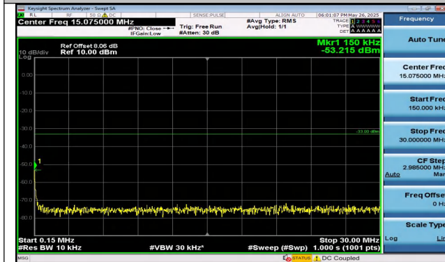
Band2-1.4MHz-16QAM-19193-1RB#0-0.15~30-PASS
