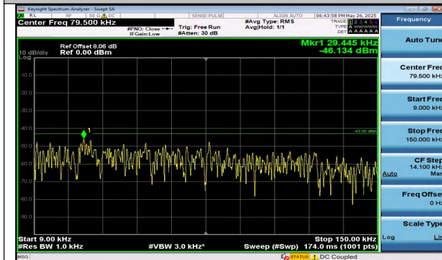
Band2-3MHz-QPSK-18900-1RB#0-0.009~0.15-PASS
