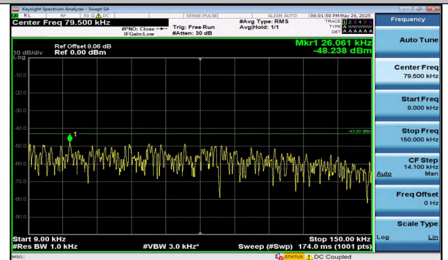
Band2-1.4MHz-QPSK-19193-1RB#5-0.009~0.15-PASS
