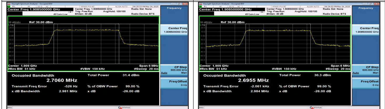
Band2-3MHz-QPSK-19185-15RB#0-PASS
