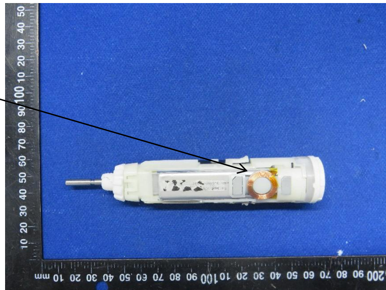
Charging RX
