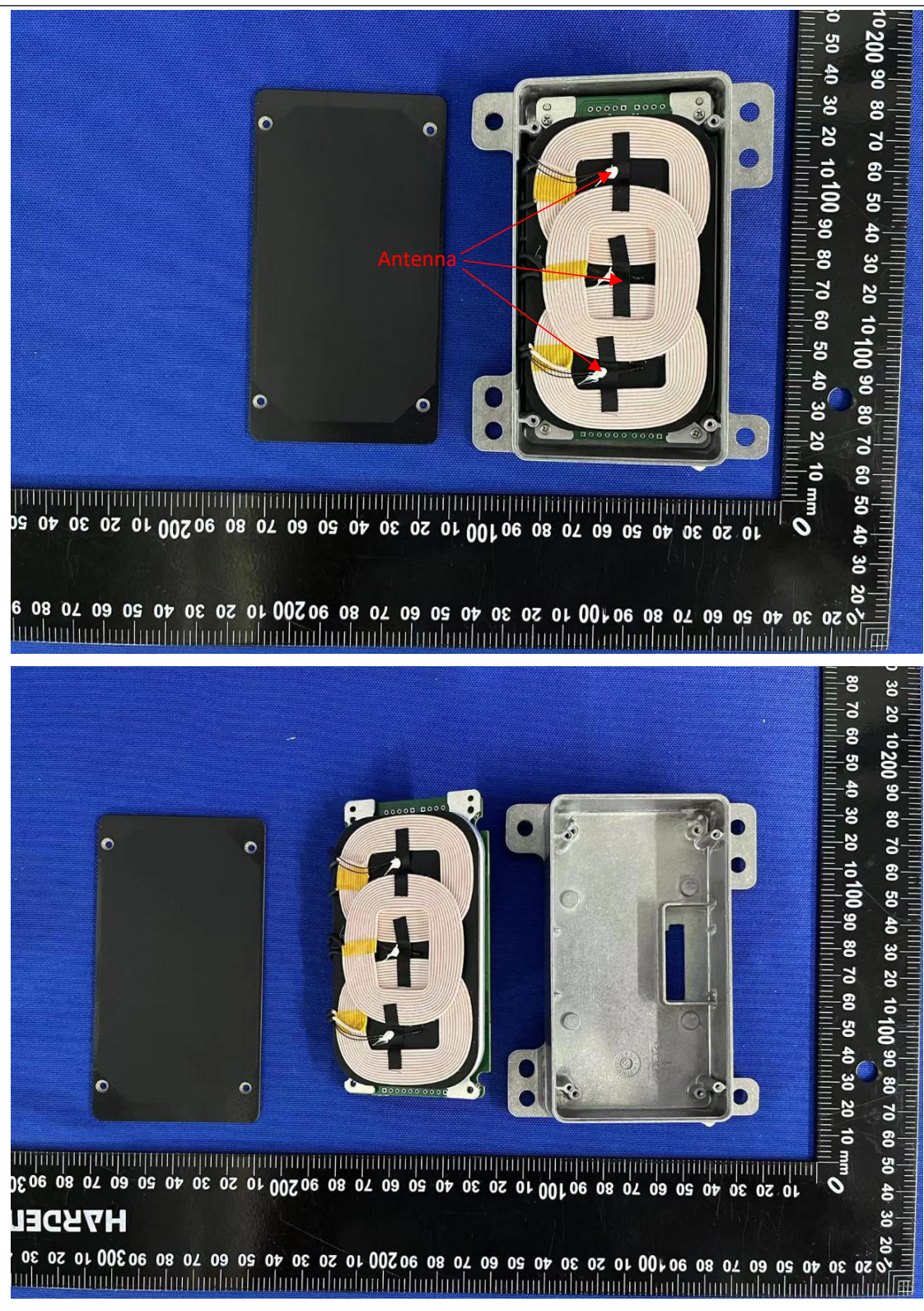
Internal Photo
