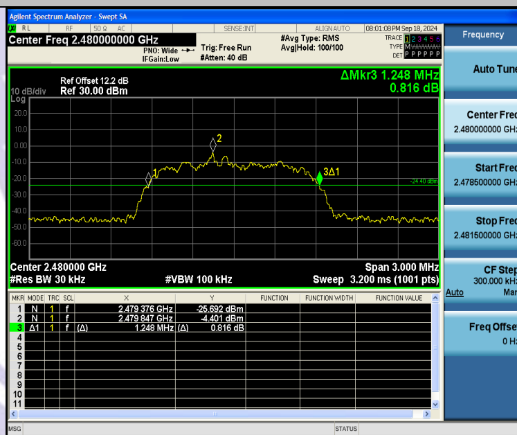
2DH5-Ant1-2480
