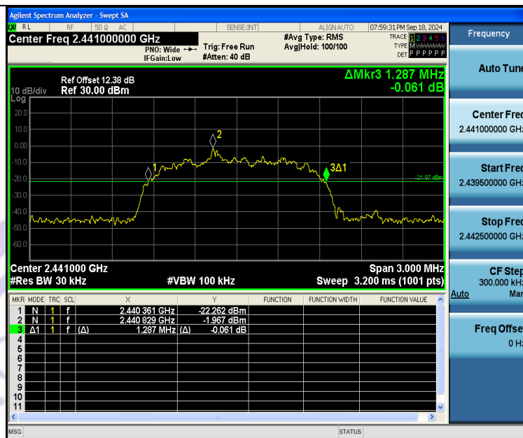
2DH5-Ant1-2441
