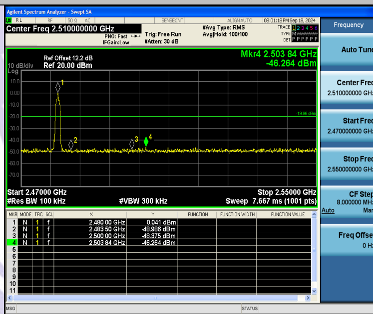
2DH5-Ant1-2480-PASS
