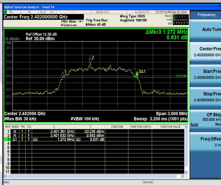
2DH5-Ant1-2402
