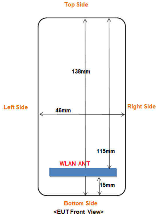
Fig 7.1 Block Diagram for EUT Antenna Position
