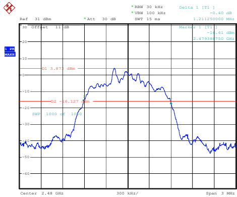
3DH1_High 1.211MHz
