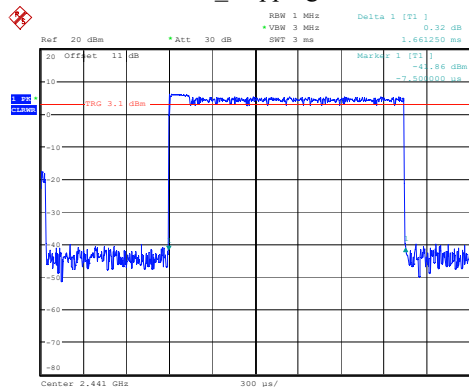
2DH3_Hopping 1.661ms
