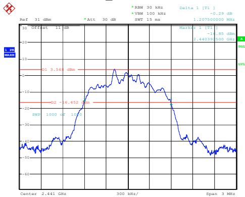
3DH1_Middle 1.208MHz
