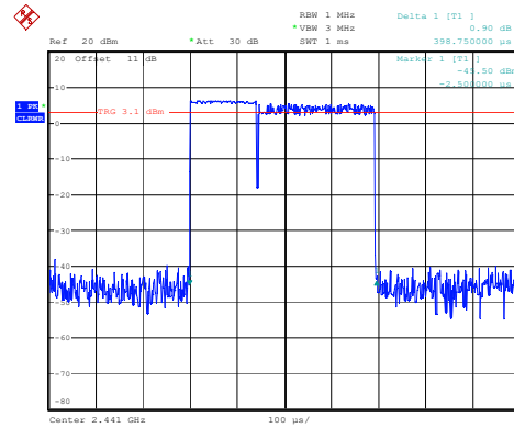
2DH1_Hopping 0.399ms
