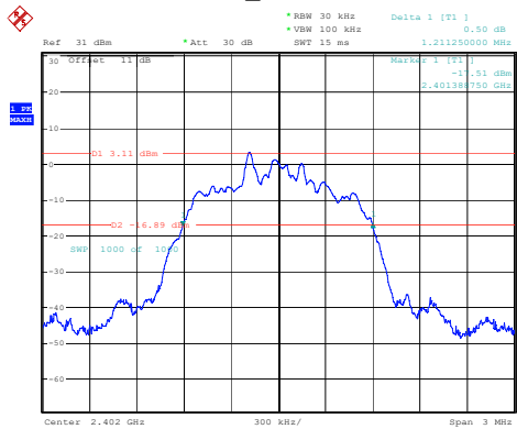
3DH1_Low 1.211MHz
