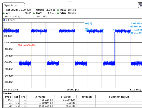
802.11a_5200MHz
