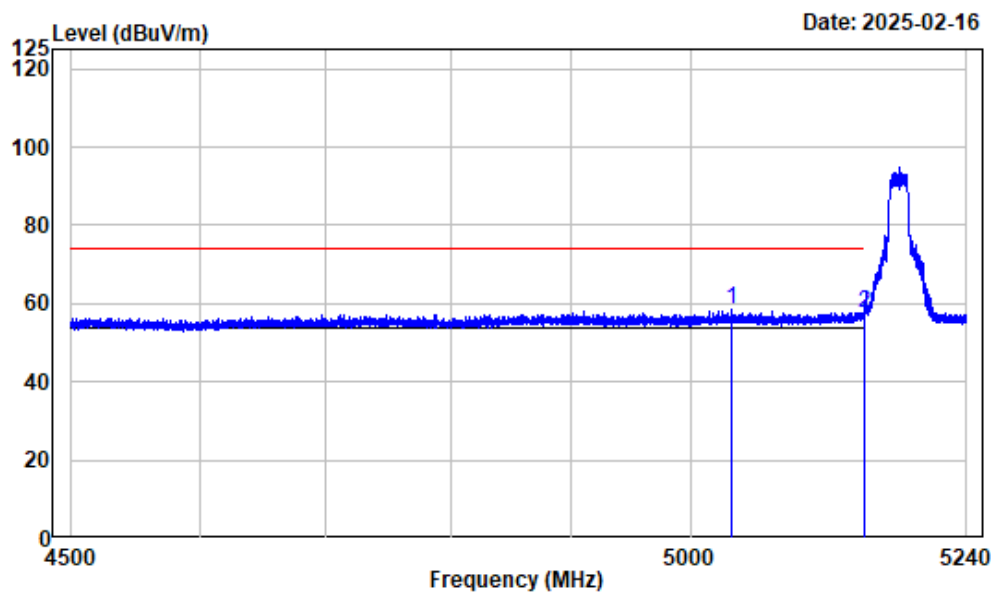
Left Band edge_Horizontal_Peak_802.11a_5180MHz
