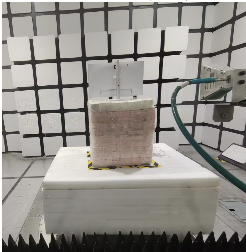
Radiated Emissions View (18-40 GHz)
