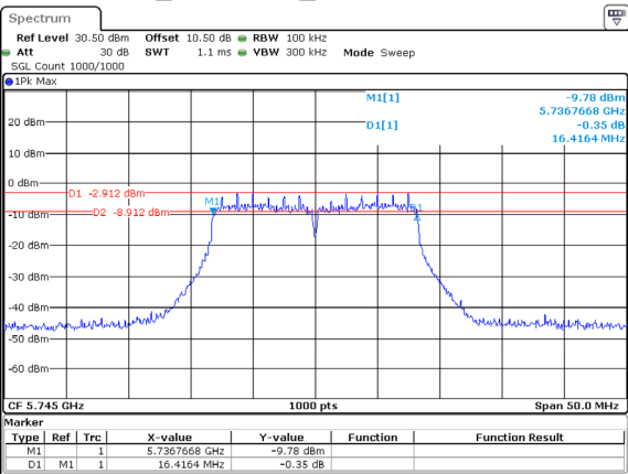
802.11a_5745MHz_Chain 1 16.416MHz
