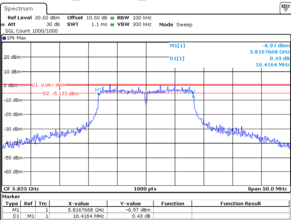
802.11a_5825MHz_Chain 1 16.416MHz
