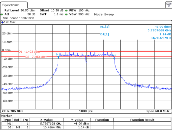
802.11a_5785MHz_Chain 0 16.416MHz
