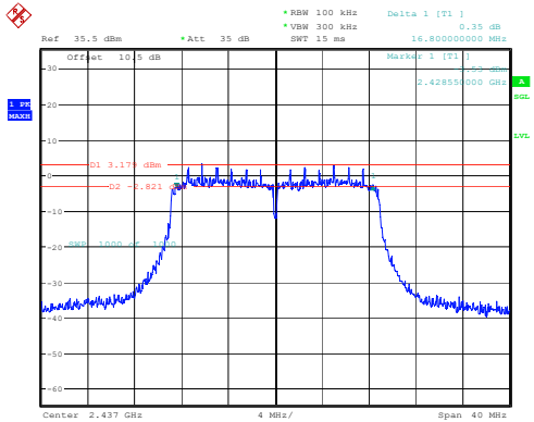
802.11n20_2437MHz_Chain 1 16.800MHz
