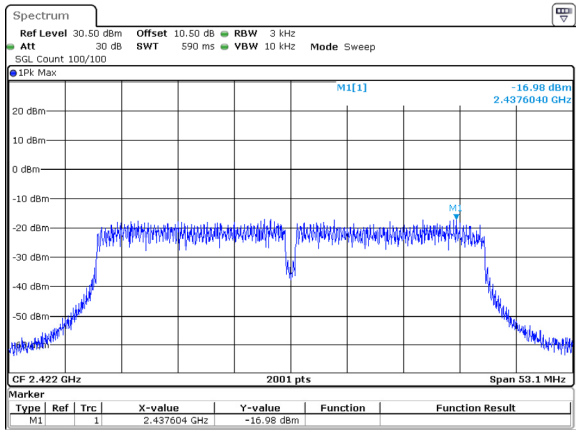
802.11n40_2422MHz_Chain 1 -16.98dBm/3kHz
