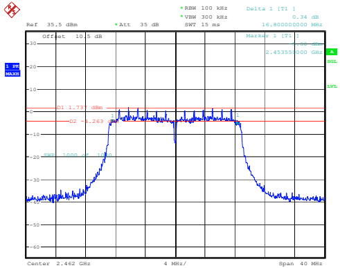
802.11n20_2462MHz_Chain 1 16.800MHz
