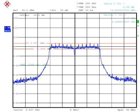
802.11g_2437MHz_Chain 0 16.400MHz
