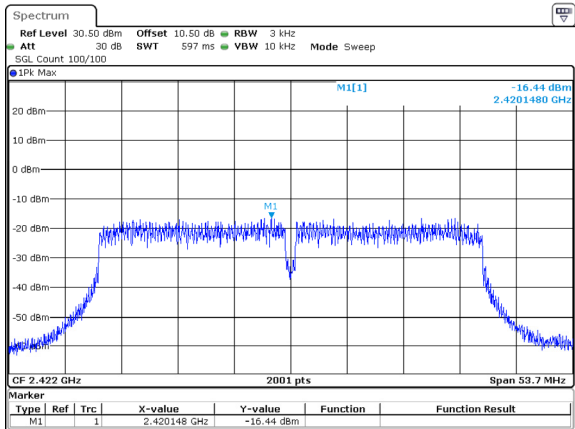
802.11n40_2422MHz_Chain 0 -16.44dBm/3kHz
