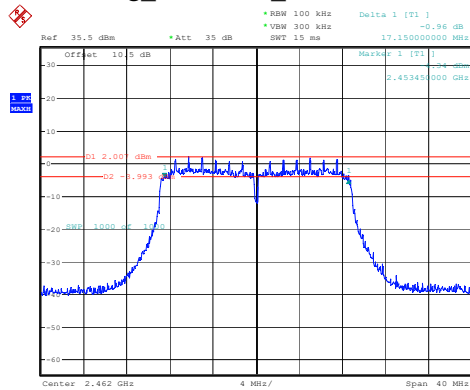
802.11g_2462MHz_Chain 0 17.150MHz
