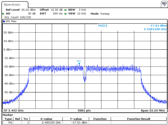
802.11n40_2452MHz_Chain 1 -17.51dBm/3kHz
