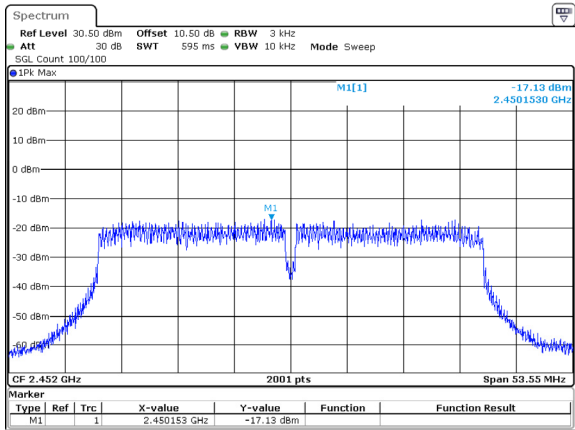
802.11n40_2452MHz_Chain 0 -17.13dBm/3kHz
