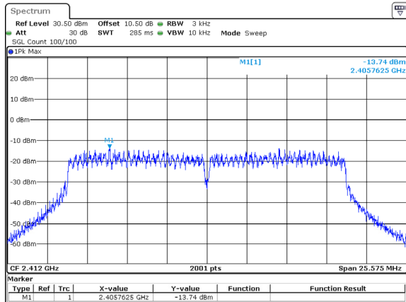
802.11n20_2412MHz_Chain 1 -13.74dBm/3kHz
