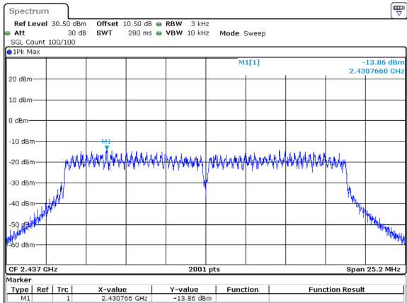
802.11n20_2437MHz_Chain 1 -13.86dBm/3kHz
