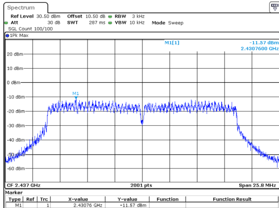
802.11n20_2437MHz_Chain 0 -11.57dBm/3kHz
