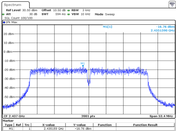
802.11n40_2437MHz_Chain 0 -16.76dBm/3kHz
