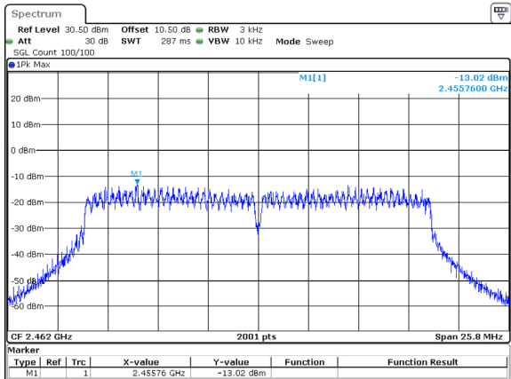
802.11n20_2462MHz_Chain 0 -13.02dBm/3kHz
