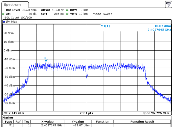
802.11n20_2412MHz_Chain 0 -13.07dBm/3kHz
