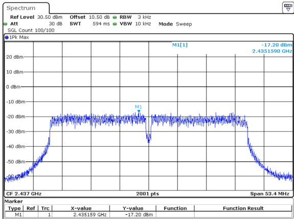
802.11n40_2437MHz_Chain 1 -17.20dBm/3kHz
