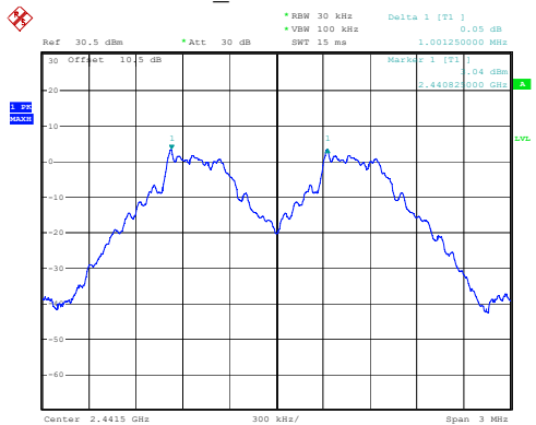
DH1_Middle 1.001MHz
