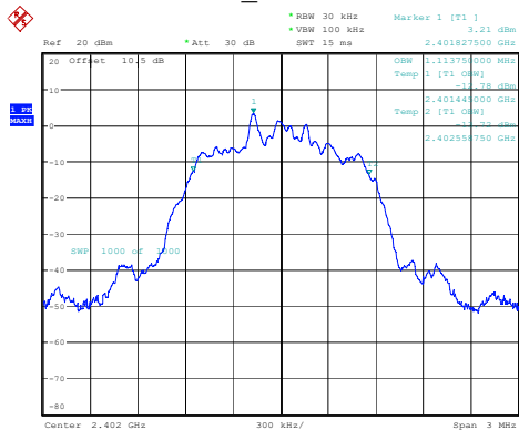
3DH1_Low 1.114MHz
