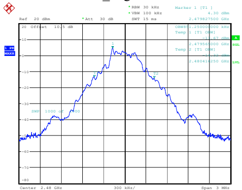
DH1_High 0.851MHz
