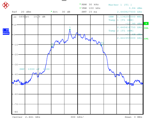
2DH1_Middle 1.136MHz
