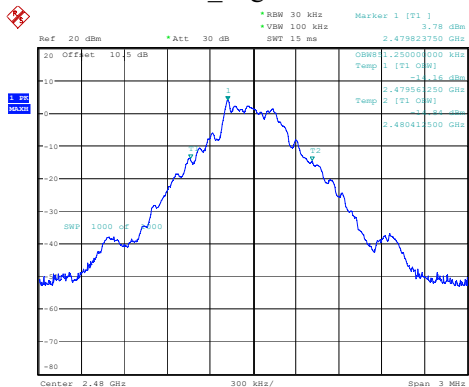
DH1_High 0.851MHz
