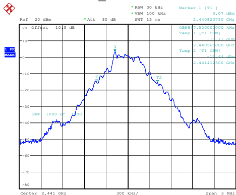
DH1_Middle 0.848MHz
