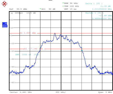
3DH1_Middle 1.211MHz
