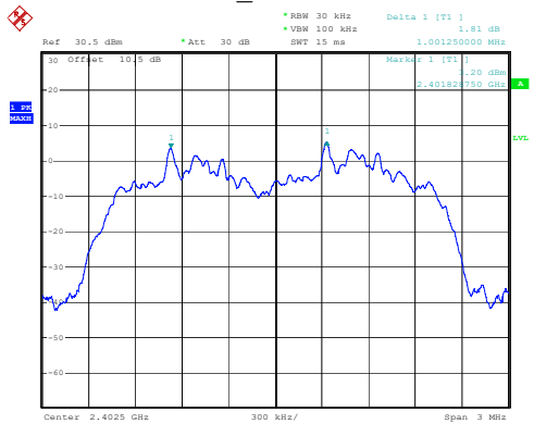
3DH1_Low 1.001MHz
