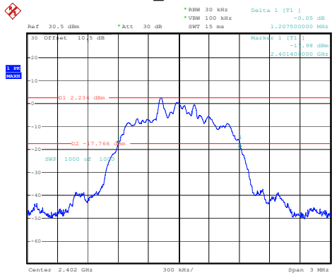
3DH1_Low 1.208MHz
