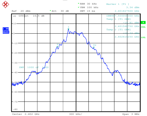
DH1_Low 0.848MHz
