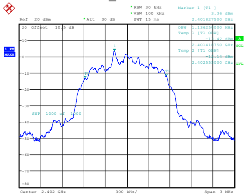
2DH1_Low 1.136MHz
