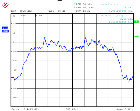
3DH1_Middle 1.001MHz
