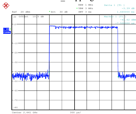
2DH3_Hopping 1.665ms
