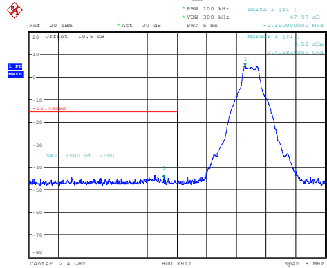
DH1_Low
