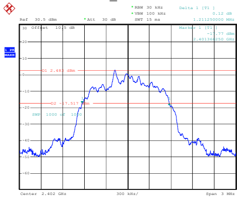
2DH1_Low 1.211MHz
