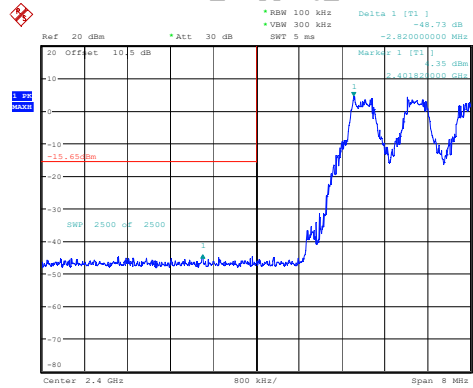
DH1_Hopping_Lower
