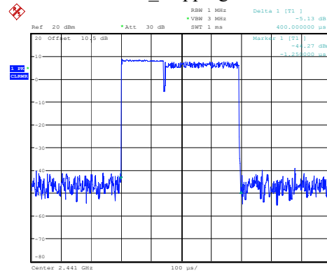
2DH1_Hopping 0.400ms
