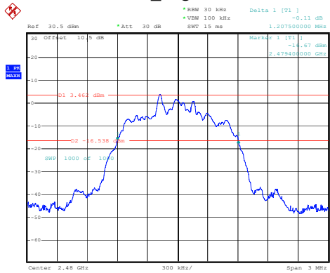
3DH1_High 1.208MHz
