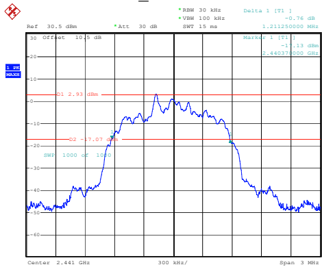
2DH1_Middle 1.211MHz
