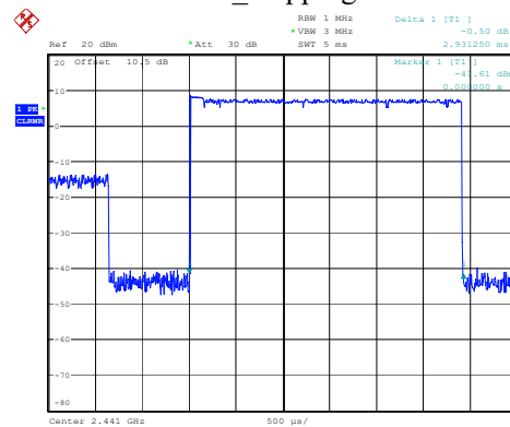
2DH5_Hopping 2.931ms
