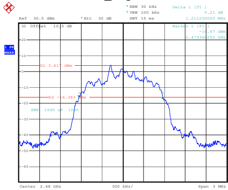
2DH1_High 1.211MHz
