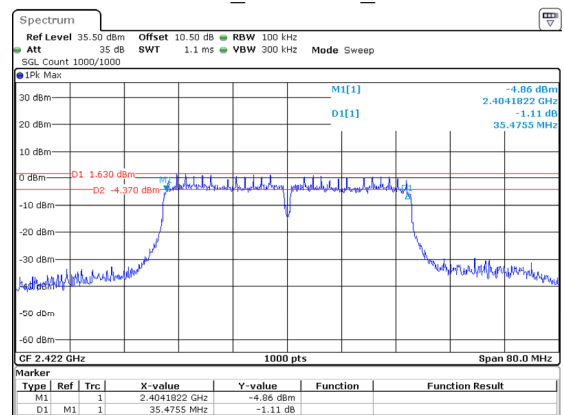
802.11n40_2422MHz_Chain 1
