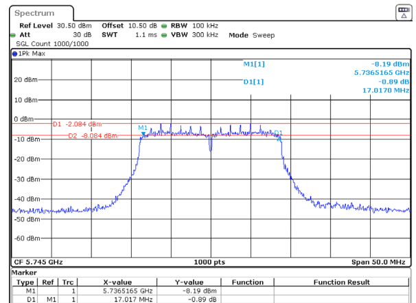
802.11ac20_5745MHz_Chain 1
