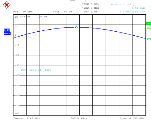
3DH1_High 7.43dBm
