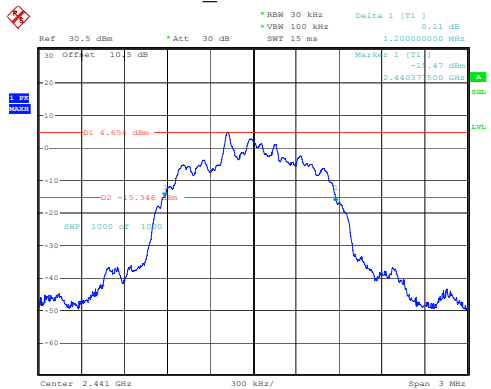
2DH1_Middle 1.200MHz
