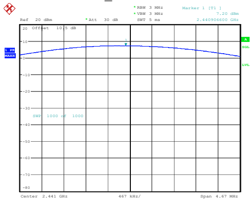
DH1_Middle 7.20dBm
