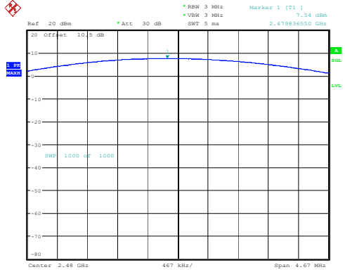
DH1_High 7.54dBm
