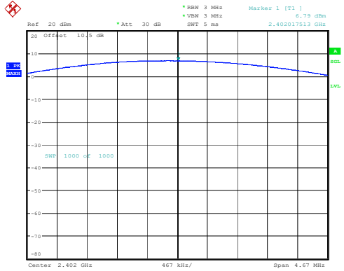
DH1_Low 6.79dBm
