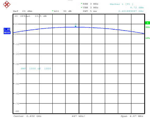
DH1_Low 6.72dBm
