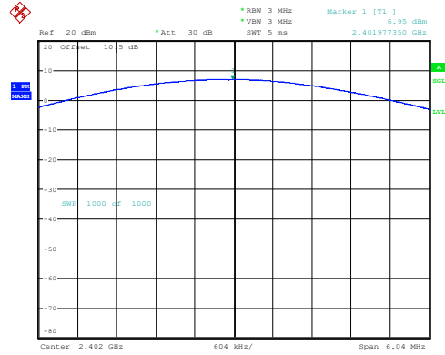
3DH1_Low 6.95dBm
