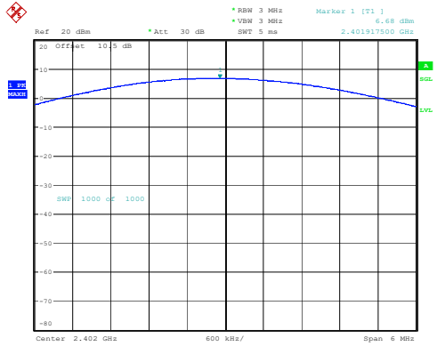
2DH1_Low 6.68dBm
