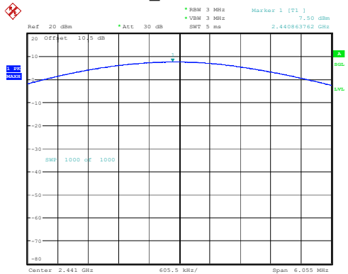
3DH1_Middle 7.50dBm
