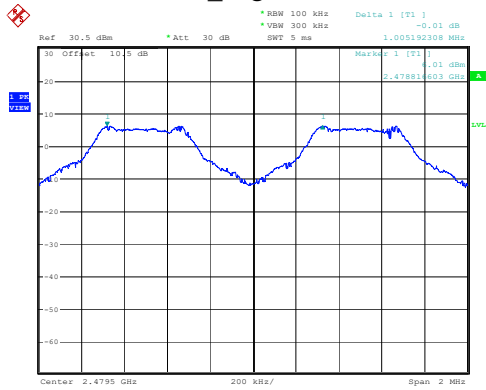
DH1_High 1.005MHz
