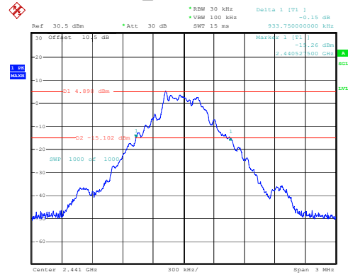
DH1_Middle 0.934MHz
