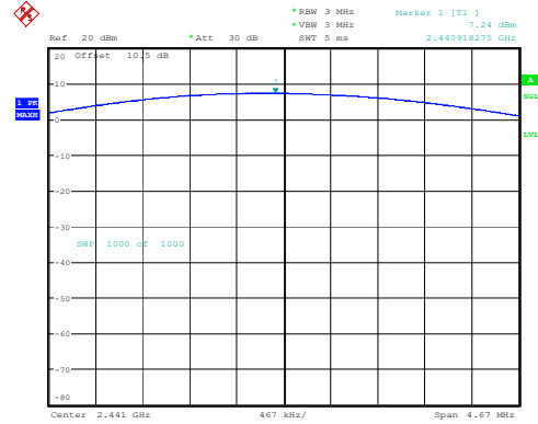
DH1_Middle 7.24dBm
