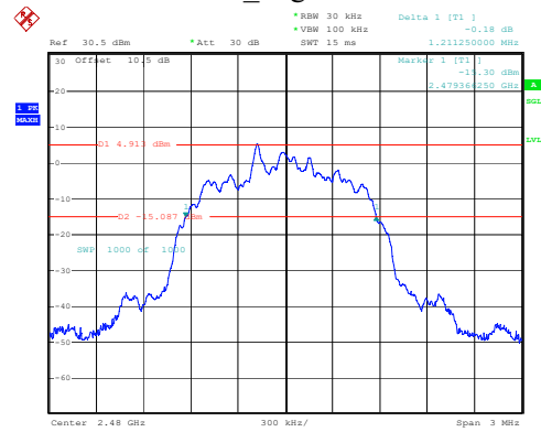
2DH1_High 1.211MHz
