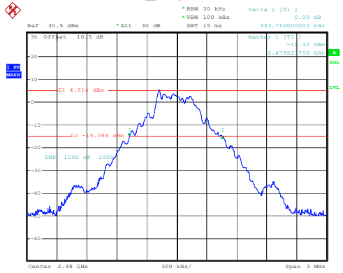
DH1_High 0.934MHz
