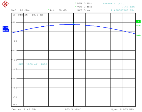
2DH1_High 7.47dBm
