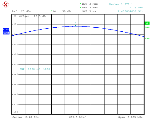
3DH1_High 7.79dBm
