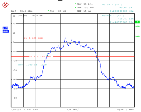
2DH1_Middle 1.200MHz
