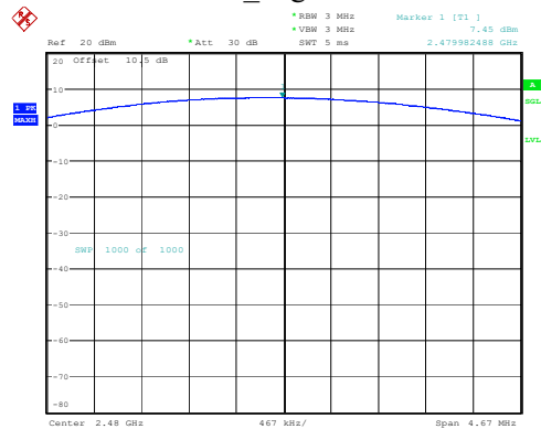
DH1_High 7.45dBm
