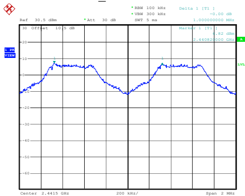
DH1_Middle 1.000MHz
