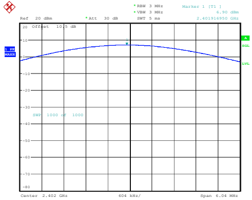
3DH1_Low 6.90dBm
