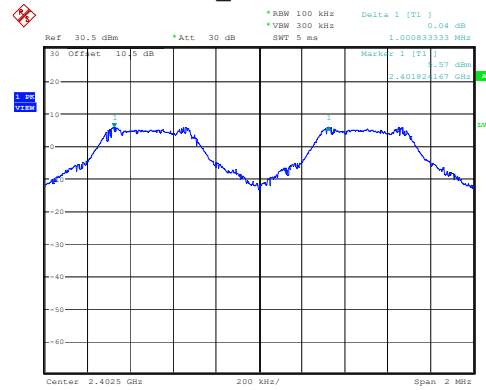
DH1_Low 1.001MHz
