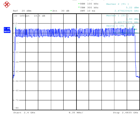
2DH1_Hopping 79
