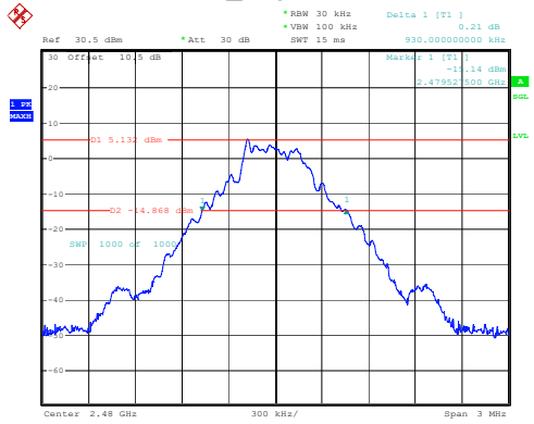
DH1_High 0.930MHz
