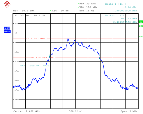
2DH1_Low 1.200MHz
