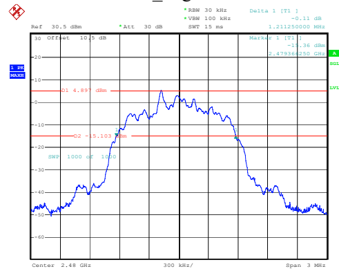
2DH1_High 1.211MHz
