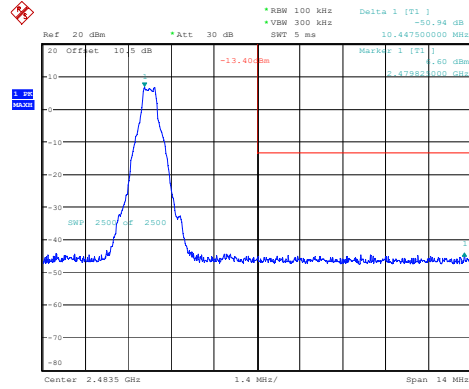
DH1_High
