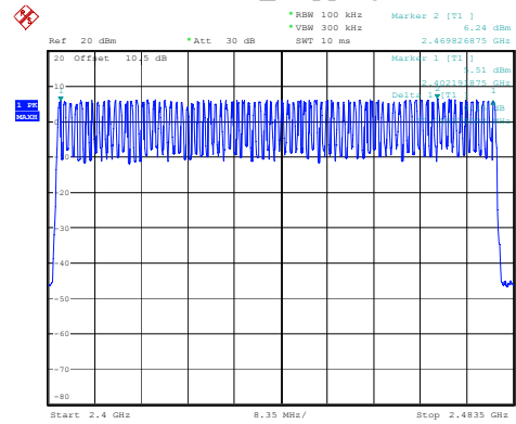
DH1_Hopping 79
