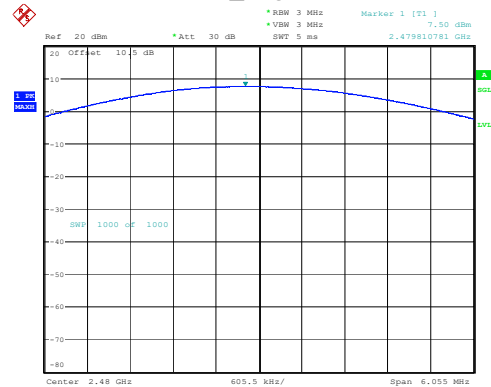
2DH1_High 7.50dBm
