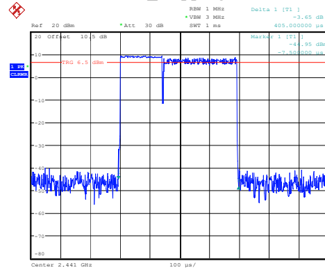
2DH1_Hopping 0.405ms
