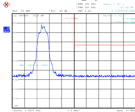
2DH1_High
