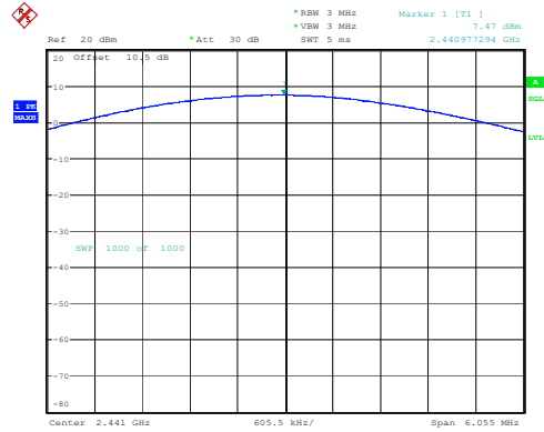
3DH1_Middle 7.47dBm
