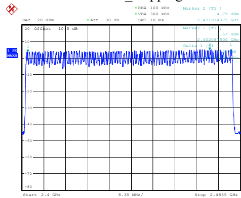
3DH1_Hopping 79
