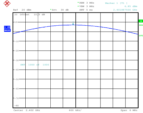
2DH1_Low 6.85dBm
