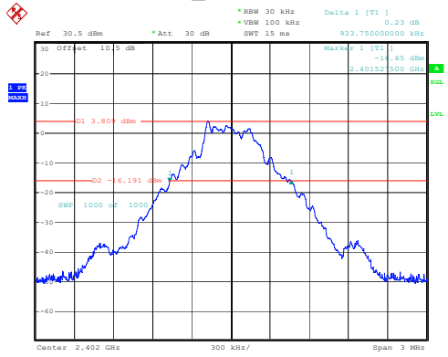
DH1_Low 0.934MHz
