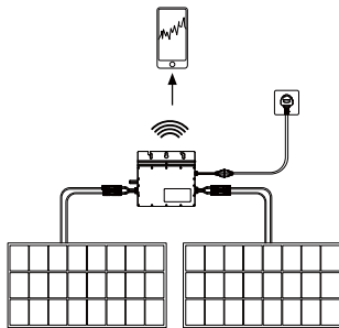
Single Microinverter Connection Diagram
