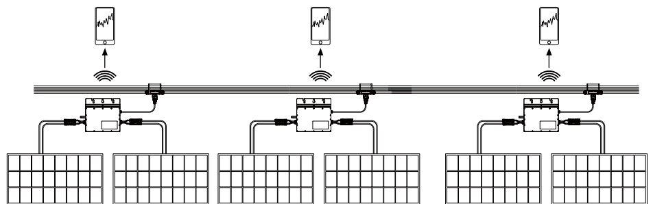
Multiple Microinverter Connection Diagram
