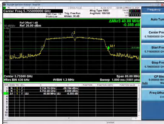
11N40MIMO-Ant2-5755
