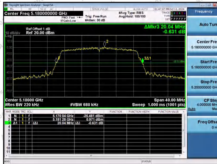
11AC20MIMO-Ant2-5180
