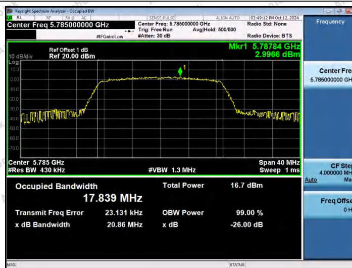
11N20MIMO-Ant1-5785
