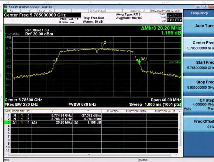
11AC20MIMO-Ant2-5785
