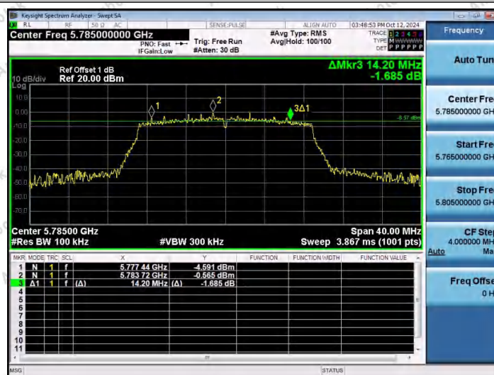
11N20MIMO-Ant1-5785-PASS
